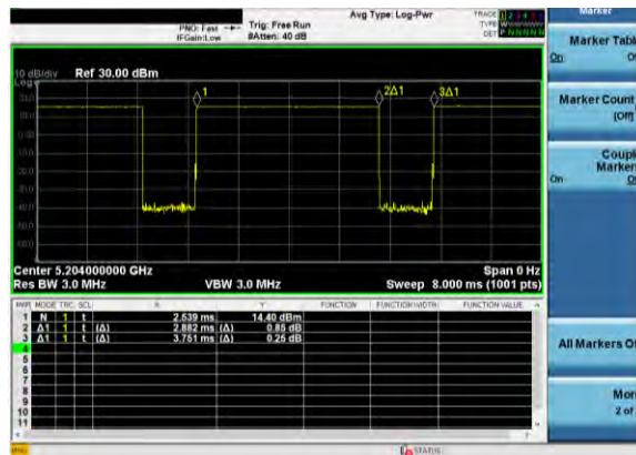
Figure 8-20 NB UNII 1 BDR Transmission Plot – Antenna 3b, Variant 2
