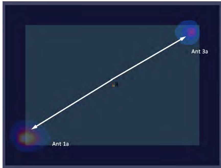
Figure 11-2 Back Side Spatial Separation for Antenna 1a and Antenna 3a
