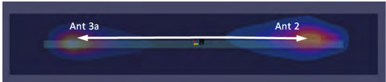
Figure 11-25 Right Edge Spatial Separation for Antenna 2 and Antenna 3a
