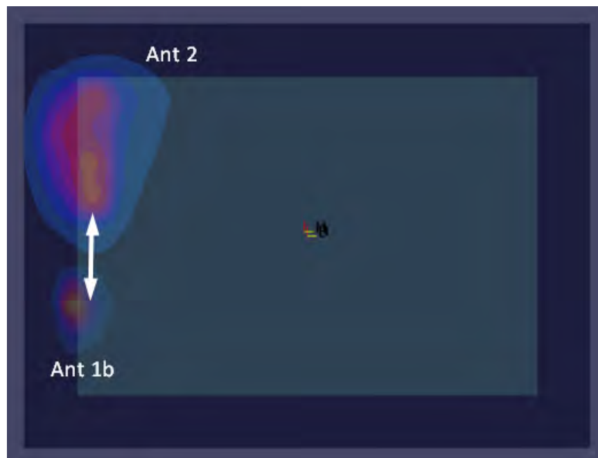
Figure 11-7 Back Side Spatial Separation for Antenna 1b and Antenna 2
