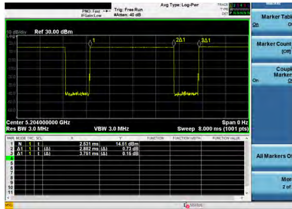
Figure 8-15 NB UNII 1 BDR Transmission Plot – Antenna 5T, Variant 1
