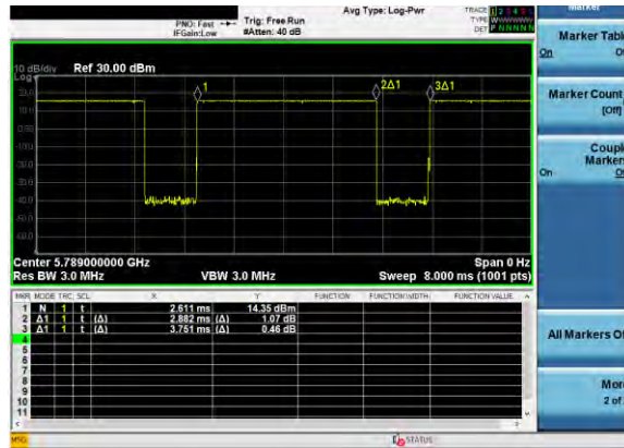
Figure 8-25 NB UNII 3 BDR Transmission Plot – Antenna 3b, Variant 1
