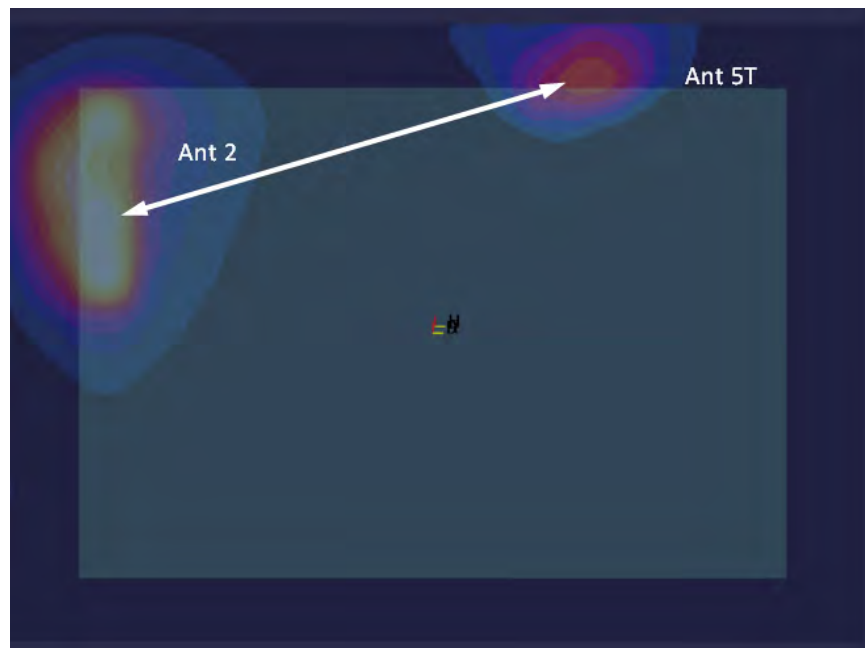
Figure 11-15 Back Side Spatial Separation for Antenna 2 and Antenna 5T
