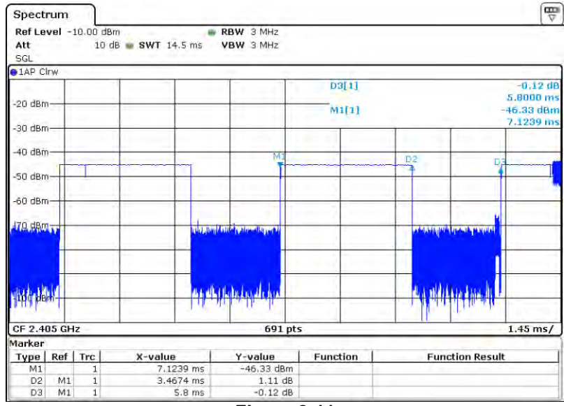
Figure 8-11 802.15.4 Transmission Plot – Antenna 1a, 3a, and 4, Variant 2
