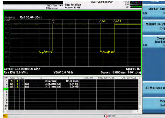
Figure 8-4 Bluetooth Transmission Plot – Antenna 3a, Variant 1
