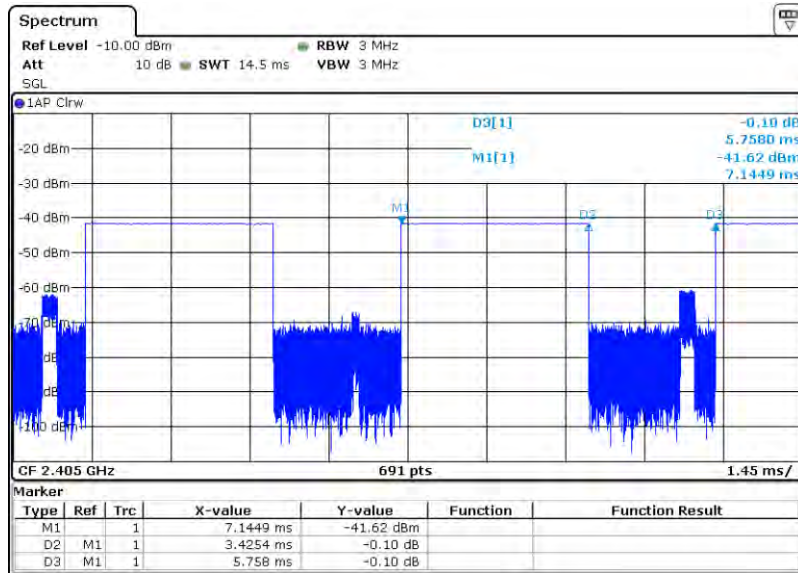
Figure 8-10 802.15.4 Transmission Plot – Antenna 1a, 3a, and 4, Variant 1
