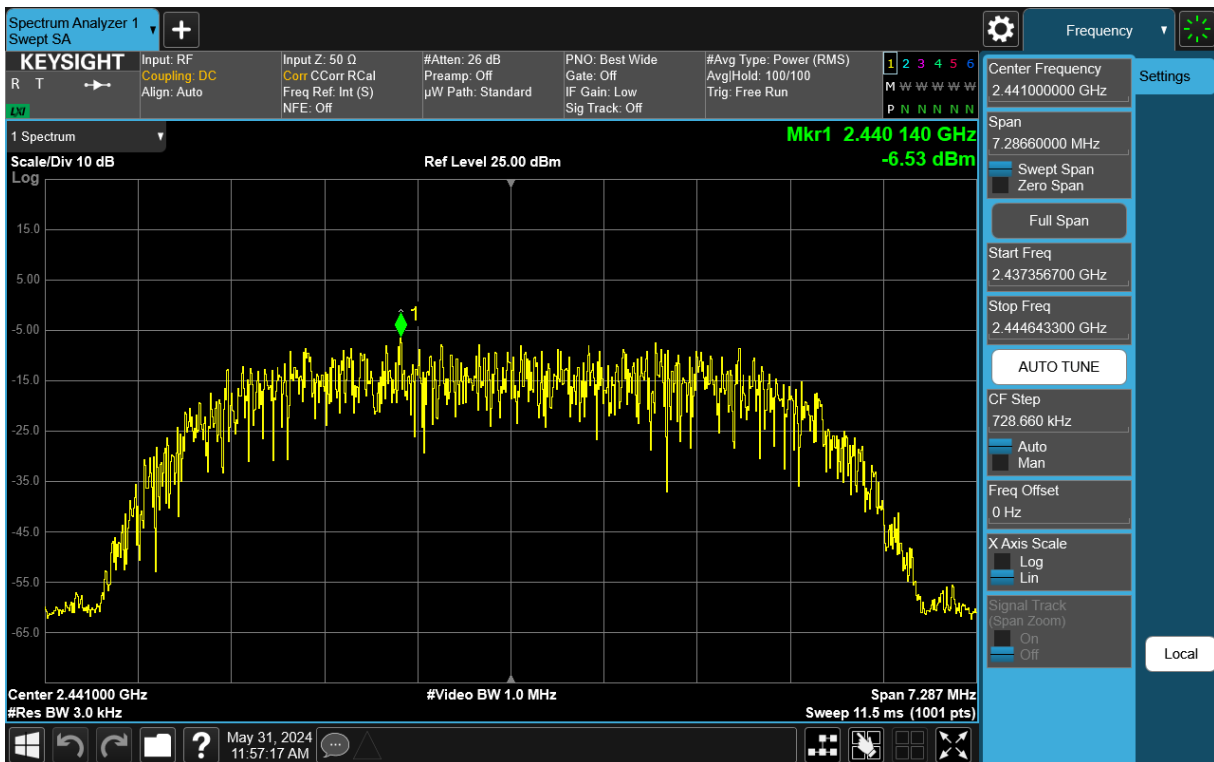
Plot 7-64. Power Spectral Density Plot TxBF Antenna 1a (Bluetooth (HDR8), 8Mbps, ePA – Ch. 38)
