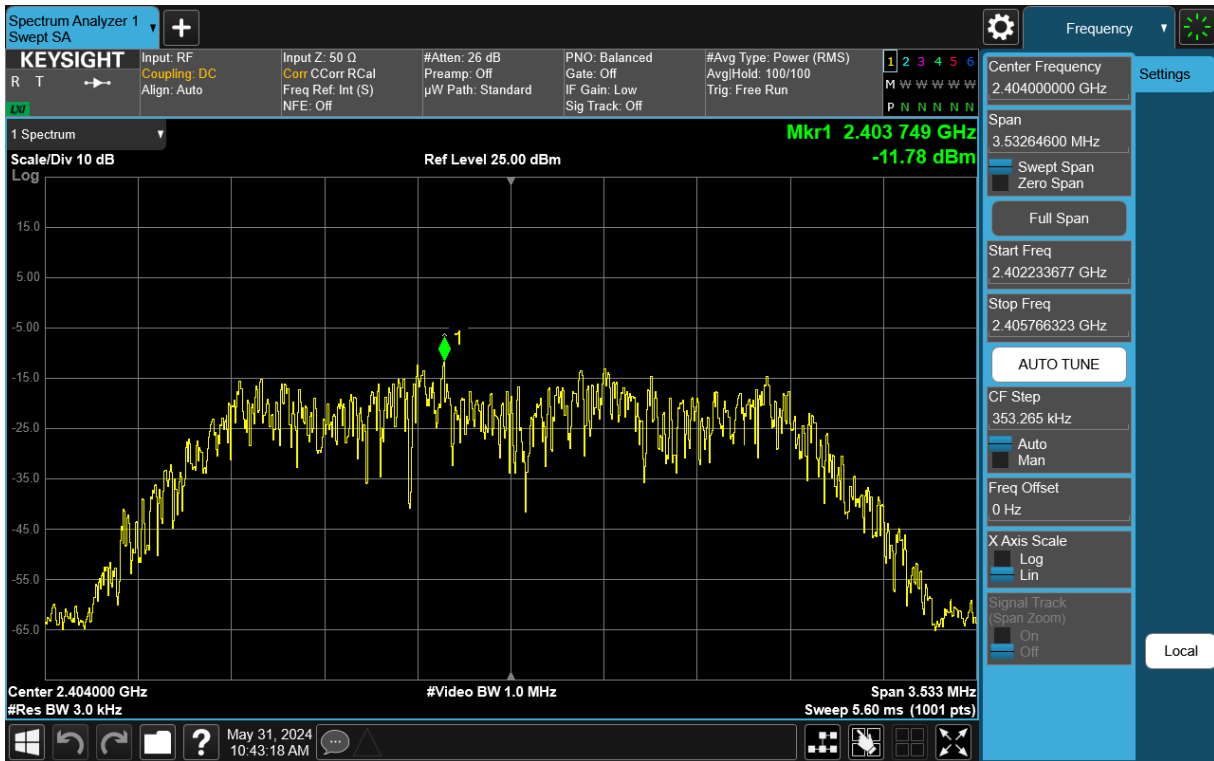
Plot 7-55. Power Spectral Density Plot TxBF Antenna 3a (Bluetooth (HDR4), 4Mbps, iPA – Ch. 1)
