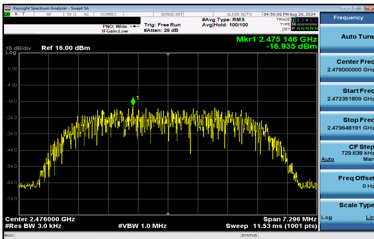
Plot 7-48. Power Spectral Density Plot Antenna 4 (Bluetooth (HDR8), 8Mbps, iPA – Ch. 73)
