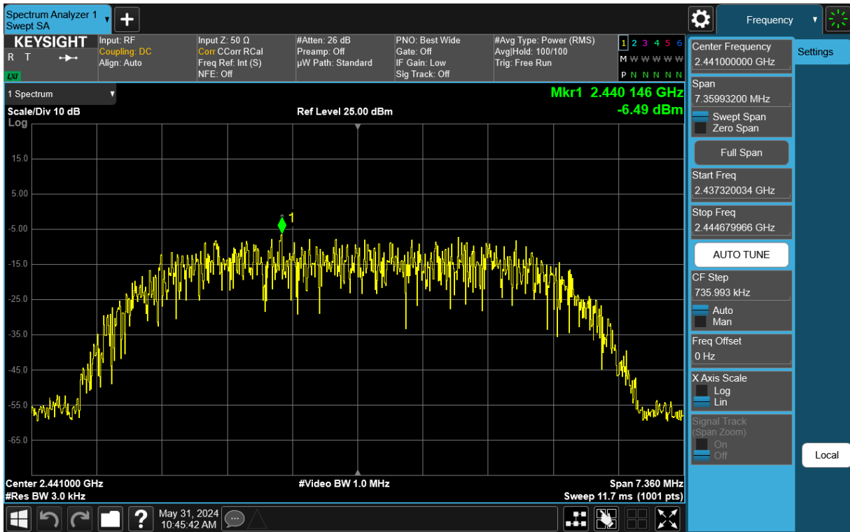
Plot 7-63. Power Spectral Density Plot TxBF Antenna 3a (Bluetooth (HDR8), 8Mbps, ePA – Ch. 38)
