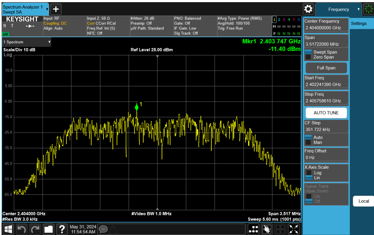
Plot 7-56. Power Spectral Density Plot TxBF Antenna 1a (Bluetooth (HDR4), 4Mbps, iPA – Ch. 1)
