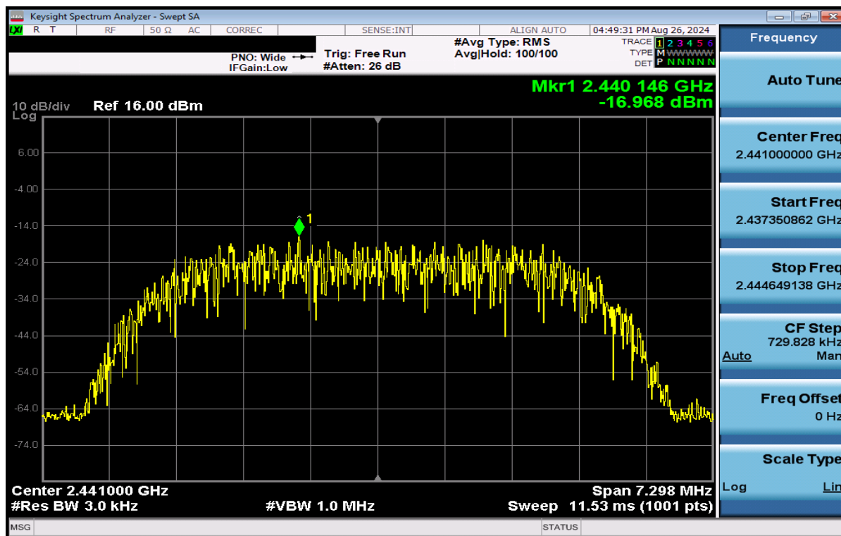
Plot 7-47. Power Spectral Density Plot Antenna 4 (Bluetooth (HDR8), 8Mbps, iPA – Ch. 38)
