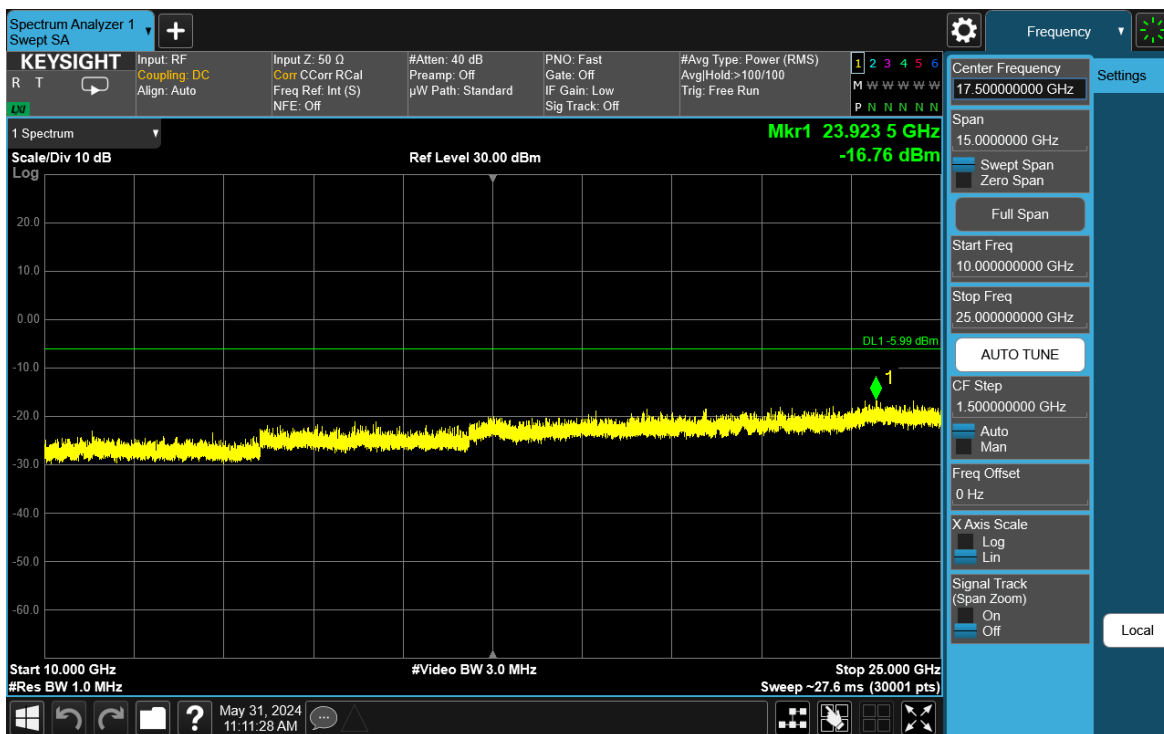
Plot 7-86. Conducted Spurious Plot Antenna 3a (Bluetooth (HDR4), 4 Mbps, ePA – Ch. 1)
