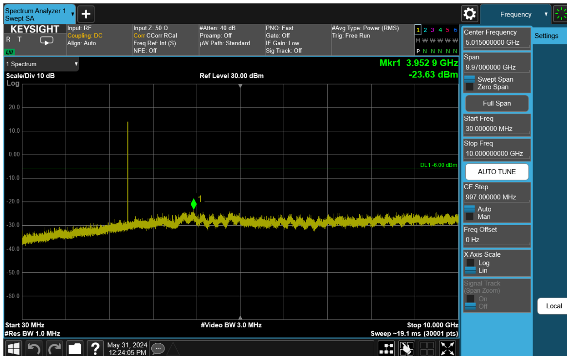
Plot 7-93. Conducted Spurious Plot Antenna 1a (Bluetooth (HDR4), 4 Mbps, ePA – Ch. 38)
