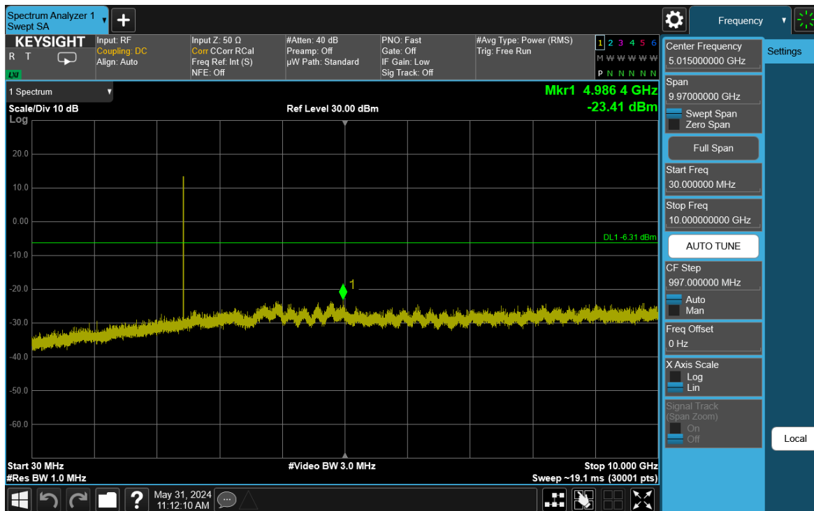
Plot 7-87. Conducted Spurious Plot Antenna 3a (Bluetooth (HDR4), 4 Mbps, ePA – Ch. 38)
