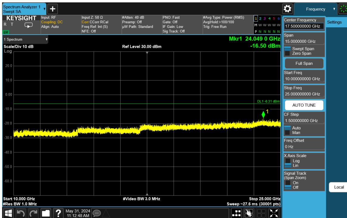
Plot 7-88. Conducted Spurious Plot Antenna 3a (Bluetooth (HDR4), 4 Mbps, ePA – Ch. 38)
