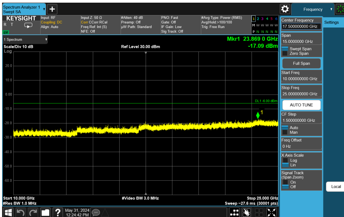
Plot 7-94. Conducted Spurious Plot Antenna 1a (Bluetooth (HDR4), 4 Mbps, ePA – Ch. 38)
