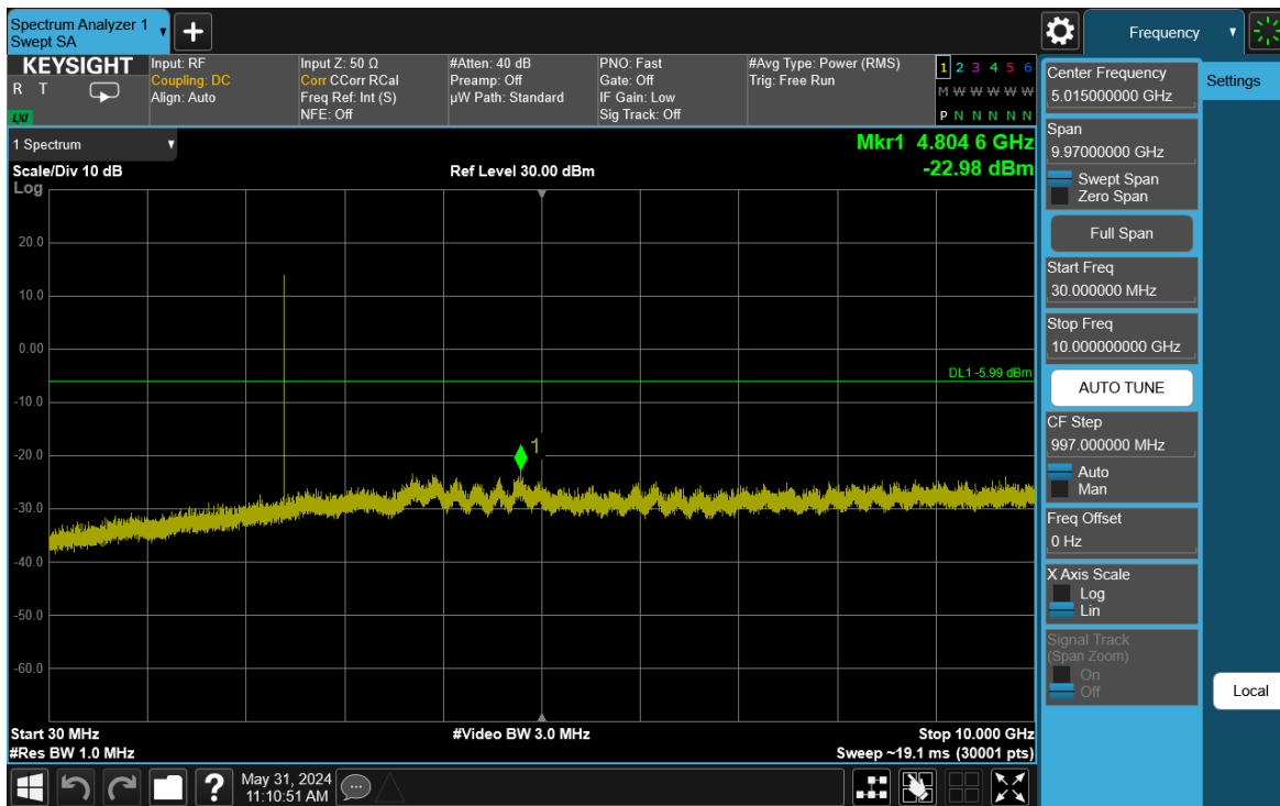
Plot 7-85. Conducted Spurious Plot Antenna 3a (Bluetooth (HDR4), 4 Mbps, ePA – Ch. 1)
