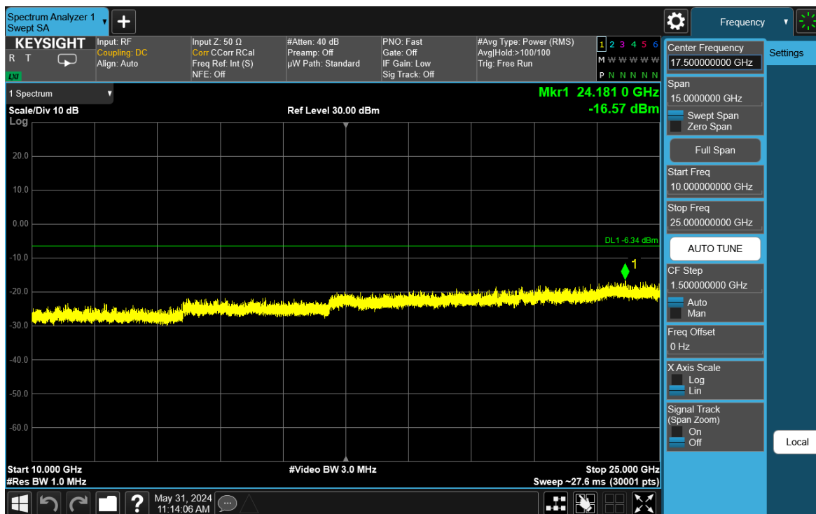
Plot 7-90. Conducted Spurious Plot Antenna 3a (Bluetooth (HDR4), 4 Mbps, ePA – Ch. 73)
