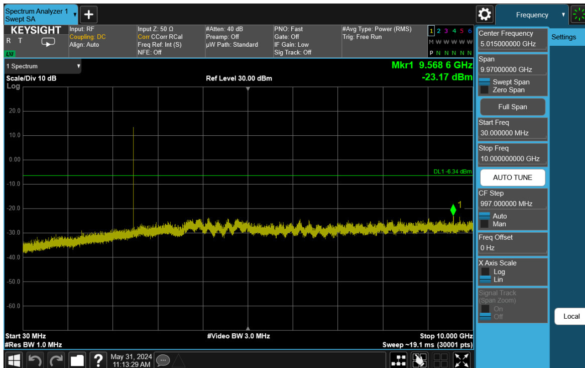
Plot 7-89. Conducted Spurious Plot Antenna 3a (Bluetooth (HDR4), 4 Mbps, ePA – Ch. 73)
