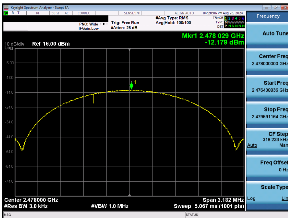
Plot 7-71. Power Spectral Density Plot Antenna 3a (Bluetooth (LE), 2Mbps, iPA – Ch. 38)
