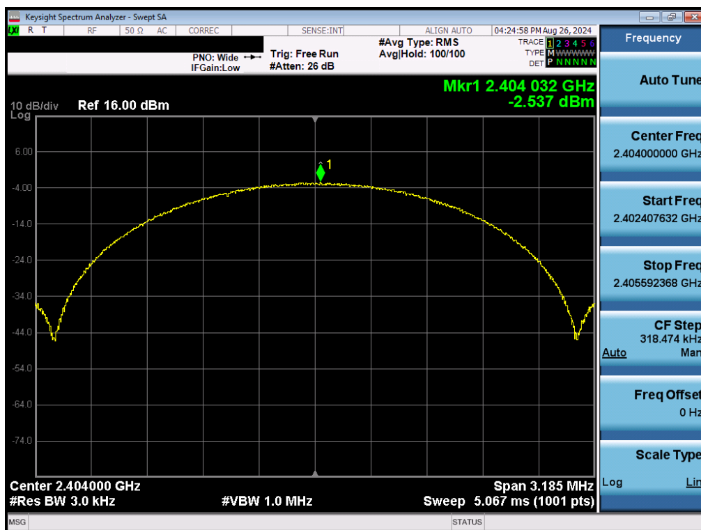
Plot 7-61. Power Spectral Density Plot Antenna 3a (Bluetooth (LE), 2Mbps, ePA – Ch. 1)
