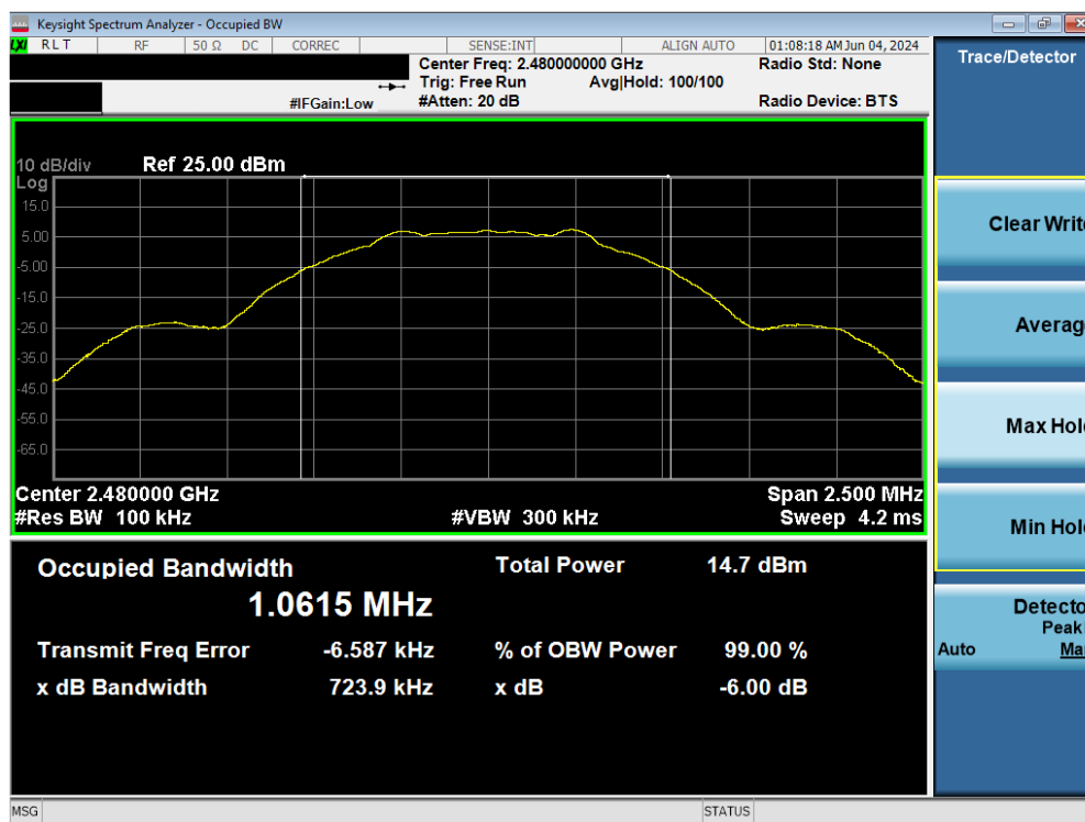
Plot 7-15. 6dB BW & 99% OBW Plot Antenna 4 (Bluetooth (LE), 1Mbps, iPA – Ch. 39)
