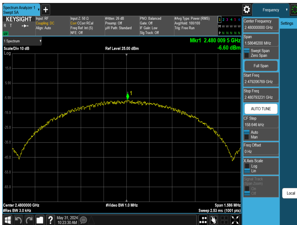
Plot 7-24. Power Spectral Density Plot Antenna 3a (Bluetooth (LE), 1Mbps, iPA – Ch. 39)
