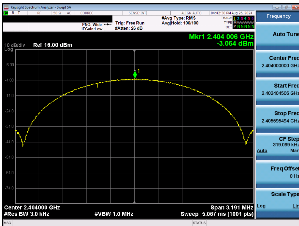
Plot 7-62. Power Spectral Density Plot Antenna 1a (Bluetooth (LE), 2Mbps, ePA – Ch. 1)
