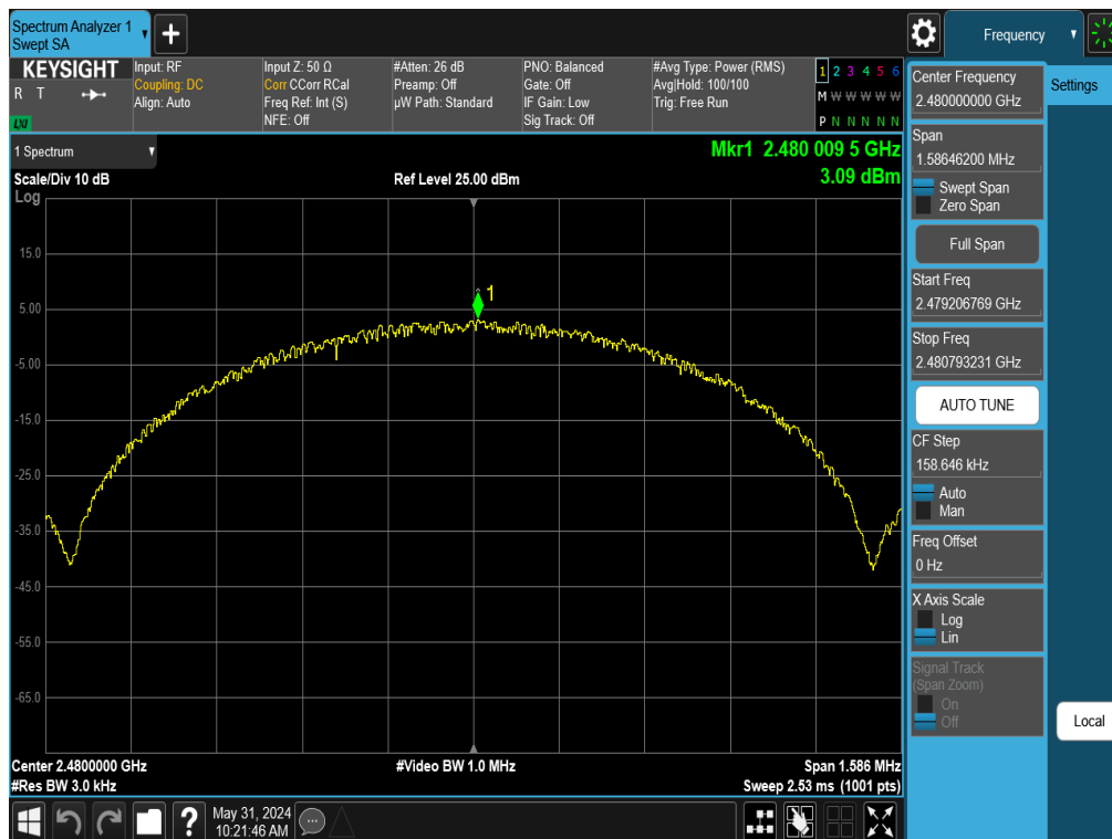
Plot 7-21. Power Spectral Density Plot Antenna 3a (Bluetooth (LE), 1Mbps, ePA – Ch. 39)
