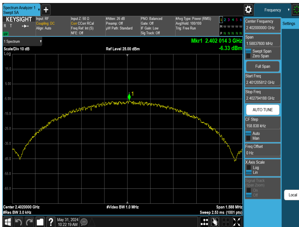
Plot 7-22. Power Spectral Density Plot Antenna 3a (Bluetooth (LE), 1Mbps, iPA – Ch. 0)
