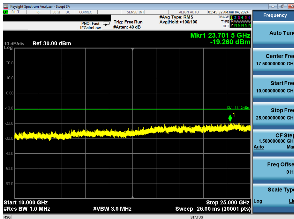
Plot 7-100. Conducted Spurious Plot Antenna 4 (Bluetooth (LE), 1Mbps, iPA – Ch. 19)
