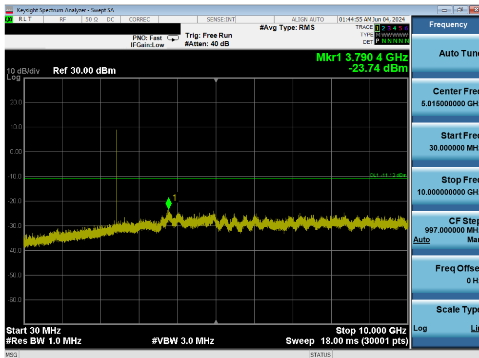
Plot 7-99. Conducted Spurious Plot Antenna 4 (Bluetooth (LE), 1Mbps, iPA – Ch. 19)
