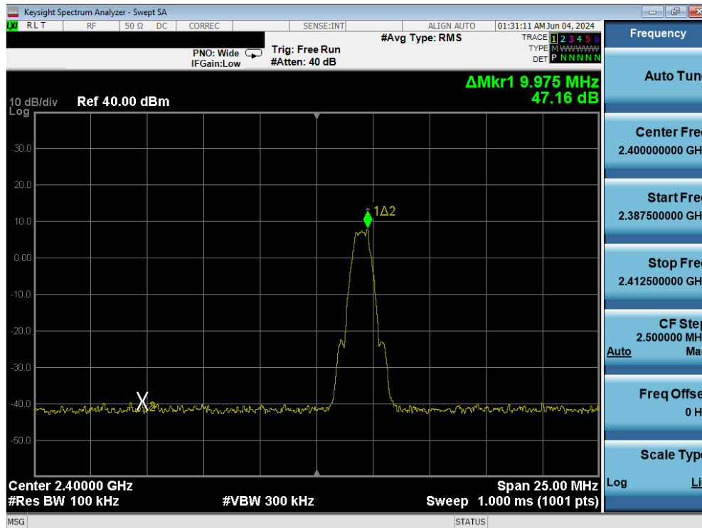
Plot 7-81. Band Edge Plot Antenna 4 (Bluetooth (LE), 1Mbps, iPA – Ch.0)
