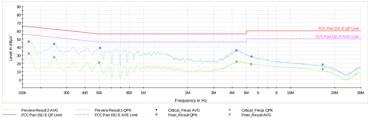
Plot 7-133. AC Line Conducted Plot with Bluetooth LE Tx BF (L1, 1Mbps ePA – Ch.39 with AC/DC Adapter and USB-C Cable)
