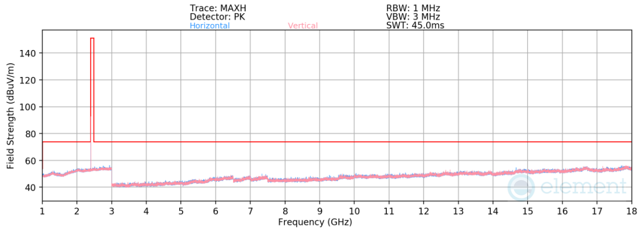
Plot 7-109. Radiated Spurious Emissions 1-18GHz Antenna 4 (1Mbps, iPA – Ch. 0)
