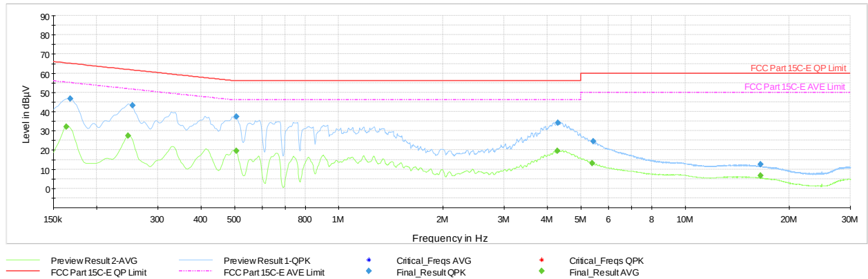
Plot 7-134. AC Line Conducted Plot with Bluetooth LE Tx BF (N, 1Mbps ePA – Ch.39, with AC/DC Adapter and USB-C Cable)
