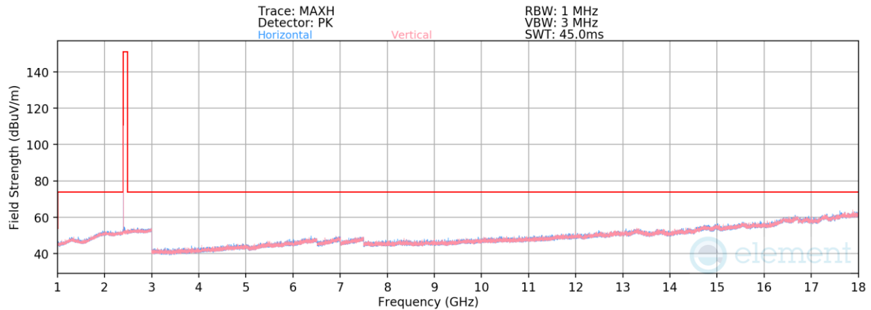
Plot 7-106. Radiated Spurious Emissions 1-18GHz Antenna 1a (1Mbps, ePA – Ch. 0)
