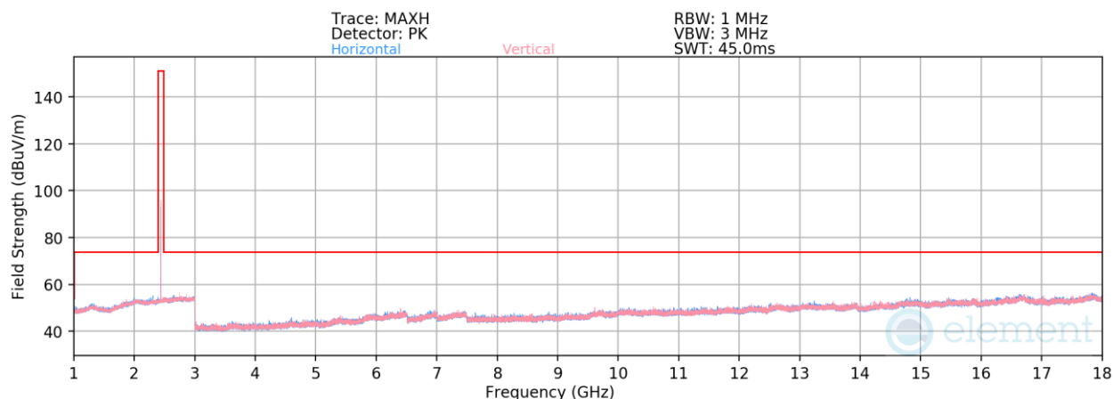
Plot 7-110. Radiated Spurious Emissions 1-18GHz Antenna 4 (1Mbps, iPA – Ch. 19)
