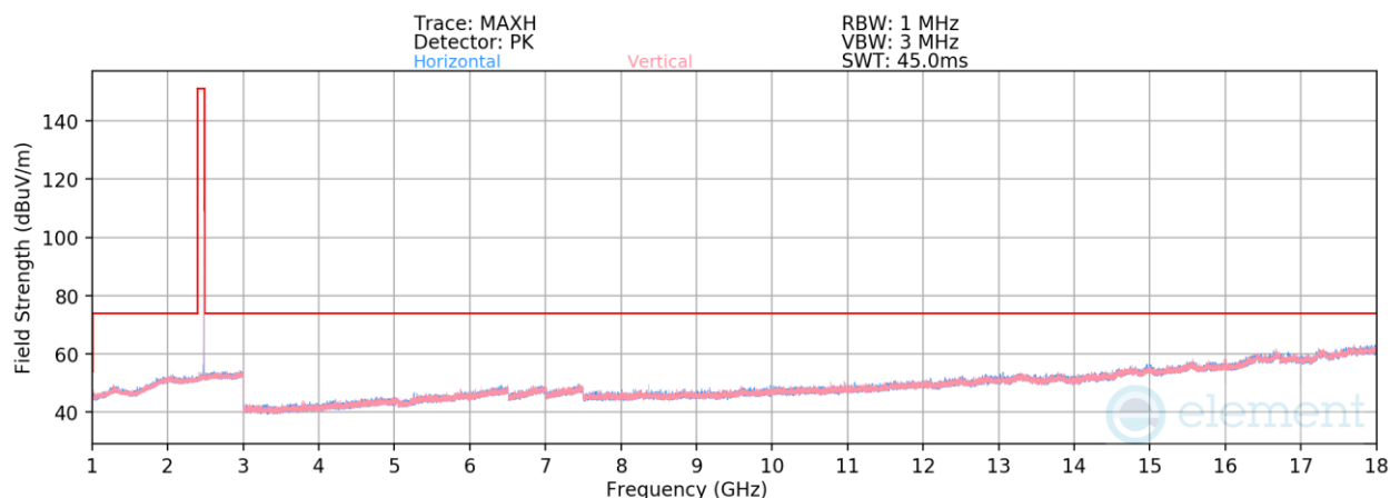
Plot 7-108. Radiated Spurious Emissions 1-18GHz Antenna 1a (1Mbps, ePA – Ch. 39)
