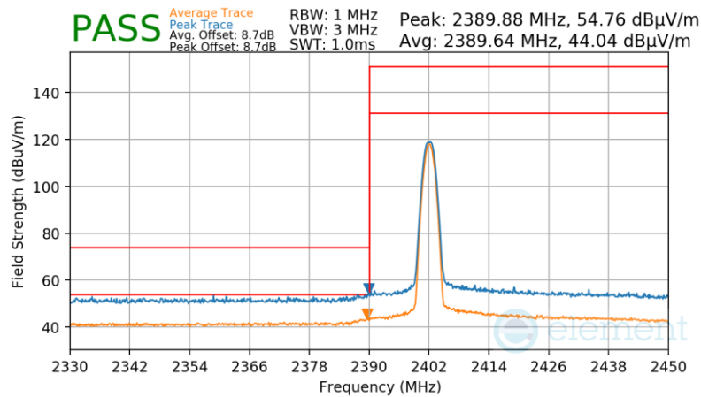
Plot 7-116. Radiated Restricted Lower Band Edge Measurement Antenna 3a (Average & Peak)
