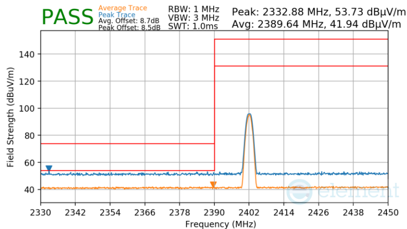
Plot 7-124. Radiated Restricted Lower Band Edge Measurement Antenna 4 (Average & Peak)
