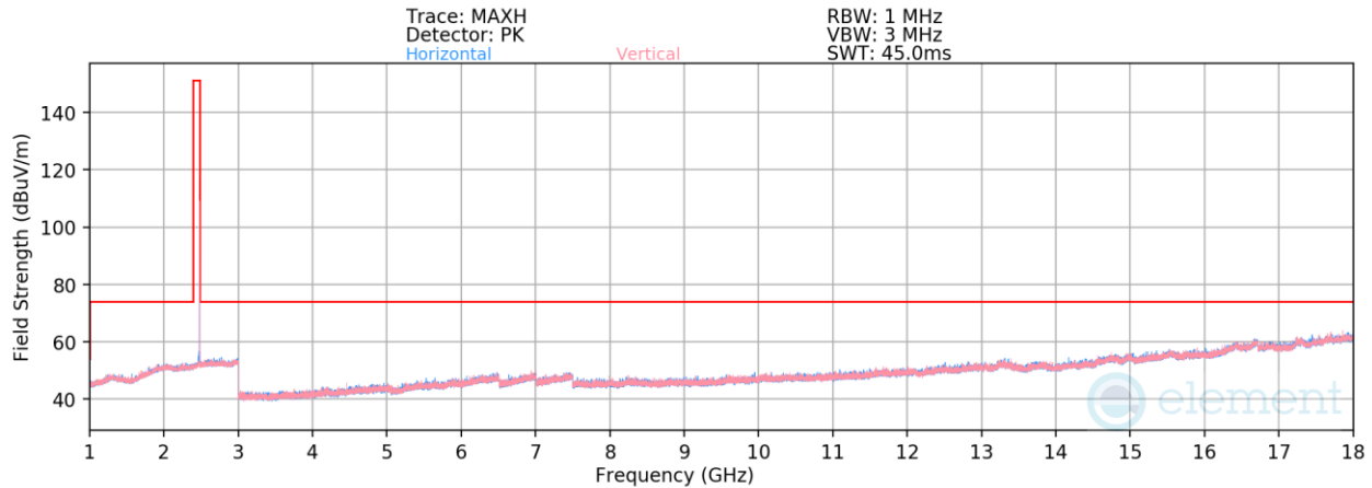
Plot 7-105. Radiated Spurious Emissions 1-18GHz Antenna 3a (1Mbps, ePA – Ch. 39)
