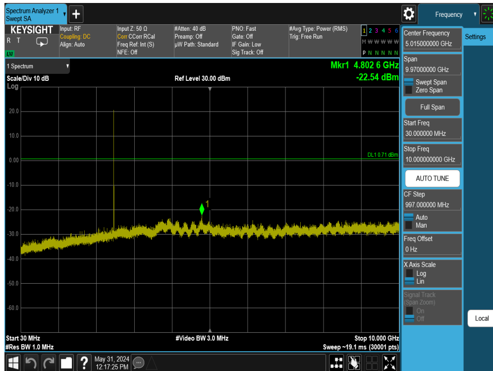
Plot 7-95. Conducted Spurious Plot Antenna 1a (Bluetooth (LE), 1Mbps, ePA – Ch. 39)
