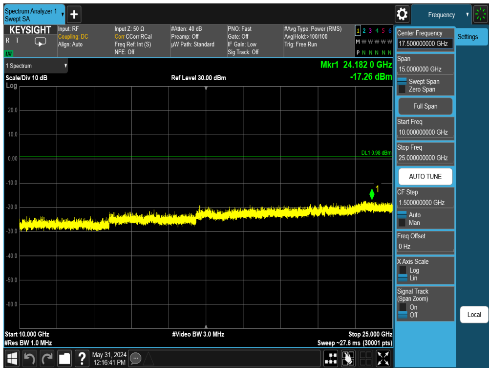
Plot 7-94. Conducted Spurious Plot Antenna 1a (Bluetooth (LE), 1Mbps, ePA – Ch. 19)
