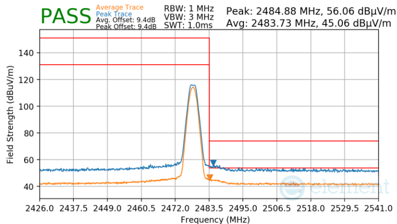
Plot 7-123. Radiated Restricted Upper Band Edge Measurement Antenna 1a (Average & Peak)
