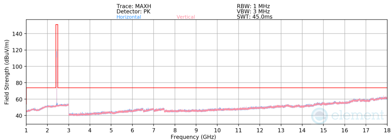
Plot 7-104. Radiated Spurious Emissions 1-18GHz Antenna 3a (1Mbps, ePA – Ch. 19)
