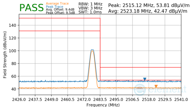
Plot 7-127. Radiated Restricted Upper Band Edge Measurement Antenna 4 (Average & Peak)
