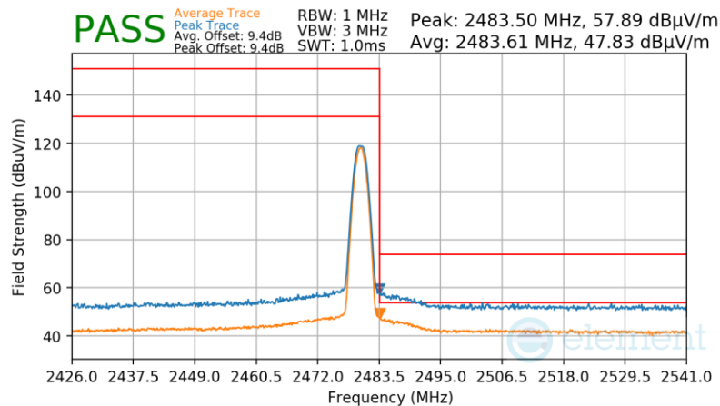
Plot 7-117. Radiated Restricted Upper Band Edge Measurement Antenna 3a (Average & Peak)
