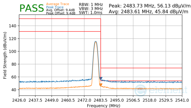
Plot 7-121. Radiated Restricted Upper Band Edge Measurement Antenna 1a (Average & Peak)
