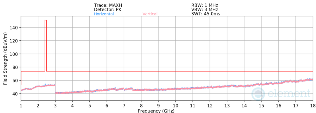
Plot 7-103. Radiated Spurious Emissions 1-18GHz Antenna 3a (1Mbps, ePA – Ch. 0)
