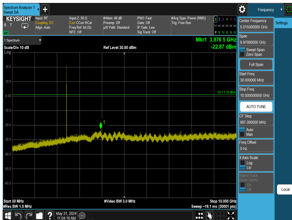
Plot 7-87. Conducted Spurious Plot Antenna 3a (Bluetooth (LE), 1Mbps, ePA – Ch. 19)
