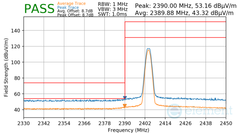
Plot 7-122. Radiated Restricted Lower Band Edge Measurement Antenna 1a (Average & Peak)
