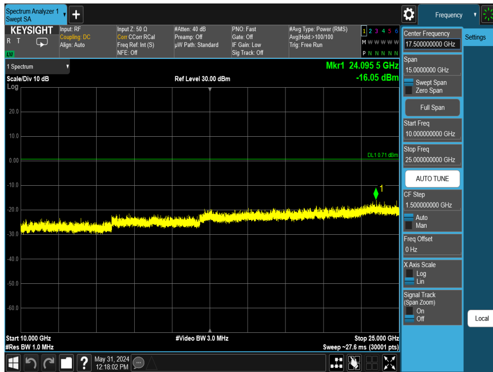
Plot 7-96. Conducted Spurious Plot Antenna 1a (Bluetooth (LE), 1Mbps, ePA – Ch. 39)
