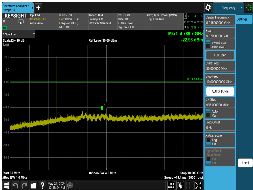
Plot 7-93. Conducted Spurious Plot Antenna 1a (Bluetooth (LE), 1Mbps, ePA – Ch. 19)
