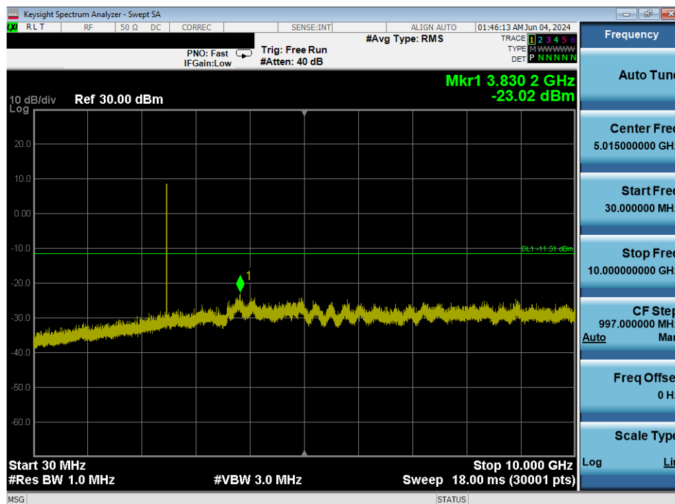
Plot 7-101. Conducted Spurious Plot Antenna 4 (Bluetooth (LE), 1Mbps, iPA – Ch. 39)
