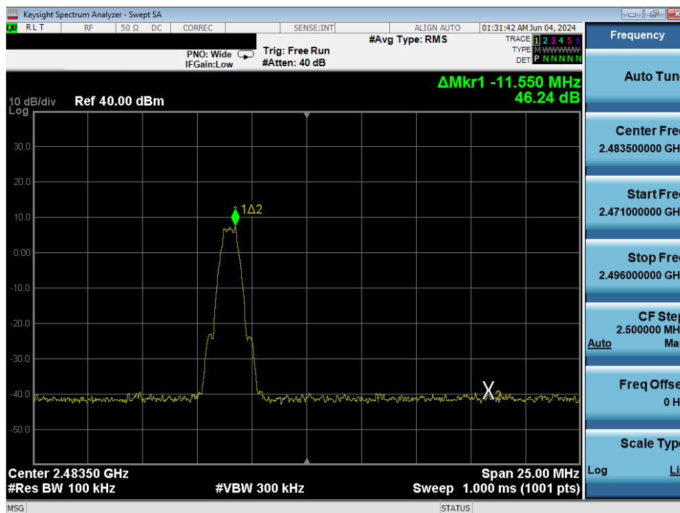
Plot 7-82. Band Edge Plot Antenna 4 (Bluetooth (LE), 1Mbps, iPA – Ch. 39)
