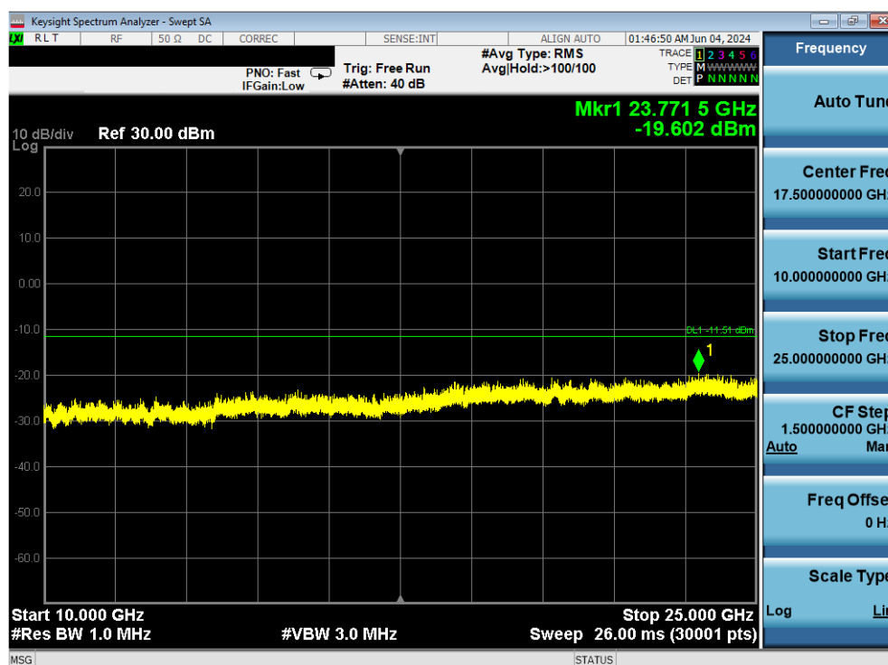
Plot 7-102. Conducted Spurious Plot Antenna 4 (Bluetooth (LE), 1Mbps, iPA – Ch. 39)
