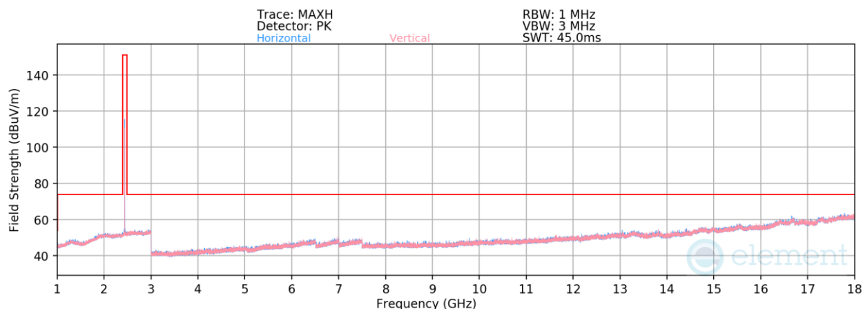
Plot 7-107. Radiated Spurious Emissions 1-18GHz Antenna 1a (1Mbps, ePA – Ch. 19)
