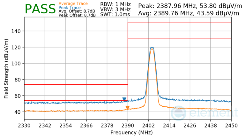
Plot 7-118. Radiated Restricted Lower Band Edge Measurement Antenna 3a (Average & Peak)
