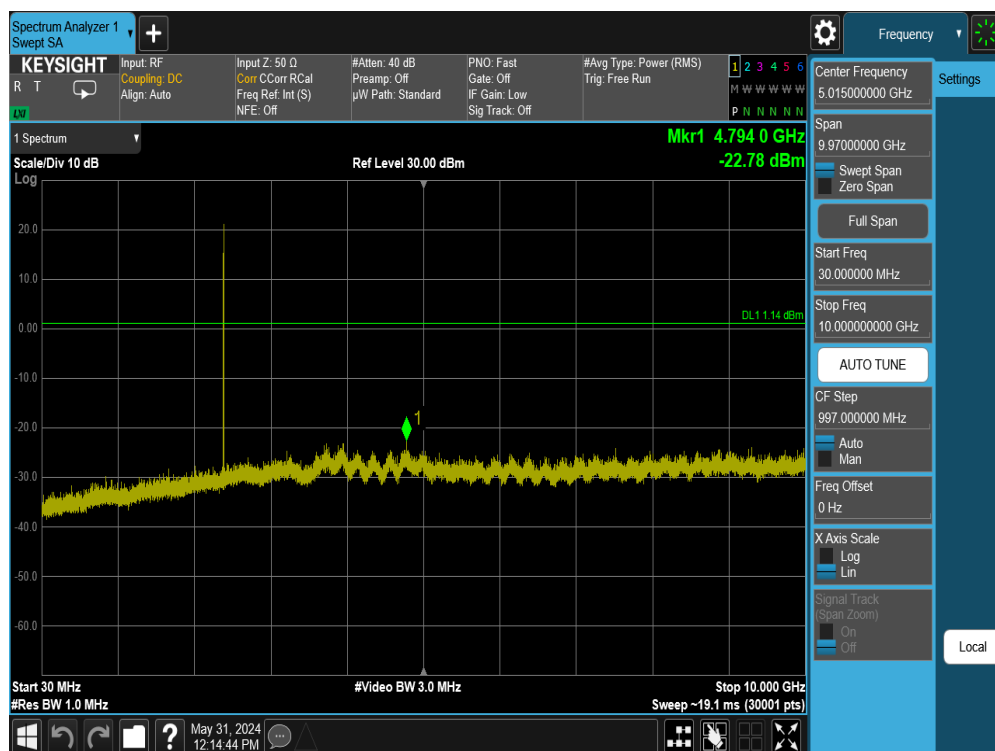
Plot 7-91. Conducted Spurious Plot Antenna 1a (Bluetooth (LE), 1Mbps, ePA – Ch. 0)
