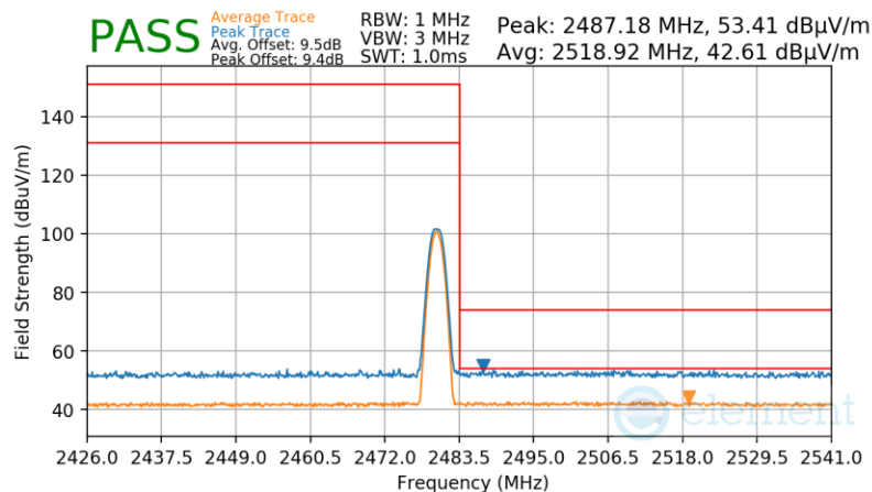
Plot 7-125. Radiated Restricted Upper Band Edge Measurement Antenna 4 (Average & Peak)
