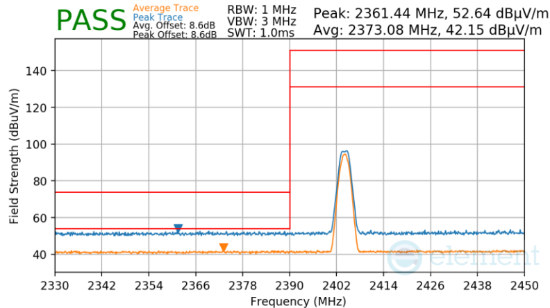
Plot 7-126. Radiated Restricted Lower Band Edge Measurement Antenna 4 (Average & Peak)
