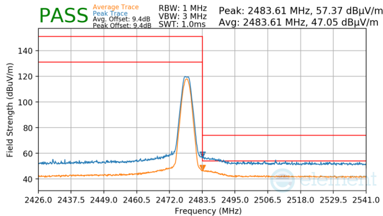
Plot 7-119. Radiated Restricted Upper Band Edge Measurement Antenna 3a (Average & Peak)
