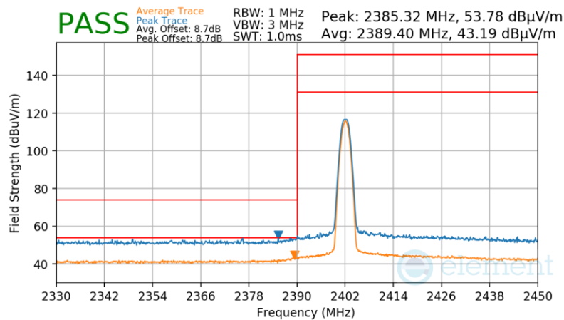
Plot 7-120. Radiated Restricted Lower Band Edge Measurement Antenna 1a (Average & Peak)
