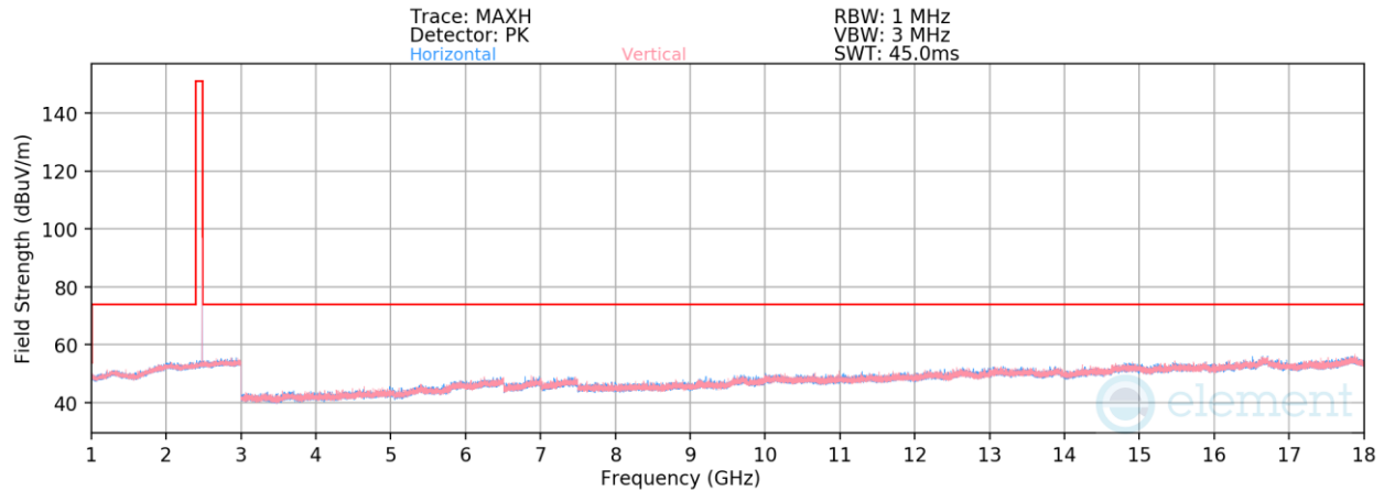
Plot 7-111. Radiated Spurious Emissions 1-18GHz Antenna 4 (1Mbps, iPA – Ch. 39)
