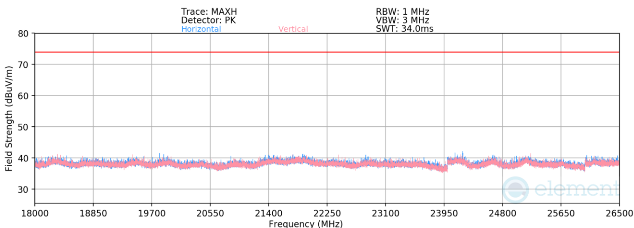
Plot 7-115. Radiated Spurious Emissions Above 18GHz TxBF (1Mbps, ePA – Ch. 39)
