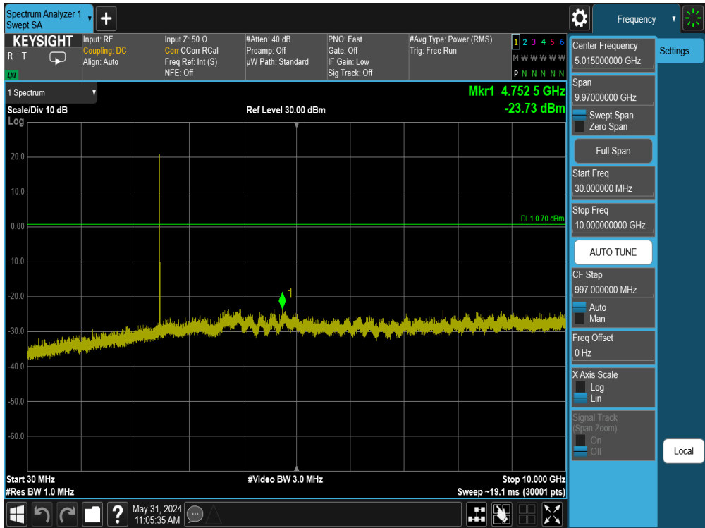
Plot 7-89. Conducted Spurious Plot Antenna 3a (Bluetooth (LE), 1Mbps, ePA – Ch. 39)
