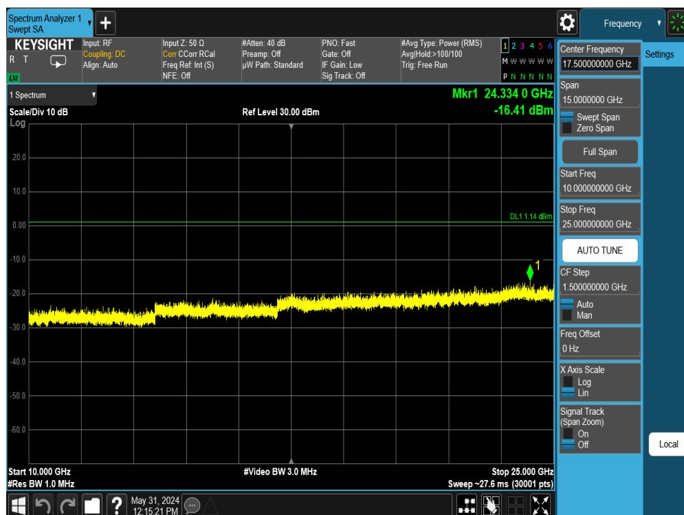
Plot 7-92. Conducted Spurious Plot Antenna 1a (Bluetooth (LE), 1Mbps, ePA – Ch. 0)
