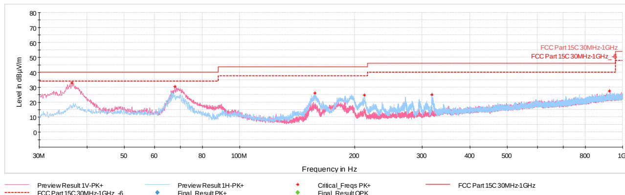
Plot 7-132. Radiated Spurious Emissions Below 1GHz TxBF (1Mbps, ePA – Ch.39, Pol. H & V, with AC/DC Adapter and USB-C Cable)
