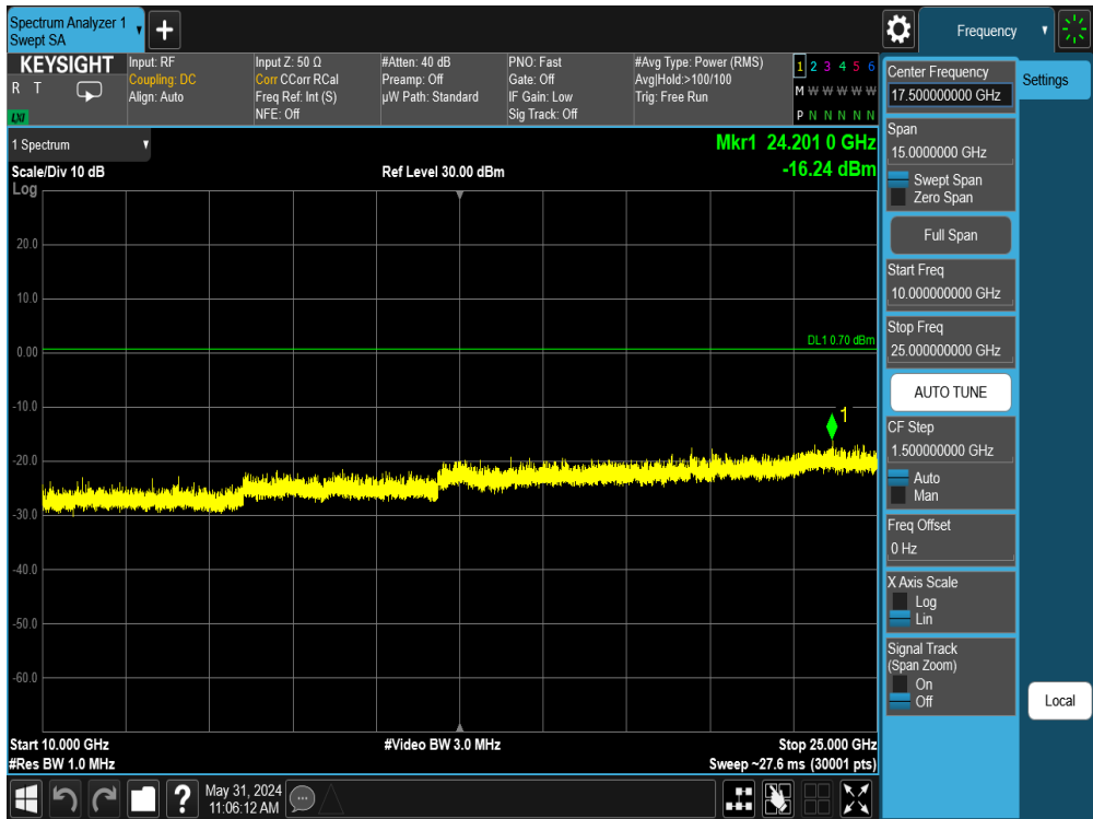
Plot 7-90. Conducted Spurious Plot Antenna 3a (Bluetooth (LE), 1Mbps, ePA – Ch. 39)
