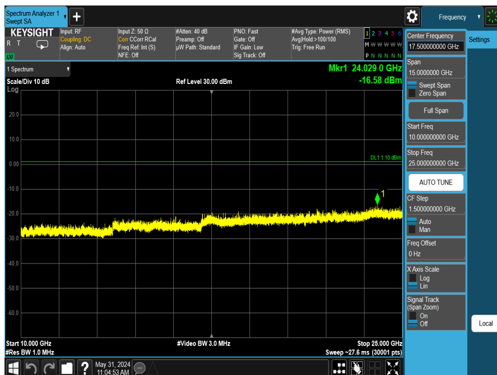
Plot 7-88. Conducted Spurious Plot Antenna 3a (Bluetooth (LE), 1Mbps, ePA – Ch. 19)
