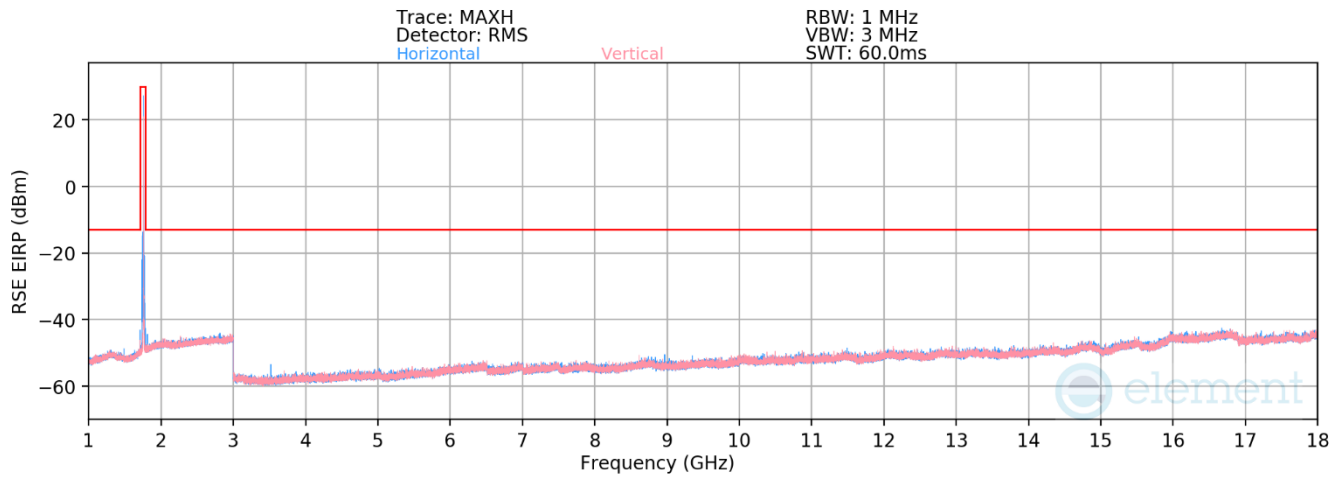
Plot 7-489. Antenna 2 Radiated Spurious Emission above 1GHz (FR1 Band n66)
