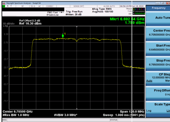
Plot 7-286. Power Spectral Density Plot CDD Antenna 3b SP (80MHz 802.11ax (UNII Band 7) – Ch. 151, MCS11)
