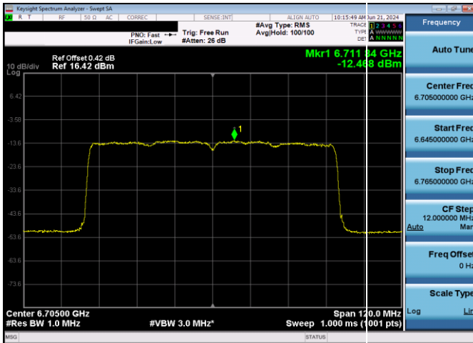
Plot 7-302. Power Spectral Density Plot CDD Antenna 3b VLP (80MHz 802.11ax (UNII Band 7) – Ch. 151, MCS11)
