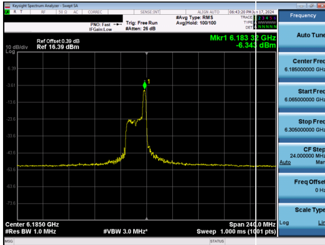
Plot 7-712. LPI Power Spectral Density Plot Antenna 1b (160MHz 802.11ax RU26 (UNII Band 5) - Ch. 47)
