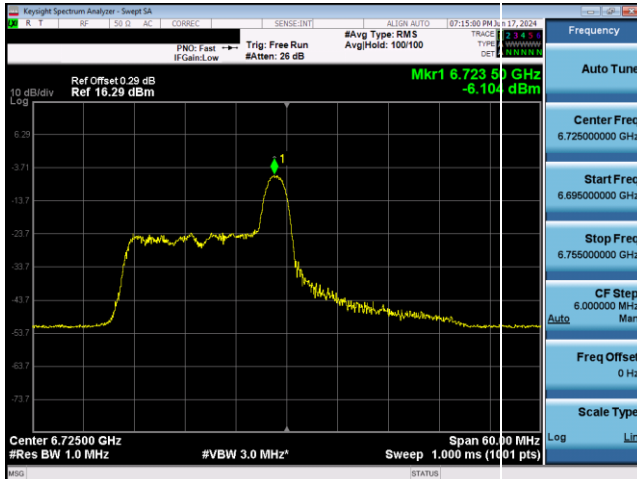
Plot 7-736. LPI Power Spectral Density Plot Antenna 1b (40MHz 802.11ax RU26 (UNII Band 7) – Ch. 155)
