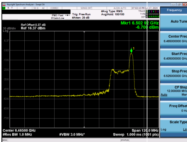
Plot 7-725. LPI Power Spectral Density Plot Antenna 1b (80MHz 802.11ax RU26 (UNII Band 6) - Ch. 103)
