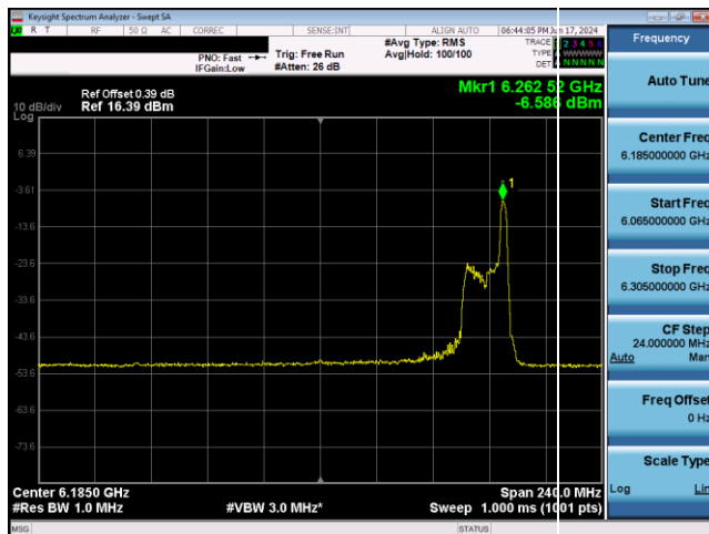
Plot 7-713. LPI Power Spectral Density Plot Antenna 1b (160MHz 802.11ax RU26 (UNII Band 5) - Ch. 47)
