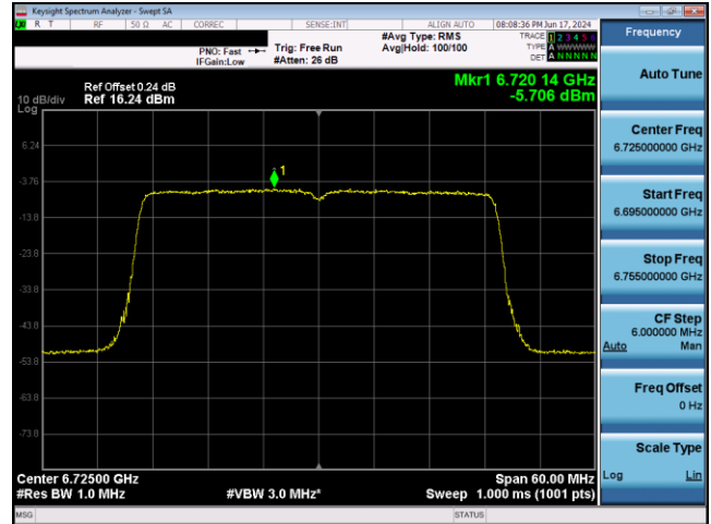
Plot 7-738. LPI Power Spectral Density Plot Antenna 1b (40MHz 802.11ax RU484 (UNII Band 7) – Ch. 155)
