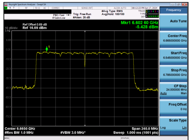
Plot 7-746. LPI Power Spectral Density Plot Antenna 1b (160MHz 802.11ax RU996x2 (UNII Band 7) - Ch. 143)
