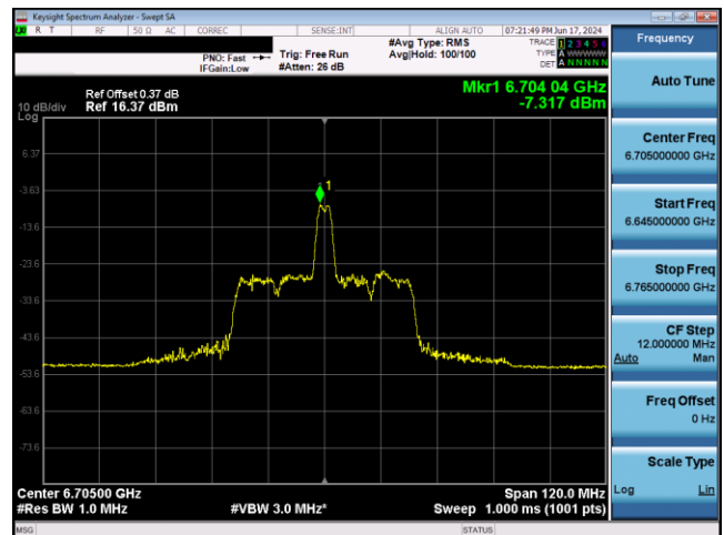
Plot 7-740. LPI Power Spectral Density Plot Antenna 1b (80MHz 802.11ax RU26 (UNII Band 7) – Ch. 151)
