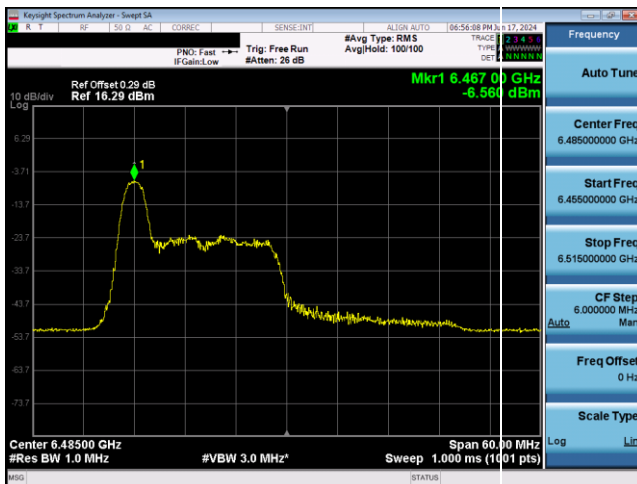
Plot 7-719. LPI Power Spectral Density Plot Antenna 1b (40MHz 802.11ax RU26 (UNII Band 6) - Ch. 107)
