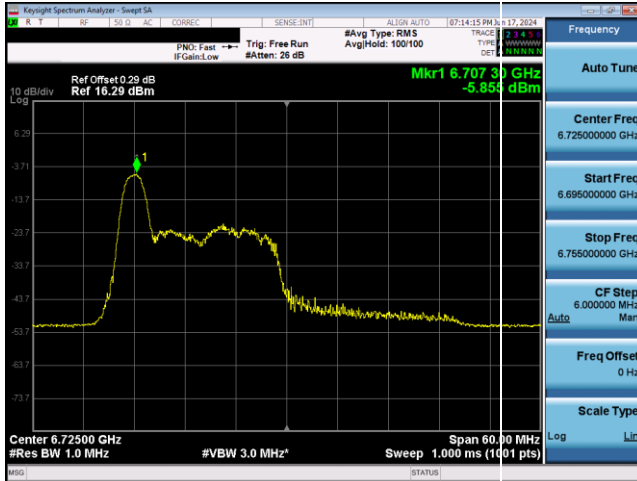
Plot 7-735. LPI Power Spectral Density Plot Antenna 1b (40MHz 802.11ax RU26 (UNII Band 7) – Ch. 155)
