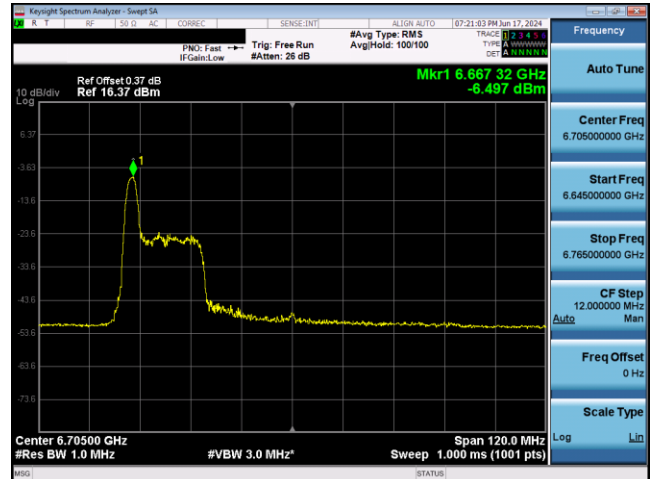
Plot 7-739. LPI Power Spectral Density Plot Antenna 1b (80MHz 802.11ax RU26 (UNII Band 7) – Ch. 151)
