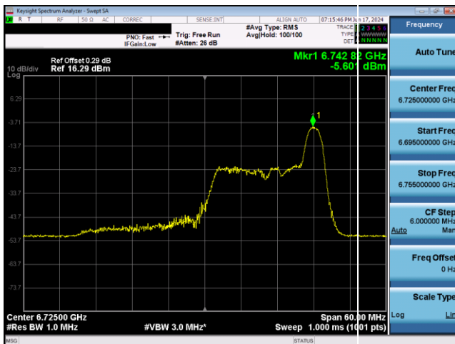
Plot 7-737. LPI Power Spectral Density Plot Antenna 1b (40MHz 802.11ax RU26 (UNII Band 7) – Ch. 155)
