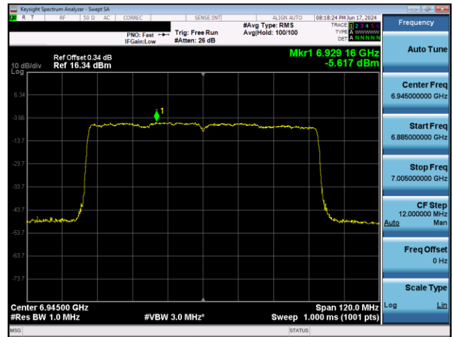
Plot 7-758. LPI Power Spectral Density Plot Antenna 1b (80MHz 802.11ax RU996 (UNII Band 8) – Ch. 199)
