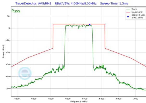
Plot 7-1148. SP In-Band Emission Plot Antenna 5T (160MHz 802.11ax RU996x2 (UNII Band 7) – Ch. 143)
