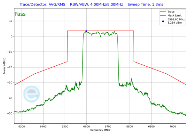
Plot 7-1180. SP In-Band Emission Plot Antenna 3b (160MHz 802.11ax RU996x2 (UNII Band 7) – Ch. 143)
