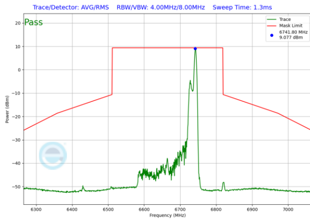
Plot 7-1179. SP In-Band Emission Plot Antenna 3b (160MHz 802.11ax RU26 (UNII Band 7) – Ch. 143)
