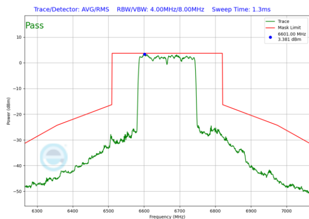
Plot 7-1212. SP In-Band Emission Plot Antenna 1b (160MHz 802.11ax RU996x2 (UNII Band 7) – Ch. 143)
