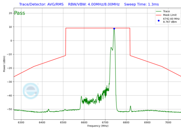
Plot 7-1147. SP In-Band Emission Plot Antenna 5T (160MHz 802.11ax RU26 (UNII Band 7) – Ch. 143)
