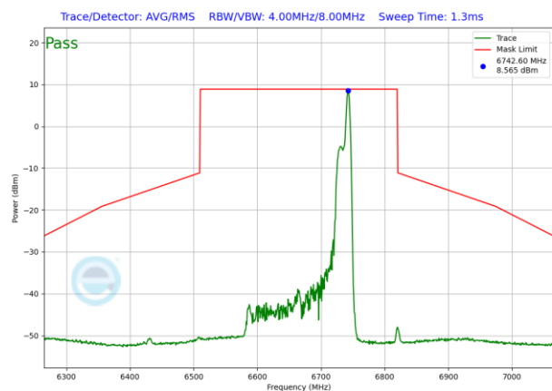
Plot 7-1211. SP In-Band Emission Plot Antenna 1b (160MHz 802.11ax RU26 (UNII Band 7) – Ch. 143)
