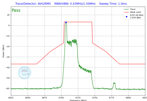
Plot 7-1169. SP In-Band Emission Plot Antenna 3b (40MHz 802.11ax RU26 (UNII Band 7) – Ch. 155)
