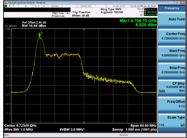
Plot 7-515. SP Power Spectral Density Plot CDD Antenna 5T (40MHz 802.11ax RU26 (UNII Band 7) - Ch. 155)
