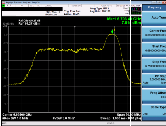
Plot 7-512. SP Power Spectral Density Plot CDD Antenna 3b (20MHz 802.11ax RU26 (UNII Band 7) - Ch. 149)
