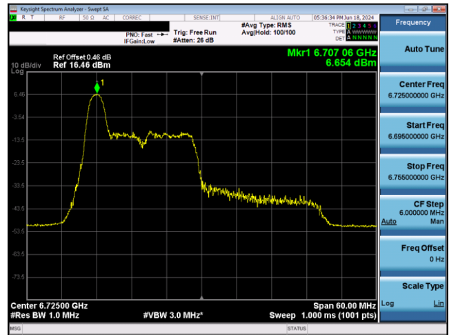
Plot 7-516. SP Power Spectral Density Plot CDD Antenna 3b (40MHz 802.11ax RU26 (UNII Band 7) - Ch. 155)
