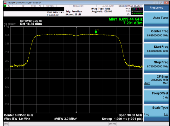
Plot 7-514. SP Power Spectral Density Plot CDD Antenna 3b (20MHz 802.11ax RU242 (UNII Band 7) - Ch. 149)
