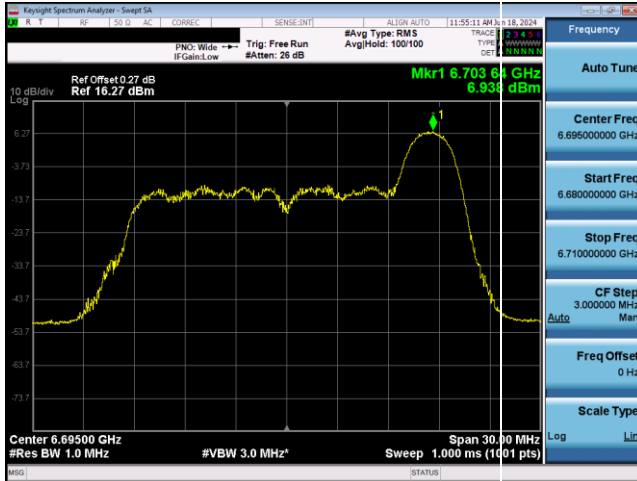
Plot 7-511. SP Power Spectral Density Plot CDD Antenna 5T (20MHz 802.11ax RU26 (UNII Band 7) - Ch. 149)
