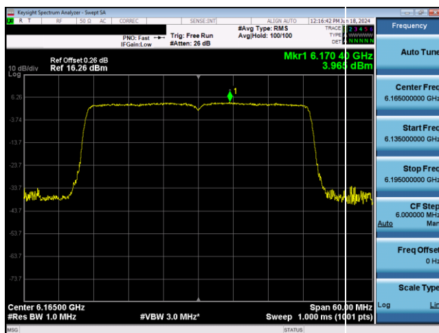
Plot 7-489. SP Power Spectral Density Plot CDD Antenna 5T (40MHz 802.11ax RU484 (UNII Band 5) – Ch. 43)
