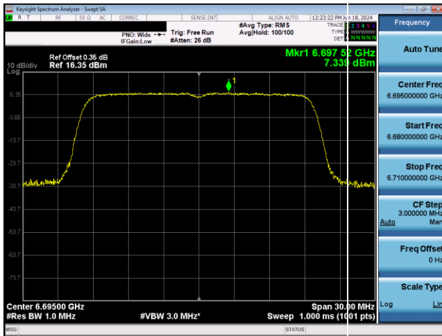
Plot 7-513. SP Power Spectral Density Plot CDD Antenna 5T (20MHz 802.11ax RU242 (UNII Band 7) - Ch. 149)
