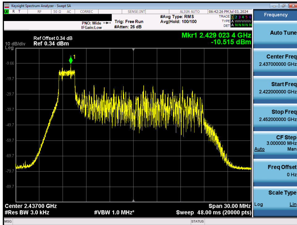
Plot 7-55. Power Spectral Density Plot Antenna 3a (802.11ax OFDMA – RU26 Index 0 – Ch. 6)
