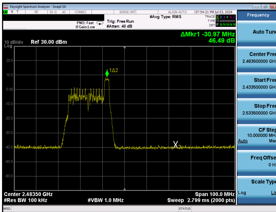
Plot 7-91. Band Edge Antenna 1a (802.11ax OFDMA – RU26 Index 8 – Ch. 12)
