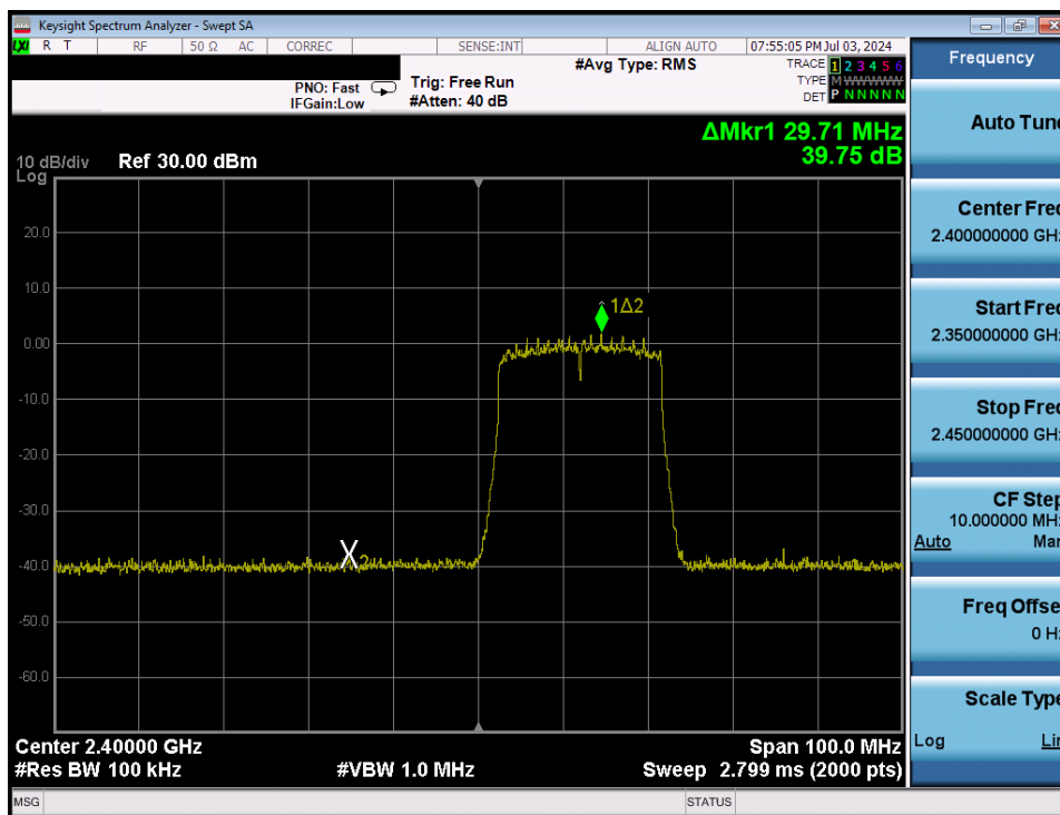
Plot 7-92. Band Edge Antenna 1a (802.11ax OFDMA – RU242 – Ch. 1)
