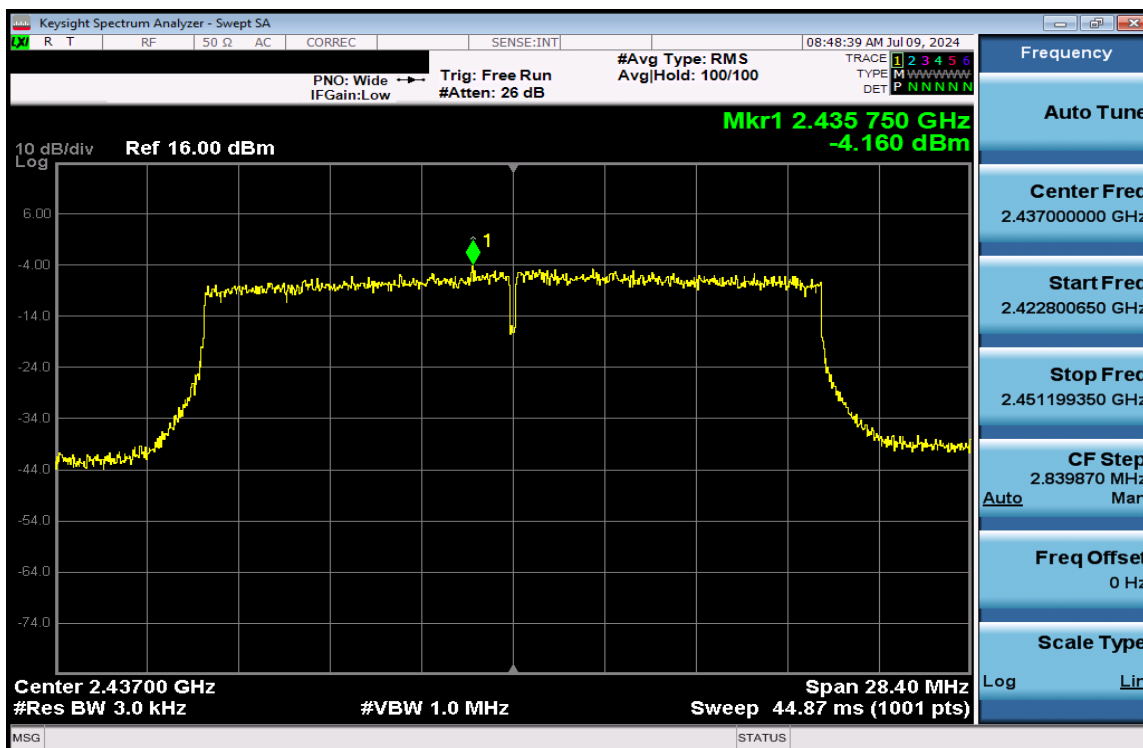
Plot 7-136. Power Spectral Density Plot CDD Antenna 1a (802.11ax (SU - 2.4GHz) – Ch. 6) – MCS2
