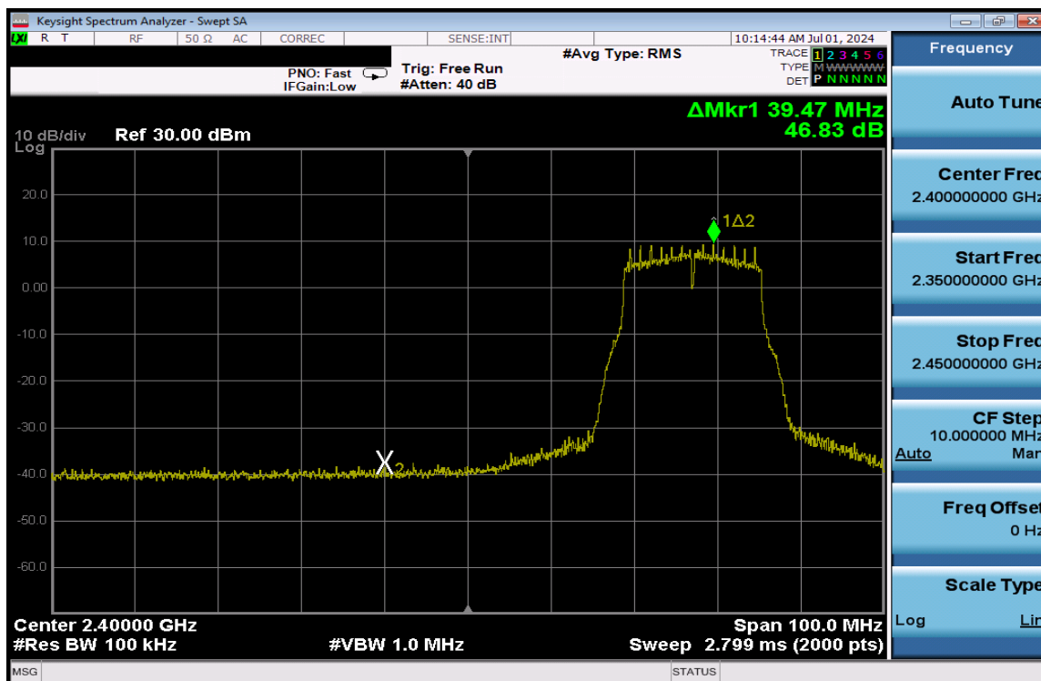
Plot 7-178. Band Edge Plot Antenna 3a (802.11g – Ch. 4) – 12Mbps
