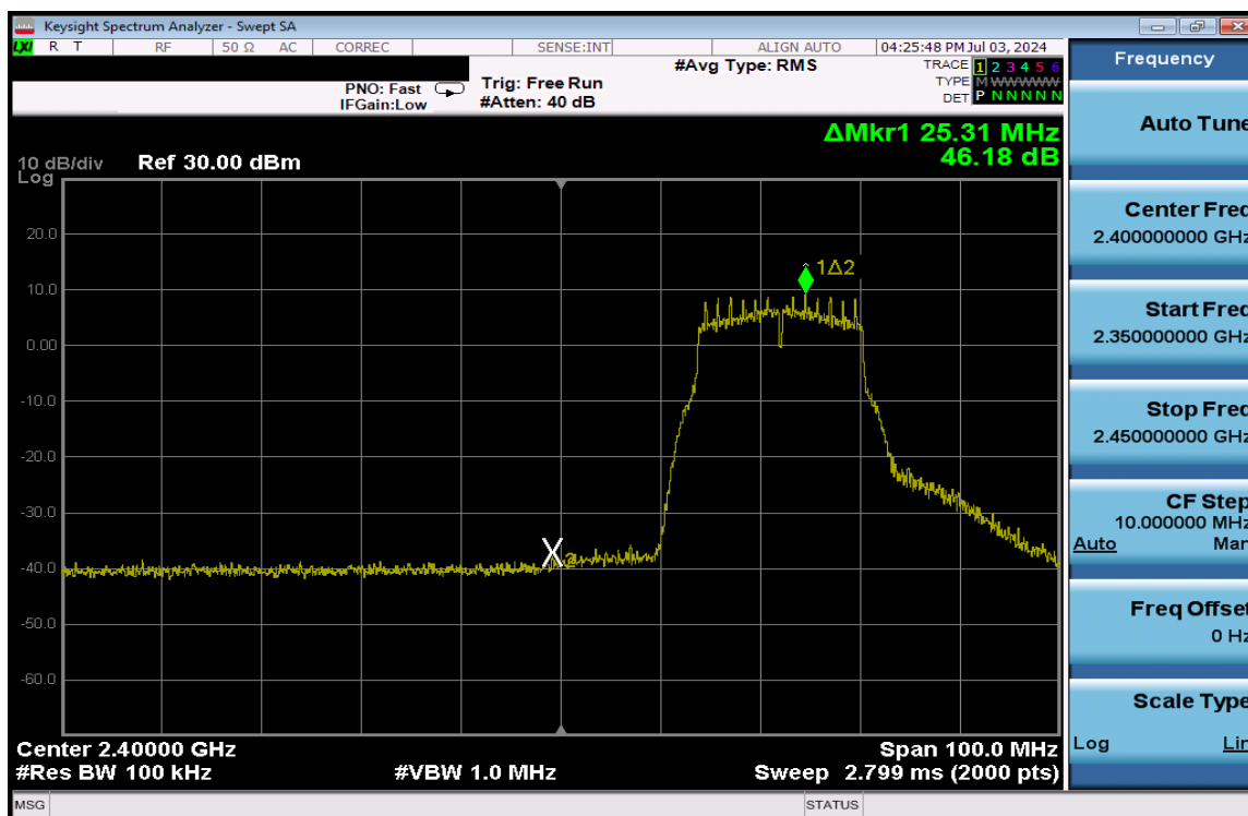
Plot 7-177. Band Edge Plot Antenna 3a (802.11g – Ch. 3) – 12Mbps
