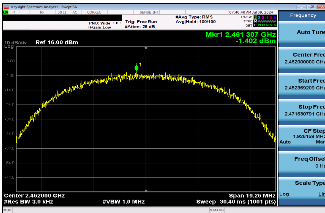
Plot 7-81. Power Spectral Density Plot Antenna 3a (802.11b – Ch. 11) – 11Mbps
