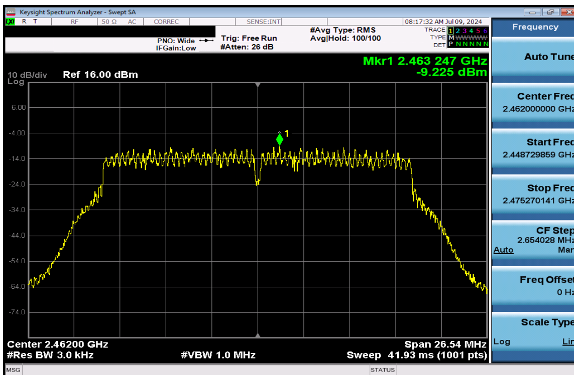
Plot 7-167. Power Spectral Density Plot CDD Antenna 3a (802.11n (2.4GHz) – Ch. 11) – MCS15
