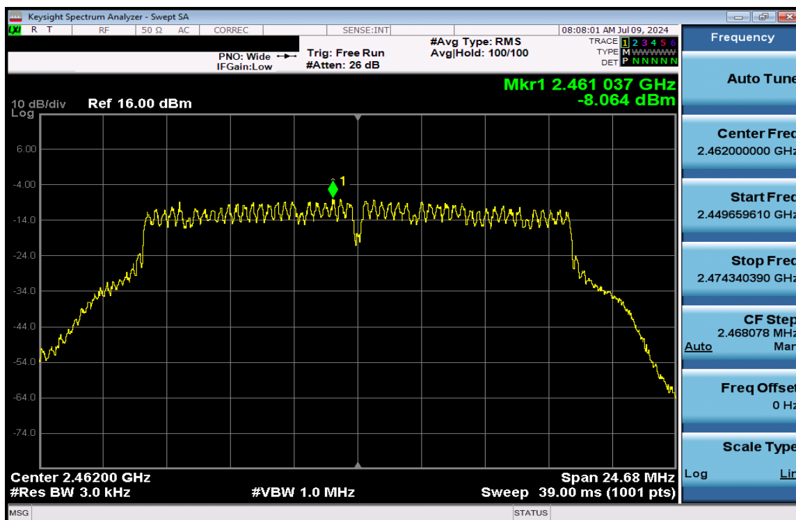
Plot 7-143. Power Spectral Density Plot CDD Antenna 3a (802.11g– Ch. 11) – 24Mbps
