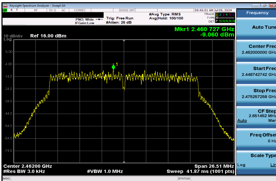
Plot 7-168. Power Spectral Density Plot CDD Antenna 1a (802.11n (2.4GHz) – Ch. 11) – MCS15
