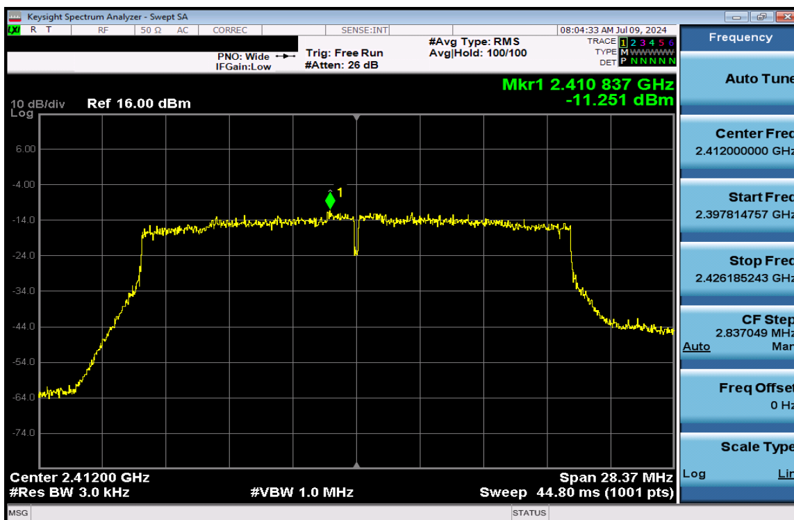
Plot 7-133. Power Spectral Density Plot CDD Antenna 3a (802.11ax (SU - 2.4GHz) – Ch. 1) – MCS2
