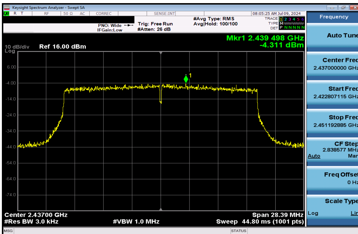
Plot 7-135. Power Spectral Density Plot CDD Antenna 3a (802.11ax (SU - 2.4GHz) – Ch. 6) – MCS2
