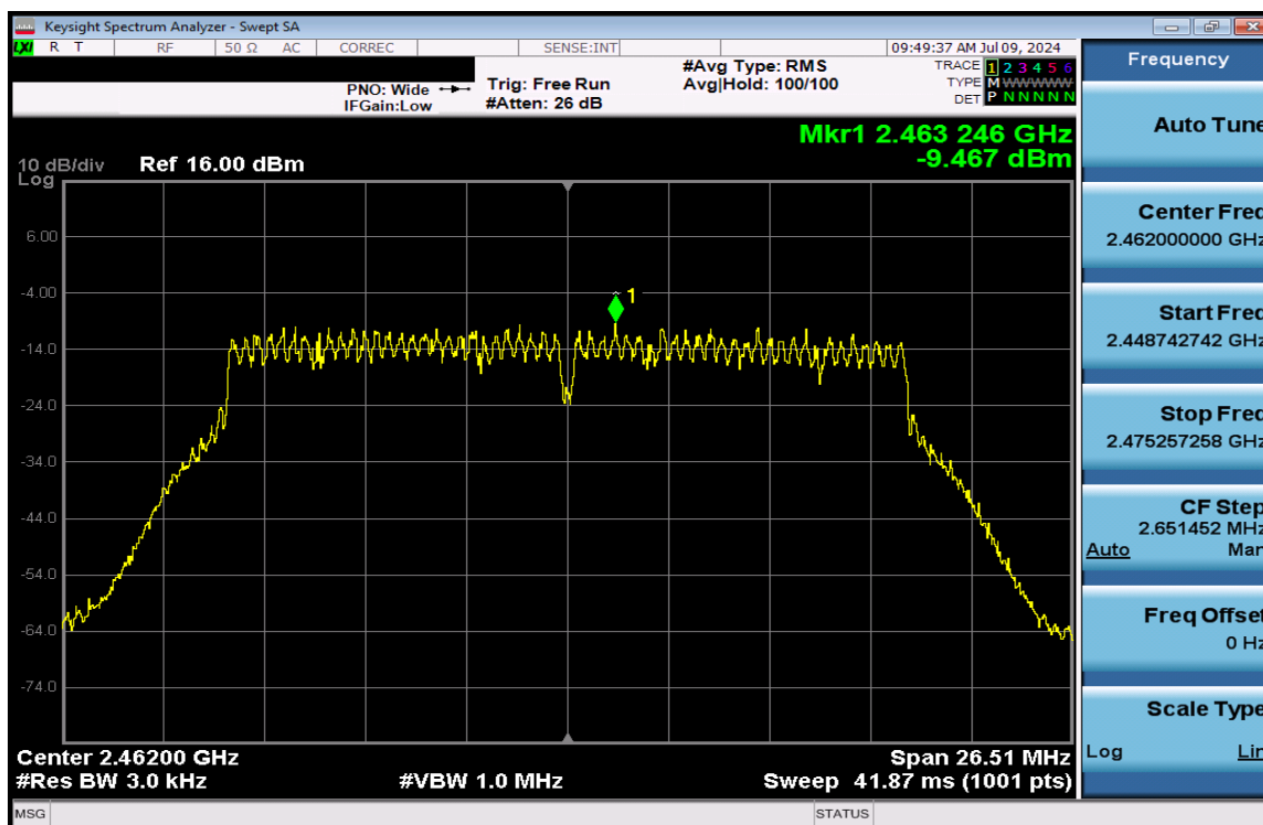
Plot 7-117. Power Spectral Density Plot Antenna 1a (802.11n (2.4GHz) – Ch. 11) – MCS7
