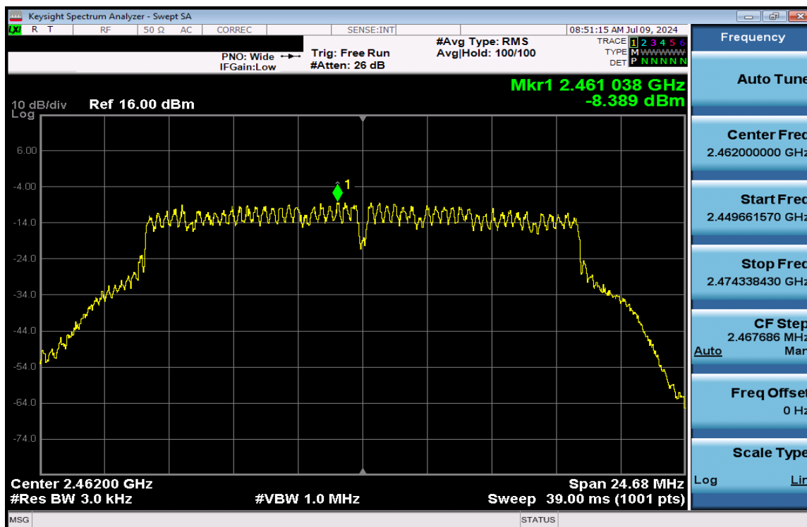
Plot 7-144. Power Spectral Density Plot CDD Antenna 1a (802.11g– Ch. 11) – 24Mbps
