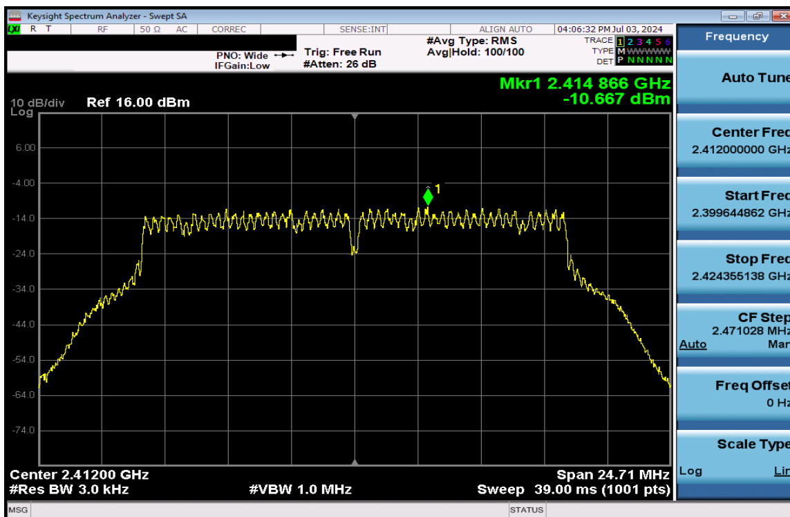
Plot 7-82. Power Spectral Density Plot Antenna 3a (802.11g – Ch. 1) – 54Mbps
