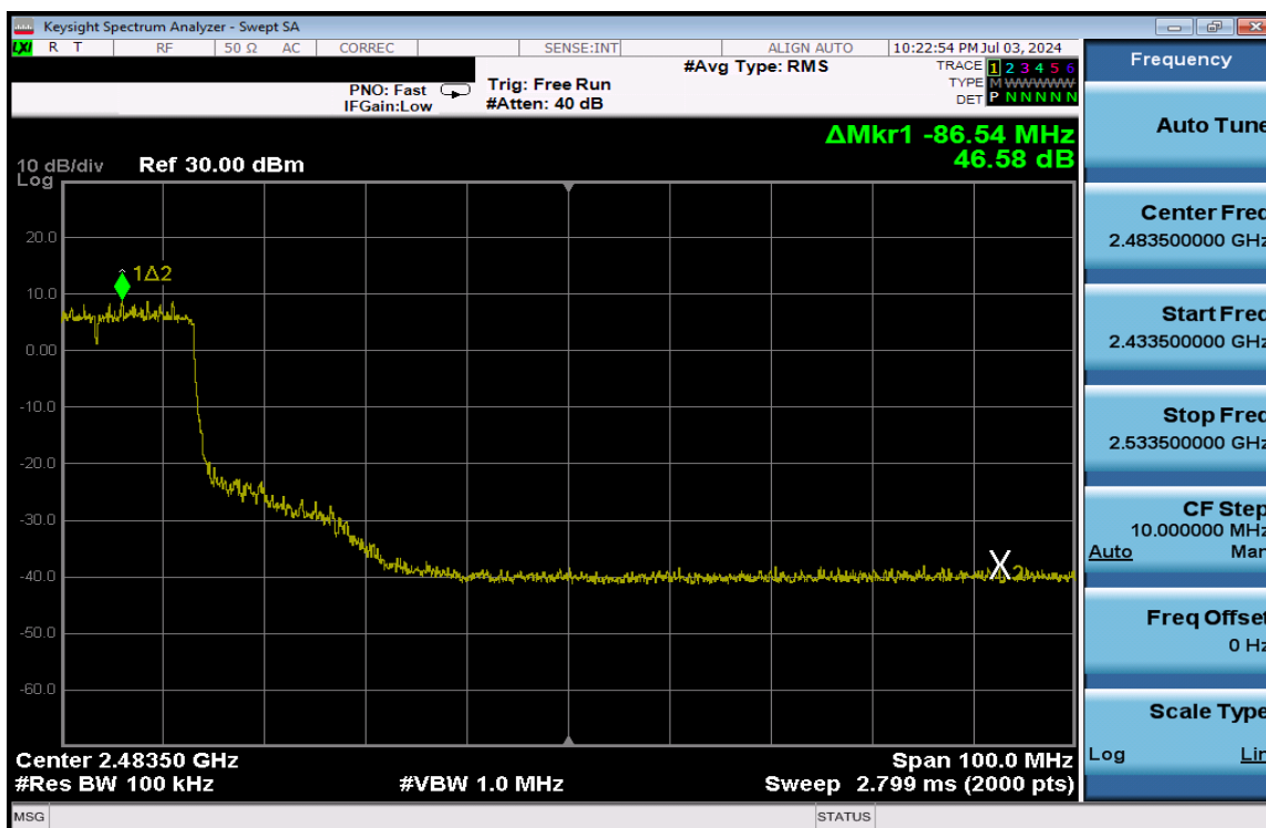
Plot 7-422. Band Edge Plot Antenna 1a (802.11ax (SU - 2.4GHz) - Ch. 6(high)) - MCS9
