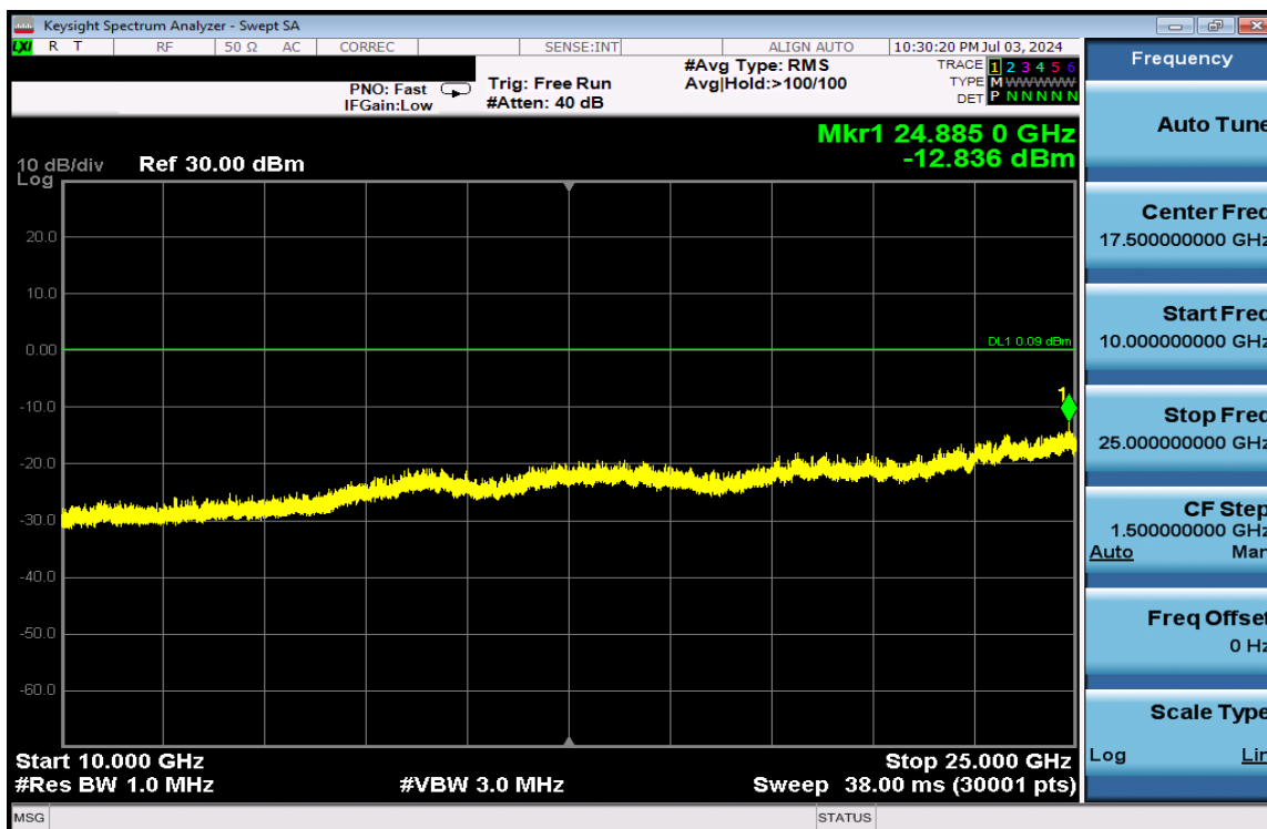
Plot 7-438. Conducted Spurious Plot Antenna 1a (802.11b – Ch. 6)
