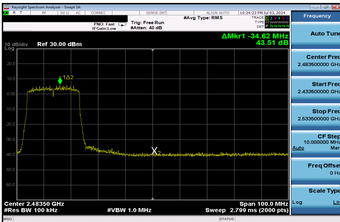
Plot 7-424. Band Edge Plot Antenna 1a (802.11ax (SU - 2.4GHz) - Ch. 8) - MCS9
