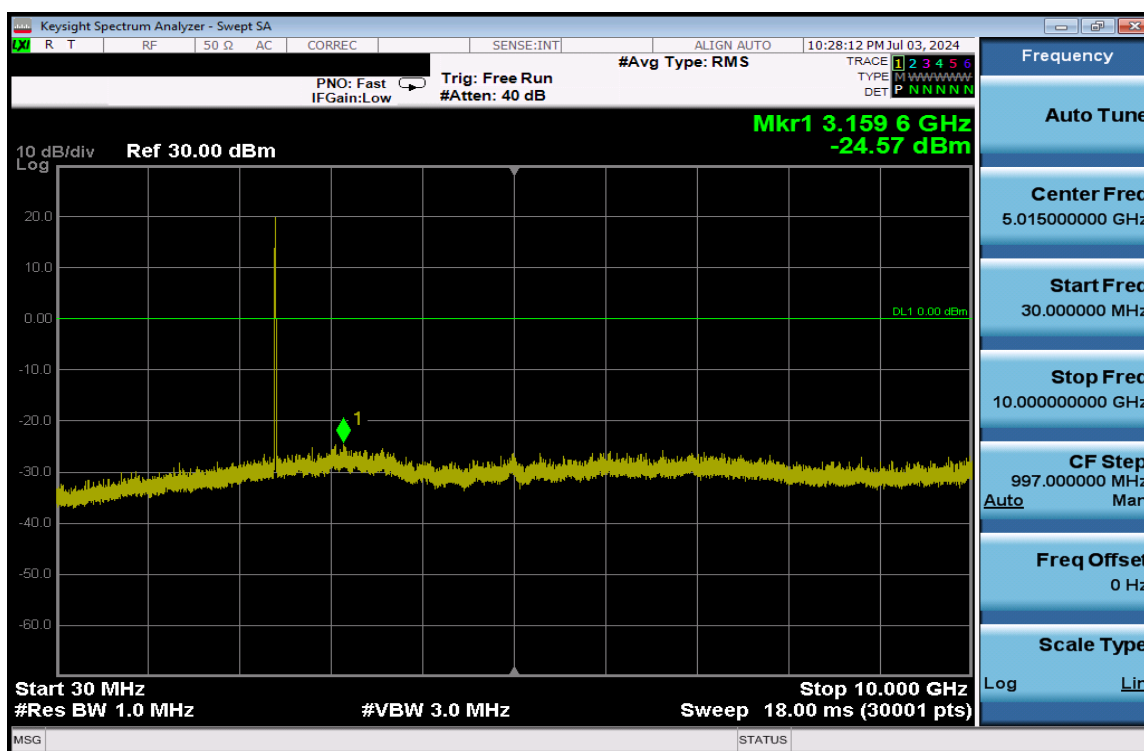
Plot 7-435. Conducted Spurious Plot Antenna 1a (802.11b – Ch. 1)
