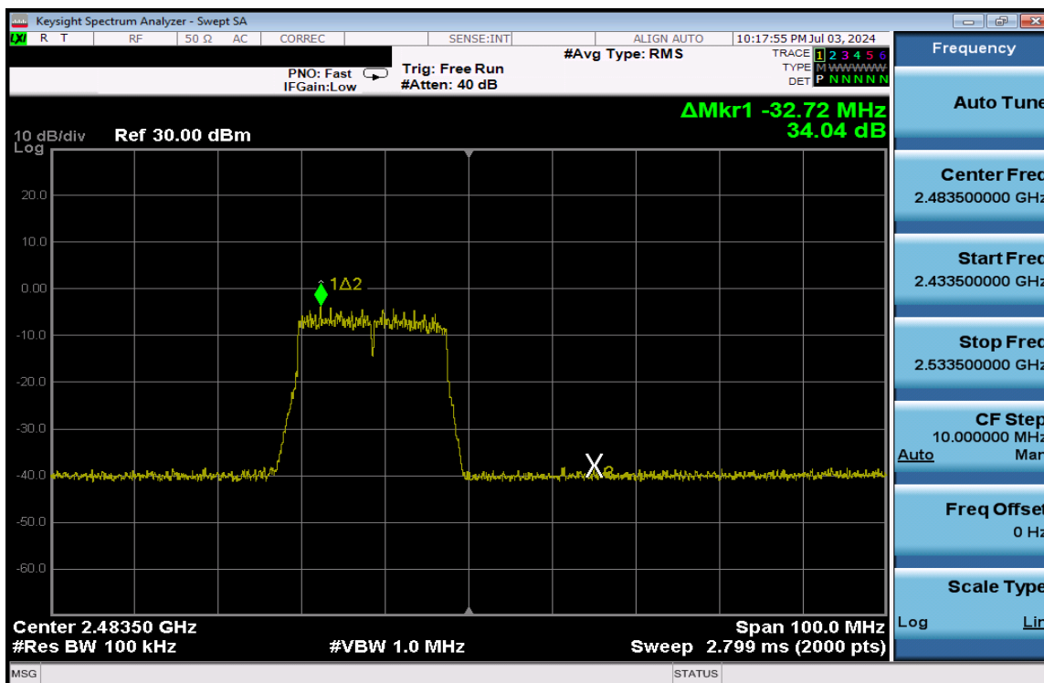
Plot 7-415. Band Edge Plot Antenna 1a (802.11n (2.4GHz) – Ch. 13) – MCS7
