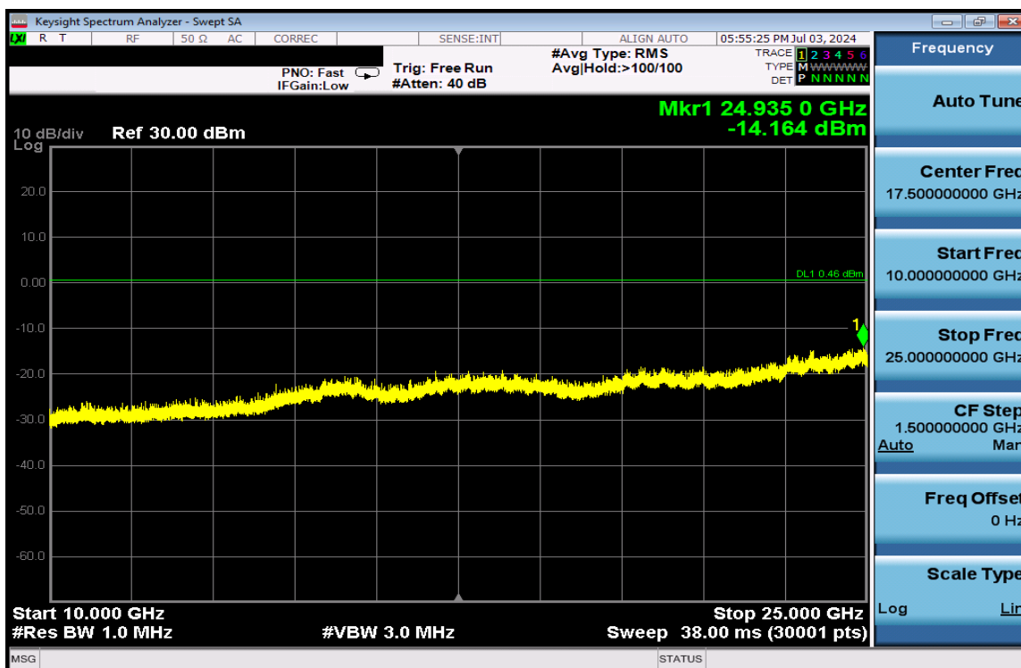
Plot 7-430. Conducted Spurious Plot Antenna 3a (802.11b – Ch. 1)
