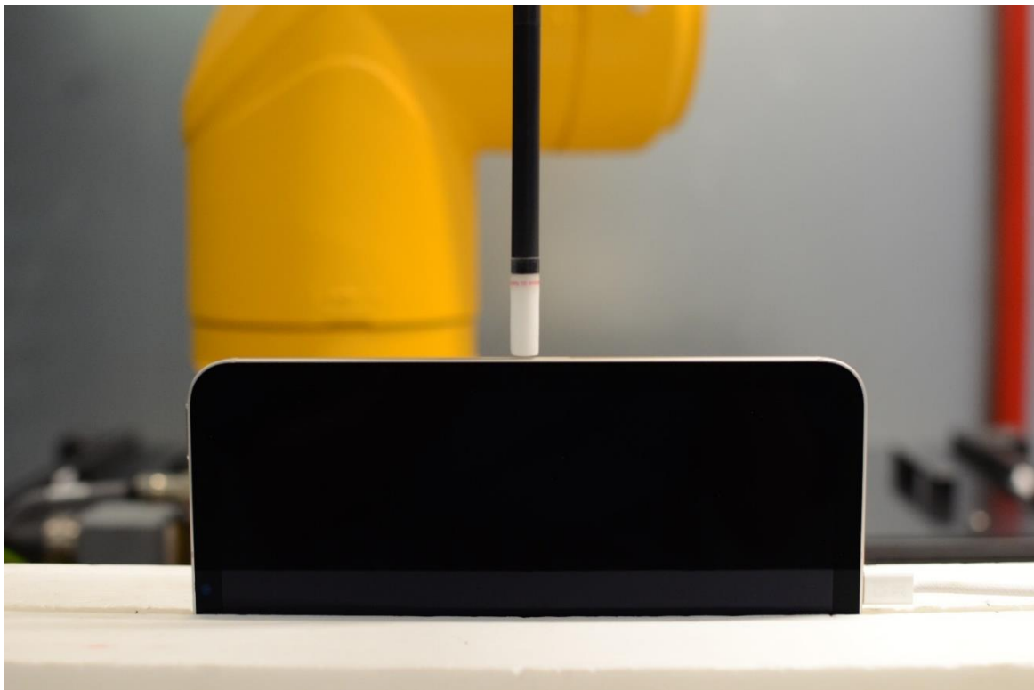
Near Field Power Density Test Setup 18: Body, Right Edge at 2mm – Ant 1b/3b/5T
