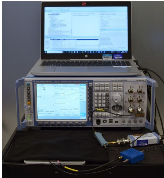
Test Setup Photo 3 – Conducted Test Setup (Figure 5-1b)
