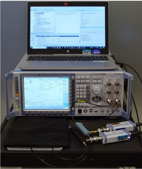
Test Setup Photo 5 – Conducted Test Setup (Figure 5-1d)
