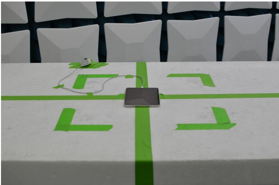
Figure 7: 30MHz-1GHz Test Setup (Front View)
