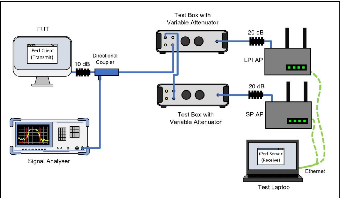
Figure 83 - Test Equipment Setup Diagram
