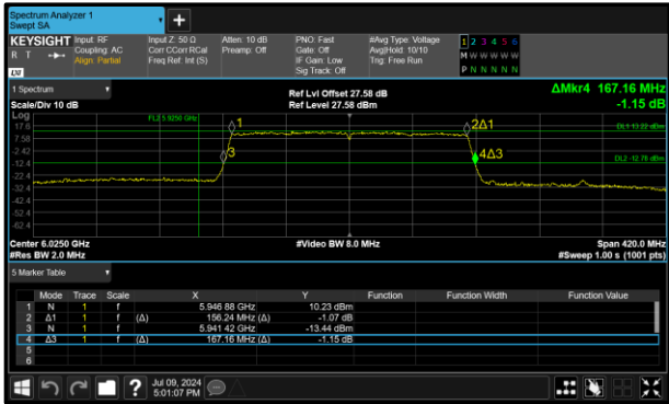
Figure 57 - 802.11ax HE160 SU SP Minimum 99% OBW
