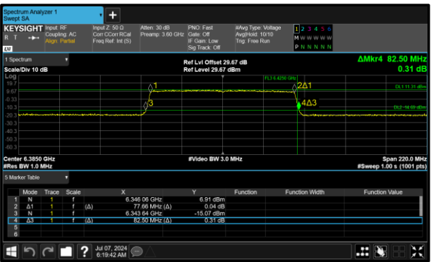
Figure 82 - 802.11ax HE80 SU SP Maximum 99% OBW
