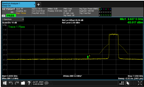
Figure 304 - A (Core 0) 6865 MHz (CH183)
