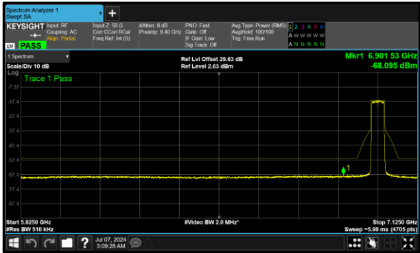
Figure 284 - A (Core 0) 7005 MHz (CH211)
