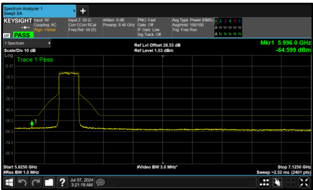
Figure 291 - B (Core 1) 6145 MHz (CH39)
