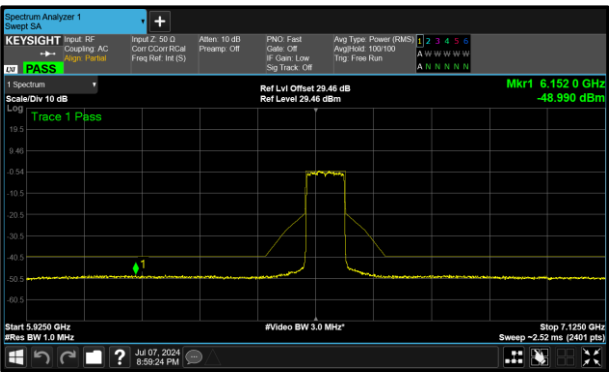
Figure 355 - B (Core 1) 6545 MHz (CH119)
