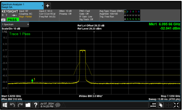
Figure 335 - B (Core 1) 6445 MHz (CH99)
