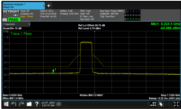
Figure 294 - A (Core 0) 6465 MHz (CH103)
