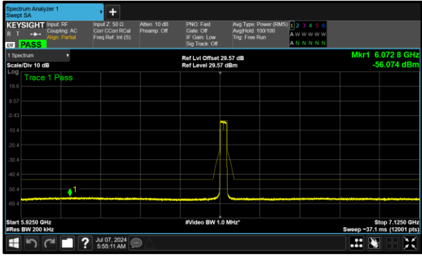
Figure 322 - A (Core 0) 6535 MHz (CH117)
