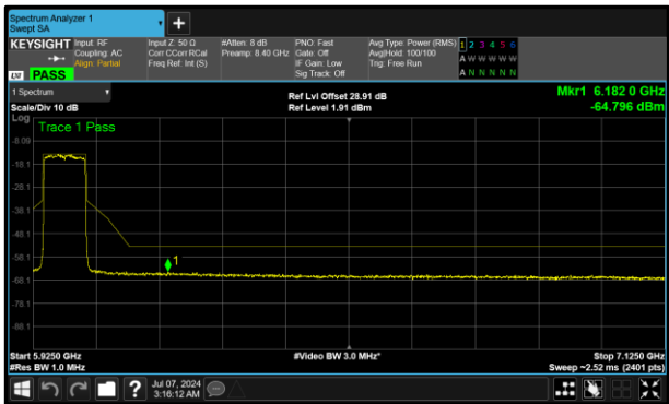
Figure 288 - A (Core 0) 5985 MHz (CH7)
