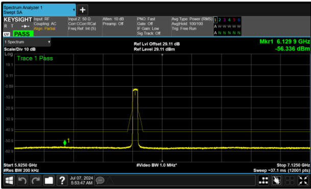
Figure 315 - B (Core 1) 6415 MHz (CH93)
