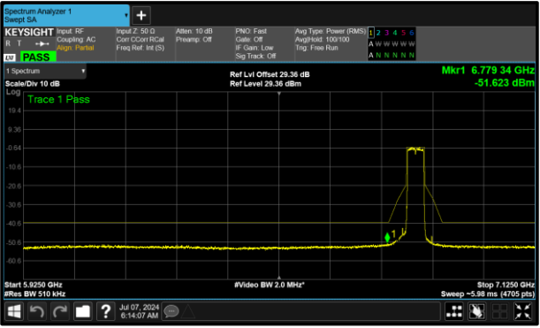
Figure 345 - B (Core 1) 6845 MHz (CH179)
