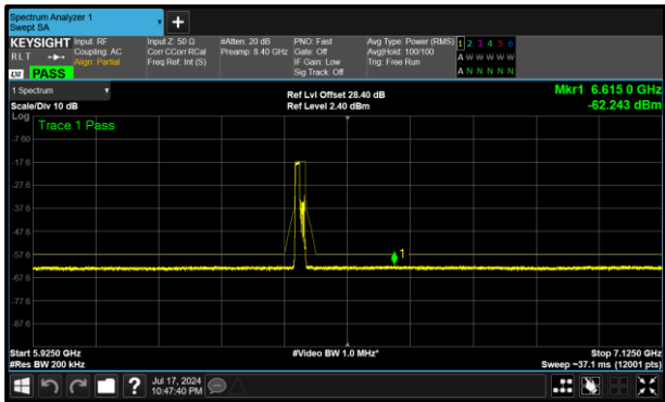
Figure 272 - B (Core 1) 802.11ax HE20 RU106 6435 MHz (CH97)
