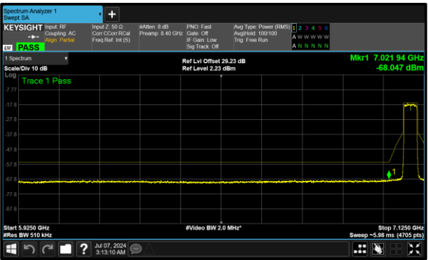
Figure 287 - B (Core 1) 7085 MHz (CH227)
