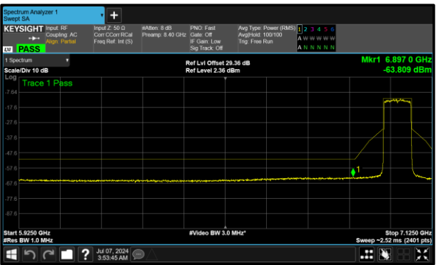
Figure 309 - B (Core 1) 7025 MHz (CH215)
