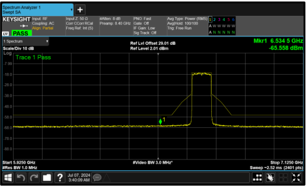
Figure 301 - B (Core 1) 6705 MHz (CH151)
