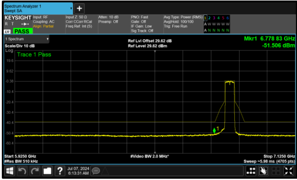
Figure 344 - A (Core 0) 6845 MHz (CH179)
