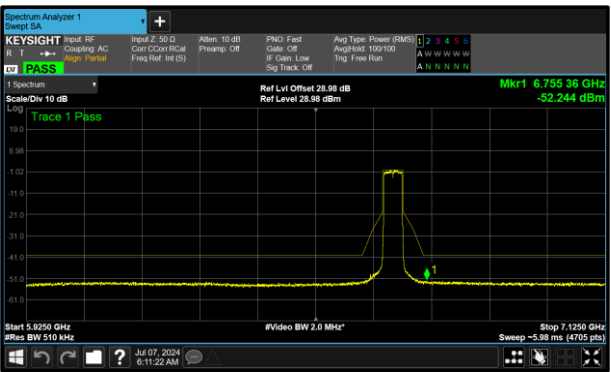
Figure 343 - B (Core 1) 6685 MHz (CH147)
