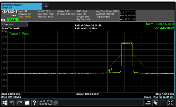
Figure 303 - B (Core 1) 6785 MHz (CH167)
