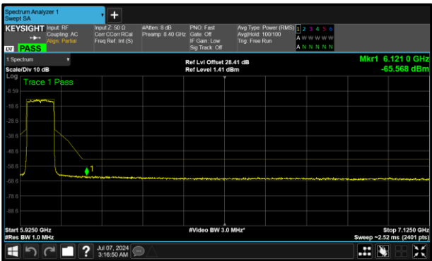
Figure 289 - B (Core 1) 5985 MHz (CH7)
