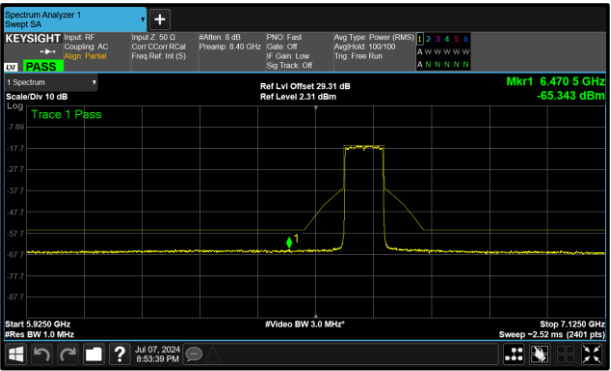
Figure 299 - B (Core 1) 6625 MHz (CH135)
