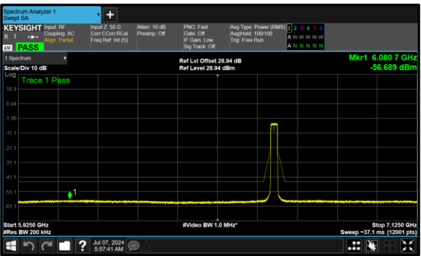
Figure 325 - B (Core 1) 6695 MHz (CH149)
