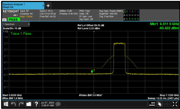
Figure 300 - A (Core 0) 6705 MHz (CH151)
