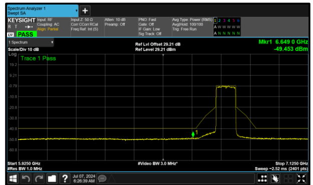
Figure 361 - B (Core 1) 6785 MHz (CH167)
