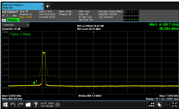
Figure 313 - B (Core 1) 6175 MHz (CH45)
