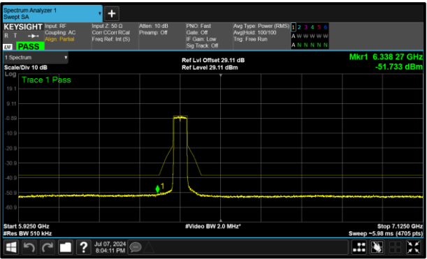
Figure 333 - B (Core 1) 6405 MHz (CH91)
