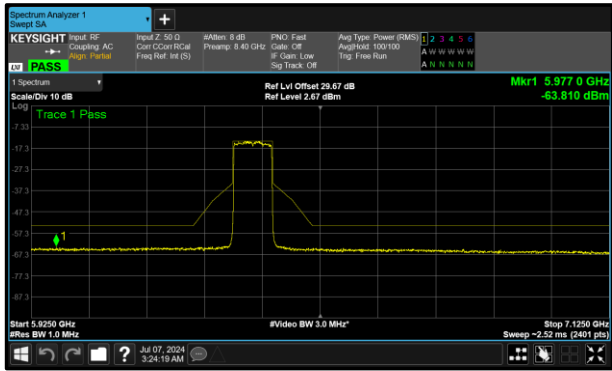
Figure 292 - A (Core 0) 6385 MHz (CH87)
