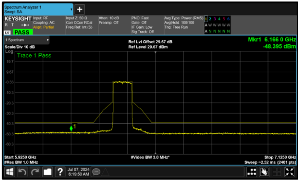
Figure 350 - A (Core 0) 6385 MHz (CH87)
