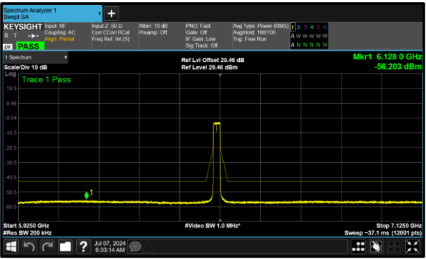
Figure 321 - B (Core 1) 6515 MHz (CH113)
