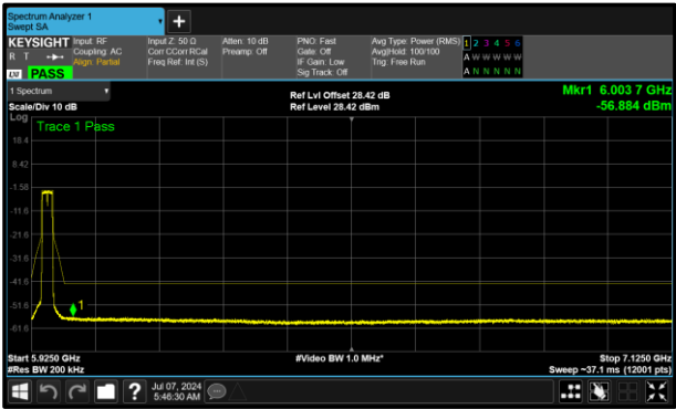
Figure 311 - B (Core 1) 5955 MHz (CH1)
