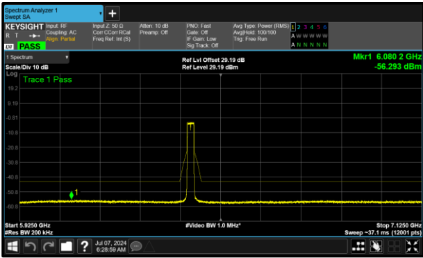
Figure 317 - B (Core 1) 6435 MHz (CH97)
