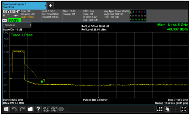
Figure 346 - A (Core 0) 5985 MHz (CH7)
