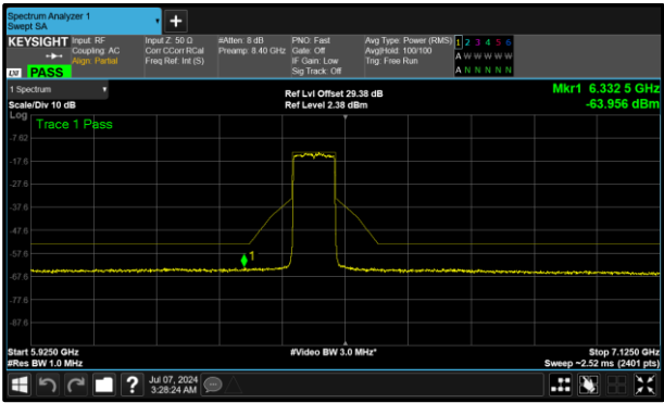
Figure 295 - B (Core 1) 6465 MHz (CH103)
