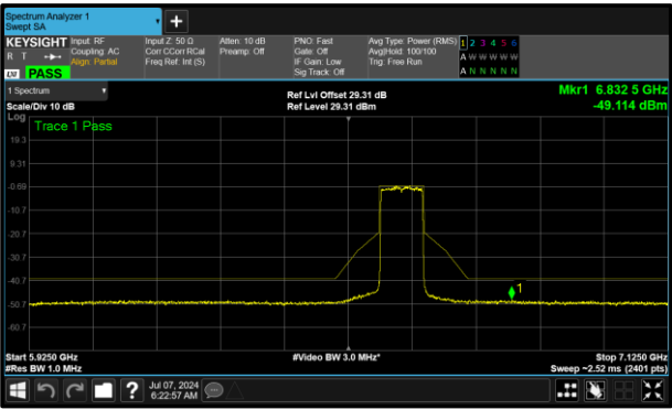
Figure 357 - B (Core 1) 6625 MHz (CH135)
