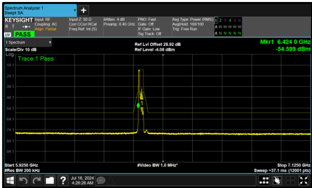
Figure 274 - A (Core 0) 802.11ax HE20 RU52 6435 MHz (CH97)
