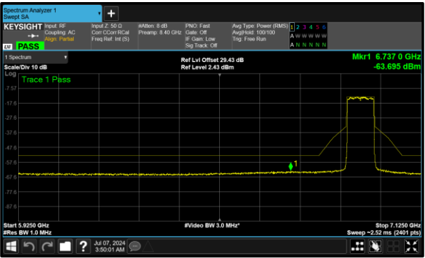
Figure 307 - B (Core 1) 6945 MHz (CH199)
