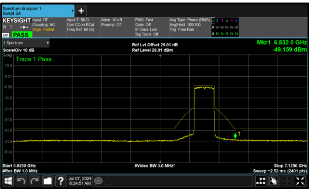
Figure 359 - B (Core 1) 6705 MHz (CH151)
