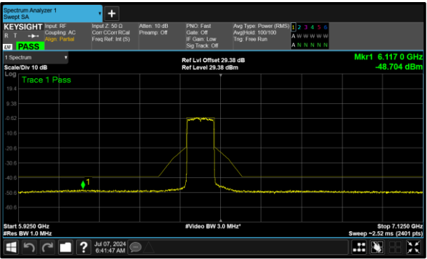
Figure 353 - B (Core 1) 6465 MHz (CH103)
