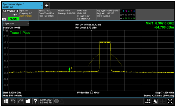
Figure 298 - A (Core 0) 6625 MHz (CH135)
