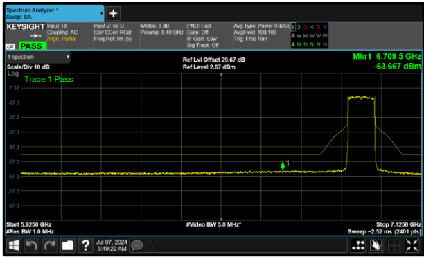
Figure 306 - A (Core 0) 6945 MHz (CH199)
