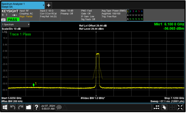
Figure 323 - B (Core 1) 6535 MHz (CH117)
