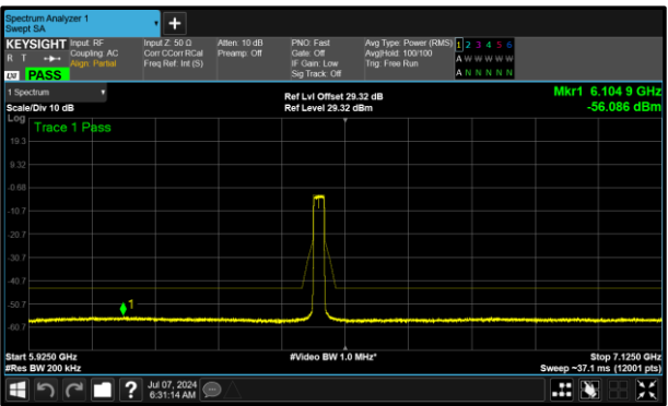
Figure 319 - B (Core 1) 6475 MHz (CH105)
