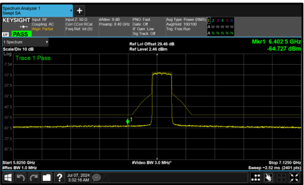
Figure 297 - B (Core 1) 6545 MHz (CH119)
