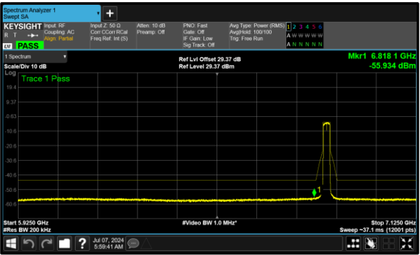
Figure 327 - B (Core 1) 6855 MHz (CH181)
