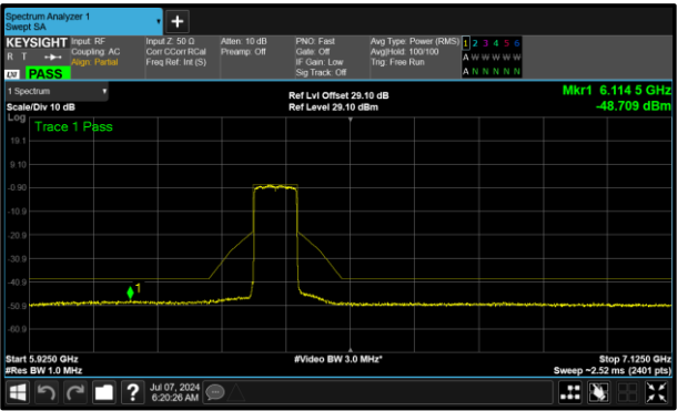
Figure 351 - B (Core 1) 6385 MHz (CH87)
