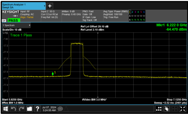
Figure 293 - B (Core 1) 6385 MHz (CH87)
