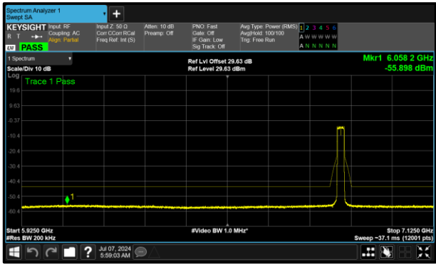
Figure 326 - A (Core 0) 6855 MHz (CH181)
