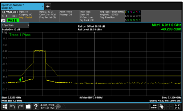
Figure 349 - B (Core 1) 6145 MHz (CH39)
