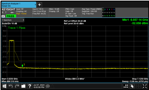
Figure 329 - B (Core 1) 5965 MHz (CH3)
