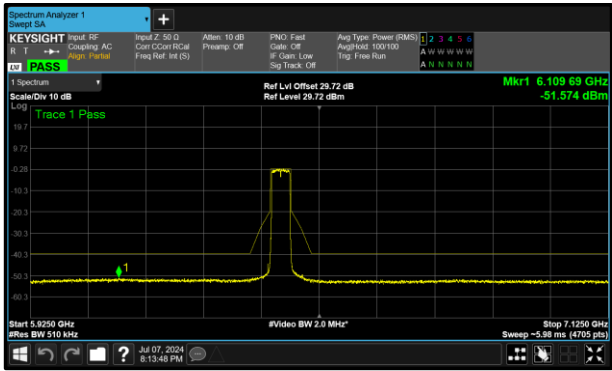
Figure 334 - A (Core 0) 6445 MHz (CH99)
