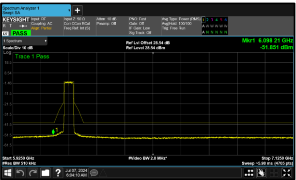
Figure 331 - B (Core 1) 6165 MHz (CH43)
