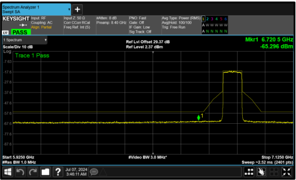
Figure 305 - B (Core 1) 6865 MHz (CH183)
