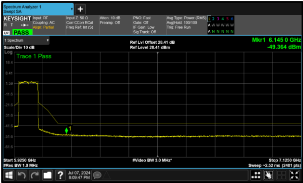
Figure 347 - B (Core 1) 5985 MHz (CH7)
