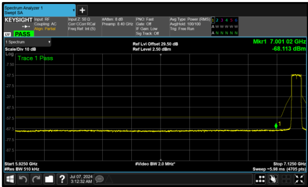
Figure 286 - A (Core 0) 7085 MHz (CH227)
