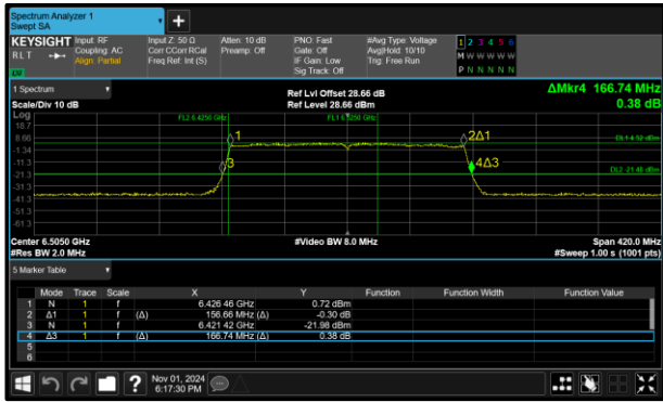
Figure 19 - 802.11ax HE160 SU LPI Minimum 26 dB EBW
