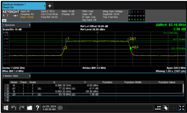
Figure 18 - 802.11ax HE80 SU LPI Maximum 26 dB EBW
