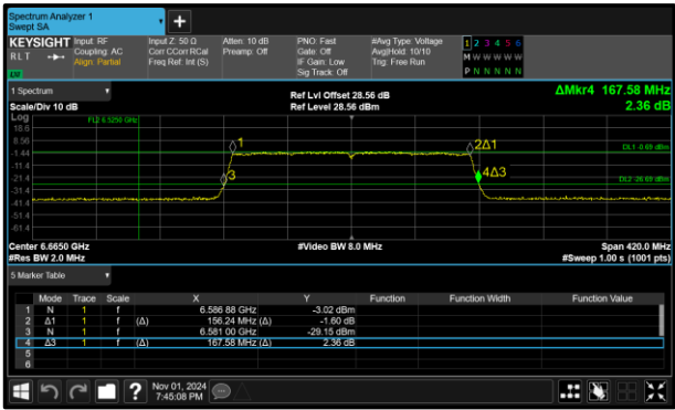
Figure 30 - 802.11ax HE160 SU VLP Maximum 26 dB EBW
