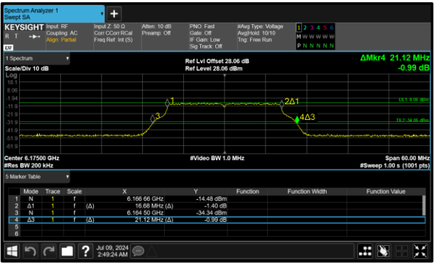
Figure 42 - 802.11a LPI Maximum 99% OBW
