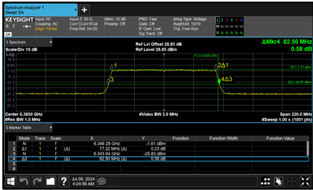
Figure 17 - 802.11ax HE80 SU LPI Minimum 26 dB EBW
