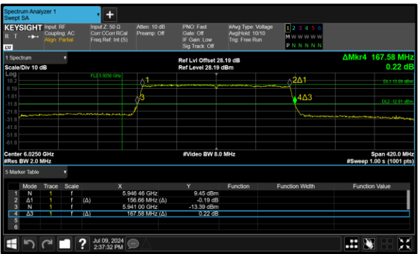
Figure 40 - 802.11ax HE160 SU SP Maximum 99% OBW
