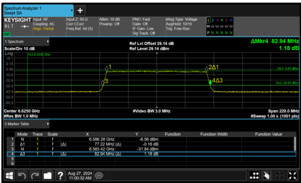
Figure 28 - 802.11ax HE80 SU VLP Maximum 26 dB EBW
