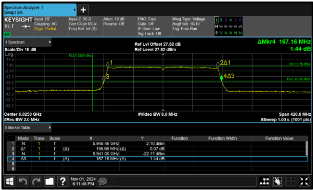
Figure 20 - 802.11ax HE160 SU LPI Maximum 26 dB EBW
