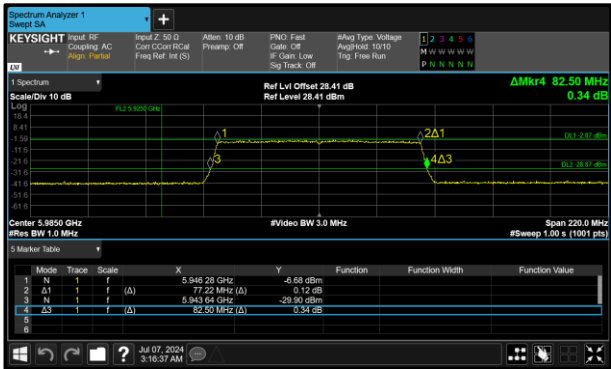
Figure 147 - 802.11ax HE80 SU LPI Minimum 26 dB EBW
