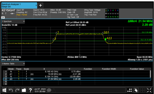
Figure 150 - 802.11ax HE20 SU SP Maximum 26 dB EBW
