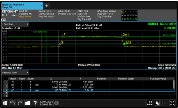
Figure 154 - 802.11ax HE80 SU SP Maximum 26 dB EBW
