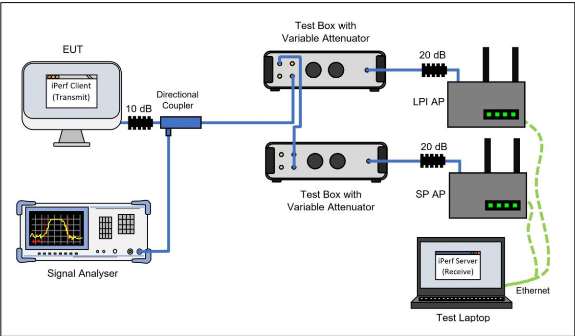
Figure 165 - Test Equipment Setup Diagram
