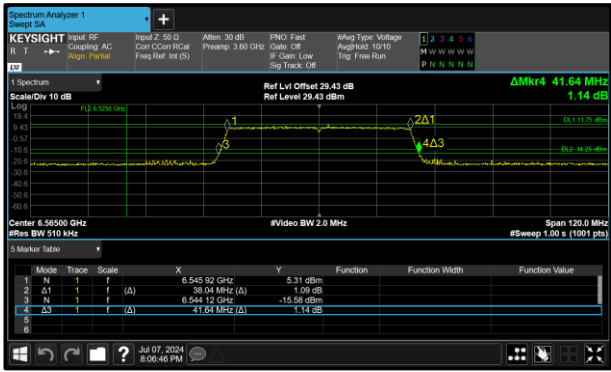
Figure 151 - 802.11ax HE40 SU SP Minimum 26 dB EBW
