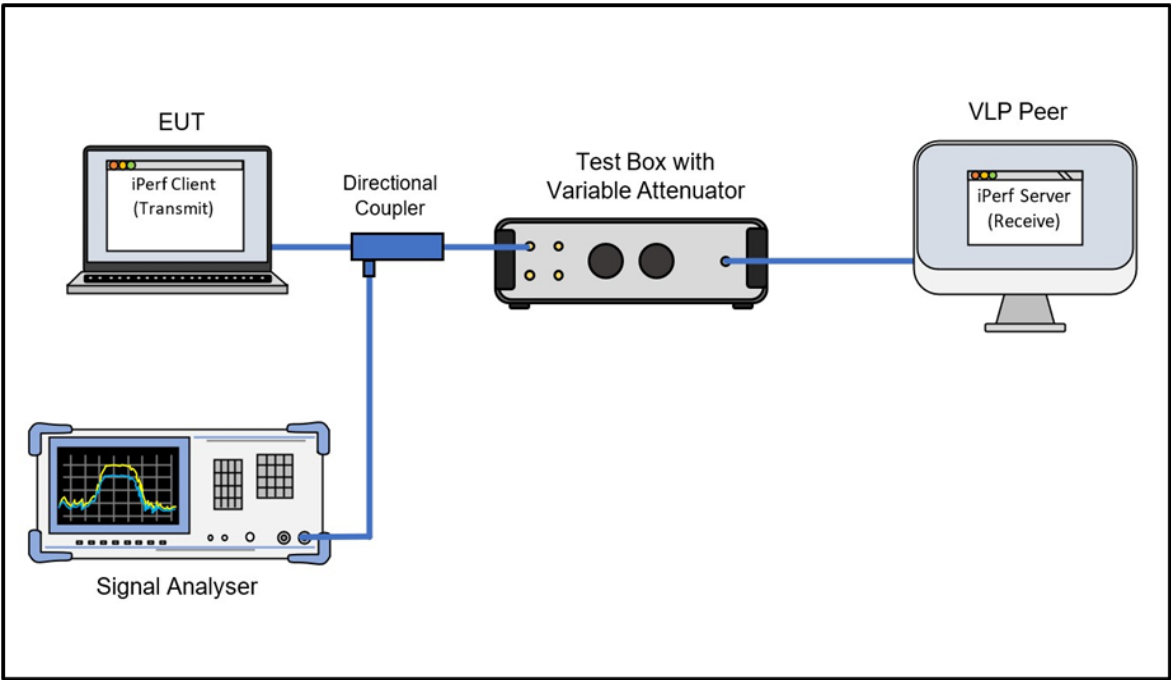
Figure 166 - Test Equipment Setup Diagram
