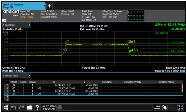
Figure 148 - 802.11ax HE80 SU LPI Maximum 26 dB EBW
