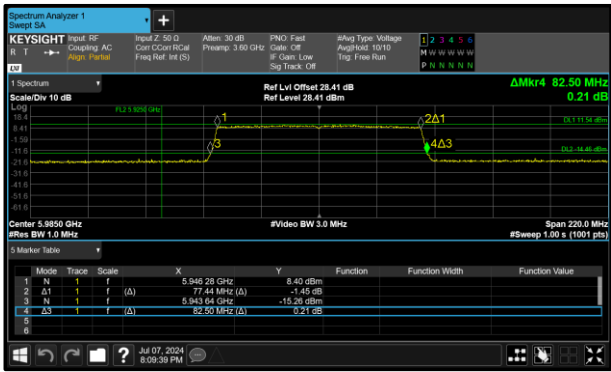
Figure 153 - 802.11ax HE80 SU SP Minimum 26 dB EBW
