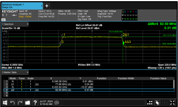
Figure 164 - 802.11ax HE80 SU SP Maximum 99% OBW
