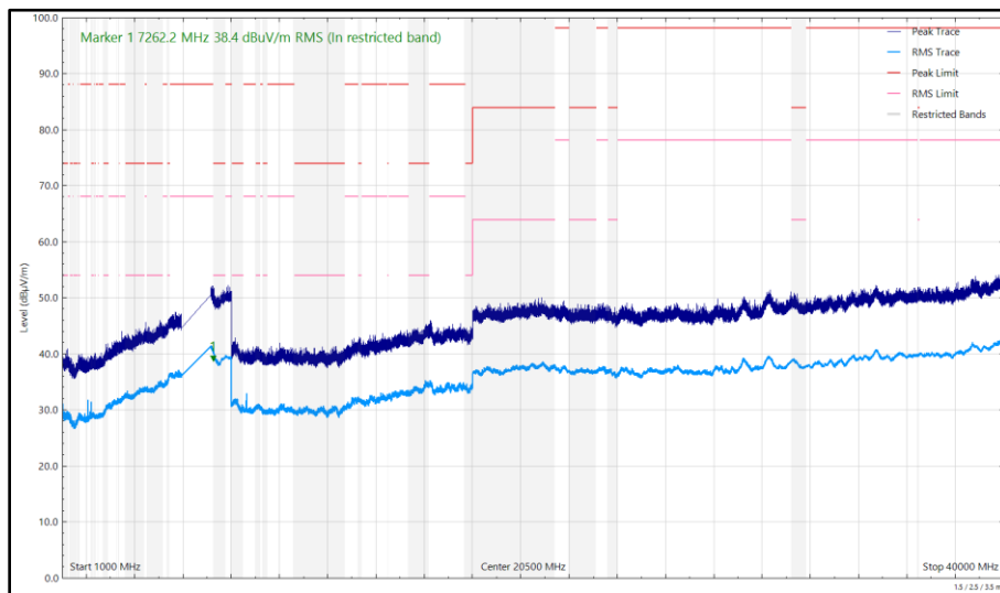
Figure 303 - 6895 MHz (CH189), HE20, SU, CDD, Core 0 + Core 1, 1 GHz to 40 GHz, Horizontal
