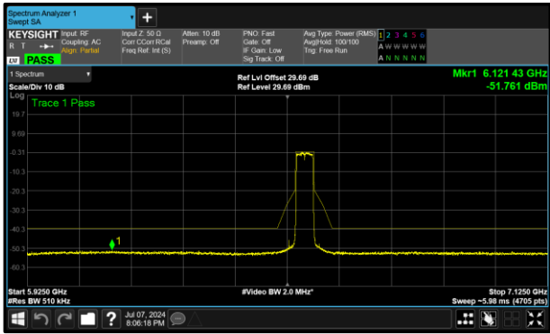
Figure 422 - A (Core 0) 6565 MHz (CH123)
