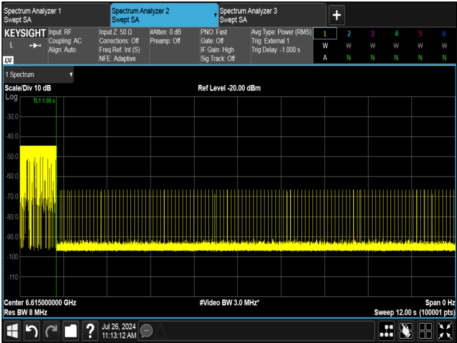
Figure 456 - U-NII-7, Minimum Bandwidth (AWGN Mid)
