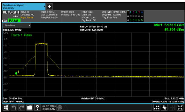
Figure 372 - A (Core 0) 6145 MHz (CH39)
