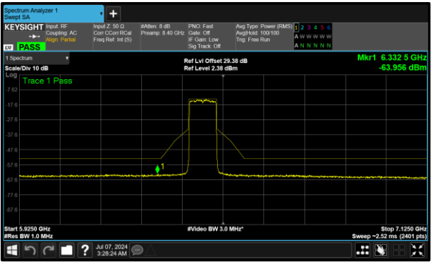
Figure 377 - B (Core 1) 6465 MHz (CH103)
