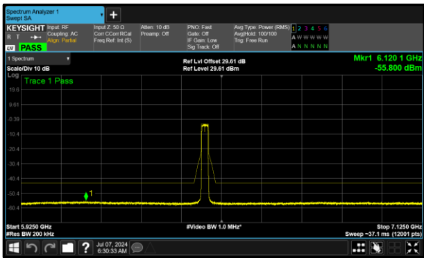
Figure 400 - A (Core 0) 6475 MHz (CH105)
