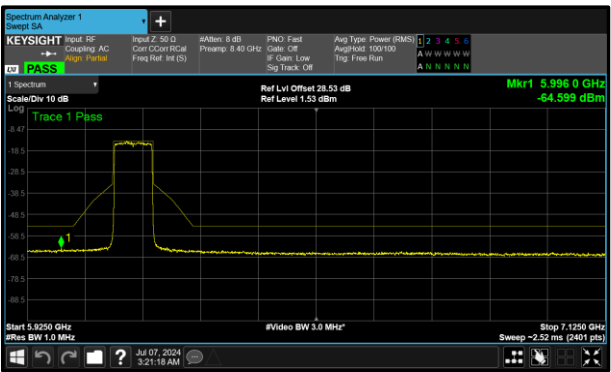
Figure 373 - B (Core 1) 6145 MHz (CH39)
