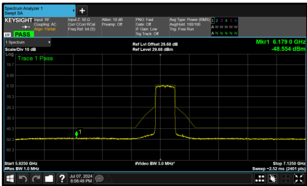
Figure 436 - A (Core 0) 6545 MHz (CH119)
