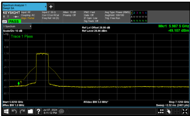
Figure 430 - A (Core 0) 6145 MHz (CH39)
