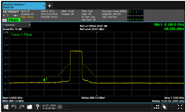
Figure 432 - A (Core 0) 6385 MHz (CH87)
