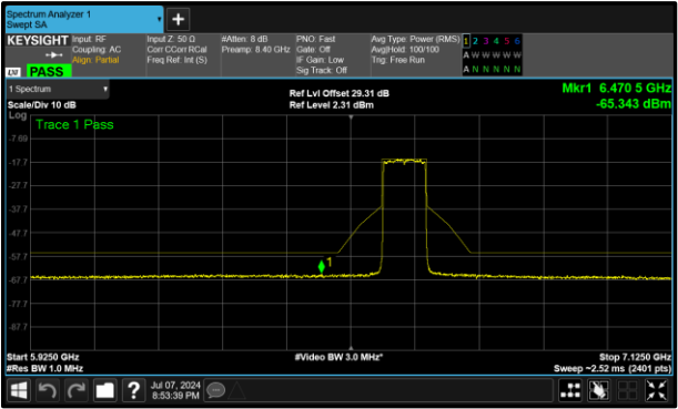
Figure 381 - B (Core 1) 6625 MHz (CH135)
