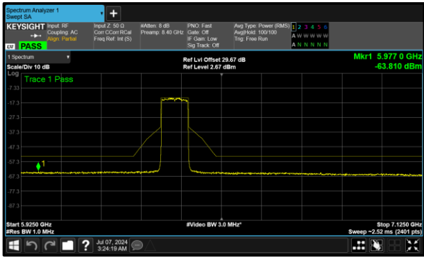
Figure 374 - A (Core 0) 6385 MHz (CH87)
