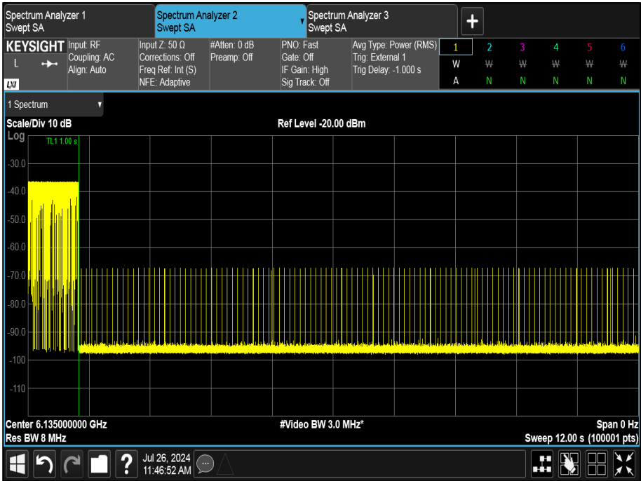
Figure 449 - U-NII-5, Minimum Bandwidth (AWGN High)
