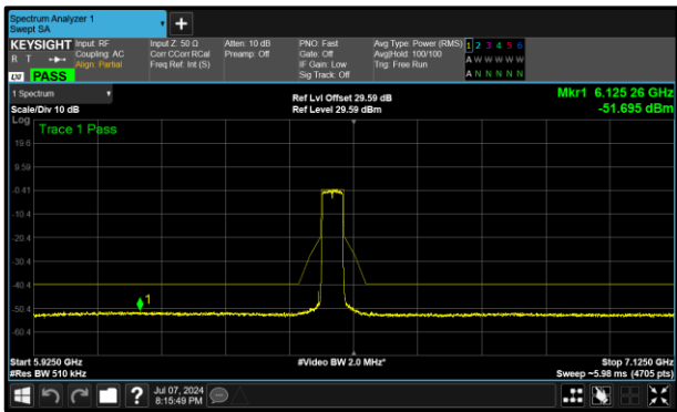
Figure 418 - A (Core 0) 6485 MHz (CH107)
