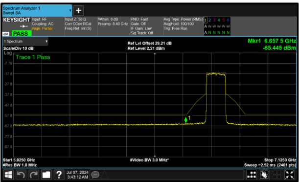
Figure 385 - B (Core 1) 6785 MHz (CH167)
