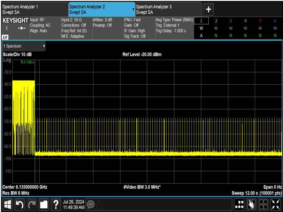
Figure 448 - U-NII-5, Minimum Bandwidth (AWGN Mid)
