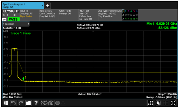
Figure 410 - A (Core 0) 5965 MHz (CH3)
