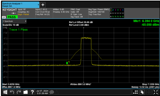
Figure 378 - A (Core 0) 6545 MHz (CH119)
