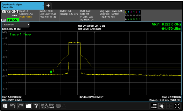
Figure 375 - B (Core 1) 6385 MHz (CH87)
