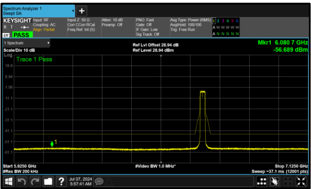
Figure 407 - B (Core 1) 6695 MHz (CH149)
