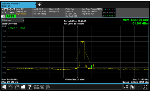
Figure 423 - B (Core 1) 6565 MHz (CH123)
