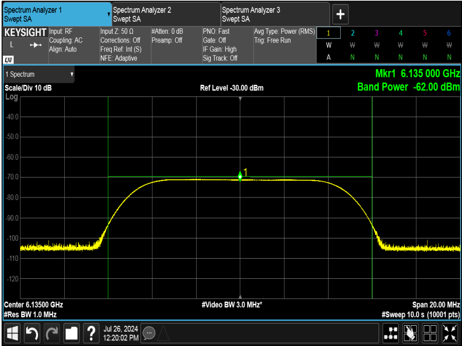
Figure 445 - Example of AWGN Signal
