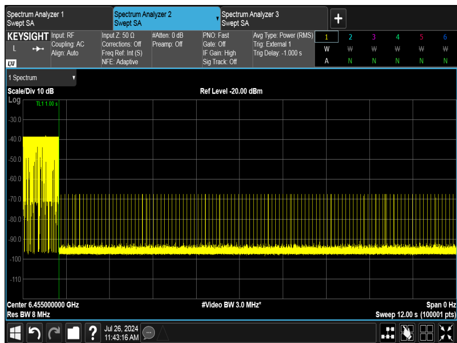
Figure 451 - U-NII-6, Minimum Bandwidth (AWGN Low)
