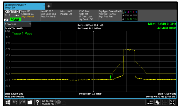
Figure 443 - B (Core 1) 6785 MHz (CH167)
