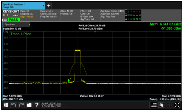
Figure 414 - A (Core 0) 6405 MHz (CH91)
