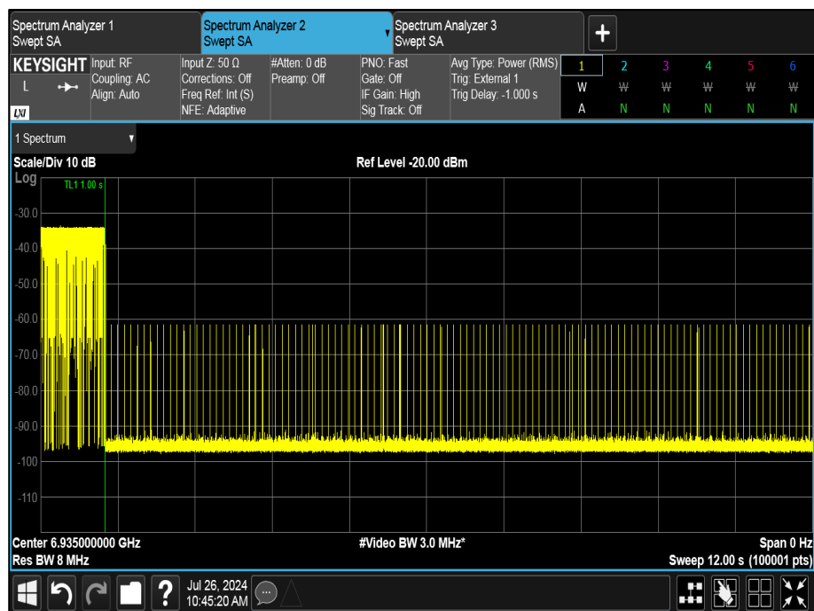
Figure 461 - U-NII-8, Minimum Bandwidth (AWGN High)
