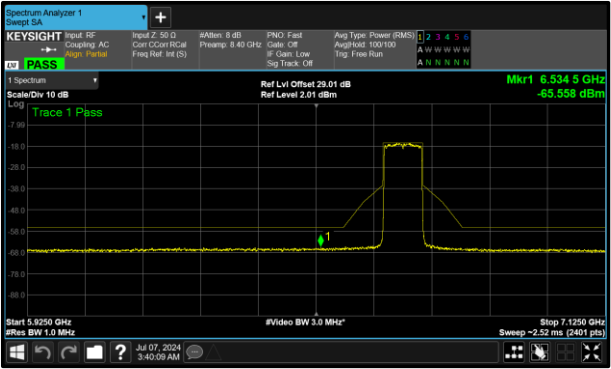
Figure 383 - B (Core 1) 6705 MHz (CH151)
