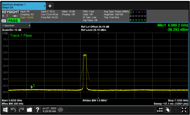
Figure 399 - B (Core 1) 6435 MHz (CH97)
