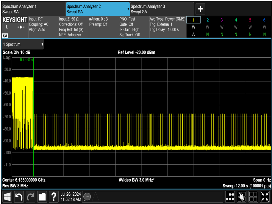
Figure 447 - U-NII-5, Minimum Bandwidth (AWGN Low)
