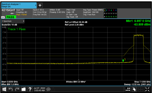
Figure 391 - B (Core 1) 7025 MHz (CH215)
