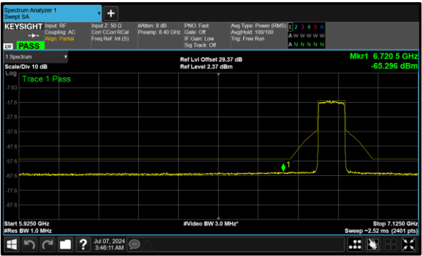
Figure 387 - B (Core 1) 6865 MHz (CH183)
