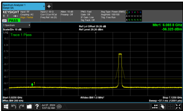
Figure 406 - A (Core 0) 6695 MHz (CH149)
