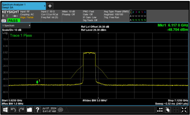
Figure 435 - B (Core 1) 6465 MHz (CH103)
