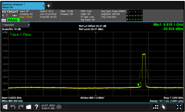
Figure 409 - B (Core 1) 6855 MHz (CH181)
