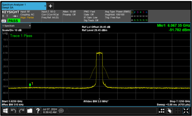
Figure 421 - B (Core 1) 6525 MHz (CH115)
