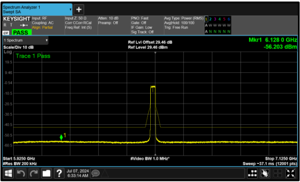
Figure 403 - B (Core 1) 6515 MHz (CH113)
