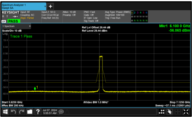
Figure 405 - B (Core 1) 6535 MHz (CH117)
