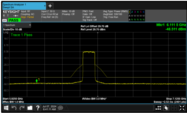
Figure 434 - A (Core 0) 6465 MHz (CH103)
