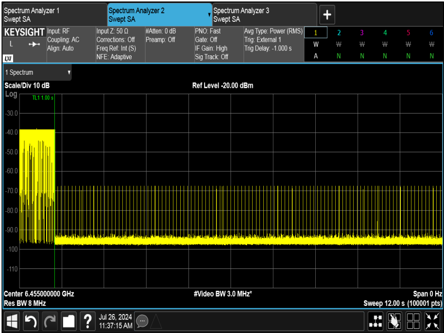
Figure 453 - U-NII-6, Minimum Bandwidth (AWGN High)
