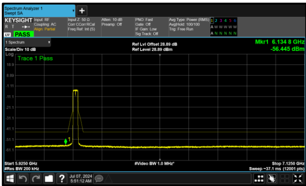
Figure 394 - A (Core 0) 6175 MHz (CH45)
