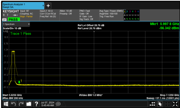
Figure 392 - A (Core 0) 5955 MHz (CH1)
