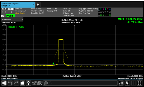
Figure 415 - B (Core 1) 6405 MHz (CH91)
