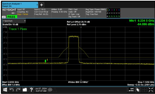
Figure 376 - A (Core 0) 6465 MHz (CH103)
