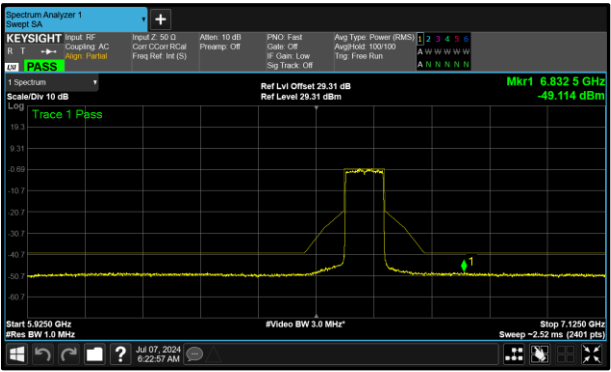
Figure 439 - B (Core 1) 6625 MHz (CH135)
