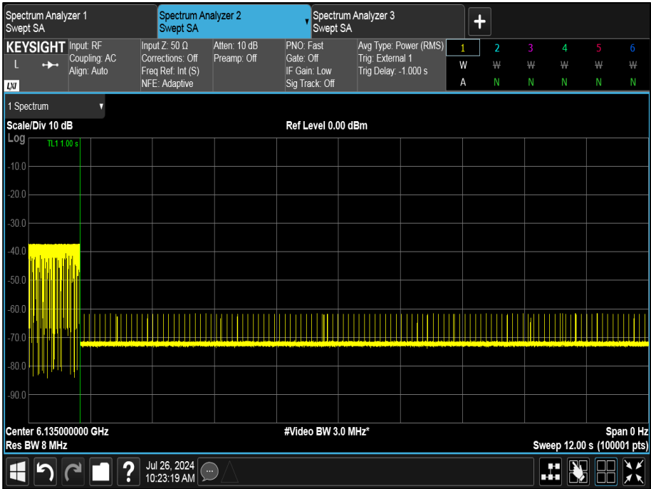
Figure 446 - U-NII-5, Minimum Bandwidth
