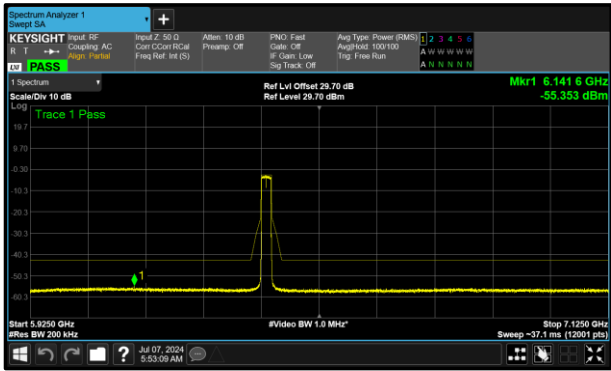
Figure 396 - A (Core 0) 6415 MHz (CH93)
