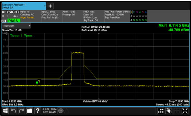
Figure 433 - B (Core 1) 6385 MHz (CH87)
