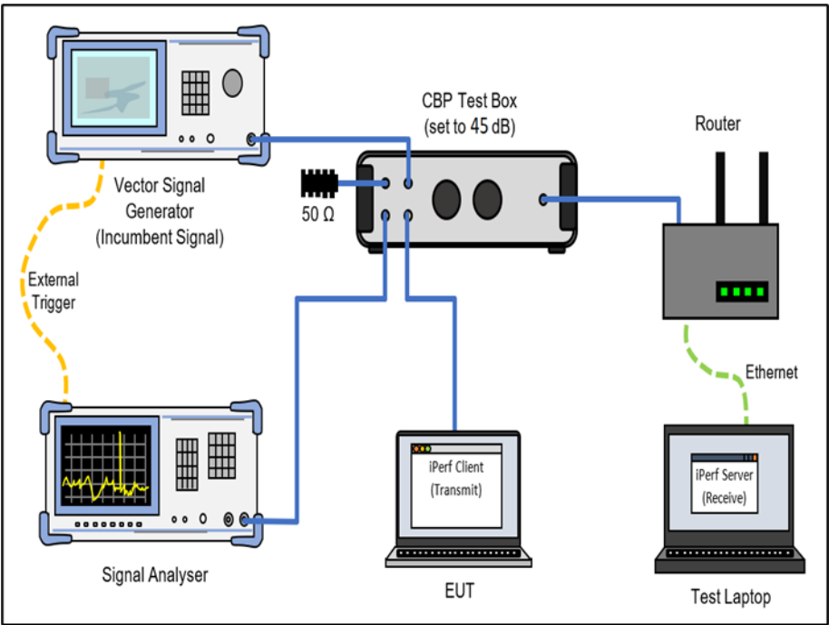
Figure 444 - Test Equipment Setup Diagram
