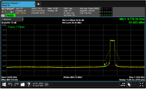
Figure 427 - B (Core 1) 6845 MHz (CH179)
