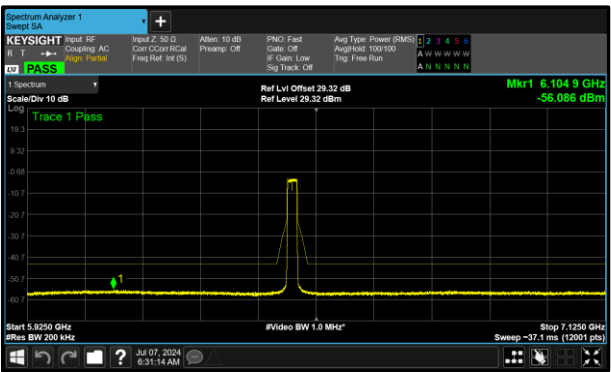
Figure 401 - B (Core 1) 6475 MHz (CH105)
