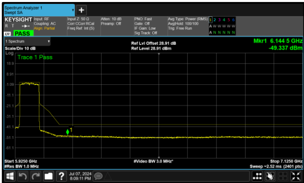
Figure 428 - A (Core 0) 5985 MHz (CH7)
