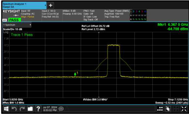
Figure 380 - A (Core 0) 6625 MHz (CH135)
