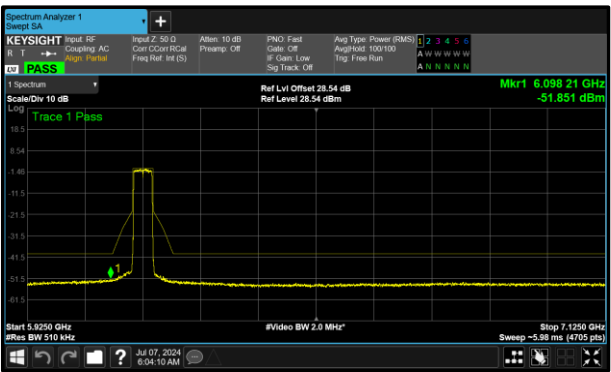
Figure 413 - B (Core 1) 6165 MHz (CH43)
