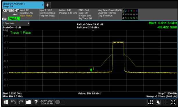
Figure 382 - A (Core 0) 6705 MHz (CH151)
