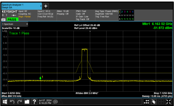
Figure 419 - B (Core 1) 6485 MHz (CH107)
