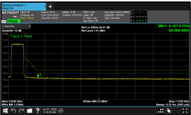
Figure 371 - B (Core 1) 5985 MHz (CH7)
