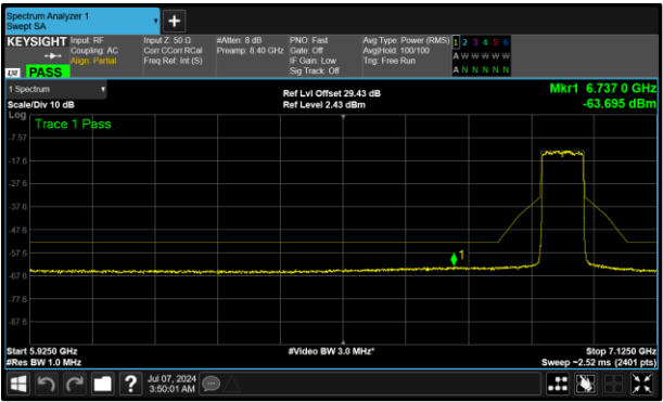
Figure 389 - B (Core 1) 6945 MHz (CH199)
