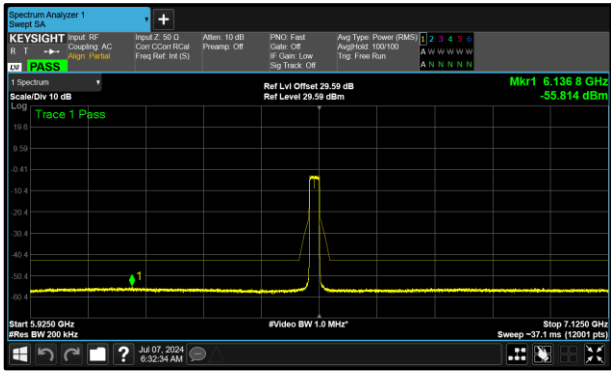
Figure 402 - A (Core 0) 6515 MHz (CH113)
