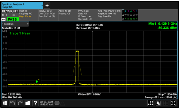
Figure 397 - B (Core 1) 6415 MHz (CH93)
