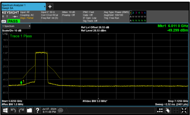
Figure 431 - B (Core 1) 6145 MHz (CH39)
