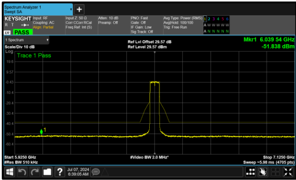
Figure 420 - A (Core 0) 6525 MHz (CH115)
