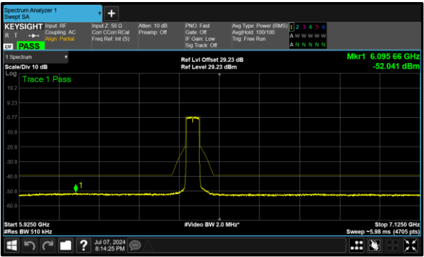
Figure 417 - B (Core 1) 6445 MHz (CH99)
