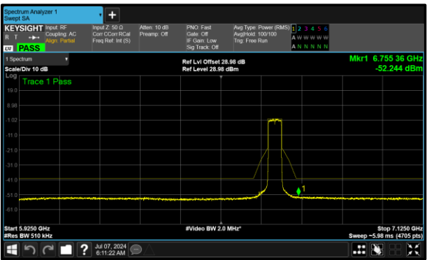
Figure 425 - B (Core 1) 6685 MHz (CH147)
