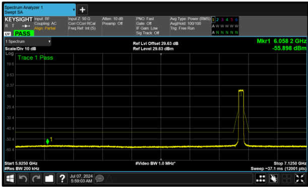
Figure 408 - A (Core 0) 6855 MHz (CH181)
