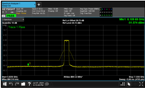
Figure 416 - A (Core 0) 6445 MHz (CH99)
