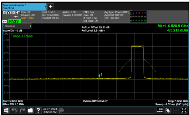
Figure 384 - A (Core 0) 6785 MHz (CH167)
