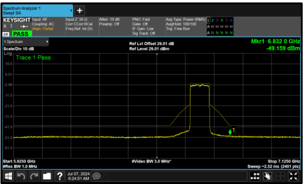
Figure 441 - B (Core 1) 6705 MHz (CH151)
