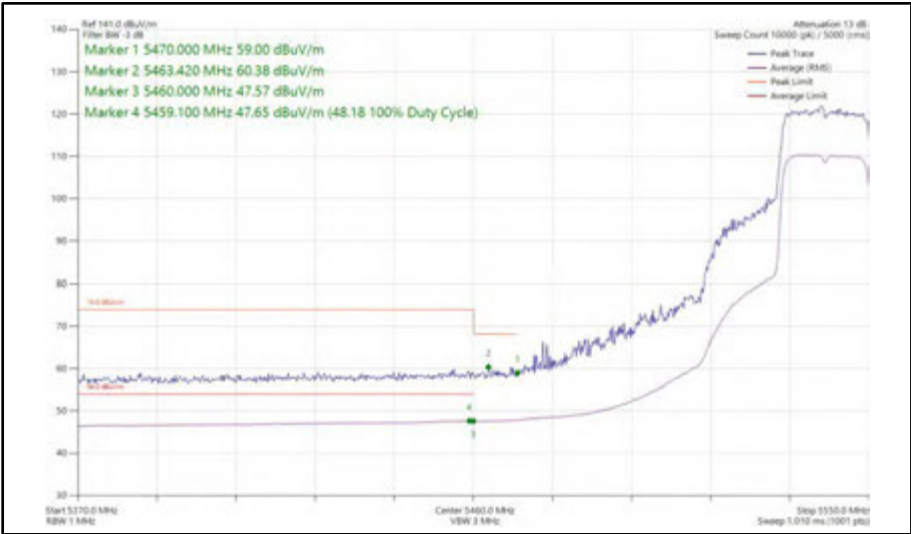
Figure 379 - 802.11ax HE20, SU, SISO, Core 0 - 5540 MHz Band Edge Frequency 5470 MHz
