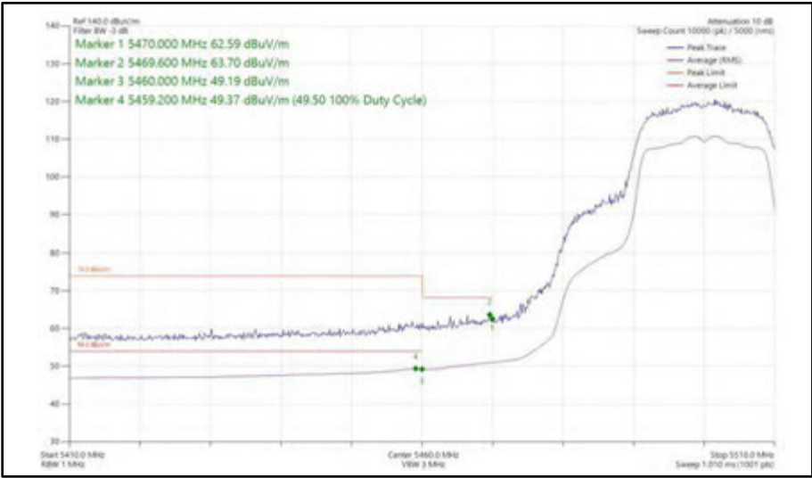
Figure 373 - 802.11n HT20, SISO, Core 0 - 5500 MHz Band Edge Frequency 5470 MHz
