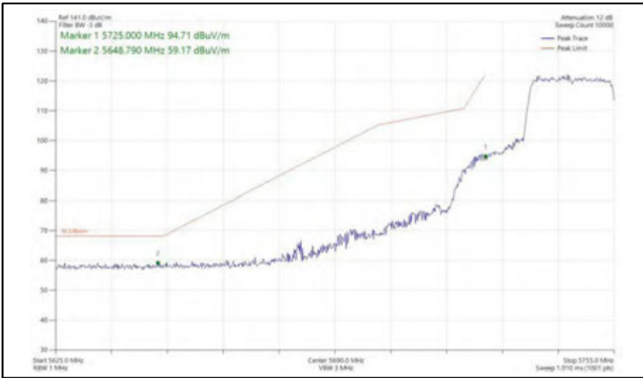
Figure 384 - 802.11ax HE20, SU, SISO, Core 0 - 5745 MHz Band Edge Frequency 5725 MHz
