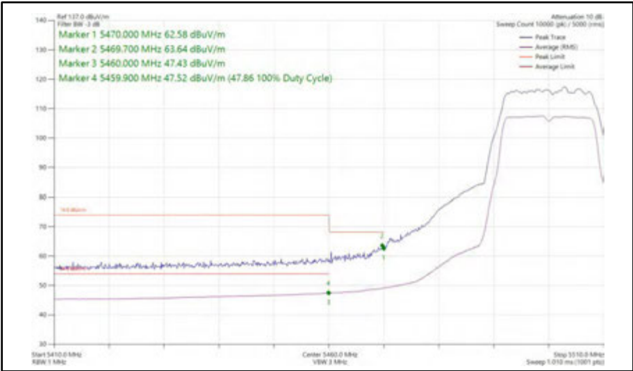
Figure 371 - 802.11a, SISO, Core 0 - 5500 MHz Band Edge Frequency 5470 MHz
