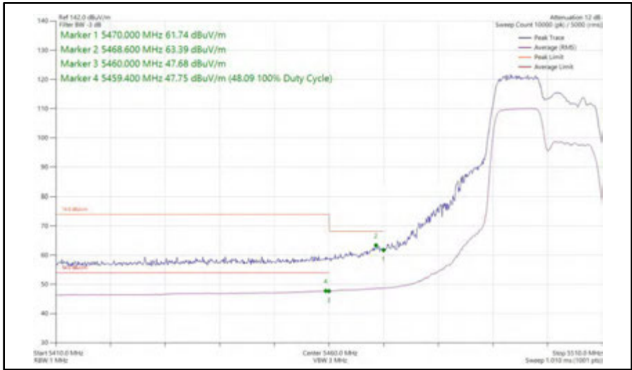
Figure 376 - 802.11ax HE20, RU 106-53, SISO, Core 0 - 5500 MHz Band Edge Frequency 5470 MHz
