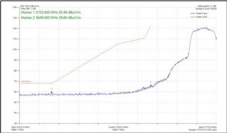
Figure 383 - 802.11n HT20, SISO, Core 0 - 5765 MHz Band Edge Frequency 5725 MHz
