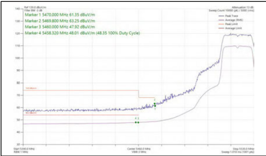
Figure 374 - 802.11n HT20, SISO, Core 0 - 5520 MHz Band Edge Frequency 5470 MHz
