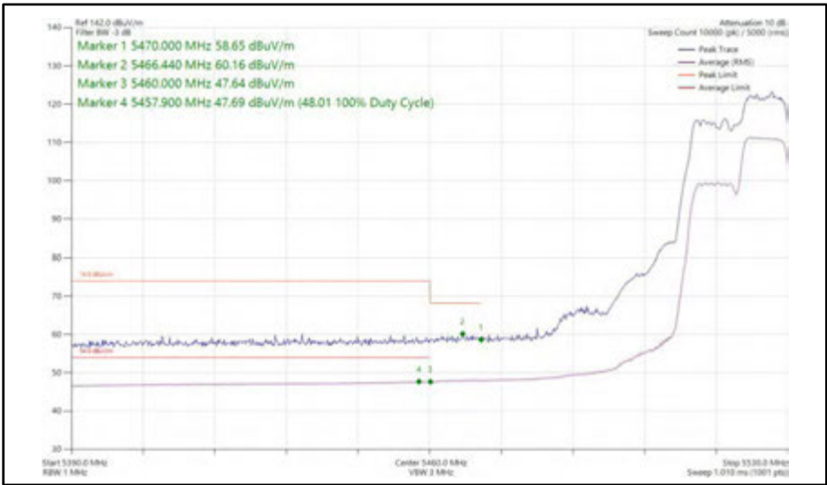
Figure 378 - 802.11ax HE20, RU 106-54, SISO, Core 0 - 5520 MHz Band Edge Frequency 5470 MHz
