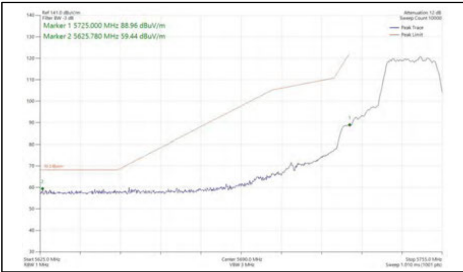
Figure 380 - 802.11a, SISO, Core 0 - 5745 MHz Band Edge Frequency 5725 MHz
