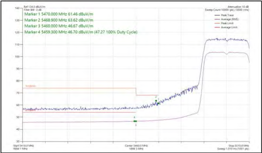
Figure 375 - 802.11ax HE20, SU, SISO, Core 0 - 5500 MHz Band Edge Frequency 5470 MHz
