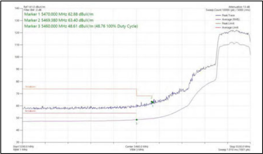
Figure 377 - 802.11ax HE20, SU, SISO, Core 0 - 5520 MHz Band Edge Frequency 5470 MHz
