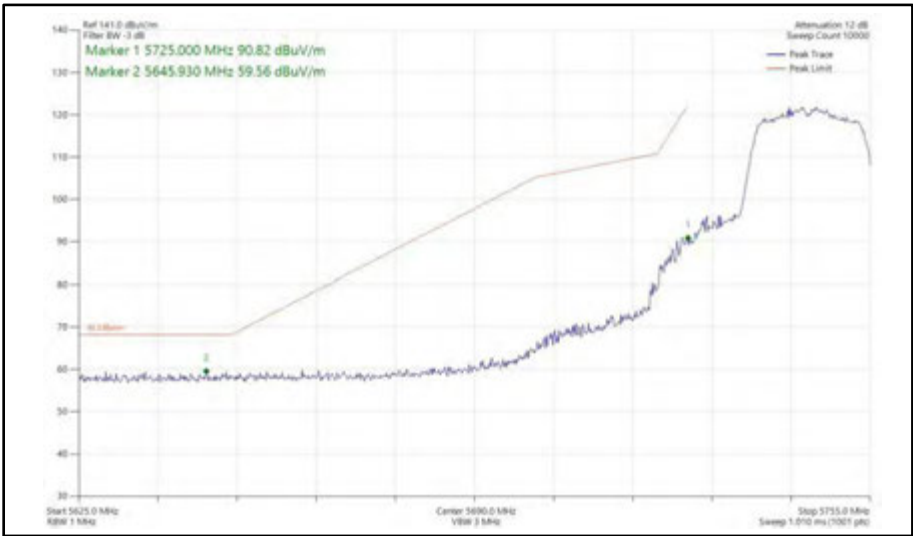
Figure 382 - 802.11n HT20, SISO, Core 0 - 5745 MHz Band Edge Frequency 5725 MHz
