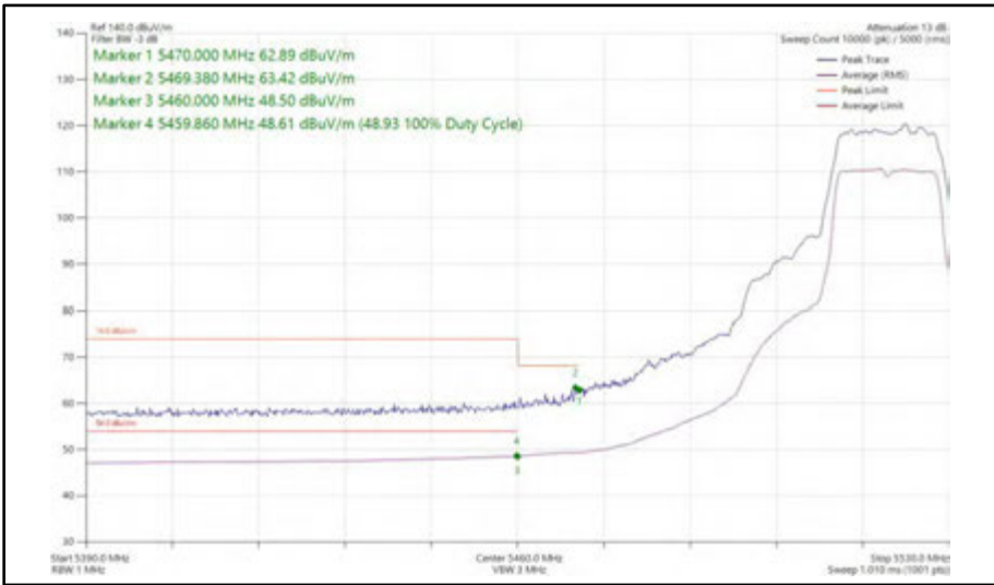
Figure 372 - 802.11a, SISO, Core 0 - 5520 MHz Band Edge Frequency 5470 MHz
