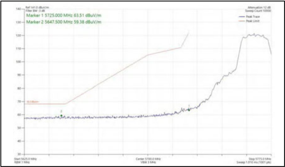
Figure 381 - 802.11a, SISO, Core 0 - 5765 MHz Band Edge Frequency 5725 MHz
