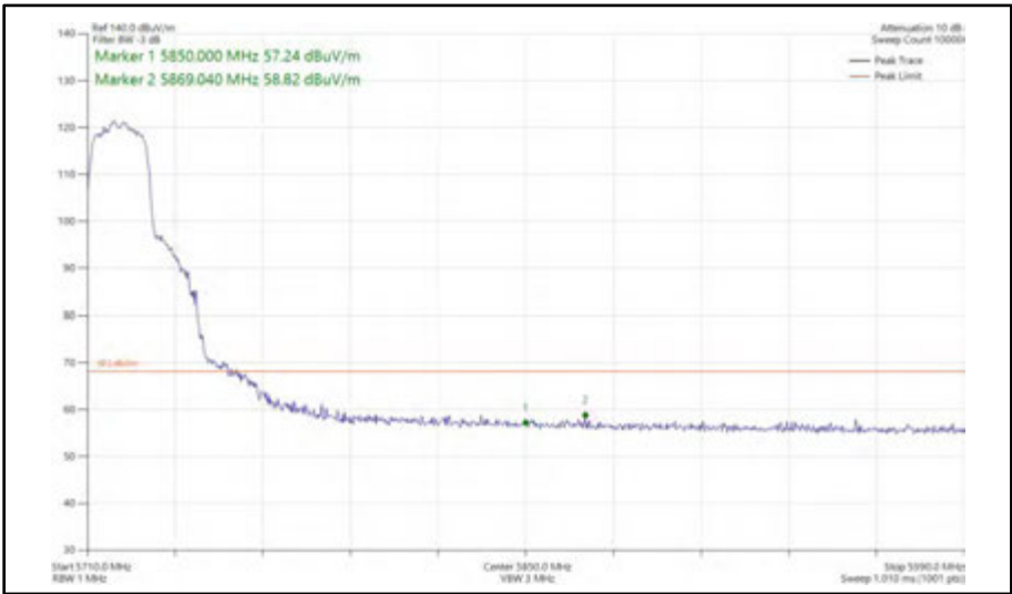
Figure 400 - 802.11n HT20, SISO, Core 0 - 5720 MHz Band Edge Frequency 5850 MHz
