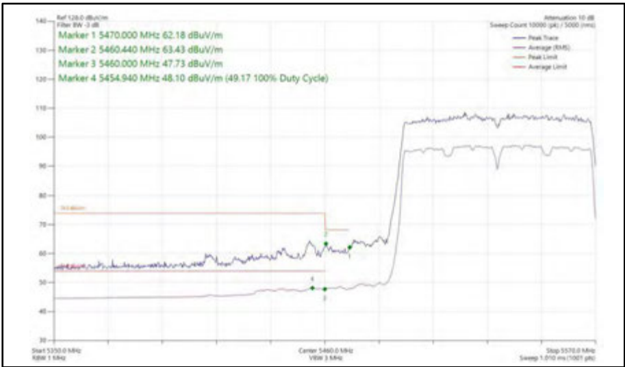
Figure 629 - 802.11ac VHT80, SISO, Core 1 - 5530 MHz Band Edge Frequency 5470 MHz
