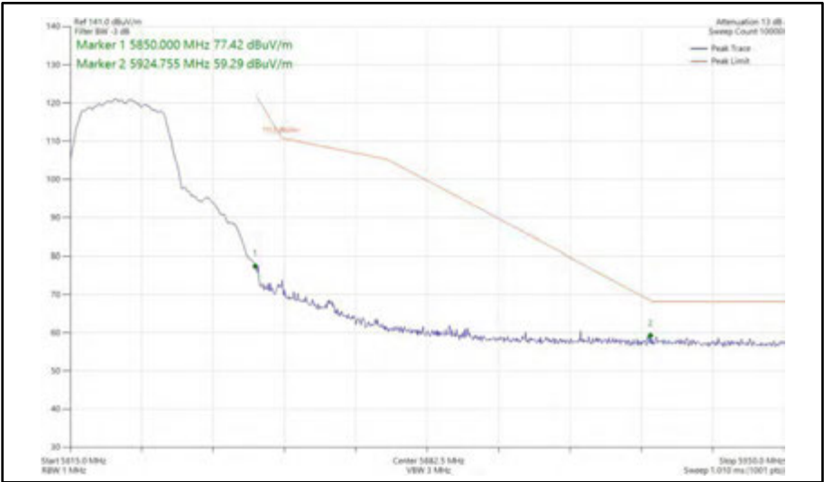
Figure 399 - 802.11a, SISO, Core 0 - 5825 MHz Band Edge Frequency 5850 MHz
