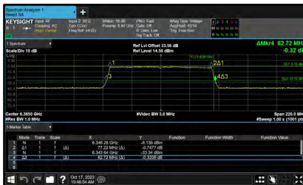
Figure 67 - Core 0 (A) 6385 MHz (CH87) 26 dB and 99% Bandwidth
