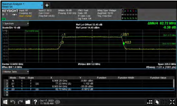
Figure 92 - Core 1 (B) 6945 MHz (CH199) 26 dB and 99% Bandwidth
