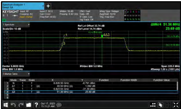
Figure 81 - Core 0 (A) 6865 MHz (CH183) 26 dB and 99% Bandwidth
