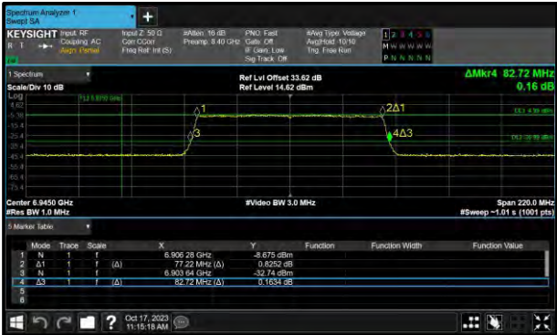
Figure 91 - Core 0 (A) 6945 MHz (CH199) 26 dB and 99% Bandwidth
