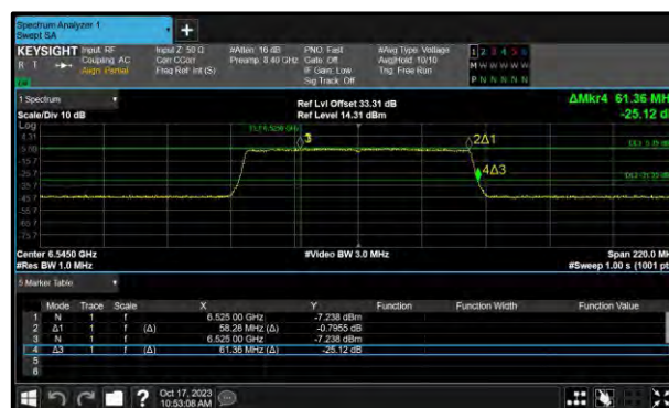
Figure 74 - Core 1 (B) 6545 MHz (CH119) 26 dB and 99% Bandwidth
