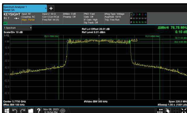
Figure 314 - 802.11ax HE80 SU Minimum 6 dB EBW
