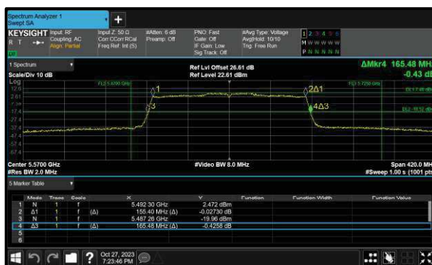
Figure 330 - 802.11ax HE160 SU Minimum 99% OBW
