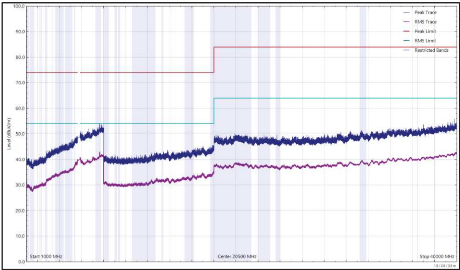
Figure 659 - U-NII-3 - 5745 MHz (CH149), 802.11a, Core 1, 1 GHz to 40 GHz, Horizontal
