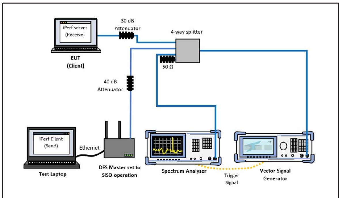
Figure 697 - Test Equipment Setup Diagram for Client without Radar Detection with Injection at the Master
