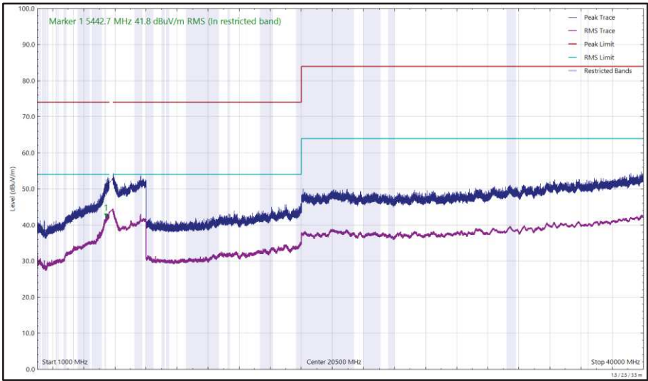
Figure 660 - U-NII-3 - 5745 MHz (CH149), 802.11a, Core 1, 1 GHz to 40 GHz, Vertical
