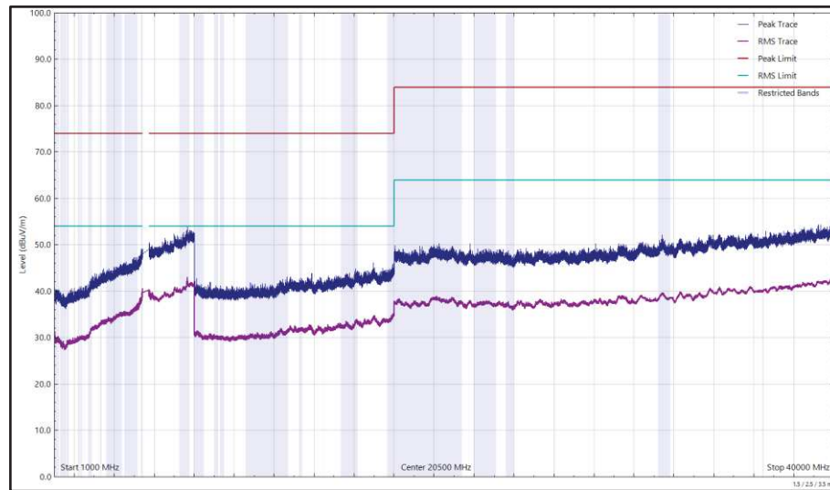
Figure 655 - U-NII-2C - 5500 MHz (CH100), 802.11a, Core 1, 1 GHz to 40 GHz, Horizontal
