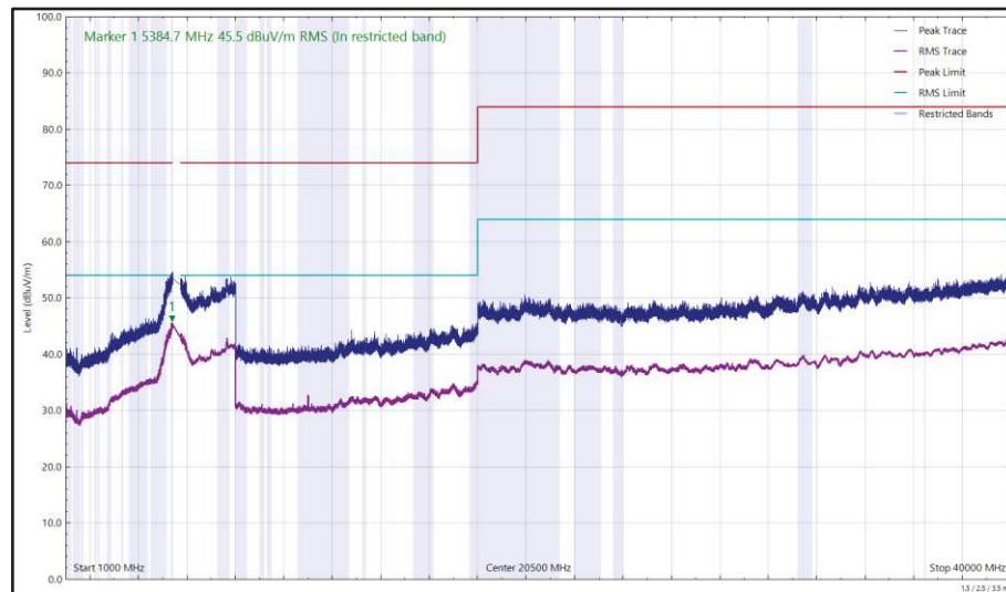
Figure 656 - U-NII-2C - 5500 MHz (CH100), 802.11a, Core 1, 1 GHz to 40 GHz, Vertical
