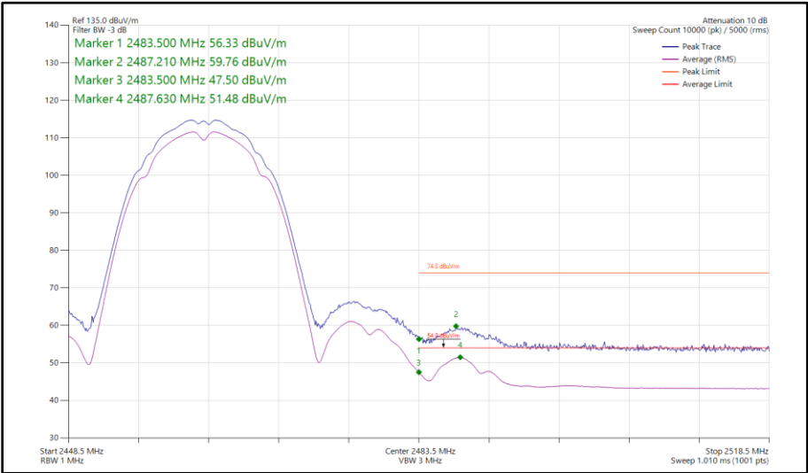
Figure 19 - 802.11b, SISO, Core 0 - 2462 MHz Band Edge Frequency 2483.5 MHz
