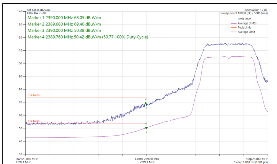
Figure 47 - 802.11g, SISO, Core 1 - 2417 MHz Band Edge Frequency 2390 MHz
