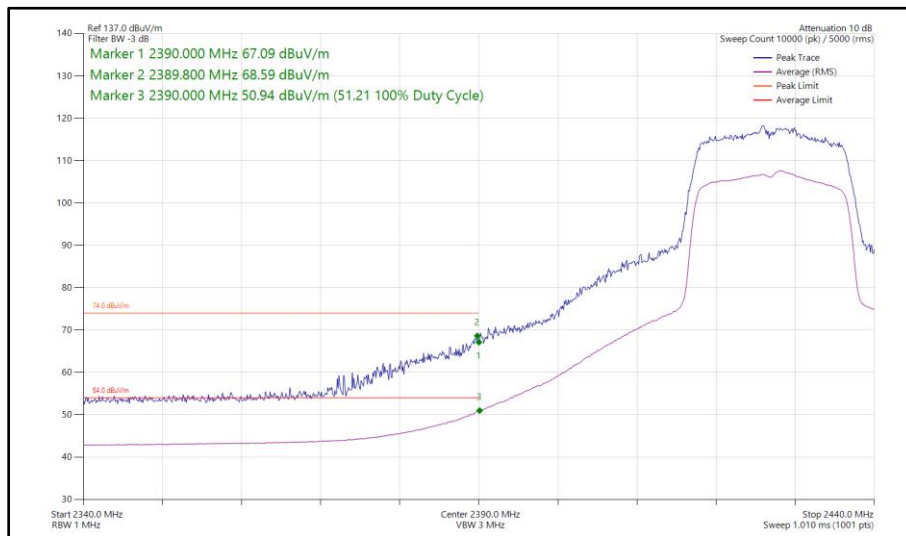
Figure 17 - 802.11ax HE20, SU, SISO, Core 0 - 2427 MHz Band Edge Frequency 2390 MHz
