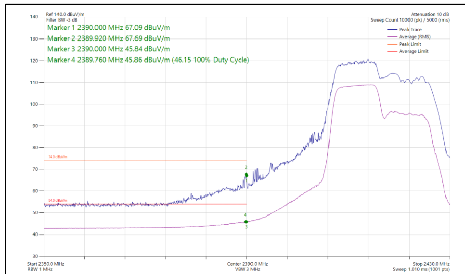
Figure 58 - 802.11ax HE20, RU 106-53, SISO, Core 1 - 2417 MHz Band Edge Frequency 2390 MHz
