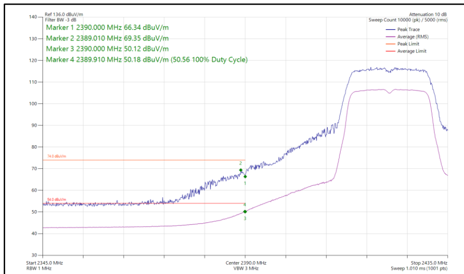
Figure 52 - 802.11n HT20, SISO, Core 1 - 2422 MHz Band Edge Frequency 2390 MHz
