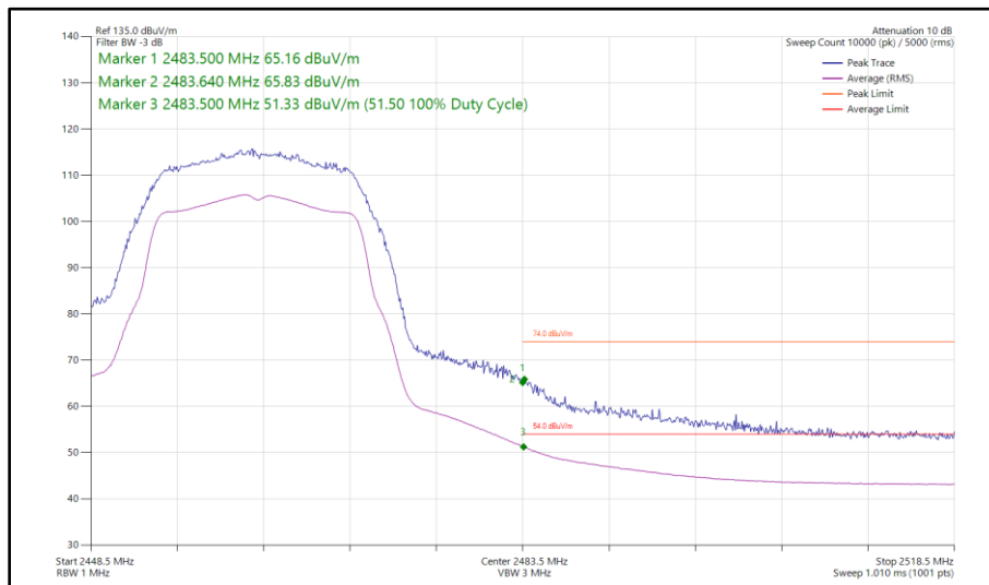
Figure 25 - 802.11g, SISO, Core 0 - 2462 MHz Band Edge Frequency 2483.5 MHz
