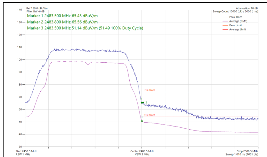
Figure 70 - 802.11g, SISO, Core 1 - 2472 MHz Band Edge Frequency 2483.5 MHz
