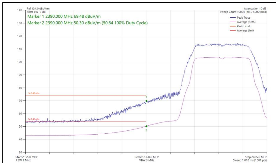
Figure 46 - 802.11g, SISO, Core 1 - 2412 MHz Band Edge Frequency 2390 MHz
