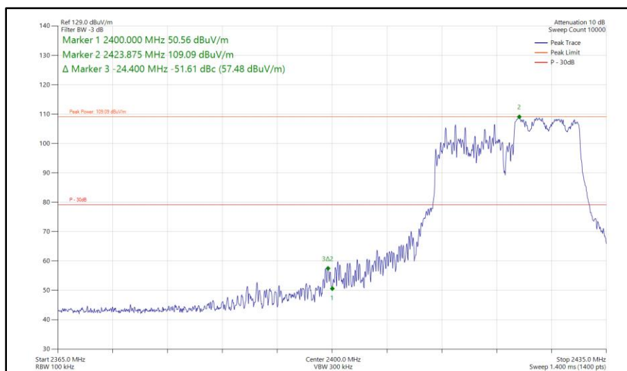
Figure 184 - 802.11ax HE20, RU 106-54, CDD, Core 0 - Core 1 - 2422 MHz Band Edge Frequency 2400 MHz
