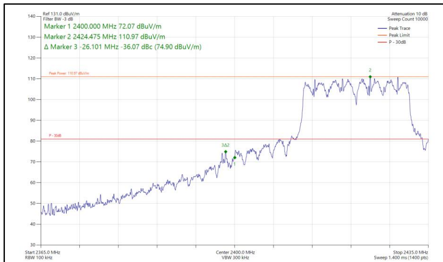
Figure 183 - 802.11ax HE20, SU, CDD, Core 0 - Core 1 - 2422 MHz Band Edge Frequency 2400 MHz
