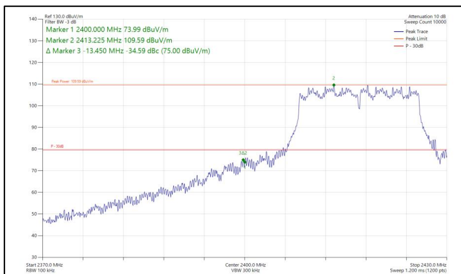
Figure 175 - 802.11n HT20, CDD, Core 0 - Core 1 - 2417 MHz Band Edge Frequency 2400 MHz
