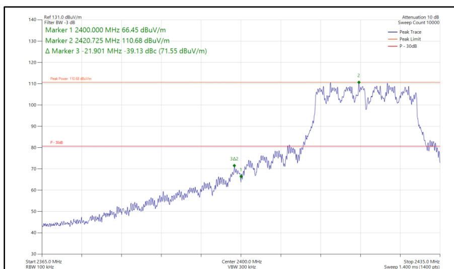
Figure 176 - 802.11n HT20, CDD, Core 0 - Core 1 - 2422 MHz Band Edge Frequency 2400 MHz
