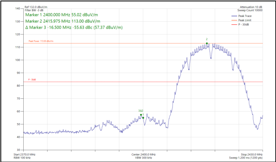
Figure 157 - 802.11b, SISO, Core 1 - 2417 MHz Band Edge Frequency 2400 MHz
