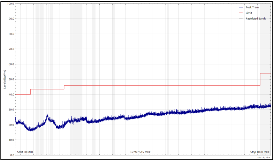
Figure 198 - 2442 MHz (CH7), 802.11b, Core 1, 30 MHz to 1 GHz, Horizontal (Peak)
