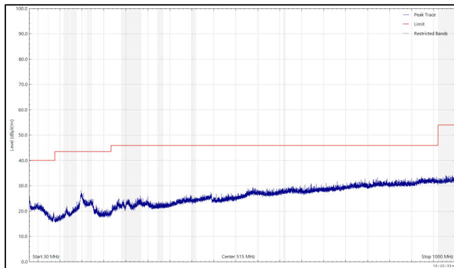
Figure 214 - 2442 MHz (CH7), 802.11g, Core 1, 30 MHz to 1 GHz, Horizontal (Peak)
