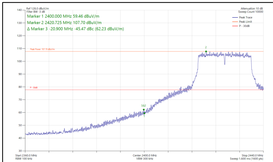
Figure 147 - 802.11n HT20, SISO, Core 0 - 2427 MHz Band Edge Frequency 2400 MHz
