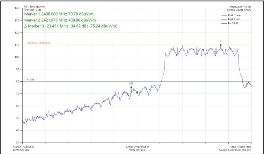
Figure 181 - 802.11ax HE20, SU, CDD, Core 0 - Core 1 - 2417 MHz Band Edge Frequency 2400 MHz
