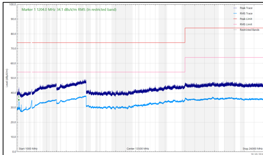
Figure 195 - 2472 MHz (CH13), 802.11b, Core 0, 1 GHz to 26 GHz, Vertical
