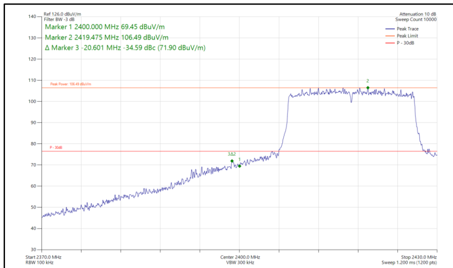
Figure 151 - 802.11ax HE20, SU, SISO, Core 0 - 2417 MHz Band Edge Frequency 2400 MHz
