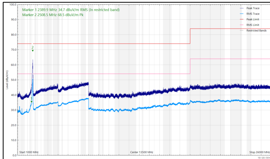
Figure 226 - 2472 MHz (CH13), HT20, CDD, Core 0 + Core 1, 1 GHz to 26 GHz, Horizontal
