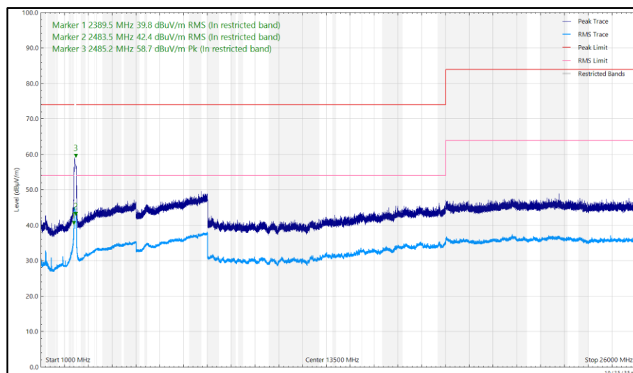
Figure 223 - 2442 MHz (CH7), HT20, CDD, Core 0 + Core 1, 1 GHz to 26 GHz, Horizontal
