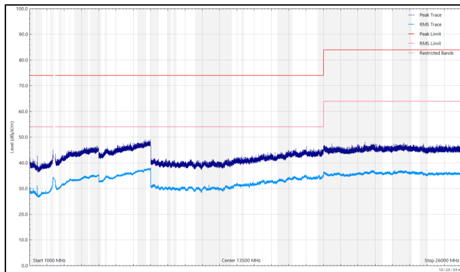
Figure 229 - 2412 MHz (CH1), HE20, RU26-0, CDD, Core 0 + Core 1, 1 GHz to 26 GHz, Vertical
