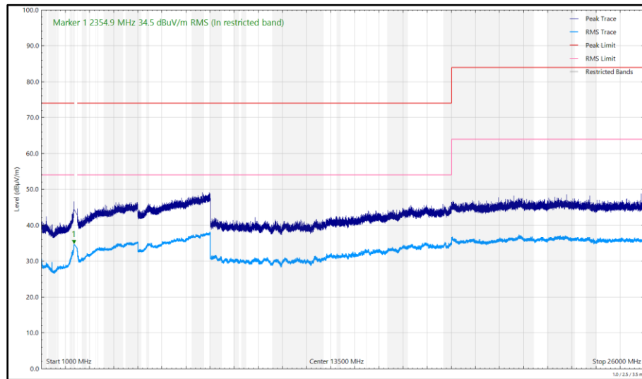
Figure 228 - 2412 MHz (CH1), HE20, RU26-0, CDD, Core 0 + Core 1, 1 GHz to 26 GHz, Horizontal
