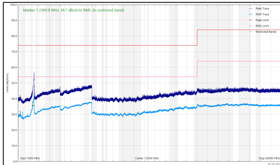
Figure 234 - 2472 MHz (CH13), HE20, RU26-0, CDD, Core 0 + Core 1, 1 GHz to 26 GHz, Horizontal
