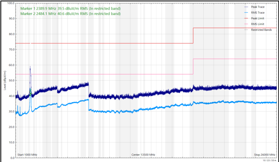
Figure 225 - 2442 MHz (CH7), HT20, CDD, Core 0 + Core 1, 1 GHz to 26 GHz, Vertical
