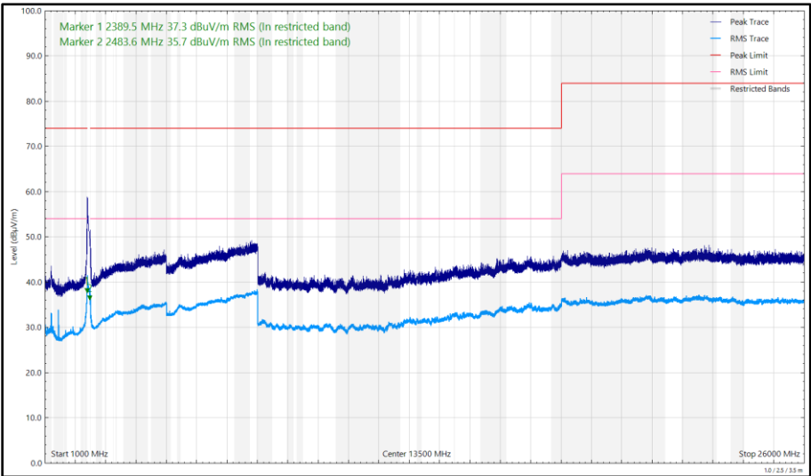
Figure 233 - 2442 MHz (CH7), HE20, RU26-0, CDD, Core 0 + Core 1, 1 GHz to 26 GHz, Vertical
