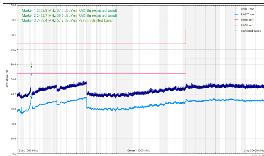
Figure 231 - 2442 MHz (CH7), HE20, RU26-0, CDD, Core 0 + Core 1, 1 GHz to 26 GHz, Horizontal
