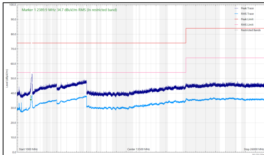
Figure 235 - 2472 MHz (CH13), HE20, RU26-0, CDD, Core 0 + Core 1, 1 GHz to 26 GHz, Vertical
