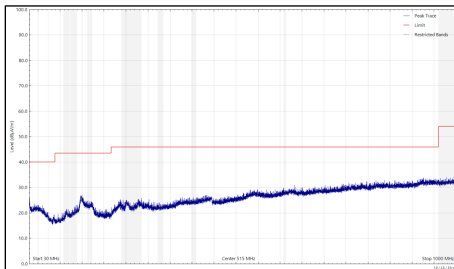
Figure 222 - 2442 MHz (CH7), HT20, CDD, Core 0 + Core 1, 30 MHz to 1 GHz, Horizontal (Peak)
