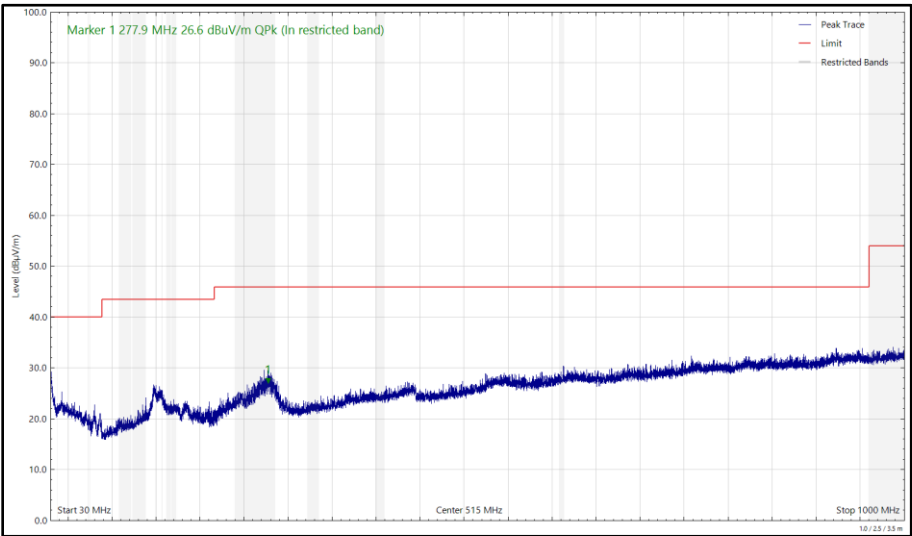
Figure 232 - 2442 MHz (CH7), HE20, RU26-0, CDD, Core 0 + Core 1, 30 MHz to 1 GHz, Vertical (Peak)
