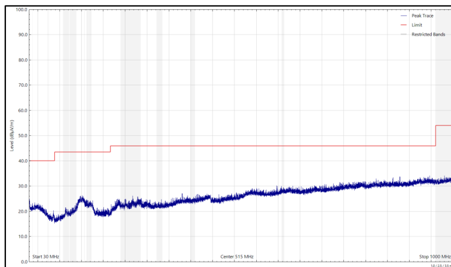
Figure 230 - 2442 MHz (CH7), HE20, RU26-0, CDD, Core 0 + Core 1, 30 MHz to 1 GHz, Horizontal (Peak)
