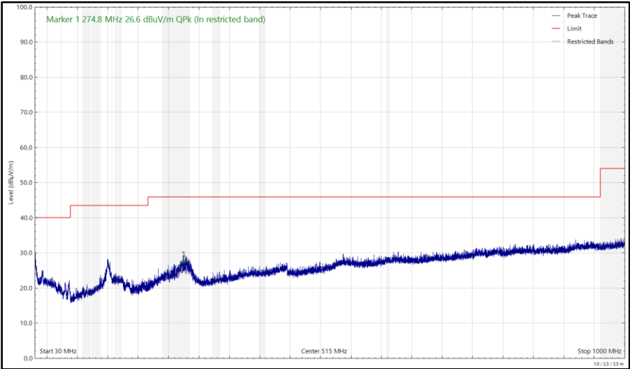
Figure 224 - 2442 MHz (CH7), HT20, CDD, Core 0 + Core 1, 30 MHz to 1 GHz, Vertical (Peak)
