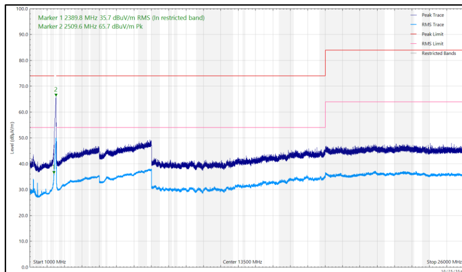
Figure 227 - 2472 MHz (CH13), HT20, CDD, Core 0 + Core 1, 1 GHz to 26 GHz, Vertical
