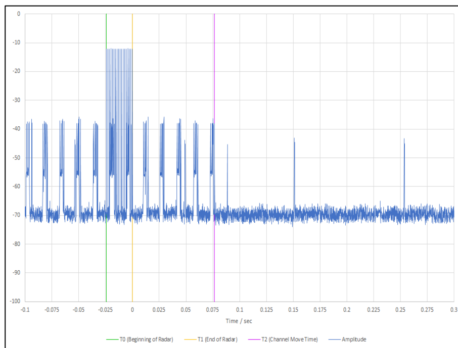
Figure 649 - First 200 ms of Channel Shutdown Period
