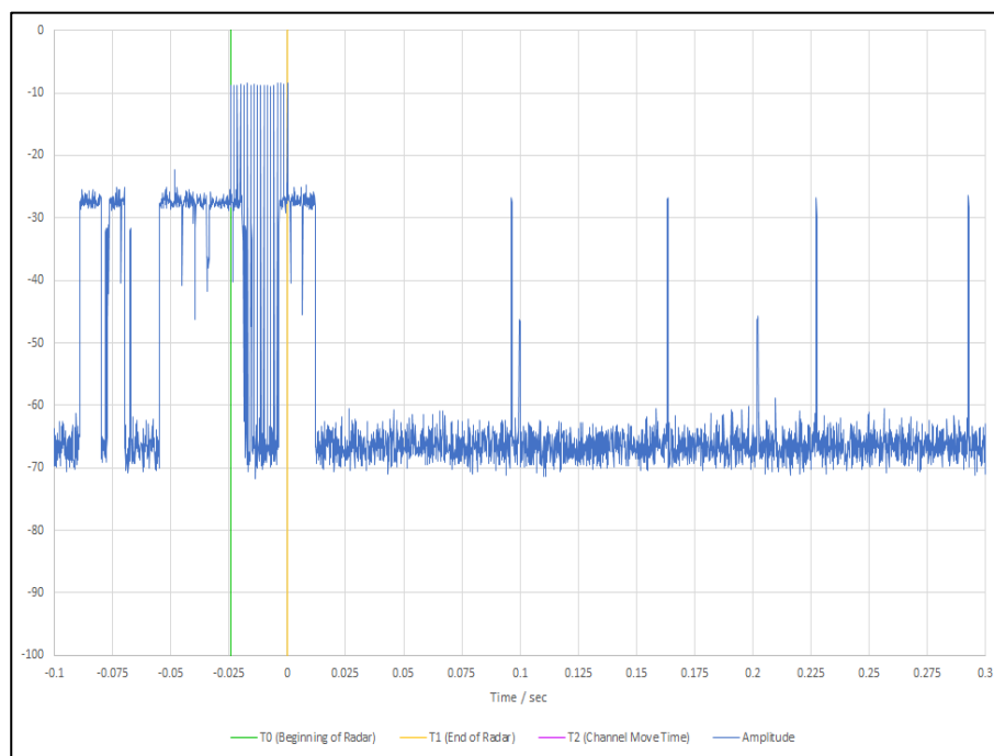
Figure 655 - First 200 ms of Channel Shutdown Period
