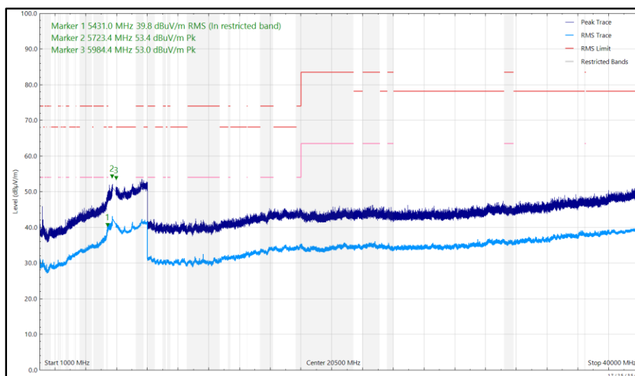
Figure 645 - U-NII-3 - 5825 MHz (CH165), HE20, RU26-0, CDD, Core 0 + Core 1, 1 GHz to 40 GHz, Vertical
