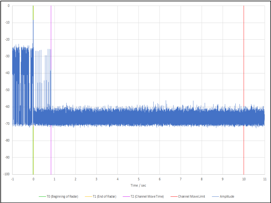
Figure 656 - First 12 s of Channel Shutdown Period
