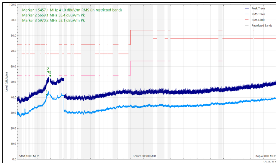
Figure 643 - U-NII-3 - 5825 MHz (CH165), HE20, RU26-0, CDD, Core 0 + Core 1, 1 GHz to 40 GHz, Horizontal
