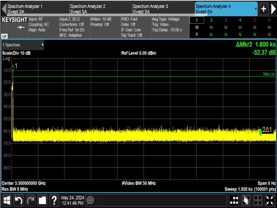
Figure 651 - 30 minute Non-Occupancy Period
