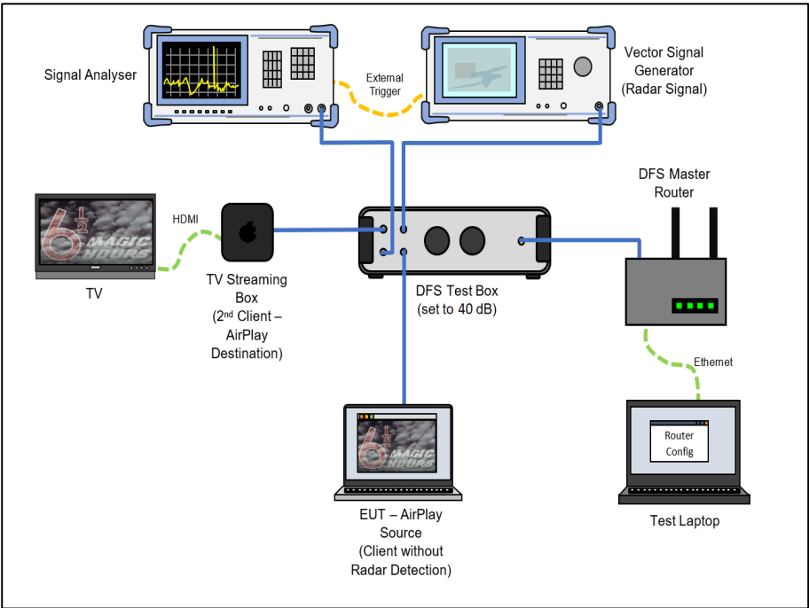
Figure 652- Test Equipment Setup Diagram for Client without Radar Detection with Injection at the Master
