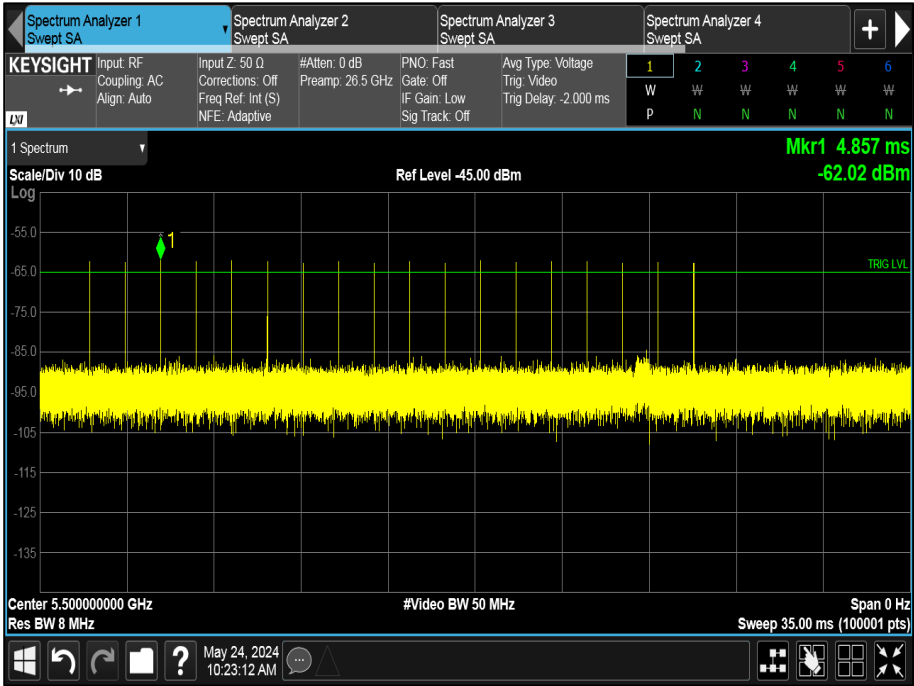
Figure 653- Verification of Radar Type 0
