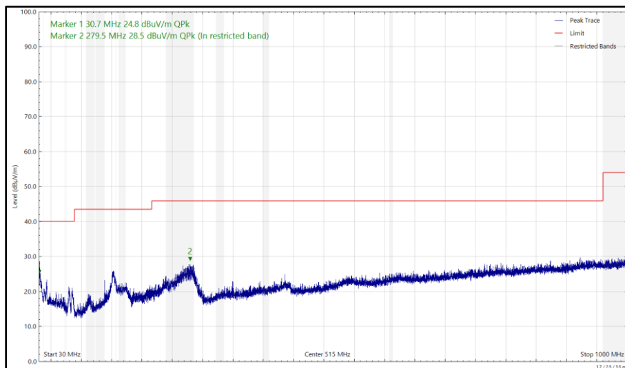
Figure 644 - U-NII-3 - 5825 MHz (CH165), HE20, RU26-0, CDD, Core 0 + Core 1, 30 MHz to 1 GHz, Vertical (Peak)
