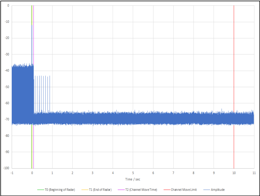
Figure 650 - First 12 s of Channel Shutdown Period
