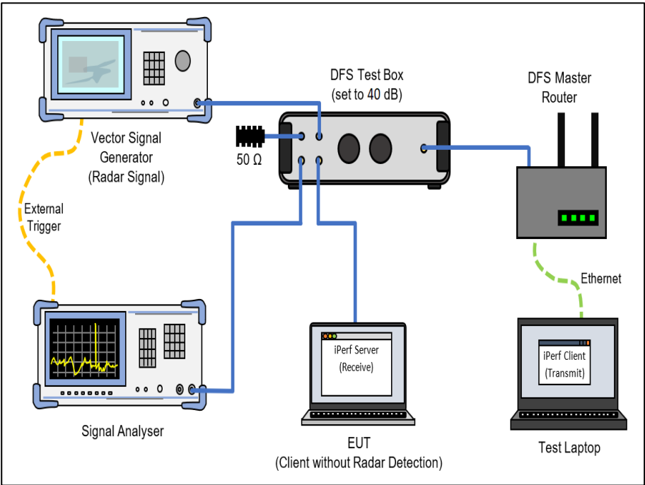
Figure 646- Test Equipment Setup Diagram for Client without Radar Detection with Injection at the Master
