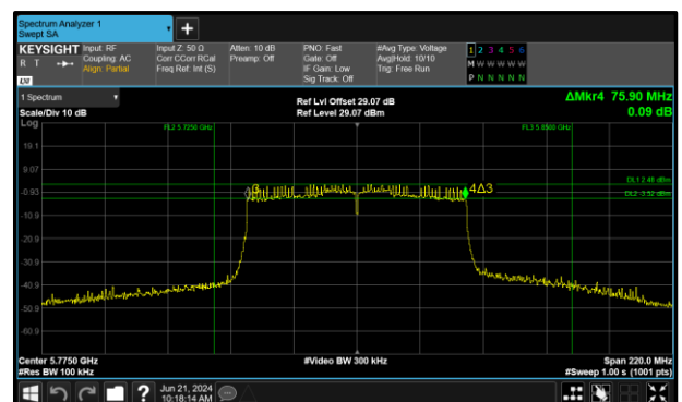
Figure 252 - 802.11ac VHT80 Maximum 6 dB EBW
