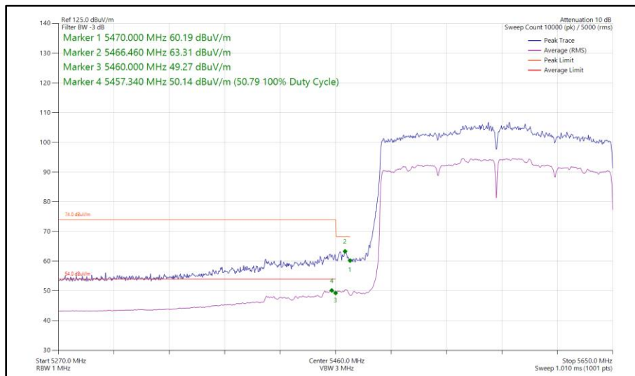
Figure 213 - 802.11ax HE160, SU, SDM, Core 0 - Core 1 - 5570 MHz Band Edge Frequency 5460 MHz
