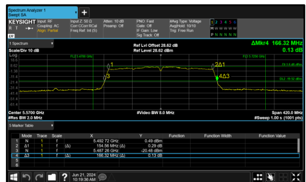
Figure 266 - 802.11ac VHT160 Maximum 99% OBW
