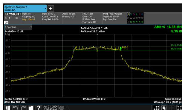
Figure 216 - 802.11a Maximum 6 dB EBW
