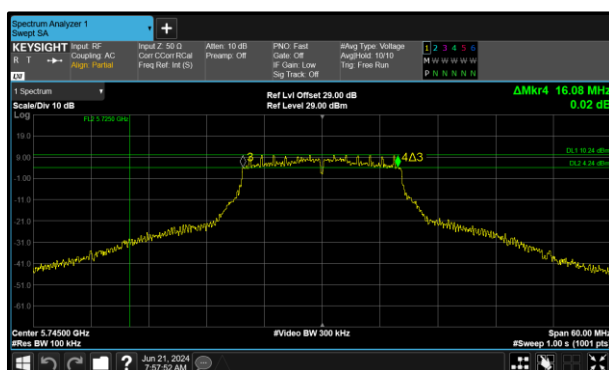
Figure 215 - 802.11a Minimum 6 dB EBW
