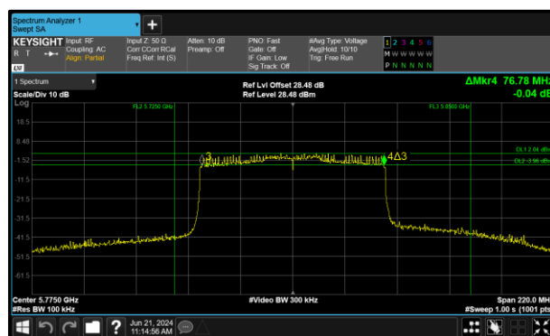
Figure 258 - 802.11ax HE80 SU Maximum 6 dB EBW
