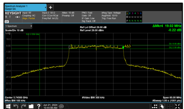
Figure 254 - 802.11ax HE20 SU Maximum 6 dB EBW
