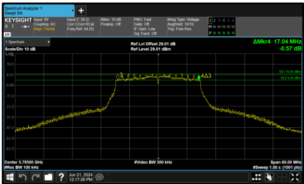
Figure 275 - 802.11n HT20 Minimum 6 dB EBW
