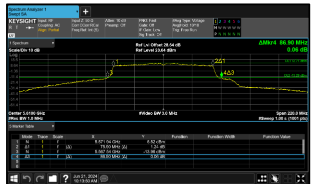
Figure 264 - 802.11ac VHT80 Maximum 99% OBW
