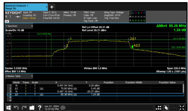
Figure 292 - 802.11ac VHT80 Maximum 99% OBW
