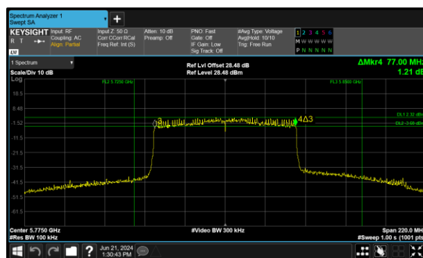
Figure 286 - 802.11ax HE80 SU Maximum 6 dB EBW
