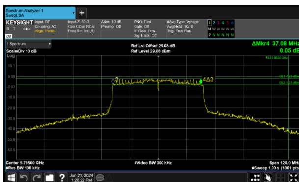
Figure 283 - 802.11ax HE40 SU Minimum 6 dB EBW
