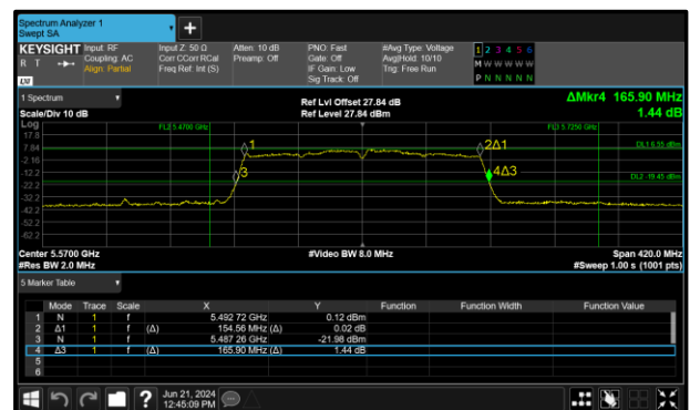
Figure 294 - 802.11ac VHT160 Maximum 99% OBW
