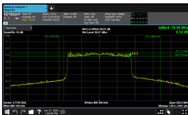
Figure 285 - 802.11ax HE80 SU Minimum 6 dB EBW
