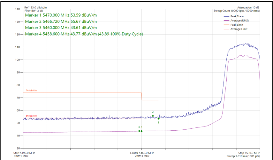
Figure 318 - 802.11n HT20, SISO, Core 0 - 5520 MHz Band Edge Frequency 5470 MHz
