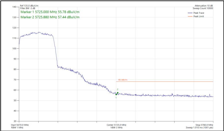
Figure 331 - 802.11ax HE20, SU, SISO, Core 0 - 5680 MHz Band Edge Frequency 5725 MHz
