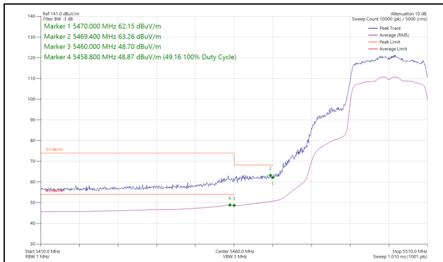
Figure 387 - 802.11ax HE20, SU, SDM, Core 0 - Core 1 - 5500 MHz Band Edge Frequency 5470 MHz
