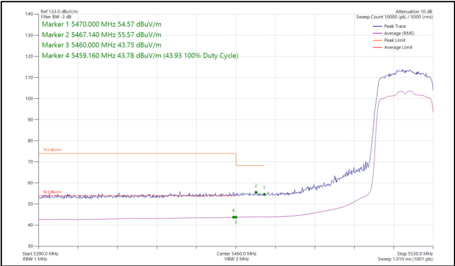
Figure 321 - 802.11ax HE20, SU, SISO, Core 0 - 5520 MHz Band Edge Frequency 5470 MHz
