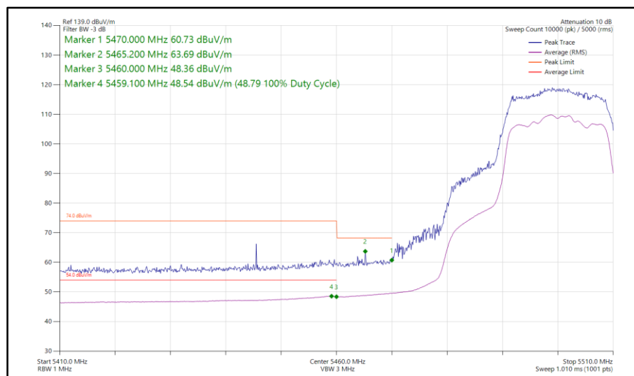
Figure 401 - 802.11ac VHT20, TxBF, Core 0 - Core 1 - 5500 MHz Band Edge Frequency 5470 MHz
