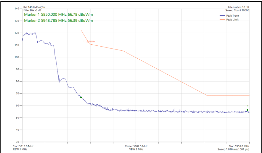
Figure 400 - 802.11ax HE20, RU 106-53, SDM, Core 0 - Core 1 - 5825 MHz Band Edge Frequency 5850 MHz
