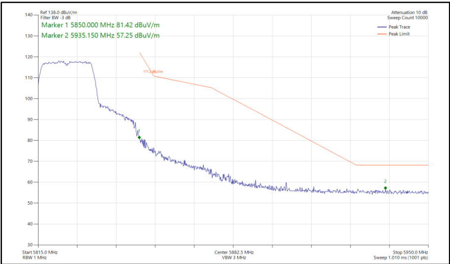
Figure 366 - 802.11n HT20, SISO, Core 1 - 5825 MHz Band Edge Frequency 5850 MHz
