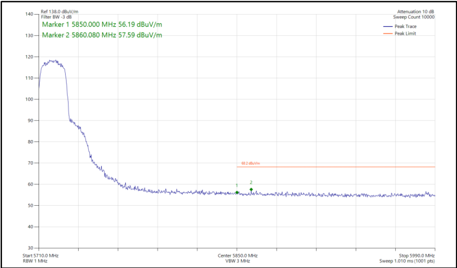
Figure 365 - 802.11n HT20, SISO, Core 1 - 5720 MHz Band Edge Frequency 5850 MHz
