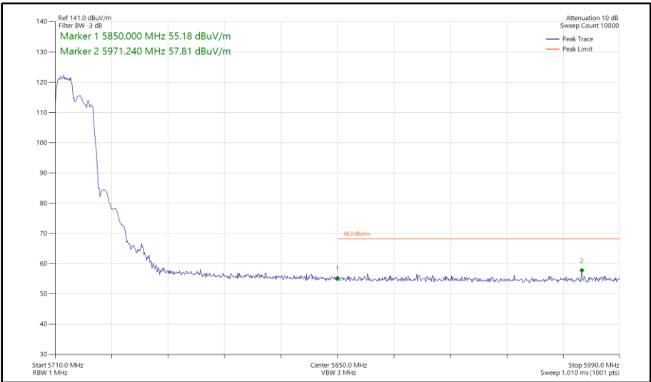
Figure 383 - 802.11ax HE20, RU 106-53, CDD, Core 0 - Core 1 - 5720 MHz Band Edge Frequency 5850 MHz
