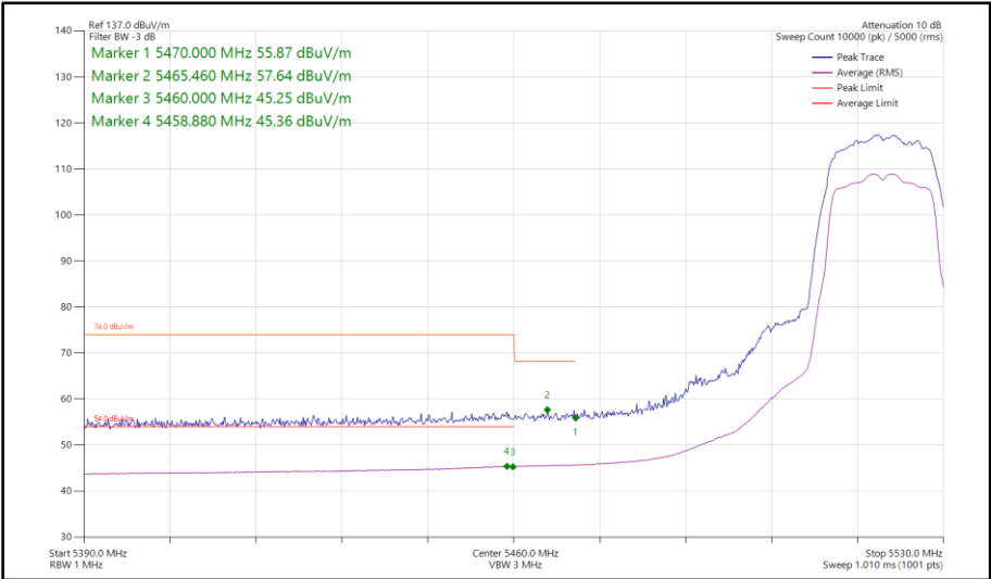
Figure 344 - 802.11a, SISO, Core 1 - 5520 MHz Band Edge Frequency 5470 MHz
