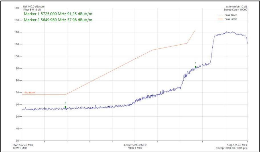
Figure 353 - 802.11ax HE20, SU, SISO, Core 1 - 5745 MHz Band Edge Frequency 5725 MHz
