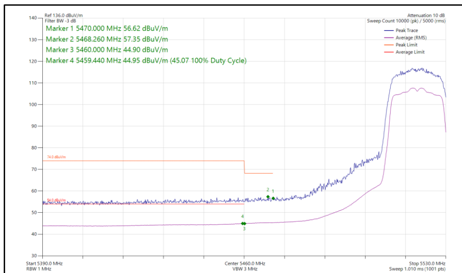
Figure 346 - 802.11n HT20, SISO, Core 1 - 5520 MHz Band Edge Frequency 5470 MHz
