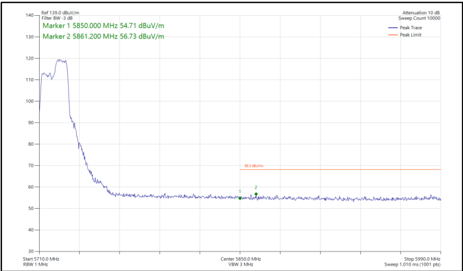
Figure 398 - 802.11ax HE20, RU 106-54, SDM, Core 0 - Core 1 - 5720 MHz Band Edge Frequency 5850 MHz
