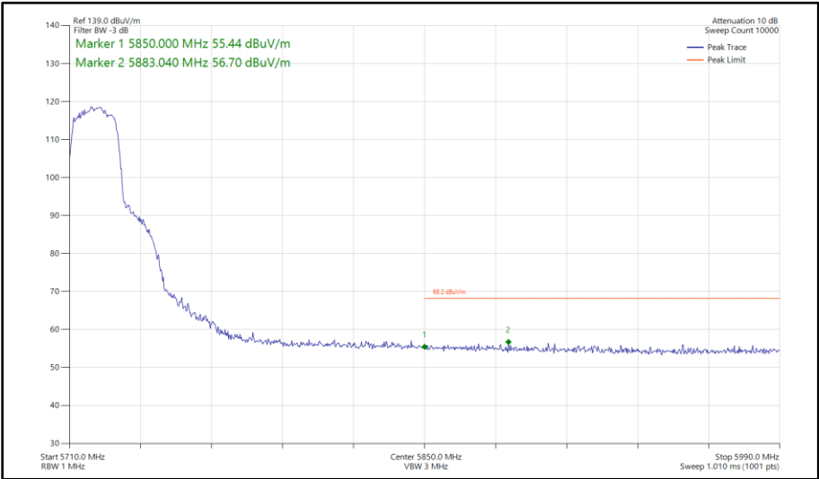
Figure 395 - 802.11n HT20, SDM, Core 0 - Core 1 - 5720 MHz Band Edge Frequency 5850 MHz
