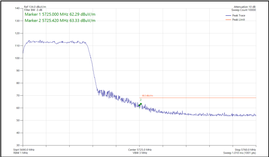
Figure 393 - 802.11ax HE20, SU, SDM, Core 0 - Core 1 - 5700 MHz Band Edge Frequency 5725 MHz
