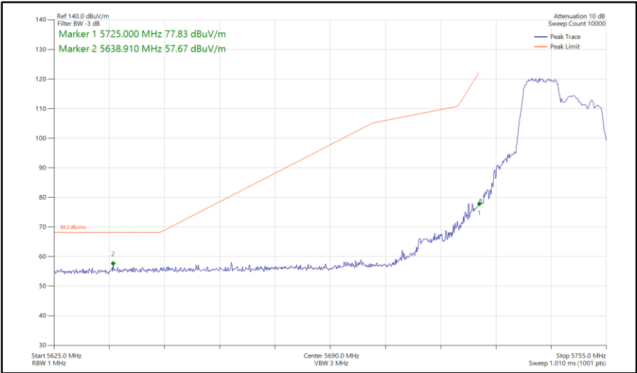
Figure 376 - 802.11ax HE20, RU 106-53, CDD, Core 0 - Core 1 - 5745 MHz Band Edge Frequency 5725 MHz
