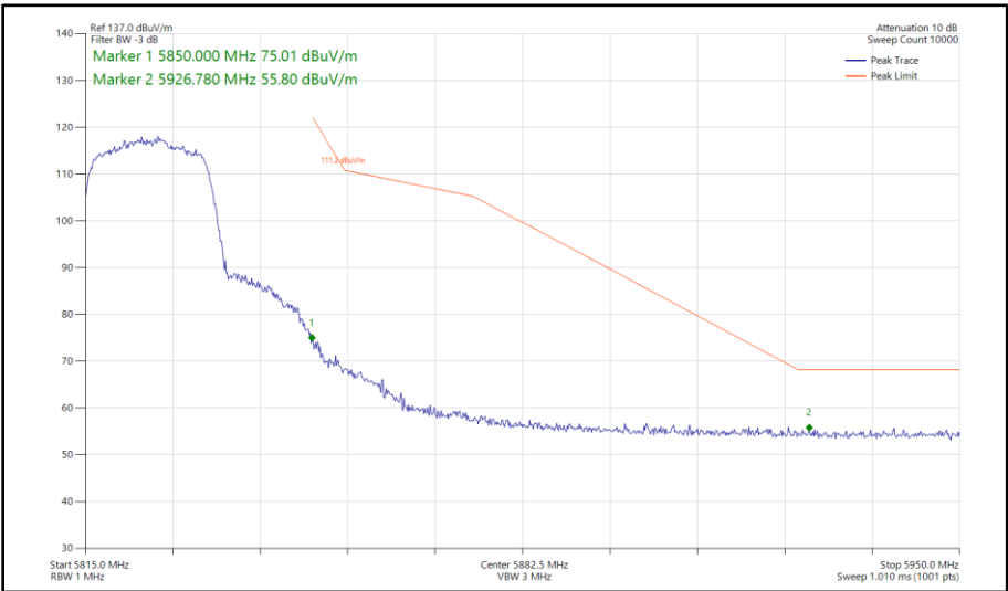
Figure 338 - 802.11n HT20, SISO, Core 0 - 5825 MHz Band Edge Frequency 5850 MHz
