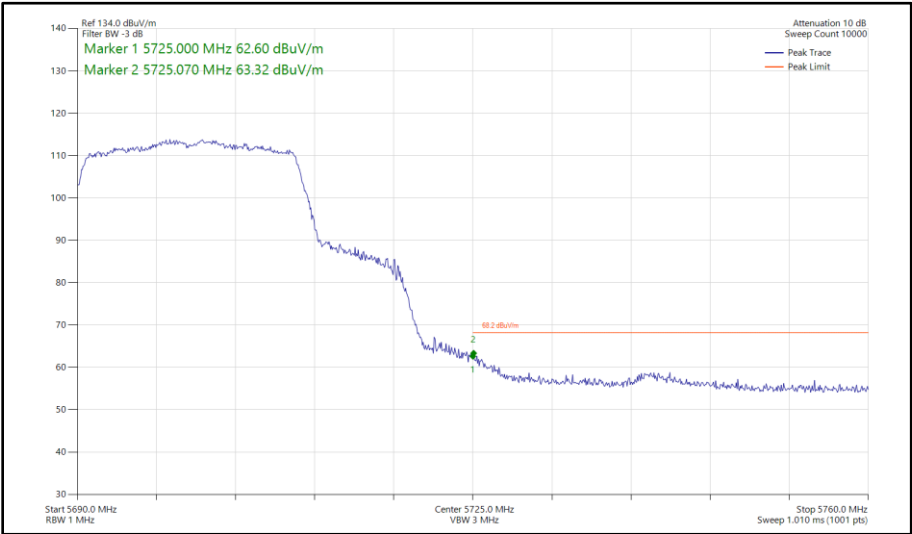
Figure 333 - 802.11ax HE20, SU, SISO, Core 0 - 5700 MHz Band Edge Frequency 5725 MHz
