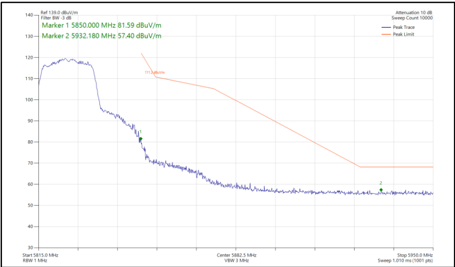
Figure 381 - 802.11n HT20, CDD, Core 0 - Core 1 - 5825 MHz Band Edge Frequency 5850 MHz
