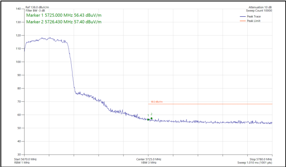
Figure 359 - 802.11ax HE20, SU, SISO, Core 1 - 5680 MHz Band Edge Frequency 5725 MHz
