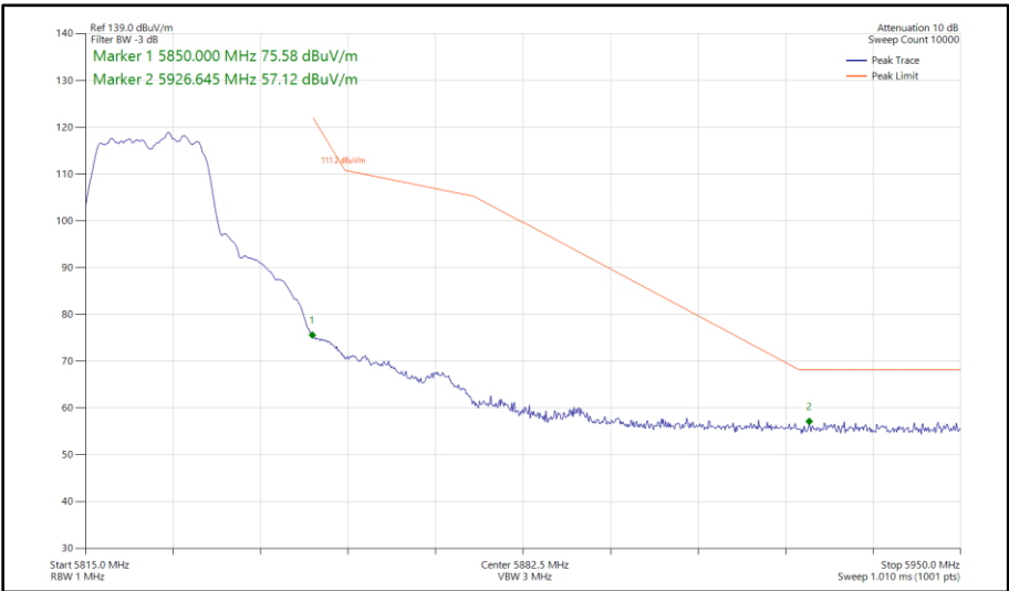
Figure 364 - 802.11a, SISO, Core 1 - 5825 MHz Band Edge Frequency 5850 MHz
