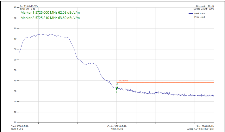
Figure 328 - 802.11a, SISO, Core 0 - 5700 MHz Band Edge Frequency 5725 MHz
