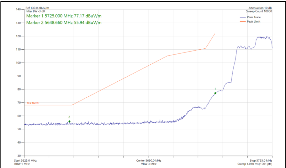
Figure 326 - 802.11ax HE20, RU 106-54, SISO, Core 0 - 5745 MHz Band Edge Frequency 5725 MHz
