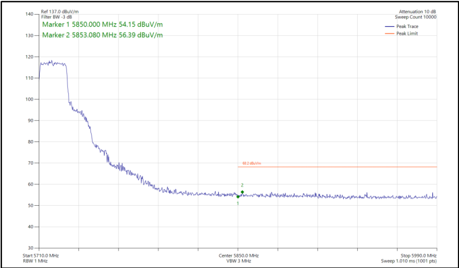
Figure 339 - 802.11ax HE20, SU, SISO, Core 0 - 5720 MHz Band Edge Frequency 5850 MHz
