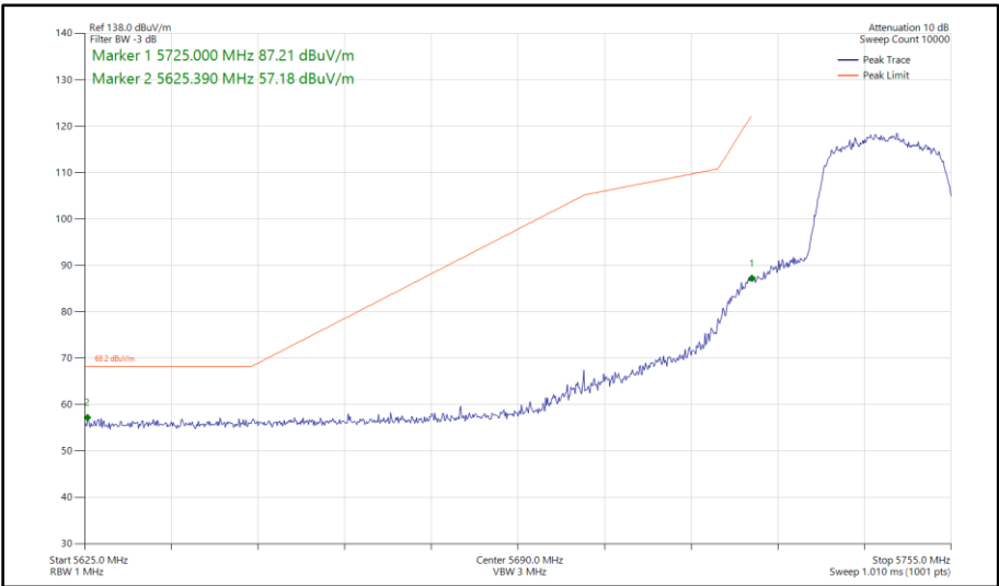
Figure 352 - 802.11n HT20, SISO, Core 1 - 5745 MHz Band Edge Frequency 5725 MHz
