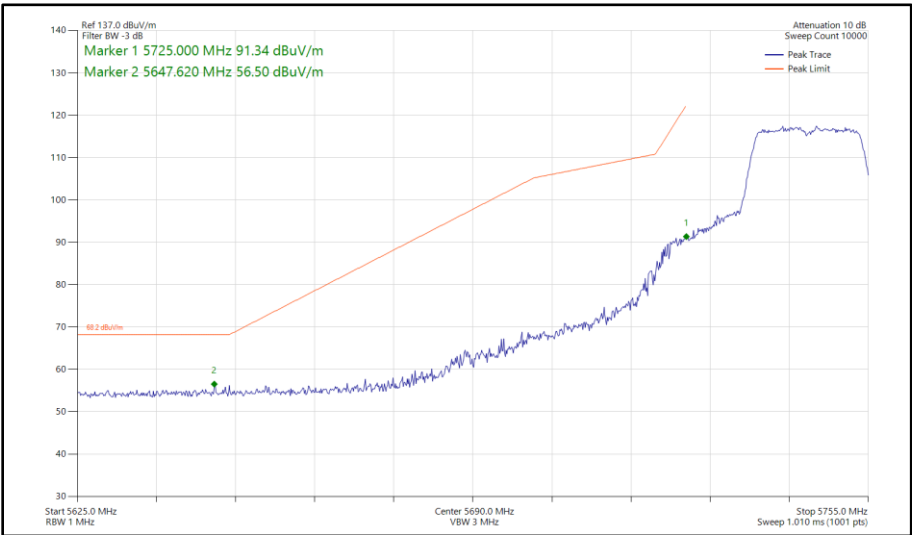
Figure 324 - 802.11n HT20, SISO, Core 0 - 5745 MHz Band Edge Frequency 5725 MHz
