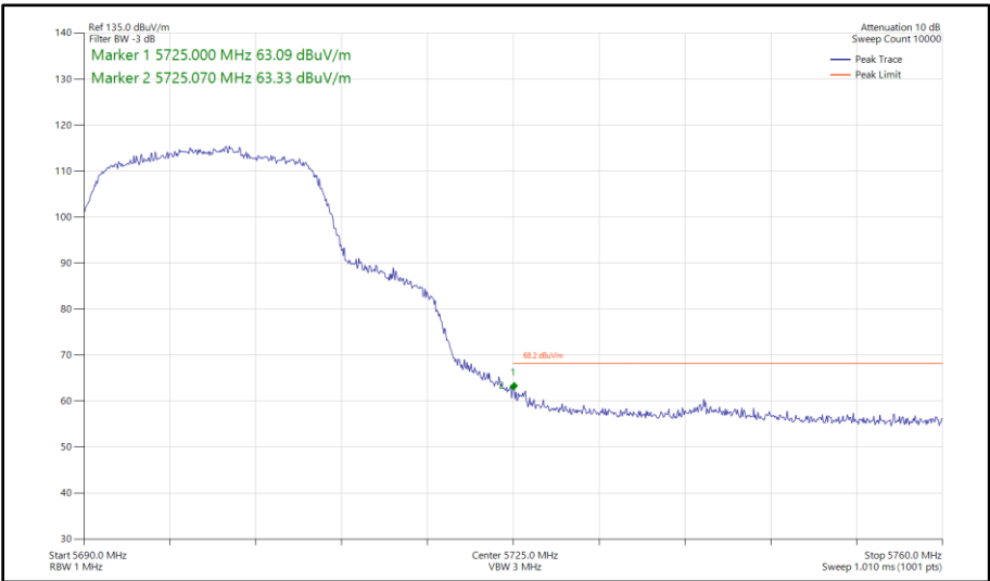
Figure 330 - 802.11n HT20, SISO, Core 0 - 5700 MHz Band Edge Frequency 5725 MHz
