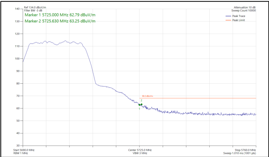
Figure 356 - 802.11a, SISO, Core 1 - 5700 MHz Band Edge Frequency 5725 MHz
