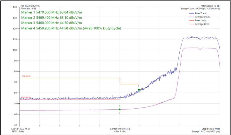
Figure 317 - 802.11n HT20, SISO, Core 0 - 5500 MHz Band Edge Frequency 5470 MHz
