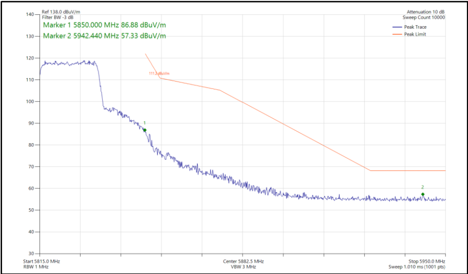
Figure 399 - 802.11ax HE20, SU, SDM, Core 0 - Core 1 - 5825 MHz Band Edge Frequency 5850 MHz
