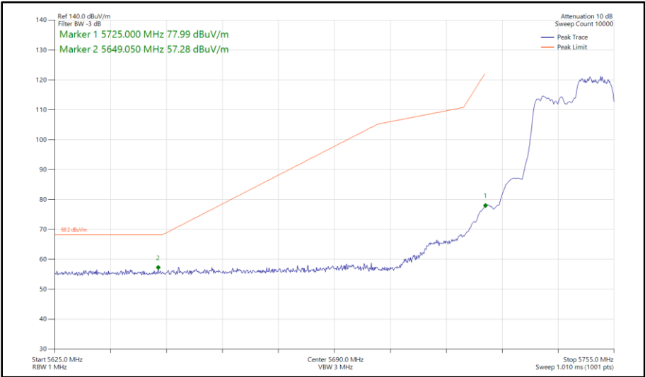
Figure 391 - 802.11ax HE20, RU 106-54, SDM, Core 0 - Core 1 - 5745 MHz Band Edge Frequency 5725 MHz
