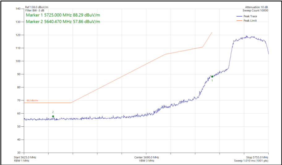
Figure 374 - 802.11n HT20, CDD, Core 0 - Core 1 - 5745 MHz Band Edge Frequency 5725 MHz
