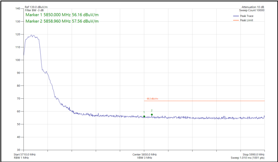
Figure 363 - 802.11a, SISO, Core 1 - 5720 MHz Band Edge Frequency 5850 MHz
