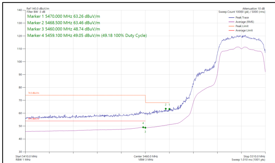
Figure 345 - 802.11n HT20, SISO, Core 1 - 5500 MHz Band Edge Frequency 5470 MHz
