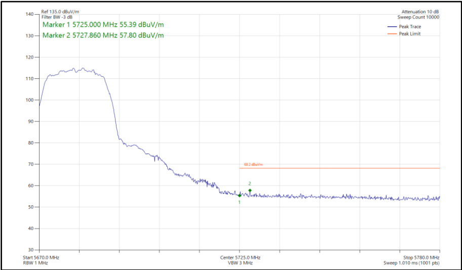
Figure 327 - 802.11a, SISO, Core 0 - 5680 MHz Band Edge Frequency 5725 MHz
