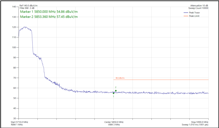
Figure 382 - 802.11ax HE20, SU, CDD, Core 0 - Core 1 - 5720 MHz Band Edge Frequency 5850 MHz
