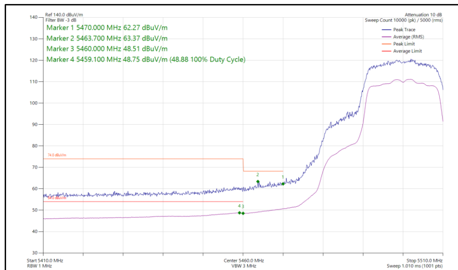
Figure 386 - 802.11n HT20, SDM, Core 0 - Core 1 - 5500 MHz Band Edge Frequency 5470 MHz
