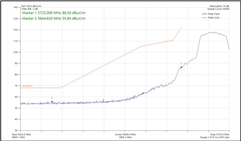
Figure 323 - 802.11a, SISO, Core 0 - 5745 MHz Band Edge Frequency 5725 MHz
