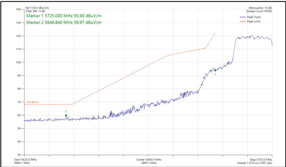
Figure 375 - 802.11ax HE20, SU, CDD, Core 0 - Core 1 - 5745 MHz Band Edge Frequency 5725 MHz
