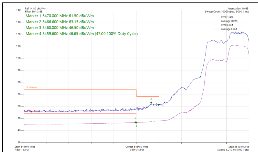
Figure 373 - 802.11ax HE20, RU 106-54, CDD, Core 0 - Core 1 - 5500 MHz Band Edge Frequency 5470 MHz
