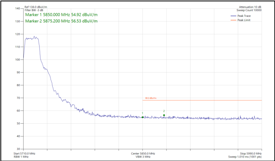
Figure 335 - 802.11a, SISO, Core 0 - 5720 MHz Band Edge Frequency 5850 MHz
