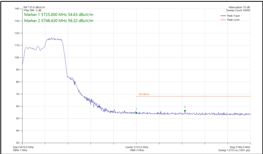
Figure 332 - 802.11ax HE20, RU 106-54, SISO, Core 0 - 5680 MHz Band Edge Frequency 5725 MHz
