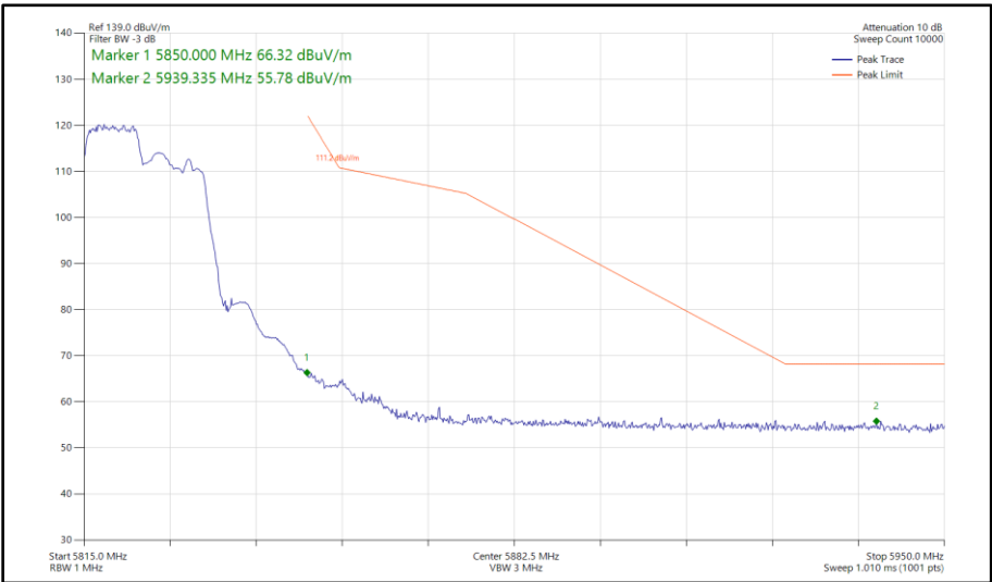
Figure 370 - 802.11ax HE20, RU 106-53, SISO, Core 1 - 5825 MHz Band Edge Frequency 5850 MHz
