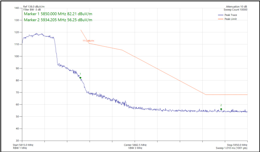
Figure 341 - 802.11ax HE20, SU, SISO, Core 0 - 5825 MHz Band Edge Frequency 5850 MHz
