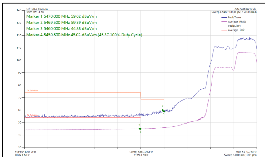
Figure 320 - 802.11ax HE20, RU 106-54, SISO, Core 0 - 5500 MHz Band Edge Frequency 5470 MHz
