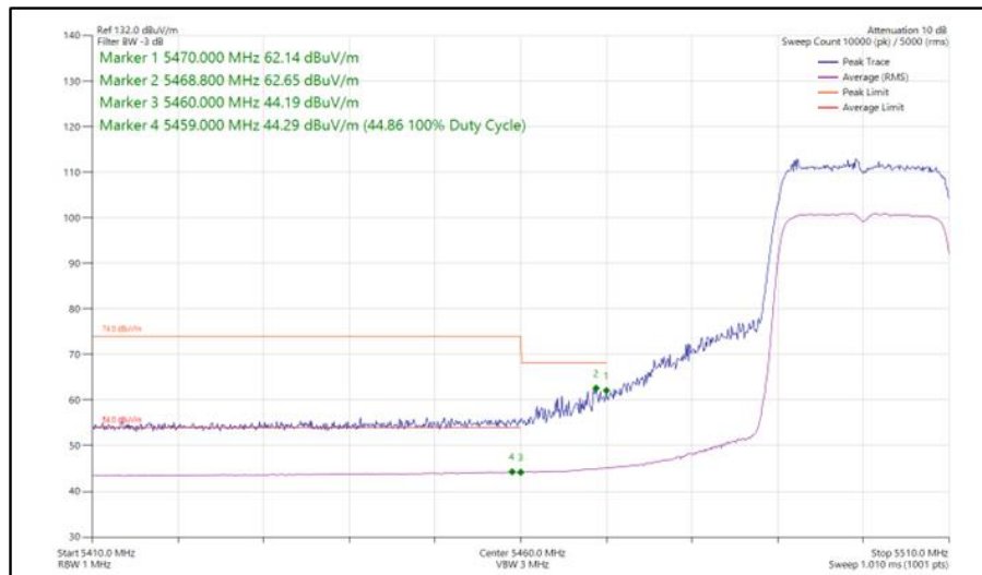
Figure 319 - 802.11ax HE20, SU, SISO, Core 0 - 5500 MHz Band Edge Frequency 5470 MHz
