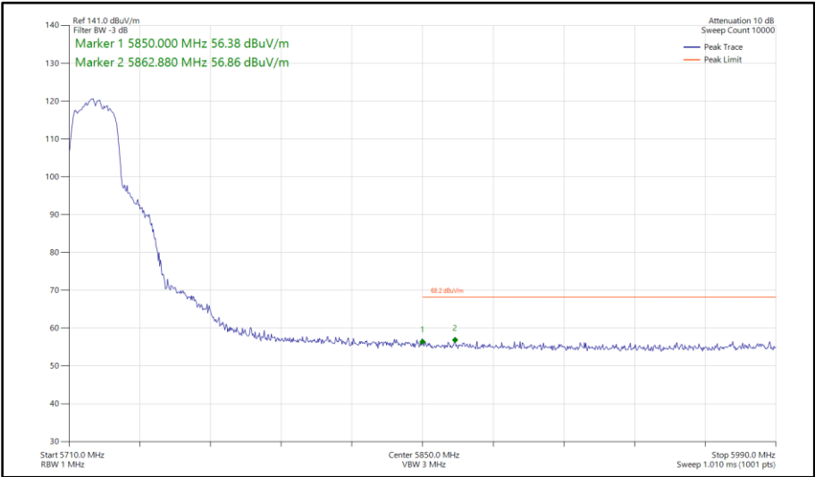
Figure 380 - 802.11n HT20, CDD, Core 0 - Core 1 - 5720 MHz Band Edge Frequency 5850 MHz
