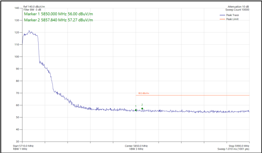
Figure 367 - 802.11ax HE20, SU, SISO, Core 1 - 5720 MHz Band Edge Frequency 5850 MHz
