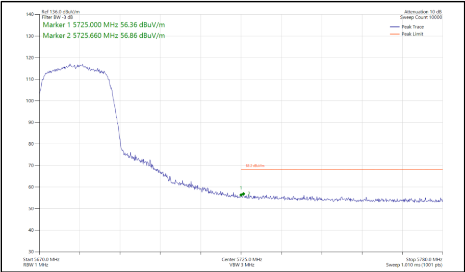
Figure 357 - 802.11n HT20, SISO, Core 1 - 5680 MHz Band Edge Frequency 5725 MHz
