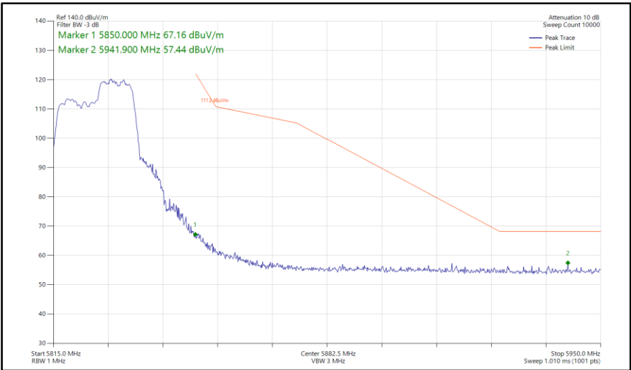
Figure 385 - 802.11ax HE20, RU 106-54, CDD, Core 0 - Core 1 - 5825 MHz Band Edge Frequency 5850 MHz
