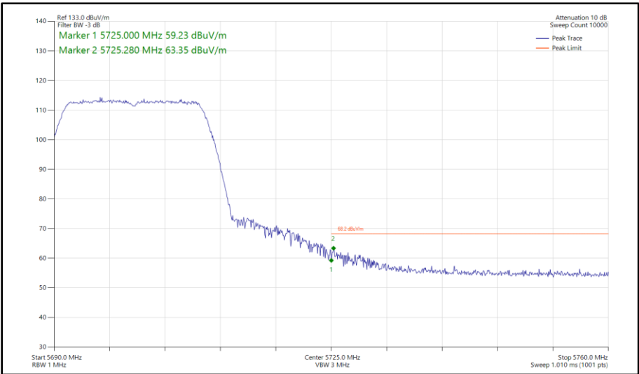
Figure 358 - 802.11n HT20, SISO, Core 1 - 5700 MHz Band Edge Frequency 5725 MHz
