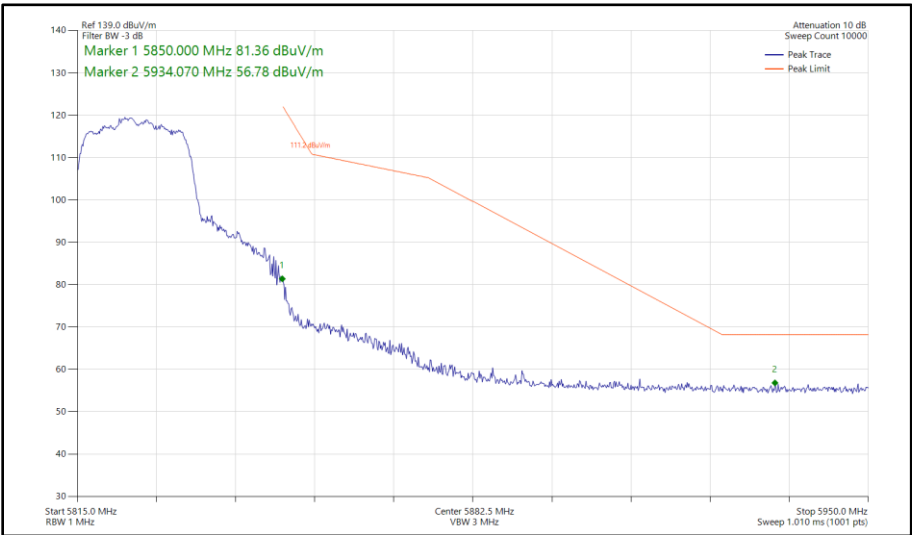
Figure 396 - 802.11n HT20, SDM, Core 0 - Core 1 - 5825 MHz Band Edge Frequency 5850 MHz
