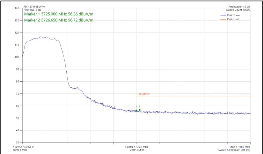
Figure 355 - 802.11a, SISO, Core 1 - 5680 MHz Band Edge Frequency 5725 MHz
