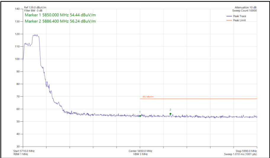
Figure 340 - 802.11ax HE20, RU 106-54, SISO, Core 0 - 5720 MHz Band Edge Frequency 5850 MHz
