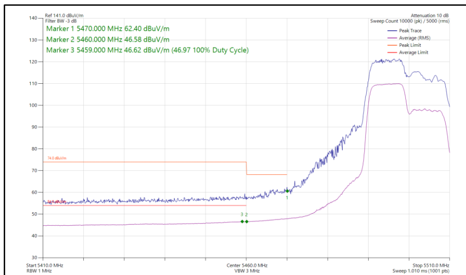
Figure 388 - 802.11ax HE20, RU 106-53, SDM, Core 0 - Core 1 - 5500 MHz Band Edge Frequency 5470 MHz
