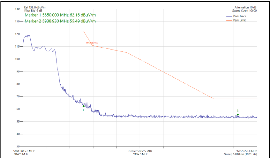
Figure 342 - 802.11ax HE20, RU 52-37, SISO, Core 0 - 5825 MHz Band Edge Frequency 5850 MHz
