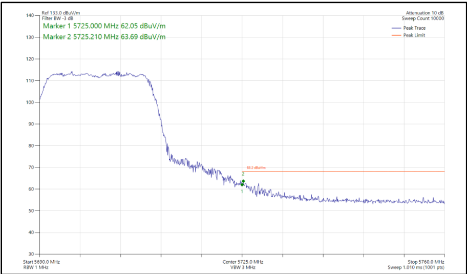
Figure 392 - 802.11n HT20, SDM, Core 0 - Core 1 - 5700 MHz Band Edge Frequency 5725 MHz
