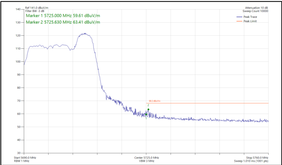
Figure 394 - 802.11ax HE20, RU 52-40, SDM, Core 0 - Core 1 - 5700 MHz Band Edge Frequency 5725 MHz
