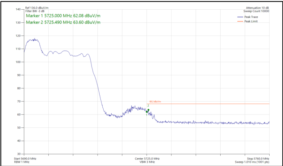
Figure 362 - 802.11ax HE20, RU 52-37, SISO, Core 1 - 5700 MHz Band Edge Frequency 5725 MHz
