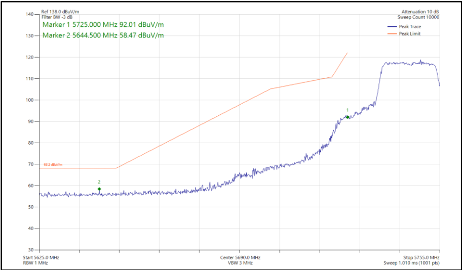
Figure 389 - 802.11n HT20, SDM, Core 0 - Core 1 - 5745 MHz Band Edge Frequency 5725 MHz
