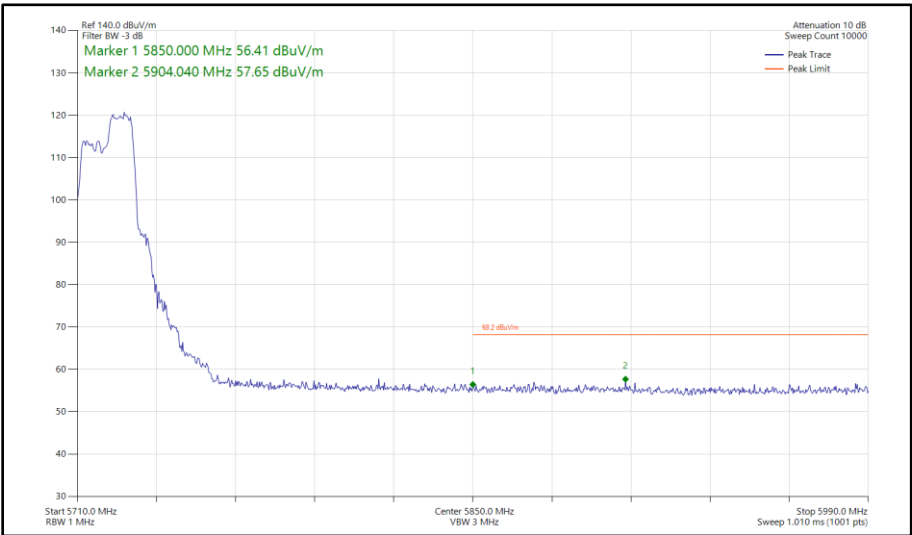
Figure 368 - 802.11ax HE20, RU 106-54, SISO, Core 1 - 5720 MHz Band Edge Frequency 5850 MHz
