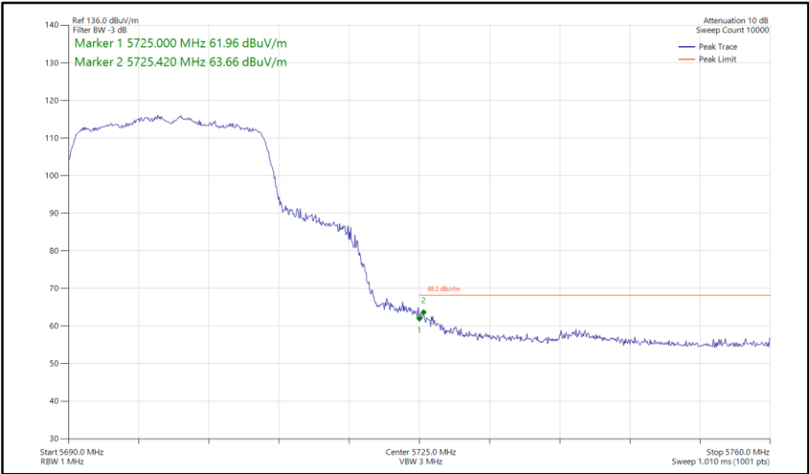
Figure 378 - 802.11ax HE20, SU, CDD, Core 0 - Core 1 - 5700 MHz Band Edge Frequency 5725 MHz
