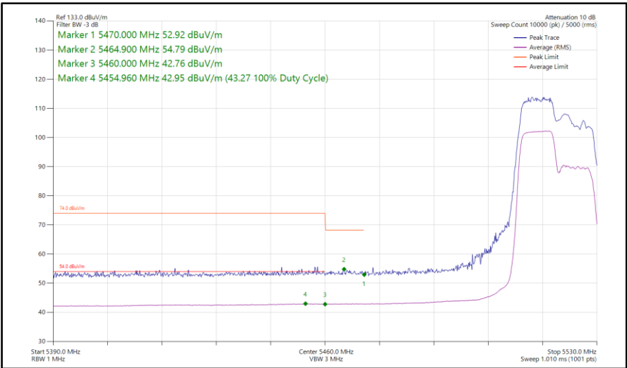
Figure 322 - 802.11ax HE20, RU 106-53, SISO, Core 0 - 5520 MHz Band Edge Frequency 5470 MHz
