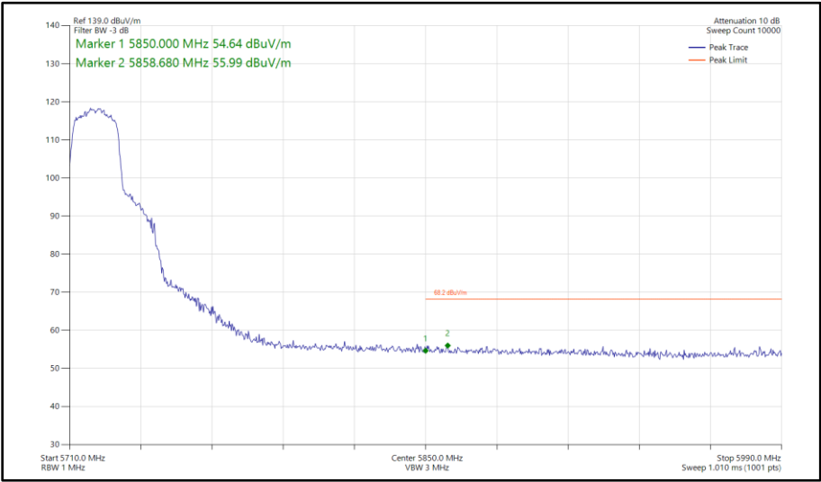
Figure 337 - 802.11n HT20, SISO, Core 0 - 5720 MHz Band Edge Frequency 5850 MHz
