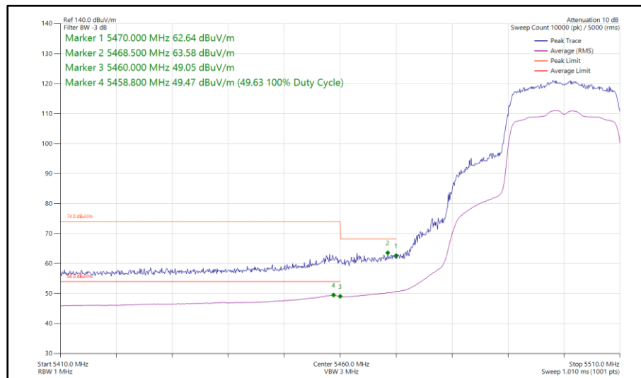
Figure 347 - 802.11ax HE20, SU, SISO, Core 1 - 5500 MHz Band Edge Frequency 5470 MHz
