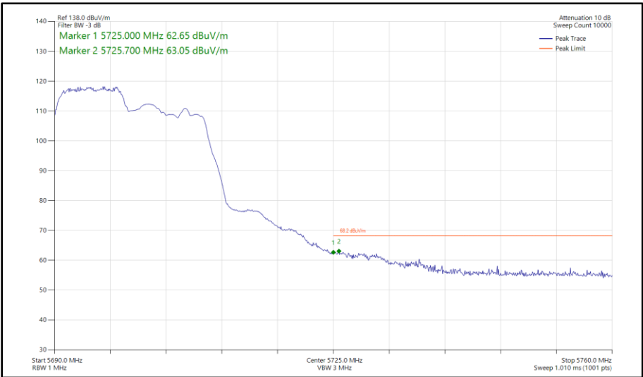
Figure 334 - 802.11ax HE20, RU 106-53, SISO, Core 0 - 5700 MHz Band Edge Frequency 5725 MHz
