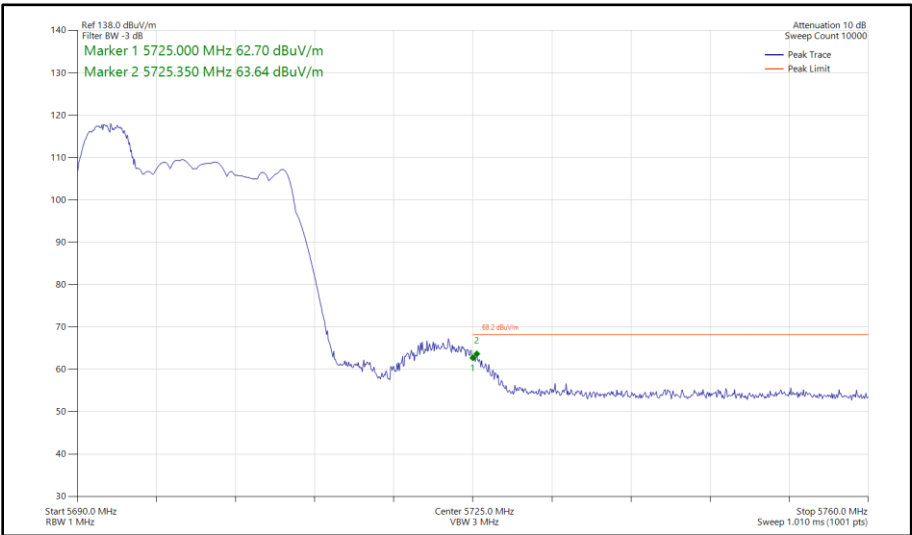
Figure 379 - 802.11ax HE20, RU 52-37, CDD, Core 0 - Core 1 - 5700 MHz Band Edge Frequency 5725 MHz
