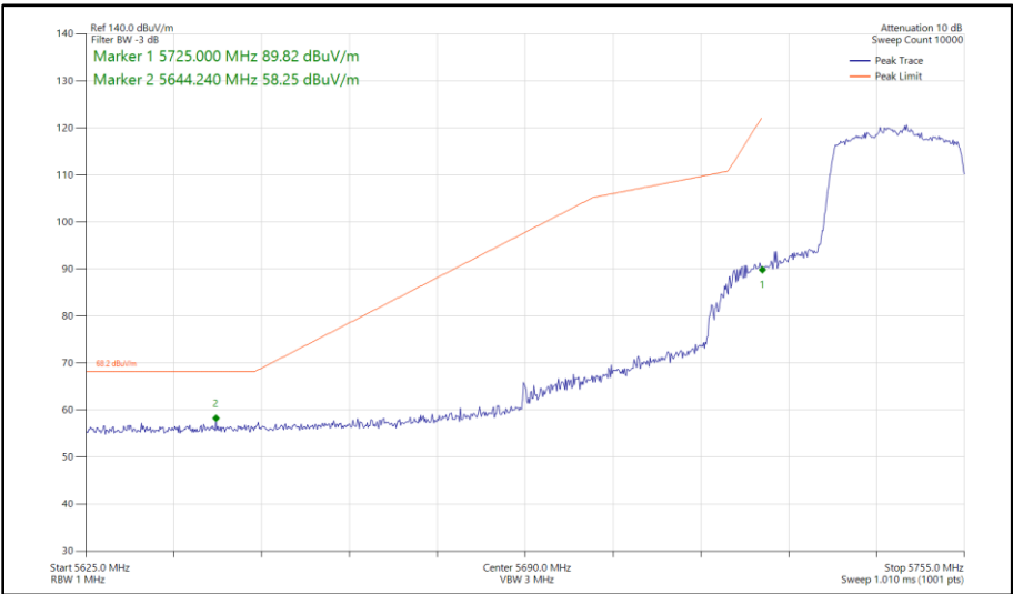
Figure 390 - 802.11ax HE20, SU, SDM, Core 0 - Core 1 - 5745 MHz Band Edge Frequency 5725 MHz
