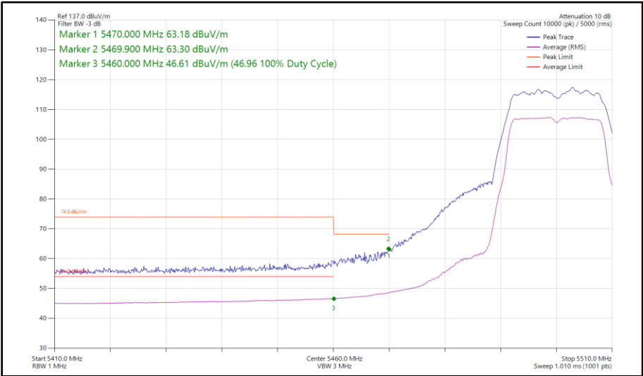
Figure 343 - 802.11a, SISO, Core 1 - 5500 MHz Band Edge Frequency 5470 MHz
