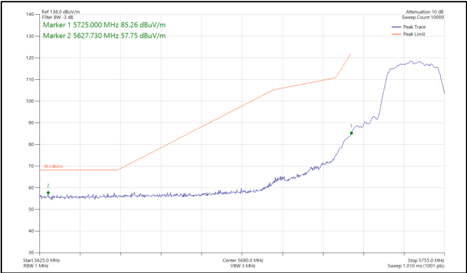
Figure 351 - 802.11a, SISO, Core 1 - 5745 MHz Band Edge Frequency 5725 MHz
