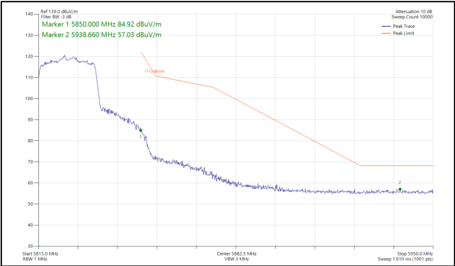
Figure 369 - 802.11ax HE20, SU, SISO, Core 1 - 5825 MHz Band Edge Frequency 5850 MHz
