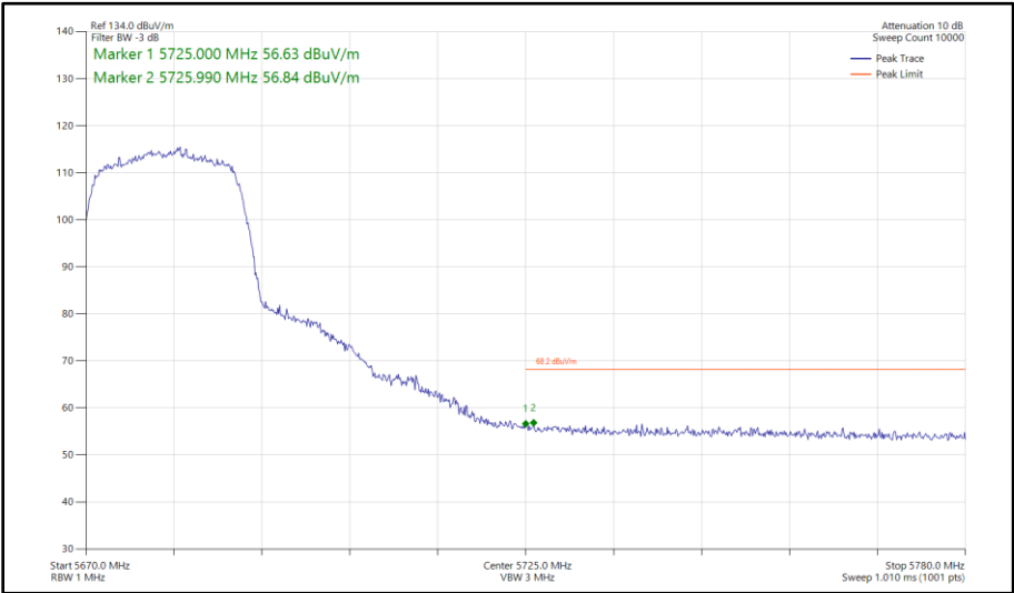
Figure 329 - 802.11n HT20, SISO, Core 0 - 5680 MHz Band Edge Frequency 5725 MHz
