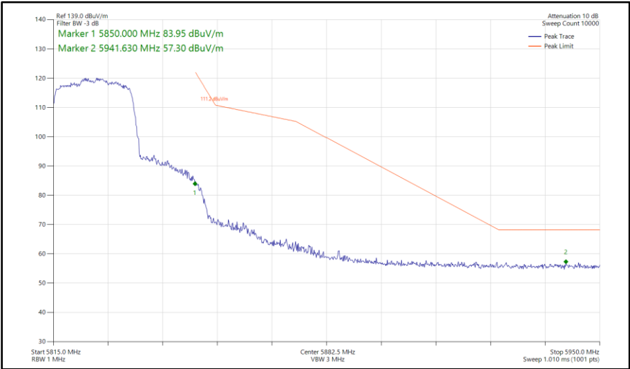
Figure 384 - 802.11ax HE20, SU, CDD, Core 0 - Core 1 - 5825 MHz Band Edge Frequency 5850 MHz
