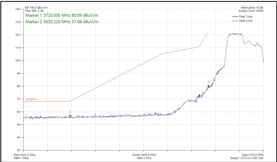
Figure 354 - 802.11ax HE20, RU 106-53, SISO, Core 1 - 5745 MHz Band Edge Frequency 5725 MHz
