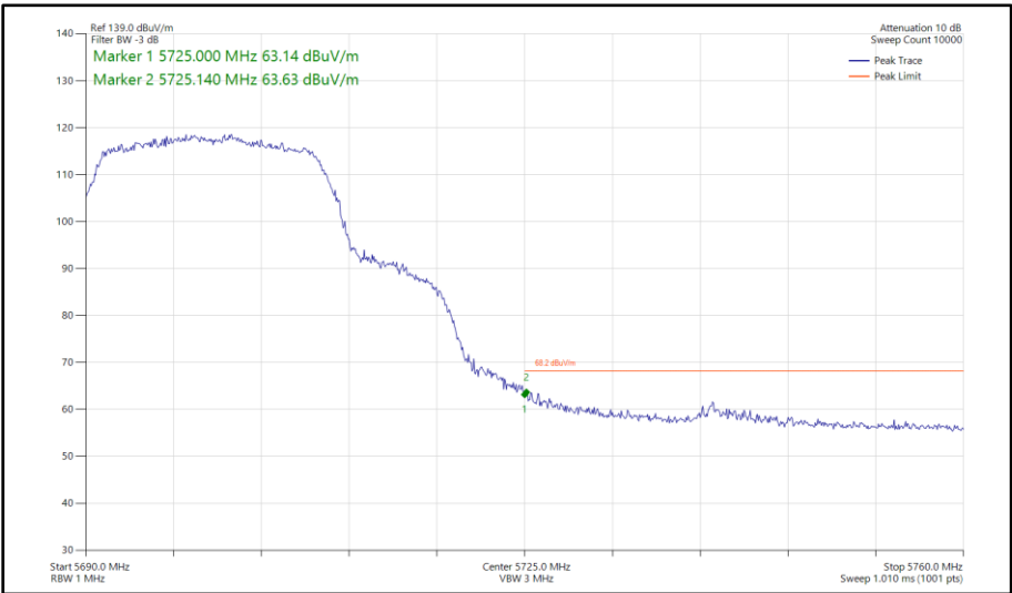
Figure 377 - 802.11n HT20, CDD, Core 0 - Core 1 - 5700 MHz Band Edge Frequency 5725 MHz
