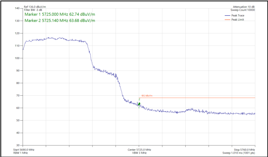
Figure 361 - 802.11ax HE20, SU, SISO, Core 1 - 5700 MHz Band Edge Frequency 5725 MHz
