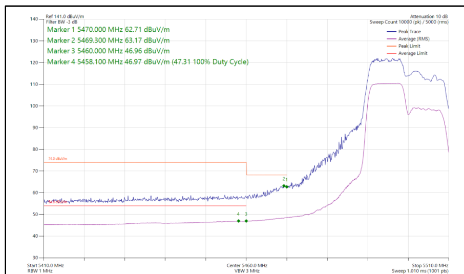
Figure 348 - 802.11ax HE20, RU 106-53, SISO, Core 1 - 5500 MHz Band Edge Frequency 5470 MHz
