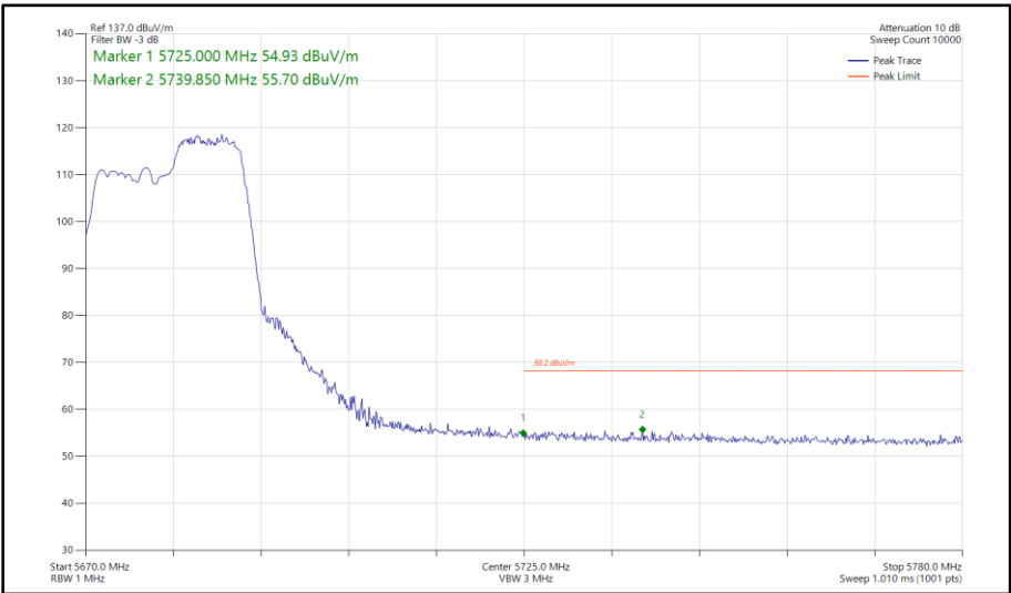
Figure 360 - 802.11ax HE20, RU 106-54, SISO, Core 1 - 5680 MHz Band Edge Frequency 5725 MHz
