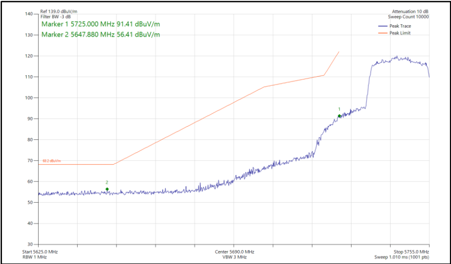
Figure 325 - 802.11ax HE20, SU, SISO, Core 0 - 5745 MHz Band Edge Frequency 5725 MHz
