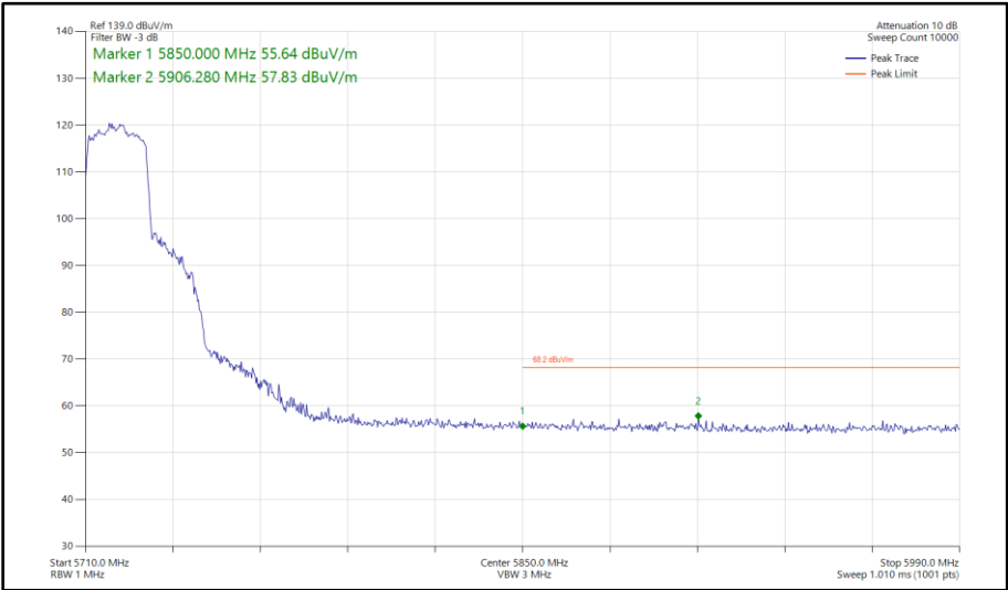
Figure 397 - 802.11ax HE20, SU, SDM, Core 0 - Core 1 - 5720 MHz Band Edge Frequency 5850 MHz
