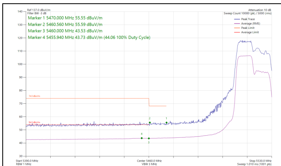
Figure 350 - 802.11ax HE20, RU 106-53, SISO, Core 1 - 5520 MHz Band Edge Frequency 5470 MHz
