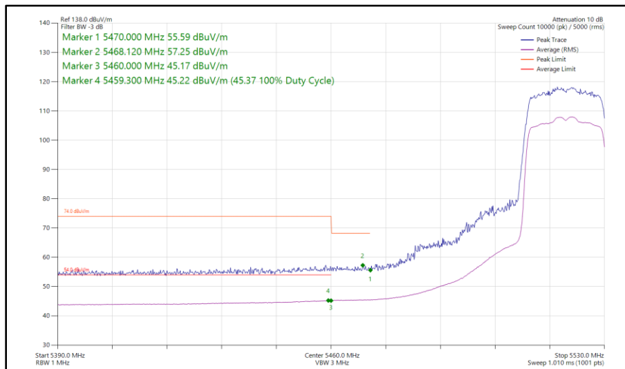
Figure 349 - 802.11ax HE20, SU, SISO, Core 1 - 5520 MHz Band Edge Frequency 5470 MHz
