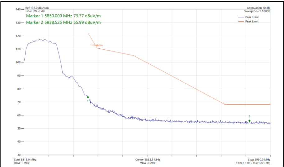
Figure 336 - 802.11a, SISO, Core 0 - 5825 MHz Band Edge Frequency 5850 MHz
