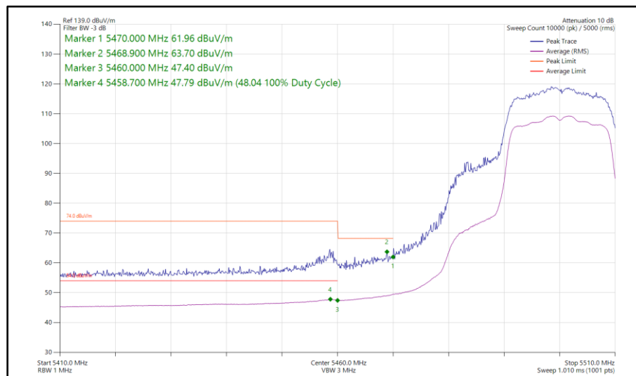
Figure 371 - 802.11n HT20, CDD, Core 0 - Core 1 - 5500 MHz Band Edge Frequency 5470 MHz
