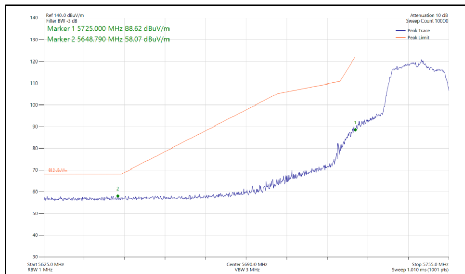
Figure 403 - 802.11ac VHT20, TxBF, Core 0 - Core 1 - 5745 MHz Band Edge Frequency 5725 MHz
