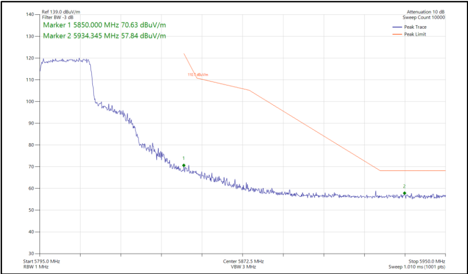
Figure 408 - 802.11ac VHT20, TxBF, Core 0 - Core 1 - 5805 MHz Band Edge Frequency 5850 MHz
