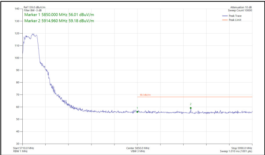
Figure 407 - 802.11ac VHT20, TxBF, Core 0 - Core 1 - 5720 MHz Band Edge Frequency 5850 MHz
