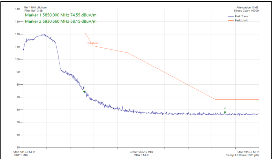
Figure 409 - 802.11ac VHT20, TxBF, Core 0 - Core 1 - 5825 MHz Band Edge Frequency 5850 MHz
