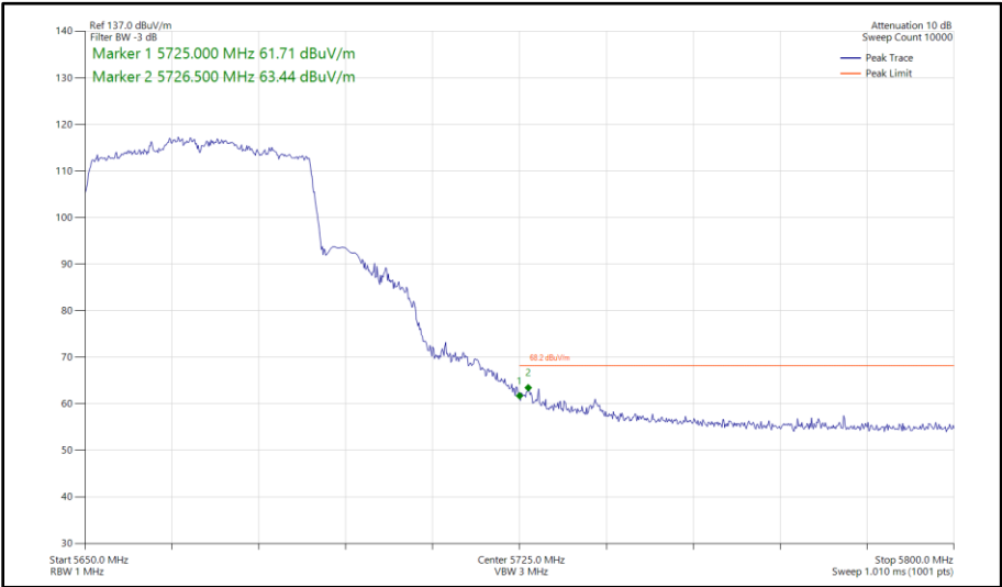
Figure 444 - 802.11ax HE40, SU, SISO, Core 1 - 5670 MHz Band Edge Frequency 5725 MHz
