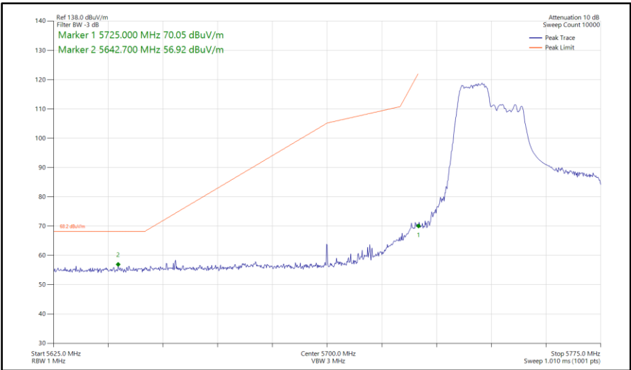
Figure 439 - 802.11ax HE40, RU 106-53, SISO, Core 1 - 5755 MHz Band Edge Frequency 5725 MHz
