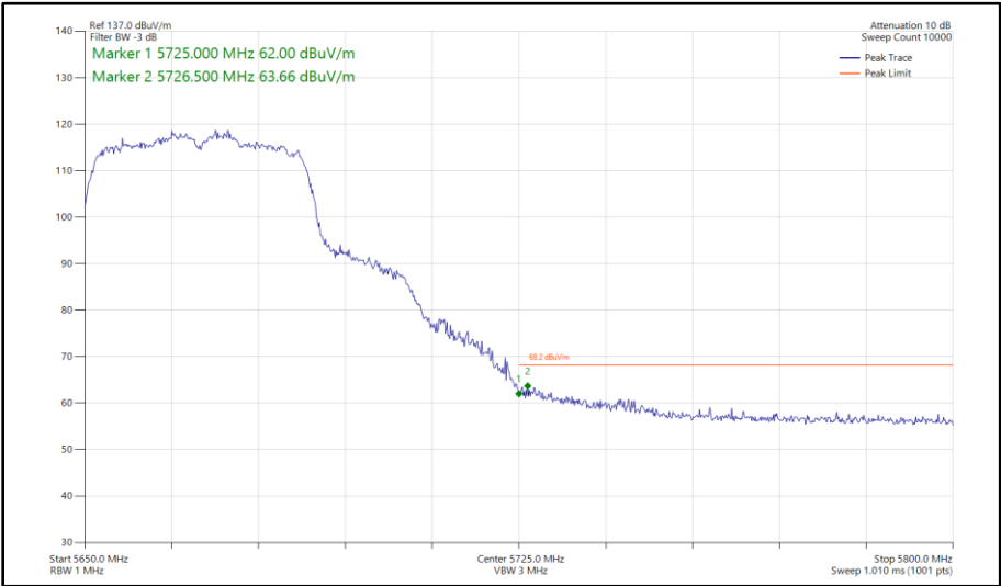
Figure 461 - 802.11n HT40, CDD, Core 0 - Core 1 - 5670 MHz Band Edge Frequency 5725 MHz
