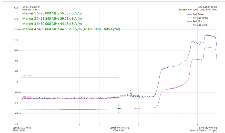
Figure 413 - 802.11ax HE40, RU 106-56, SISO, Core 0 - 5510 MHz Band Edge Frequency 5470 MHz
