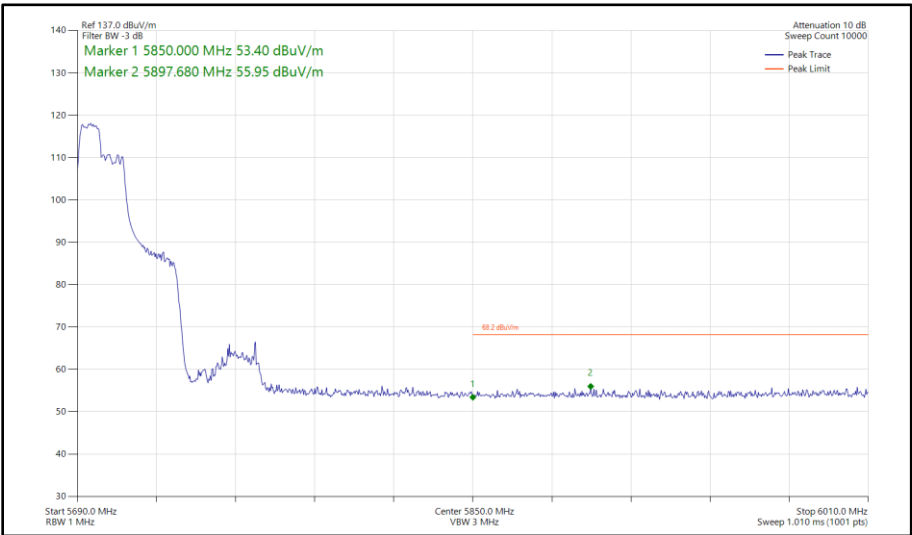
Figure 449 - 802.11ax HE40, RU 106-53, SISO, Core 1 - 5710 MHz Band Edge Frequency 5850 MHz
