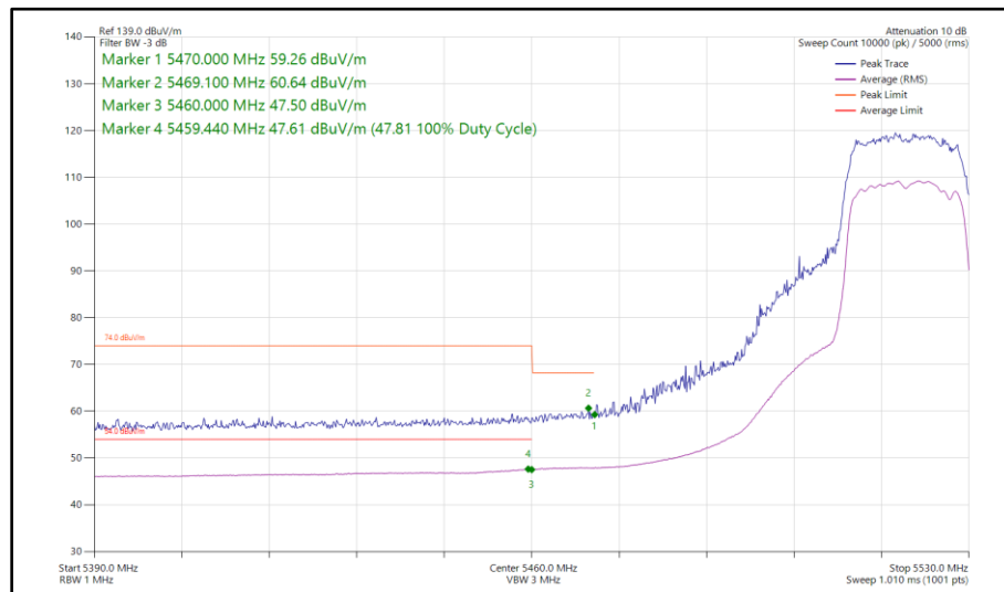
Figure 402 - 802.11ac VHT20, TxBF, Core 0 - Core 1 - 5520 MHz Band Edge Frequency 5470 MHz
