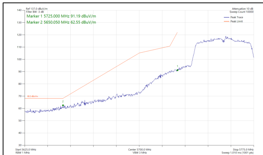
Figure 437 - 802.11n HT40, SISO, Core 1 - 5755 MHz Band Edge Frequency 5725 MHz
