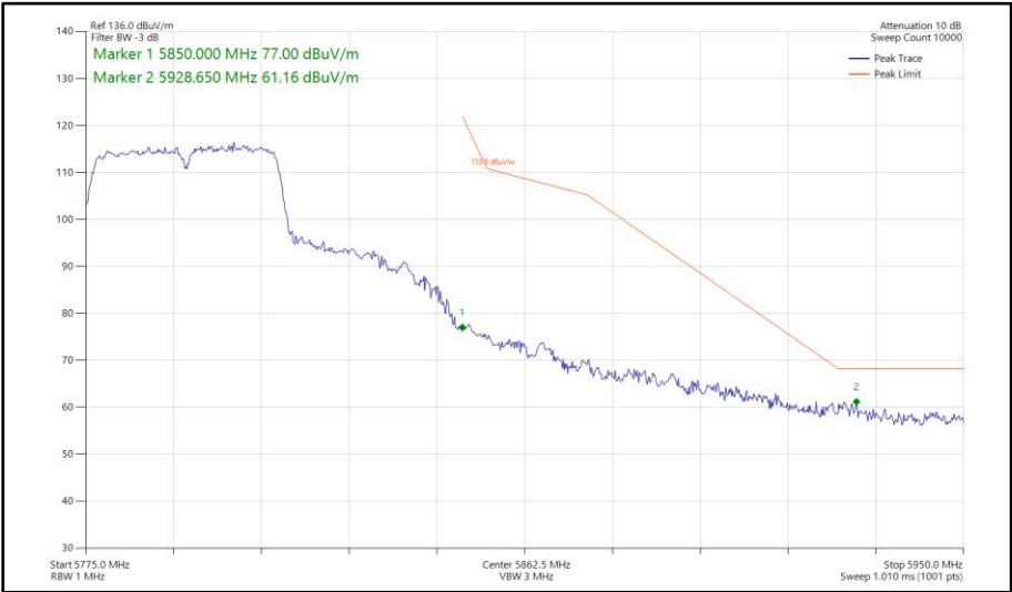
Figure 465 - 802.11n HT40, CDD, Core 0 - Core 1 - 5795 MHz Band Edge Frequency 5850 MHz
