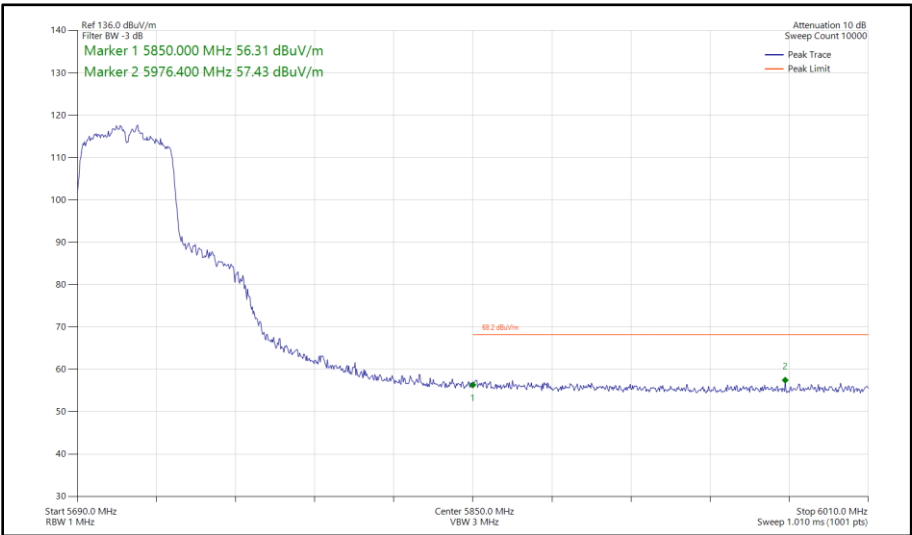
Figure 464 - 802.11n HT40, CDD, Core 0 - Core 1 - 5710 MHz Band Edge Frequency 5850 MHz
