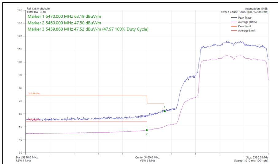
Figure 471 - 802.11ax HE40, SU, SDM, Core 0 - Core 1 - 5510 MHz Band Edge Frequency 5470 MHz
