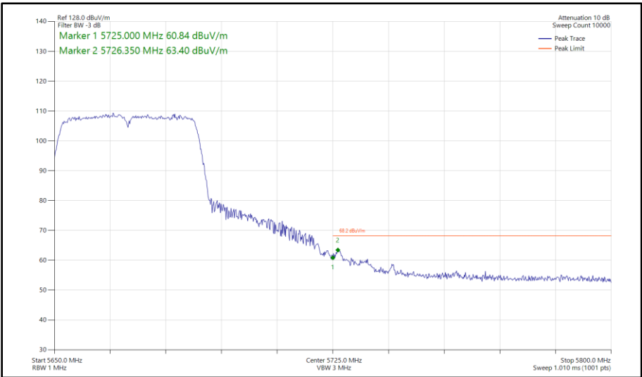
Figure 420 - 802.11n HT40, SISO, Core 0 - 5670 MHz Band Edge Frequency 5725 MHz
