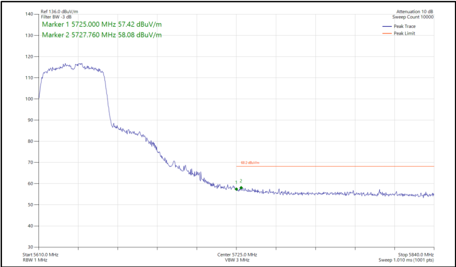
Figure 440 - 802.11n HT40, SISO, Core 1 - 5630 MHz Band Edge Frequency 5725 MHz
