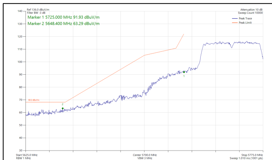
Figure 458 - 802.11n HT40, CDD, Core 0 - Core 1 - 5755 MHz Band Edge Frequency 5725 MHz
