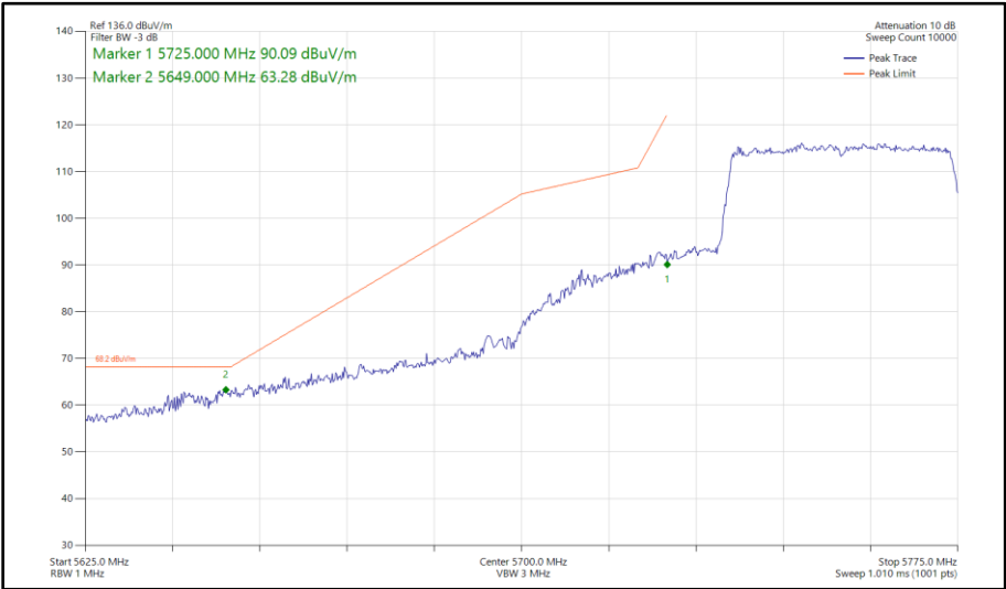
Figure 438 - 802.11ax HE40, SU, SISO, Core 1 - 5755 MHz Band Edge Frequency 5725 MHz
