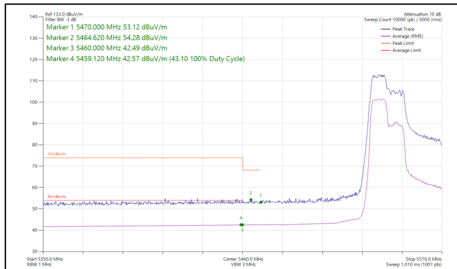
Figure 457 - 802.11ax HE40, RU 106-53, CDD, Core 0 - Core 1 - 5550 MHz Band Edge Frequency 5470 MHz
