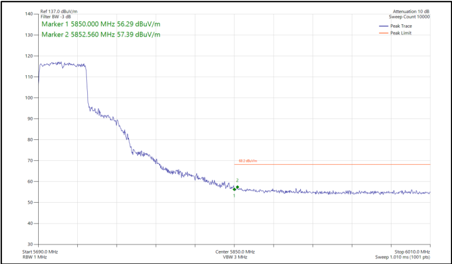
Figure 481 - 802.11ax HE40, SU, SDM, Core 0 - Core 1 - 5710 MHz Band Edge Frequency 5850 MHz
