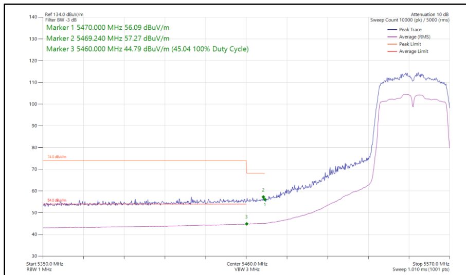
Figure 432 - 802.11n HT40, SISO, Core 1 - 5550 MHz Band Edge Frequency 5470 MHz
