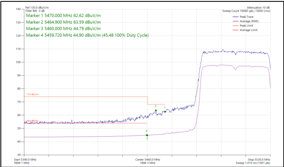
Figure 412 - 802.11ax HE40, SU, SISO, Core 0 - 5510 MHz Band Edge Frequency 5470 MHz
