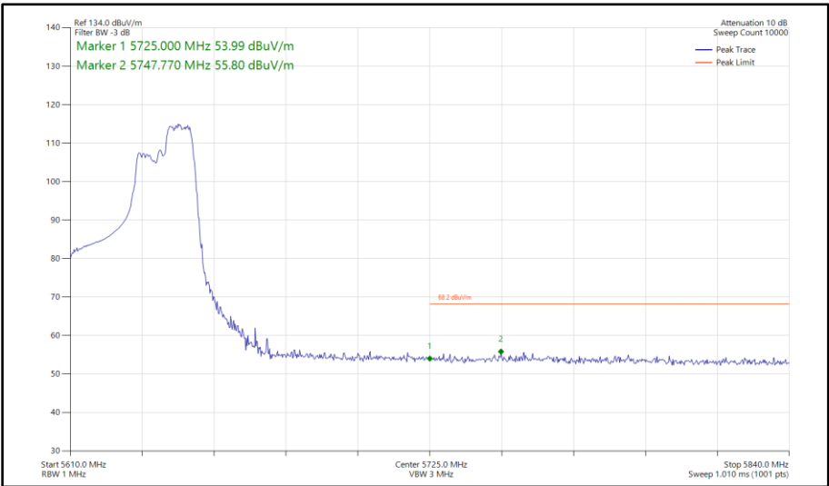
Figure 422 - 802.11ax HE40, RU 106-56, SISO, Core 0 - 5630 MHz Band Edge Frequency 5725 MHz
