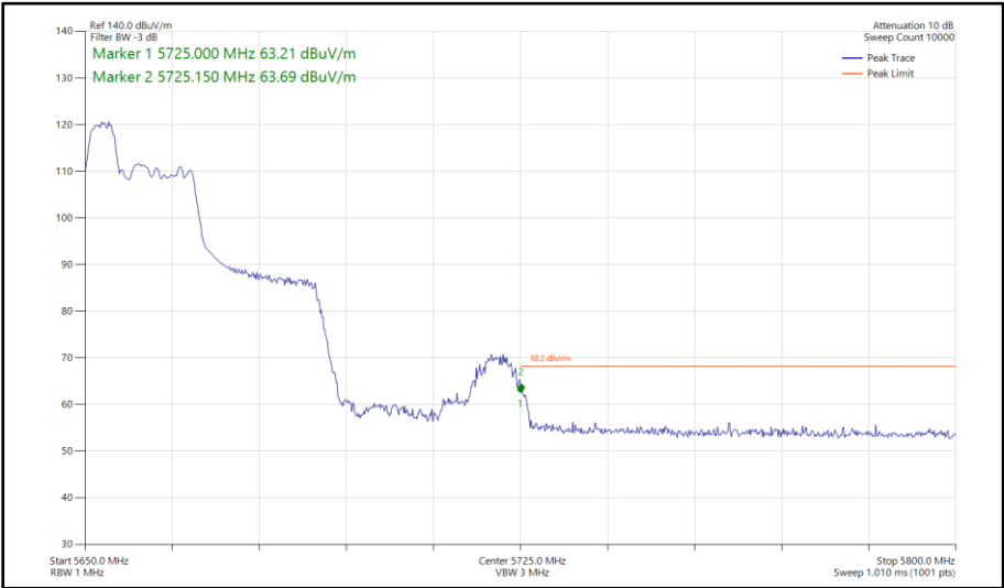
Figure 463 - 802.11ax HE40, RU 52-37, CDD, Core 0 - Core 1 - 5670 MHz Band Edge Frequency 5725 MHz
