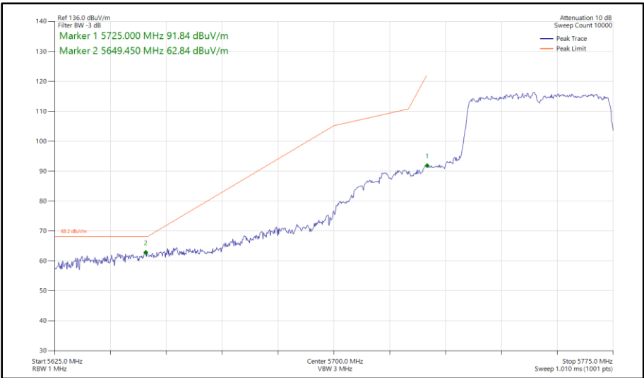
Figure 474 - 802.11ax HE40, SU, SDM, Core 0 - Core 1 - 5755 MHz Band Edge Frequency 5725 MHz
