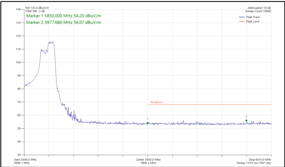
Figure 428 - 802.11ax HE40, RU 106-56, SISO, Core 0 - 5710 MHz Band Edge Frequency 5850 MHz
