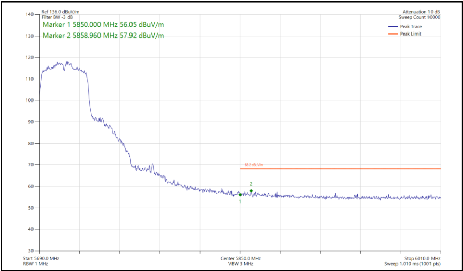
Figure 446 - 802.11n HT40, SISO, Core 1 - 5710 MHz Band Edge Frequency 5850 MHz
