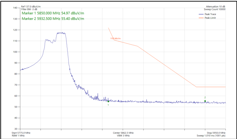
Figure 451 - 802.11ax HE40, RU 106-56, SISO, Core 1 - 5795 MHz Band Edge Frequency 5850 MHz
