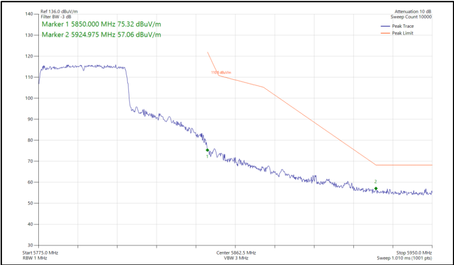
Figure 429 - 802.11ax HE40, SU, SISO, Core 0 - 5795 MHz Band Edge Frequency 5850 MHz
