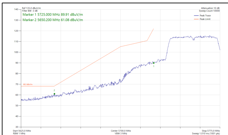
Figure 416 - 802.11n HT40, SISO, Core 0 - 5755 MHz Band Edge Frequency 5725 MHz
