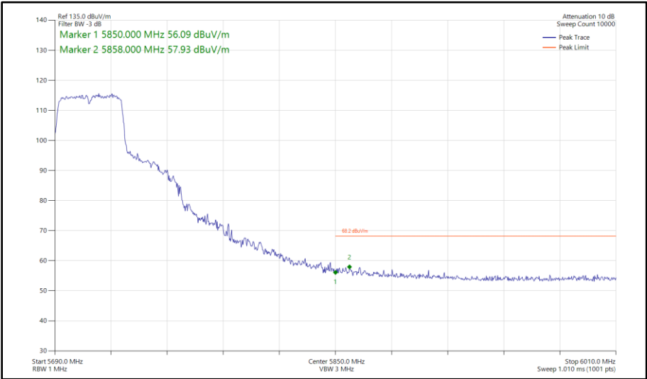
Figure 425 - 802.11n HT40, SISO, Core 0 - 5710 MHz Band Edge Frequency 5850 MHz
