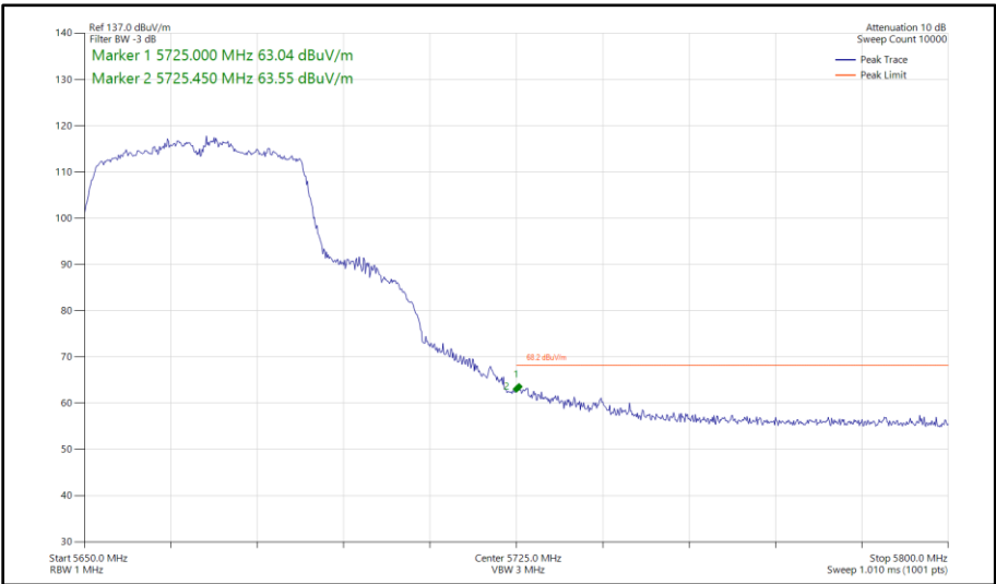
Figure 441 - 802.11n HT40, SISO, Core 1 - 5670 MHz Band Edge Frequency 5725 MHz
