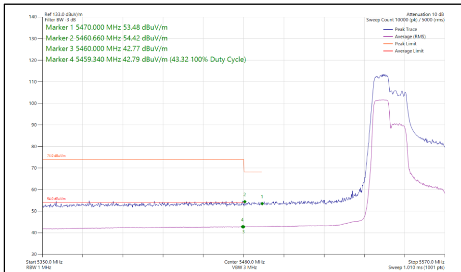
Figure 415 - 802.11ax HE40, RU 106-53, SISO, Core 0 - 5550 MHz Band Edge Frequency 5470 MHz
