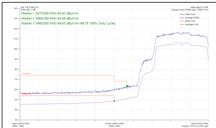
Figure 433 - 802.11ax HE40, SU, SISO, Core 1 - 5510 MHz Band Edge Frequency 5470 MHz
