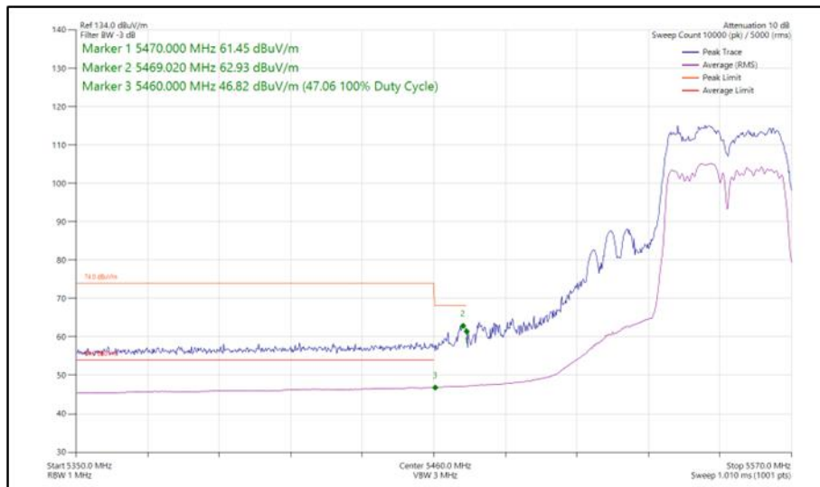
Figure 486 - 802.11ac VHT40, TxBF, Core 0 - Core 1 - 5550 MHz Band Edge Frequency 5470 MHz
