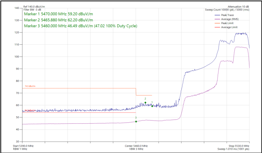
Figure 434 - 802.11ax HE40, RU 106-56, SISO, Core 1 - 5510 MHz Band Edge Frequency 5470 MHz
