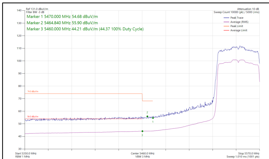
Figure 414 - 802.11ax HE40, SU, SISO, Core 0 - 5550 MHz Band Edge Frequency 5470 MHz
