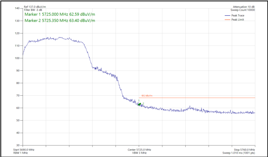
Figure 406 - 802.11ac VHT20, TxBF, Core 0 - Core 1 - 5700 MHz Band Edge Frequency 5725 MHz
