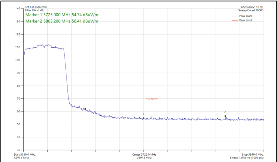
Figure 442 - 802.11ax HE40, SU, SISO, Core 1 - 5630 MHz Band Edge Frequency 5725 MHz
