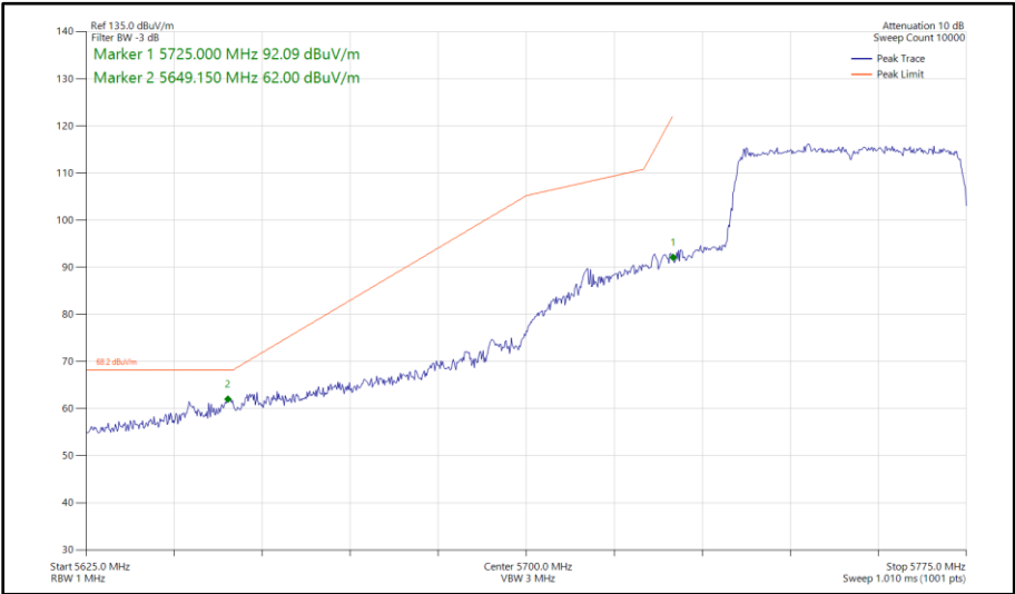
Figure 417 - 802.11ax HE40, SU, SISO, Core 0 - 5755 MHz Band Edge Frequency 5725 MHz
