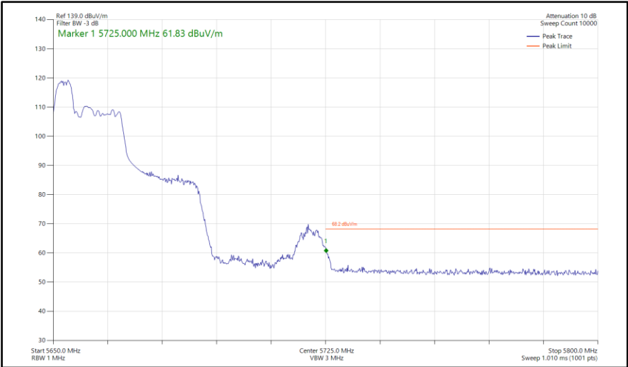
Figure 478 - 802.11ax HE40, RU 52-37, SDM, Core 0 - Core 1 - 5670 MHz Band Edge Frequency 5725 MHz
