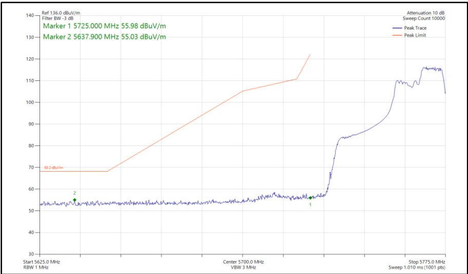
Figure 418 - 802.11ax HE40, RU 106-56, SISO, Core 0 - 5755 MHz Band Edge Frequency 5725 MHz
