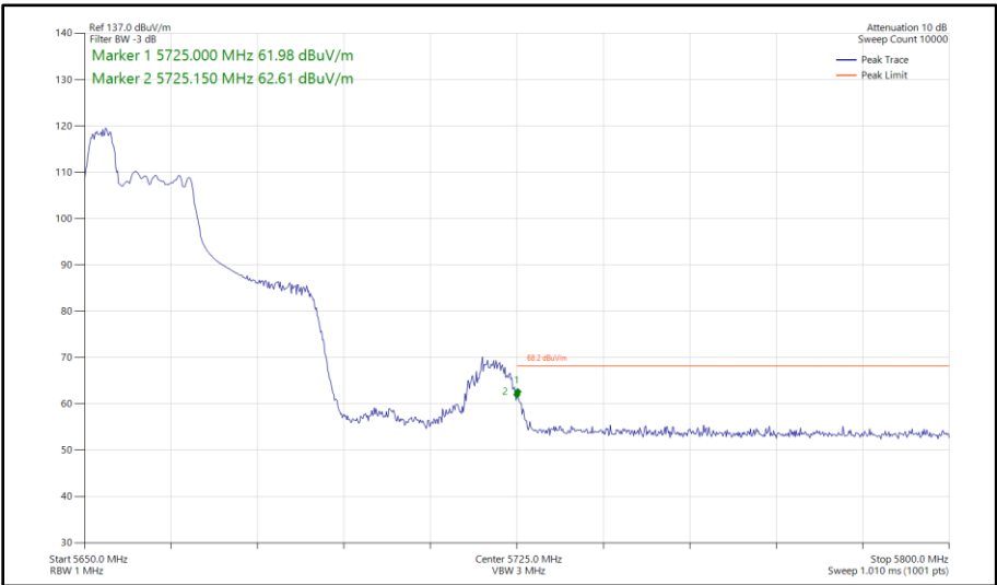
Figure 445 - 802.11ax HE40, RU 52-37, SISO, Core 1 - 5670 MHz Band Edge Frequency 5725 MHz
