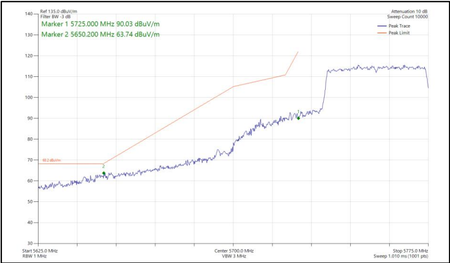
Figure 459 - 802.11ax HE40, SU, CDD, Core 0 - Core 1 - 5755 MHz Band Edge Frequency 5725 MHz
