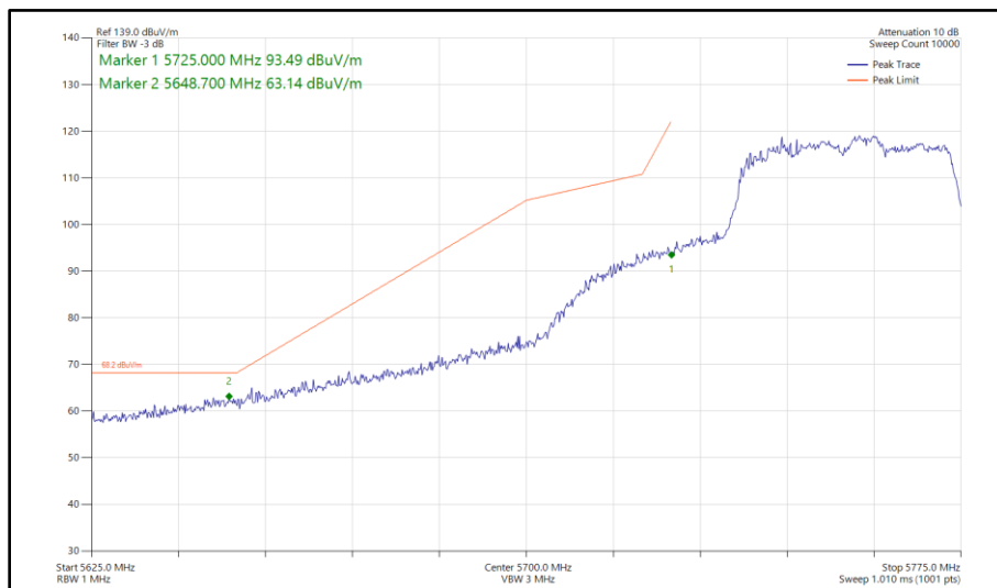
Figure 487 - 802.11ac VHT40, TxBF, Core 0 - Core 1 - 5755 MHz Band Edge Frequency 5725 MHz
