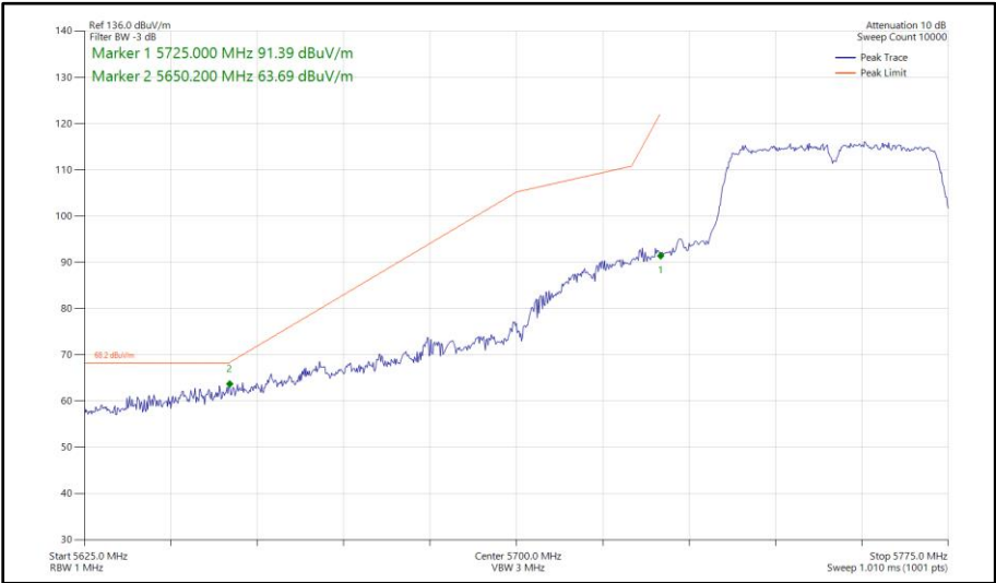
Figure 473 - 802.11n HT40, SDM, Core 0 - Core 1 - 5755 MHz Band Edge Frequency 5725 MHz
