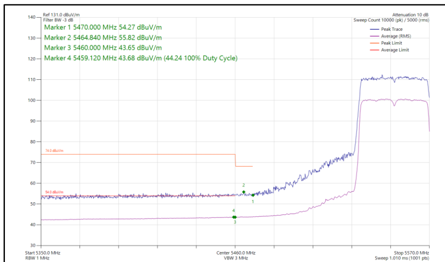
Figure 456 - 802.11ax HE40, SU, CDD, Core 0 - Core 1 - 5550 MHz Band Edge Frequency 5470 MHz
