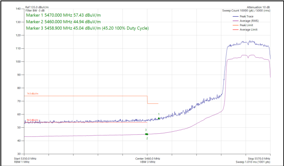
Figure 435 - 802.11ax HE40, SU, SISO, Core 1 - 5550 MHz Band Edge Frequency 5470 MHz
