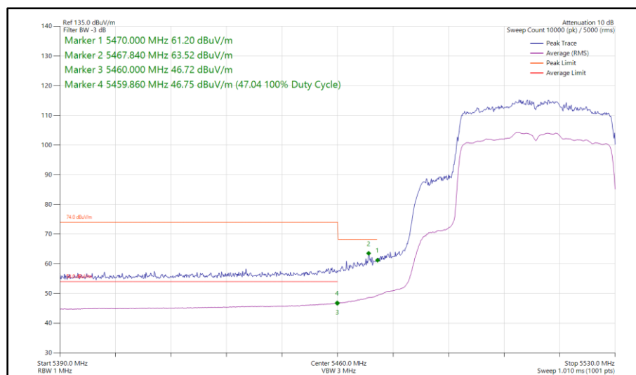
Figure 454 - 802.11ax HE40, SU, CDD, Core 0 - Core 1 - 5510 MHz Band Edge Frequency 5470 MHz
