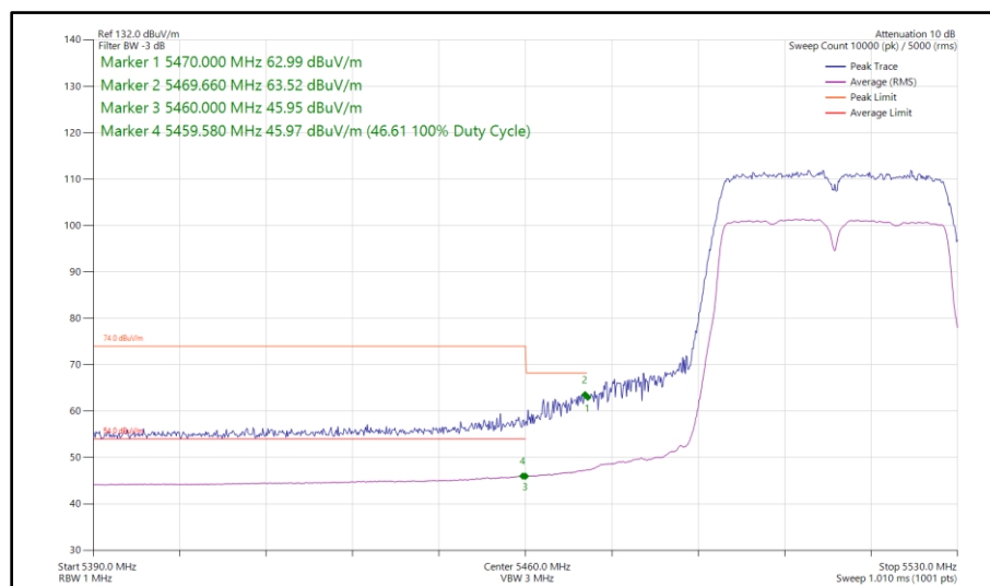
Figure 431 - 802.11n HT40, SISO, Core 1 - 5510 MHz Band Edge Frequency 5470 MHz
