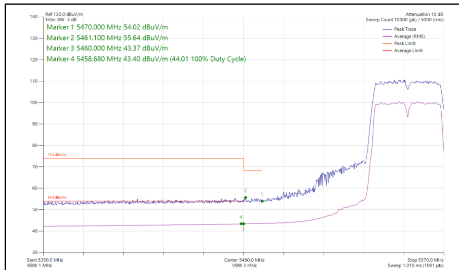
Figure 453 - 802.11n HT40, CDD, Core 0 - Core 1 - 5550 MHz Band Edge Frequency 5470 MHz
