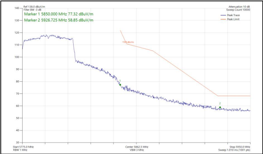
Figure 450 - 802.11ax HE40, SU, SISO, Core 1 - 5795 MHz Band Edge Frequency 5850 MHz
