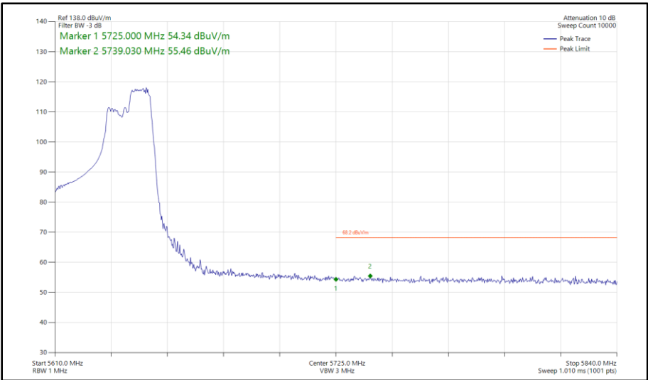
Figure 443 - 802.11ax HE40, RU 106-56, SISO, Core 1 - 5630 MHz Band Edge Frequency 5725 MHz
