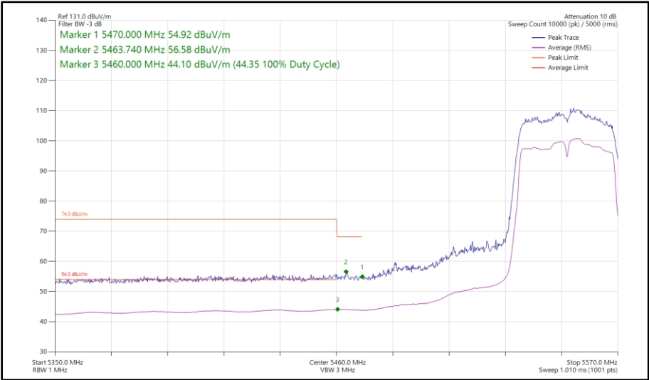
Figure 411 - 802.11n HT40, SISO, Core 0 - 5550 MHz Band Edge Frequency 5470 MHz
