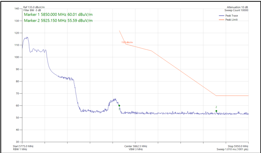
Figure 430 - 802.11ax HE40, RU 52-37, SISO, Core 0 - 5795 MHz Band Edge Frequency 5850 MHz
