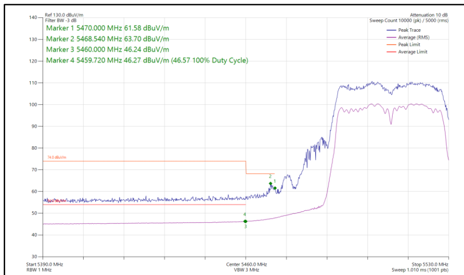
Figure 485 - 802.11ac VHT40, TxBF, Core 0 - Core 1 - 5510 MHz Band Edge Frequency 5470 MHz
