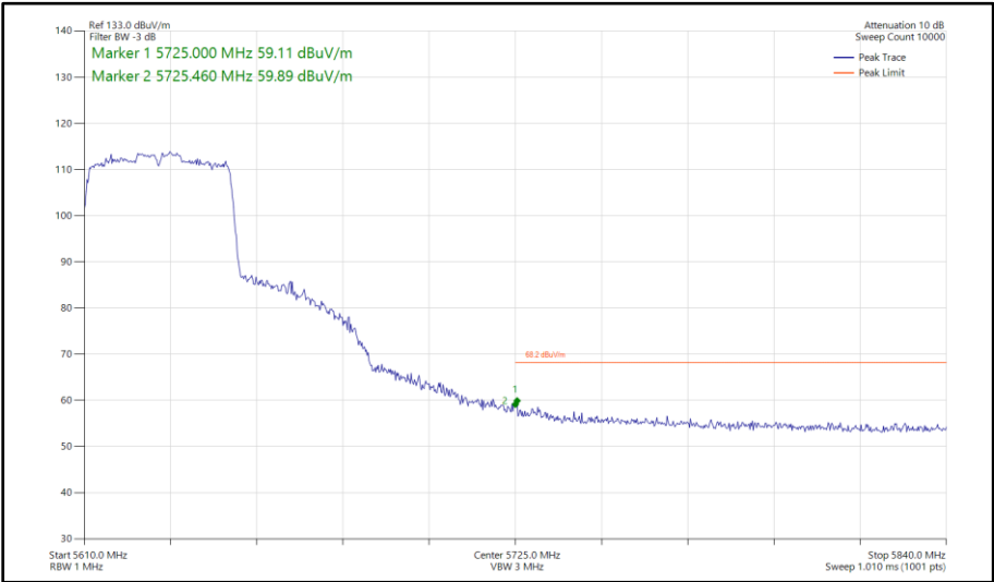
Figure 421 - 802.11ax HE40, SU, SISO, Core 0 - 5630 MHz Band Edge Frequency 5725 MHz
