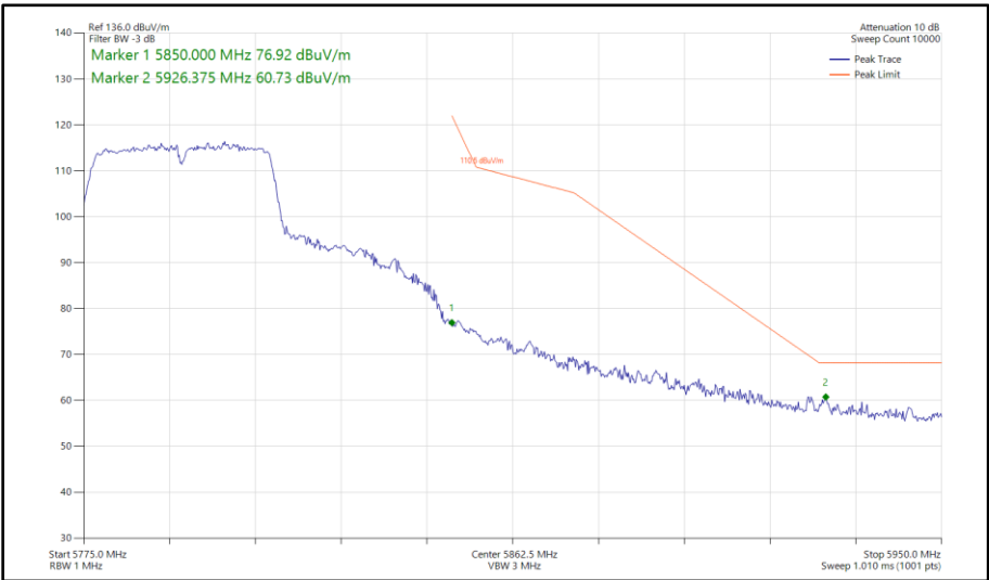
Figure 480 - 802.11n HT40, SDM, Core 0 - Core 1 - 5795 MHz Band Edge Frequency 5850 MHz
