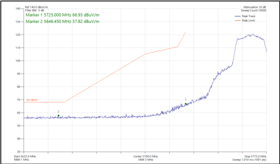
Figure 404 - 802.11ac VHT20, TxBF, Core 0 - Core 1 - 5765 MHz Band Edge Frequency 5725 MHz
