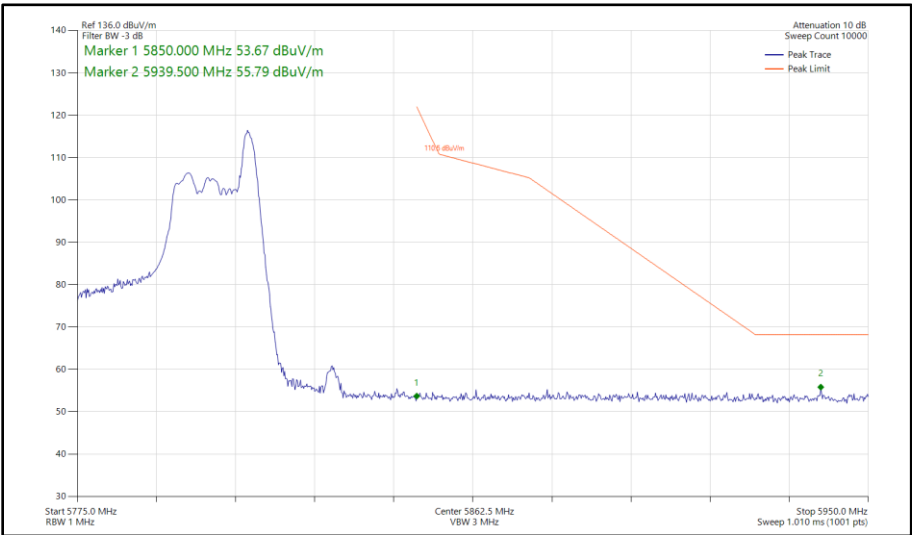
Figure 484 - 802.11ax HE40, RU 26-17, SDM, Core 0 - Core 1 - 5795 MHz Band Edge Frequency 5850 MHz
