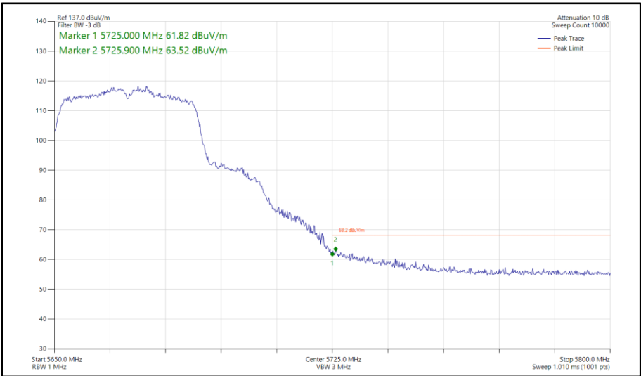
Figure 476 - 802.11n HT40, SDM, Core 0 - Core 1 - 5670 MHz Band Edge Frequency 5725 MHz
