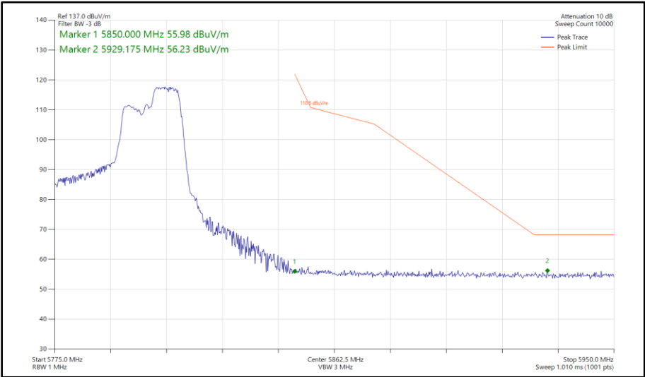
Figure 469 - 802.11ax HE40, RU 106-56, CDD, Core 0 - Core 1 - 5795 MHz Band Edge Frequency 5850 MHz
