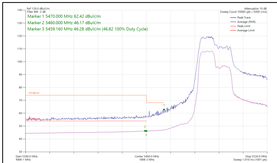
Figure 455 - 802.11ax HE40, RU 106-53, CDD, Core 0 - Core 1 - 5510 MHz Band Edge Frequency 5470 MHz
