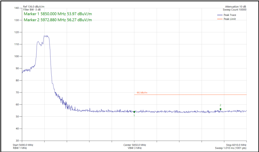
Figure 467 - 802.11ax HE40, RU 106-56, CDD, Core 0 - Core 1 - 5710 MHz Band Edge Frequency 5850 MHz
