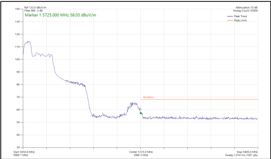
Figure 424 - 802.11ax HE40, RU 52-37, SISO, Core 0 - 5670 MHz Band Edge Frequency 5725 MHz
