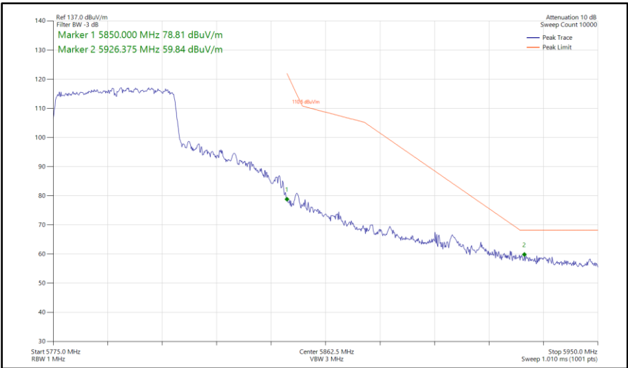
Figure 468 - 802.11ax HE40, SU, CDD, Core 0 - Core 1 - 5795 MHz Band Edge Frequency 5850 MHz
