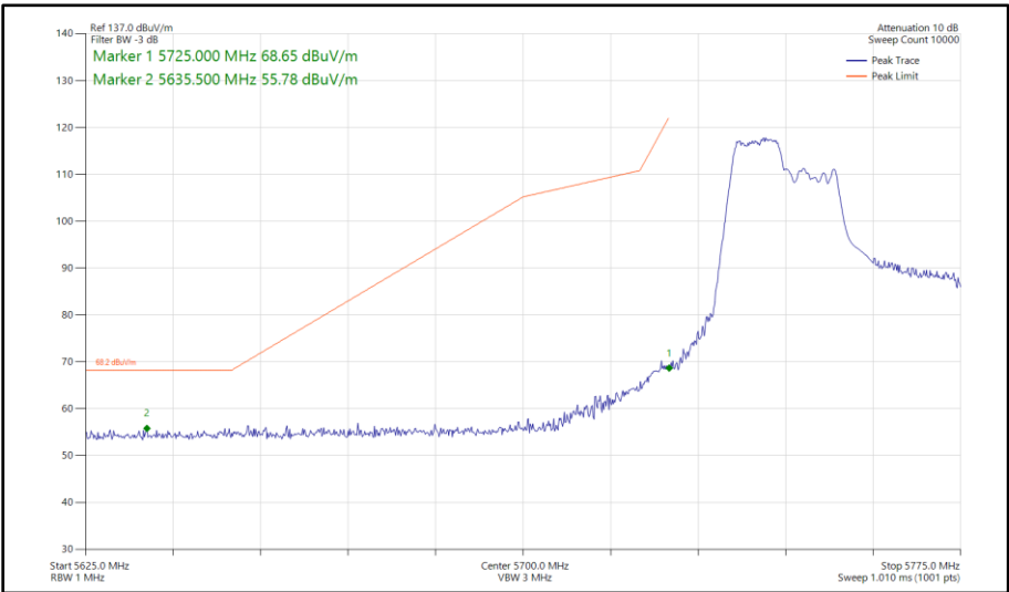
Figure 460 - 802.11ax HE40, RU 106-53, CDD, Core 0 - Core 1 - 5755 MHz Band Edge Frequency 5725 MHz
