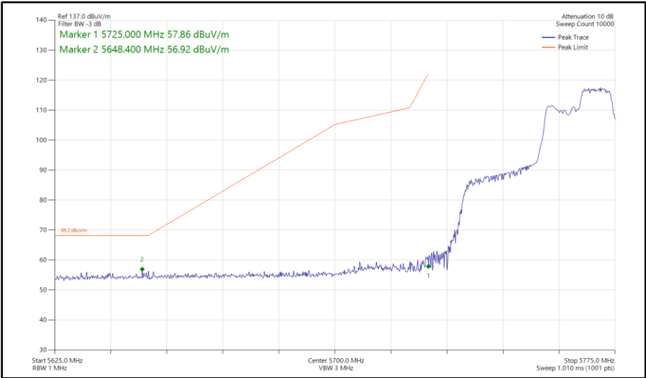
Figure 475 - 802.11ax HE40, RU 106-56, SDM, Core 0 - Core 1 - 5755 MHz Band Edge Frequency 5725 MHz
