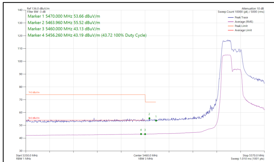
Figure 436 - 802.11ax HE40, RU 106-53, SISO, Core 1 - 5550 MHz Band Edge Frequency 5470 MHz
