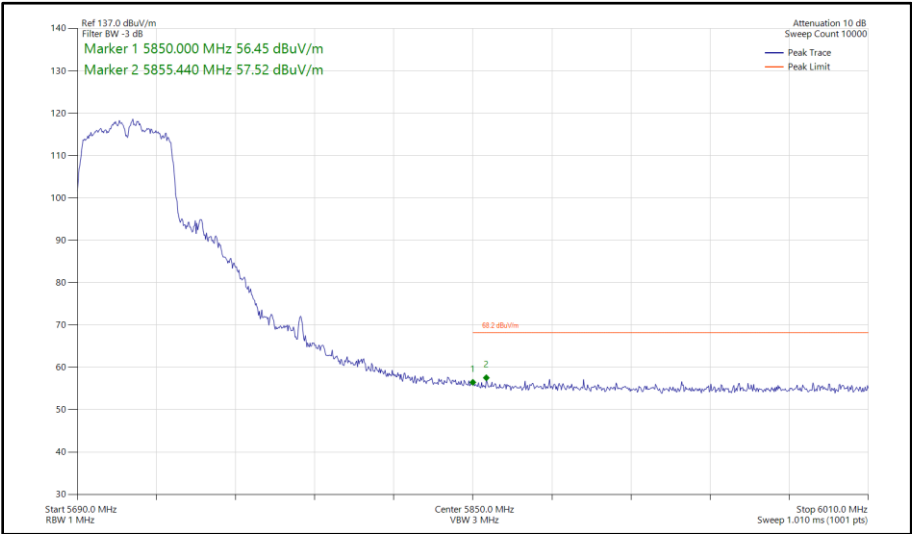
Figure 479 - 802.11n HT40, SDM, Core 0 - Core 1 - 5710 MHz Band Edge Frequency 5850 MHz
