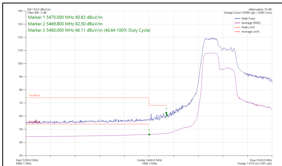
Figure 472 - 802.11ax HE40, RU 106-53, SDM, Core 0 - Core 1 - 5510 MHz Band Edge Frequency 5470 MHz
