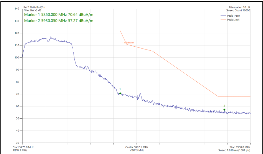
Figure 426 - 802.11n HT40, SISO, Core 0 - 5795 MHz Band Edge Frequency 5850 MHz
