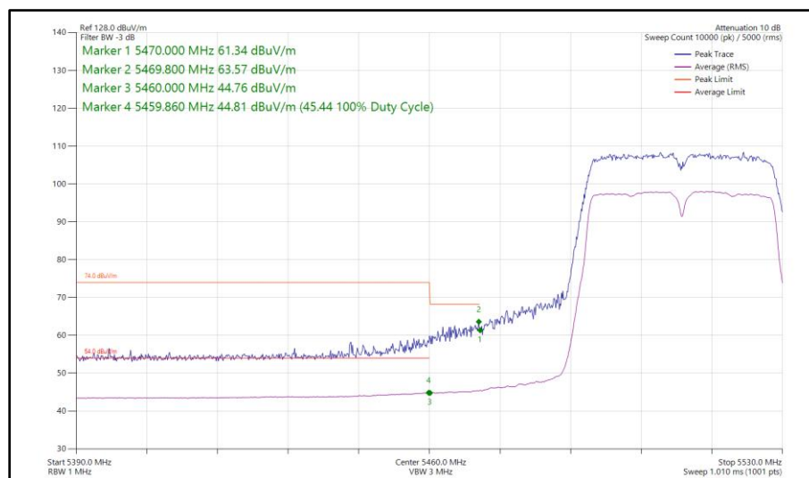
Figure 410 - 802.11n HT40, SISO, Core 0 - 5510 MHz Band Edge Frequency 5470 MHz
