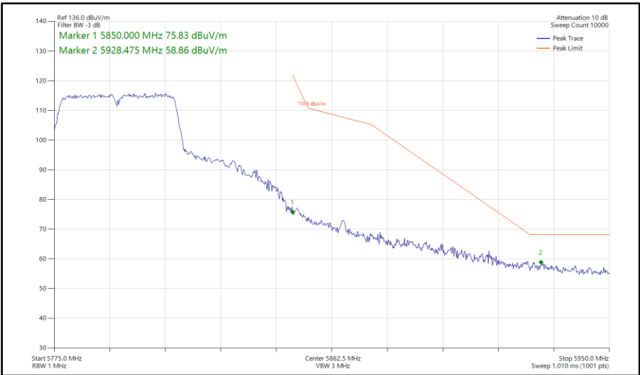
Figure 447 - 802.11n HT40, SISO, Core 1 - 5795 MHz Band Edge Frequency 5850 MHz
