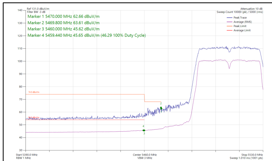
Figure 470 - 802.11n HT40, SDM, Core 0 - Core 1 - 5510 MHz Band Edge Frequency 5470 MHz
