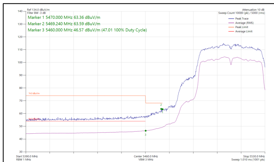
Figure 452 - 802.11n HT40, CDD, Core 0 - Core 1 - 5510 MHz Band Edge Frequency 5470 MHz
