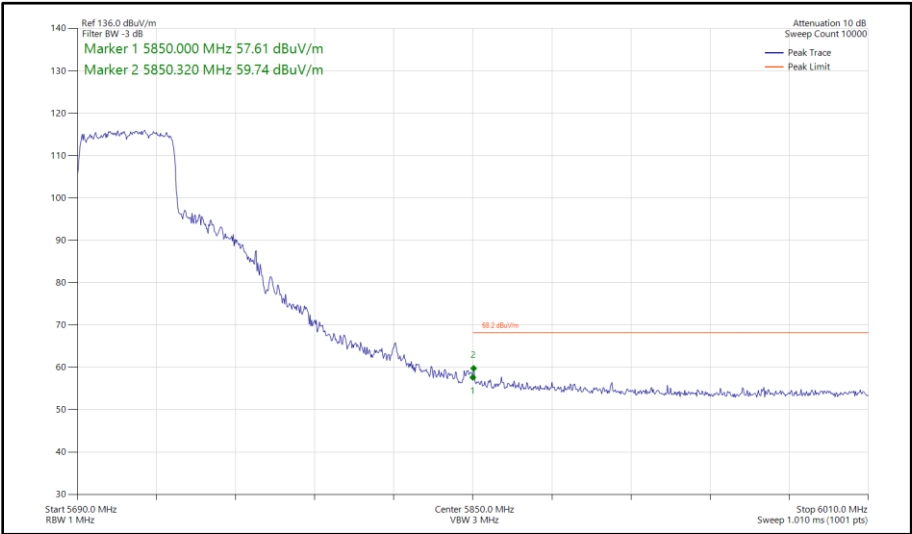
Figure 427 - 802.11ax HE40, SU, SISO, Core 0 - 5710 MHz Band Edge Frequency 5850 MHz
