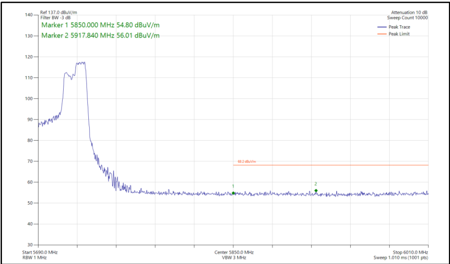
Figure 482 - 802.11ax HE40, RU 106-56, SDM, Core 0 - Core 1 - 5710 MHz Band Edge Frequency 5850 MHz
