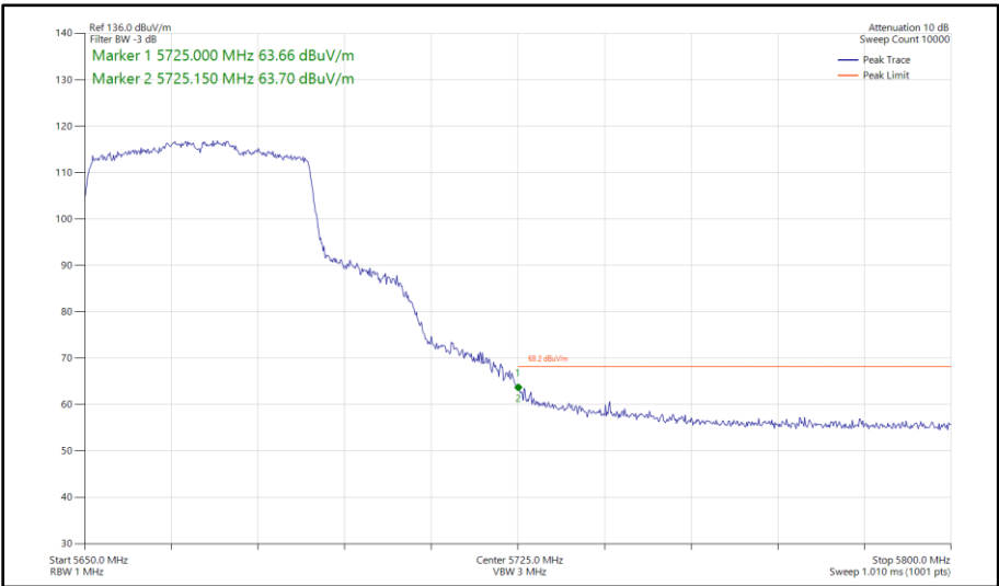
Figure 462 - 802.11ax HE40, SU, CDD, Core 0 - Core 1 - 5670 MHz Band Edge Frequency 5725 MHz
