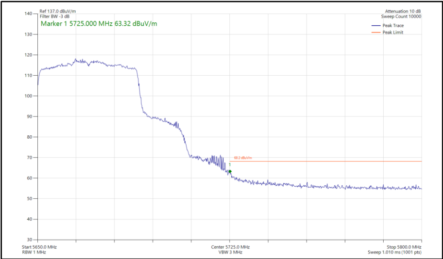
Figure 477 - 802.11ax HE40, SU, SDM, Core 0 - Core 1 - 5670 MHz Band Edge Frequency 5725 MHz
