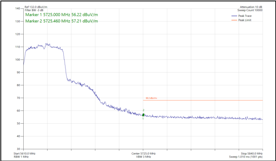
Figure 419 - 802.11n HT40, SISO, Core 0 - 5630 MHz Band Edge Frequency 5725 MHz
