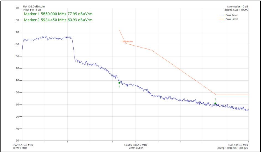
Figure 483 - 802.11ax HE40, SU, SDM, Core 0 - Core 1 - 5795 MHz Band Edge Frequency 5850 MHz
