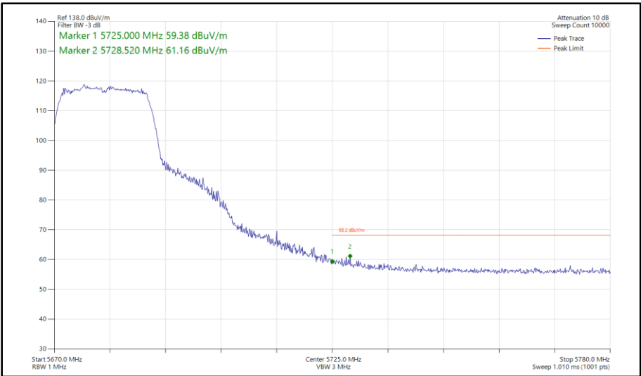
Figure 405 - 802.11ac VHT20, TxBF, Core 0 - Core 1 - 5680 MHz Band Edge Frequency 5725 MHz
