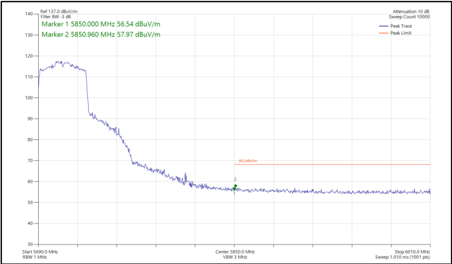
Figure 448 - 802.11ax HE40, SU, SISO, Core 1 - 5710 MHz Band Edge Frequency 5850 MHz
