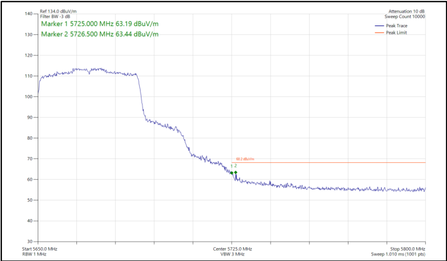
Figure 423 - 802.11ax HE40, SU, SISO, Core 0 - 5670 MHz Band Edge Frequency 5725 MHz
