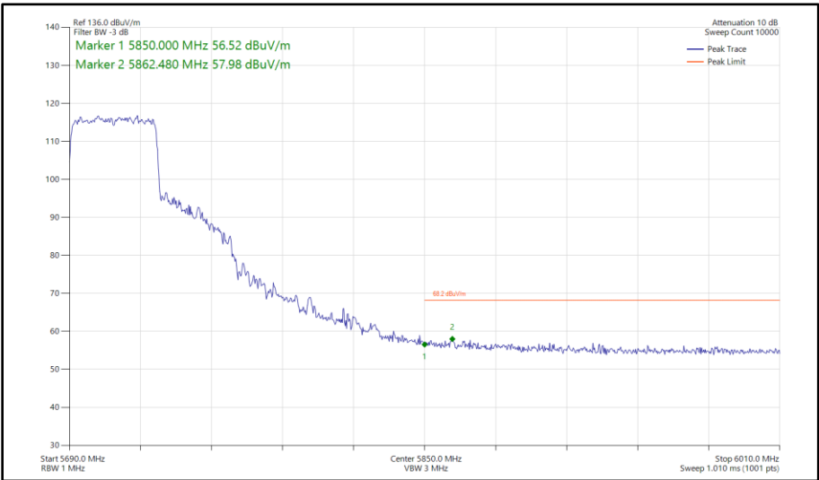
Figure 466 - 802.11ax HE40, SU, CDD, Core 0 - Core 1 - 5710 MHz Band Edge Frequency 5850 MHz
