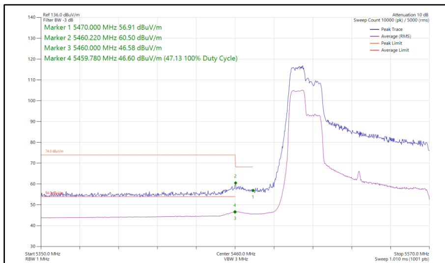
Figure 539 - 802.11ax HE80, RU 106-53, SDM, Core 0 - Core 1 - 5530 MHz Band Edge Frequency 5470 MHz
