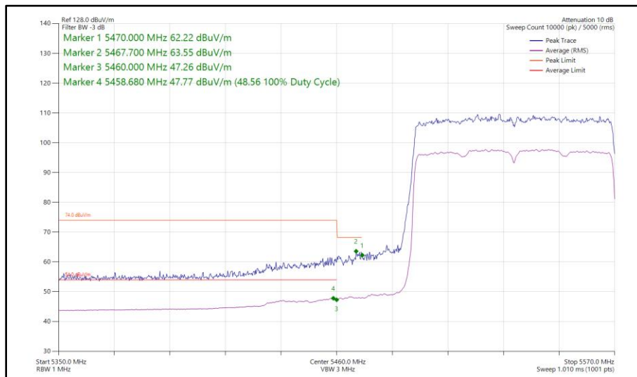
Figure 538 - 802.11ax HE80, SU, SDM, Core 0 - Core 1 - 5530 MHz Band Edge Frequency 5470 MHz
