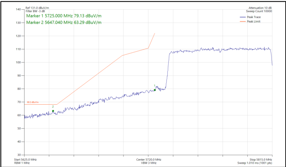
Figure 541 - 802.11ax HE80, SU, SDM, Core 0 - Core 1 - 5775 MHz Band Edge Frequency 5725 MHz
