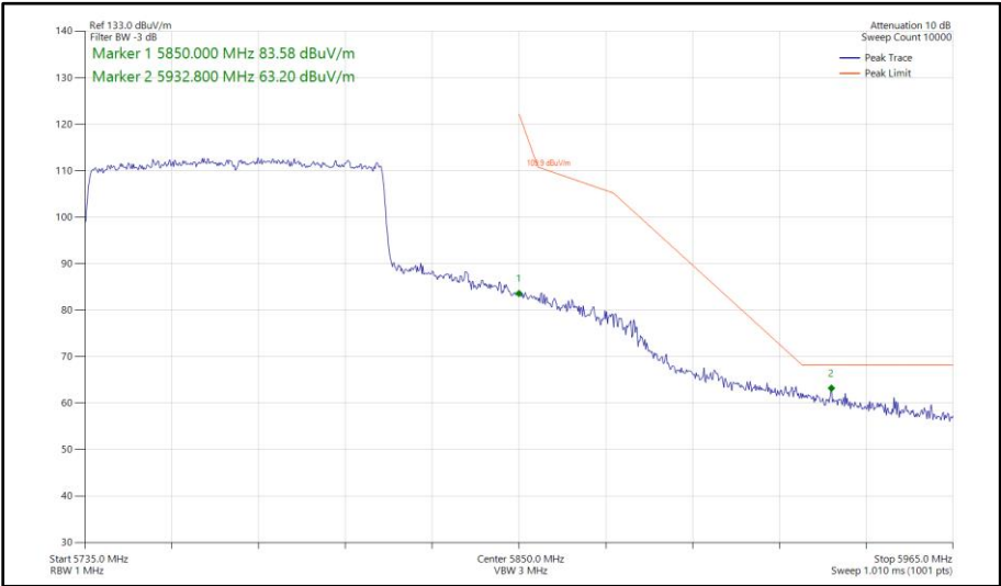
Figure 505 - 802.11ax HE80, SU, SISO, Core 0 - 5775 MHz Band Edge Frequency 5850 MHz
