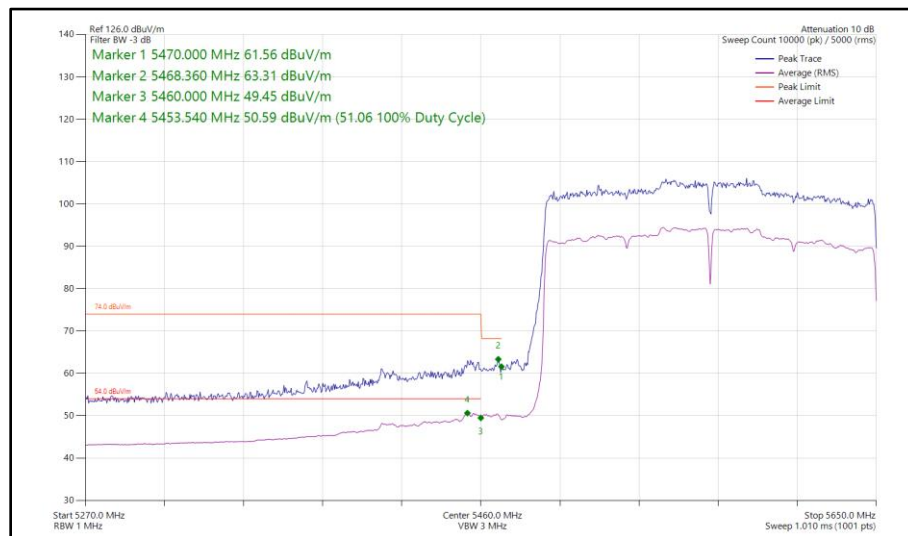
Figure 564 - 802.11ax HE160, SU, SISO, Core 1 - 5570 MHz Band Edge Frequency 5470 MHz
