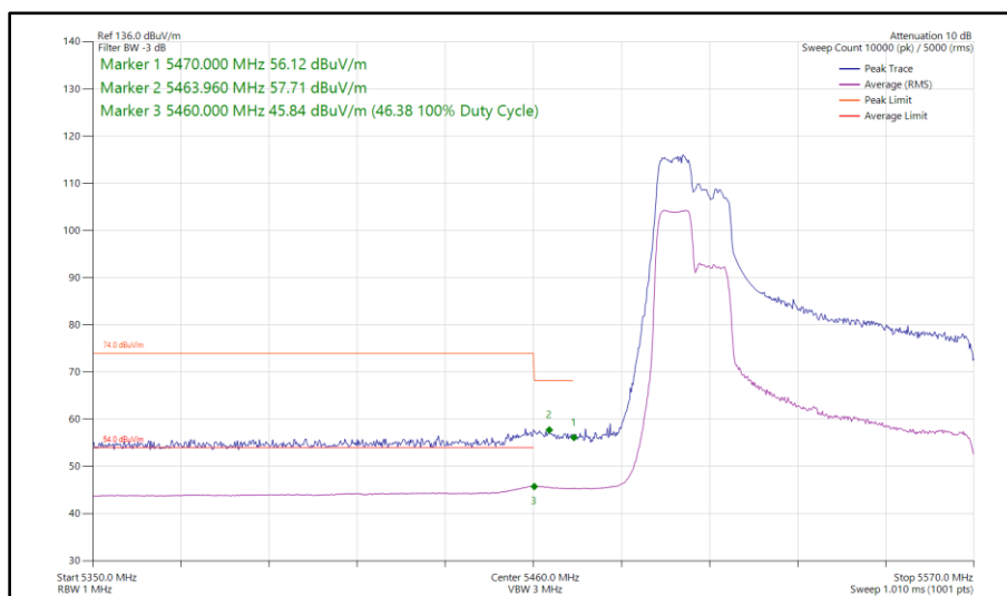
Figure 509 - 802.11ax HE80, RU 106-53, SISO, Core 1 - 5530 MHz Band Edge Frequency 5470 MHz
