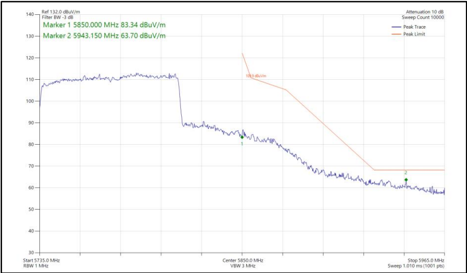
Figure 550 - 802.11ax HE80, SU, SDM, Core 0 - Core 1 - 5775 MHz Band Edge Frequency 5850 MHz
