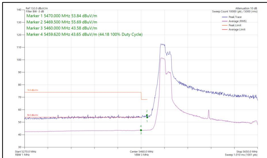
Figure 571 - 802.11ax HE160, RU 106-53P, CDD, Core 0 - Core 1 - 5570 MHz Band Edge Frequency 5470 MHz
