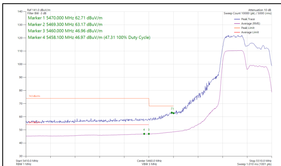
Figure 46 - 802.11ax HE20, RU 106-53, SISO, Core 1 - 5500 MHz Band Edge Frequency 5460 MHz
