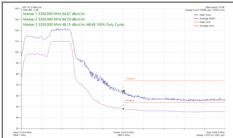
Figure 63 - 802.11ax HE20, RU 106-54, SDM, Core 0 - Core 1 - 5320 MHz Band Edge Frequency 5350 MHz
