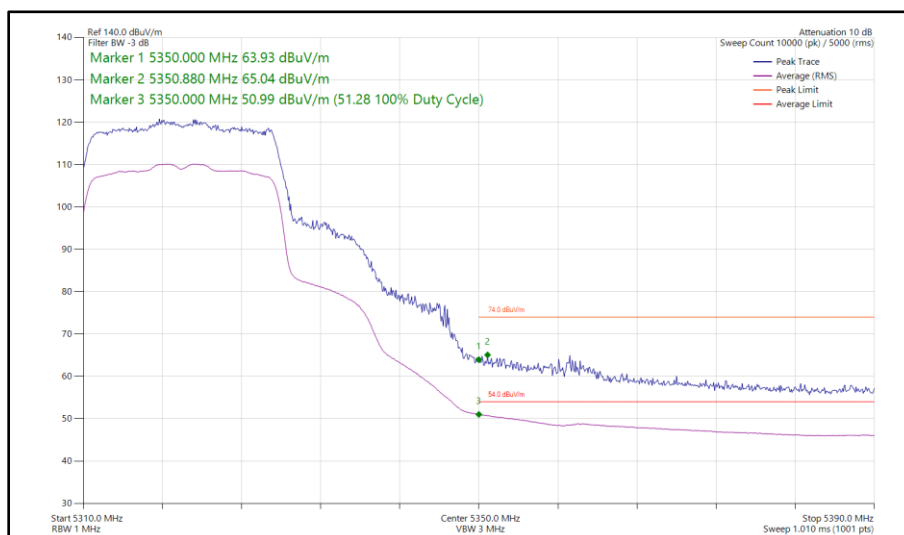
Figure 62 - 802.11ax HE20, SU, SDM, Core 0 - Core 1 - 5320 MHz Band Edge Frequency 5350 MHz
