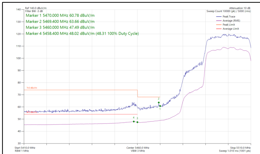
Figure 56 - 802.11ax HE20, SU, CDD, Core 0 - Core 1 - 5500 MHz Band Edge Frequency 5460 MHz
