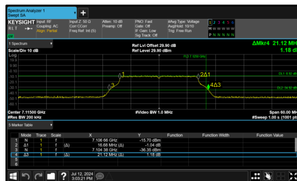
Figure 22 - 802.11a LPI Maximum 99% OBW
