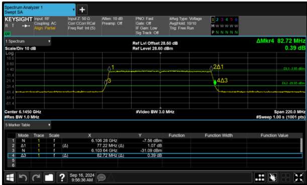
Figure 73 - 802.11ax HE80 SU VLP Minimum 99% OBW
