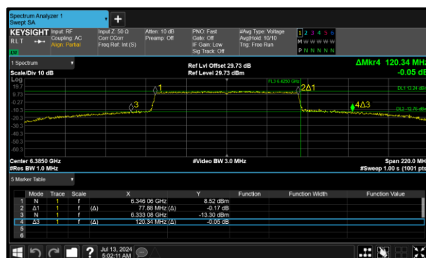
Figure 66 - 802.11ax HE80 SU SP Maximum 99% OBW
