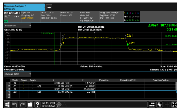
Figure 136 - 802.11ax HE160 SU SP Maximum 99% OBW
