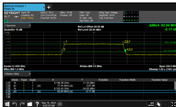
Figure 102 - 802.11ax HE80 SU VLP Maximum 99% OBW
