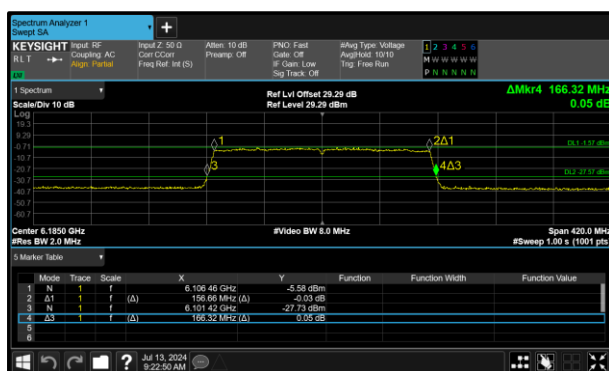
Figure 97 - 802.11ax HE160 SU VLP Minimum 26 dB EBW
