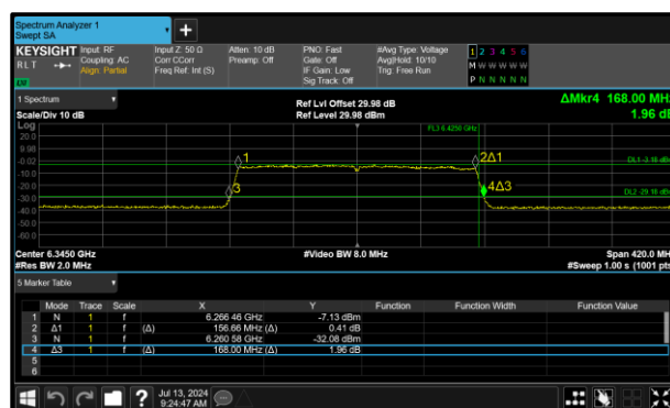
Figure 98 - 802.11ax HE160 SU VLP Maximum 26 dB EBW
