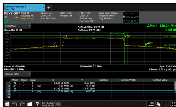
Figure 134 - 802.11ax HE80 SU SP Maximum 99% OBW
