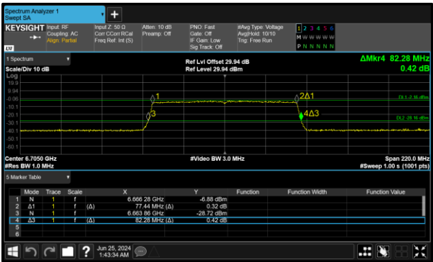
Figure 155 - 802.11ax HE80 SU LPI Minimum 26 dB EBW
