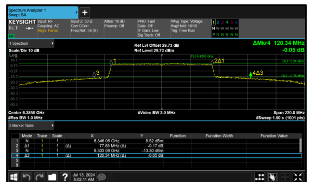
Figure 134 - 802.11ax HE80 SU SP Maximum 99% OBW
