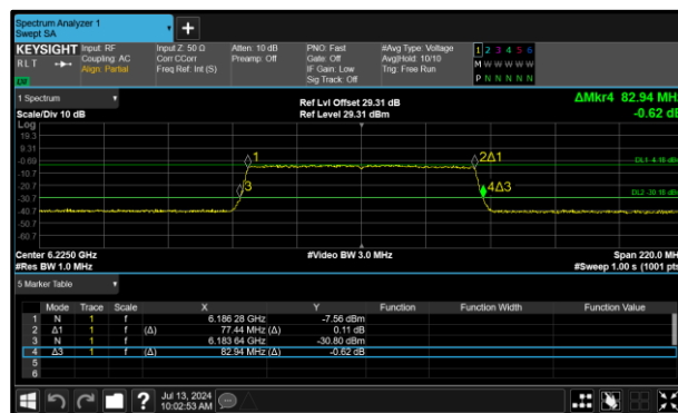
Figure 142 - 802.11ax HE80 SU VLP Maximum 26 dB EBW
