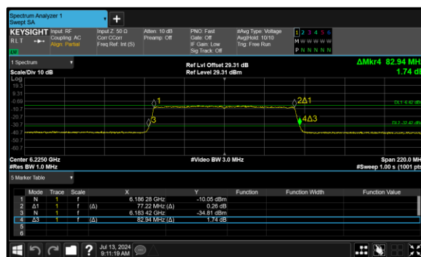
Figure 96 - 802.11ax HE80 SU VLP Maximum 26 dB EBW
