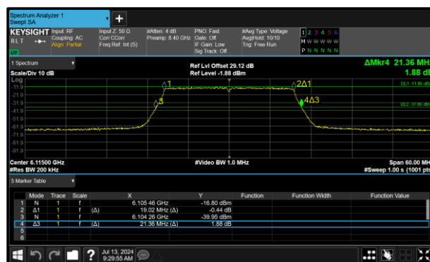
Figure 138 - 802.11ax HE20 SU VLP Maximum 26 dB EBW
