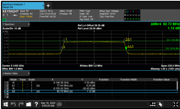
Figure 150 - 802.11ax HE80 SU VLP Maximum 99% OBW
