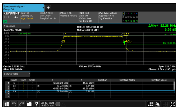
Figure 95 - 802.11ax HE80 SU VLP Minimum 26 dB EBW
