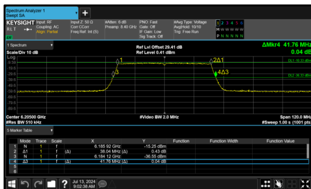
Figure 93 - 802.11ax HE40 SU VLP Minimum 26 dB EBW
