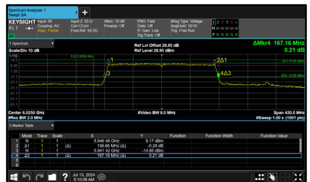
Figure 136 - 802.11ax HE160 SU SP Maximum 99% OBW
