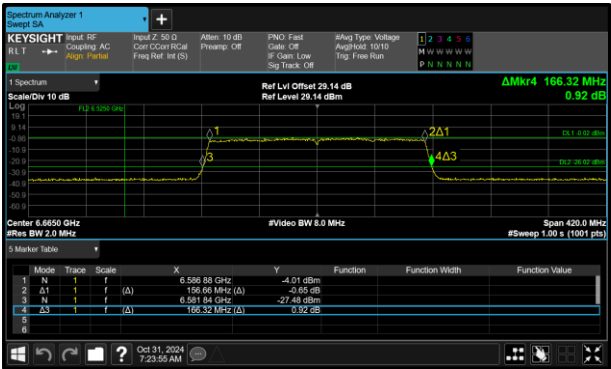
Figure 143 - 802.11ax HE160 SU VLP Minimum 26 dB EBW
