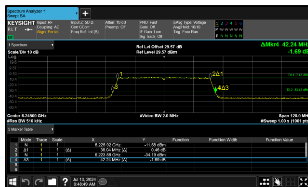
Figure 140 - 802.11ax HE40 SU VLP Maximum 26 dB EBW
