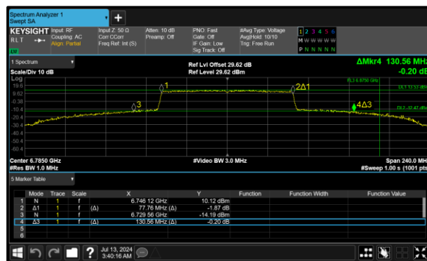
Figure 90 - 802.11ax HE80 SU SP Maximum 99% OBW
