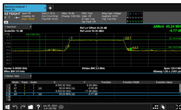
Figure 160 - 802.11ax HE40 SU SP Maximum 26 dB EBW
