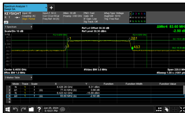
Figure 162 - 802.11ax HE80 SU SP Maximum 26 dB EBW
