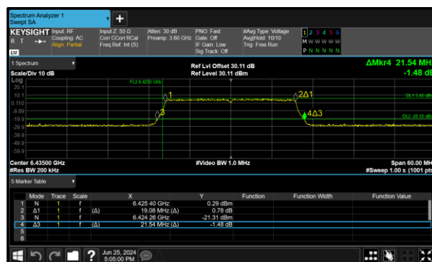
Figure 158 - 802.11ax HE20 SU SP Maximum 26 dB EBW
