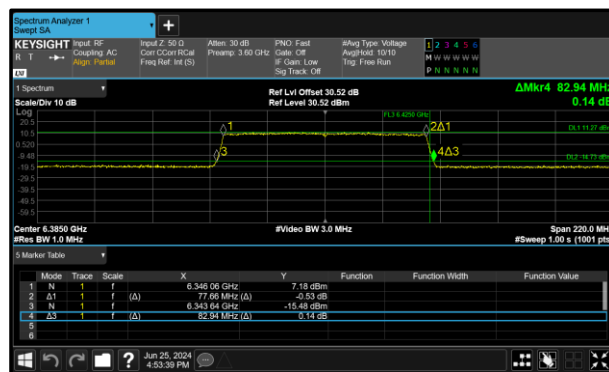
Figure 172 - 802.11ax HE80 SU SP Maximum 99% OBW
