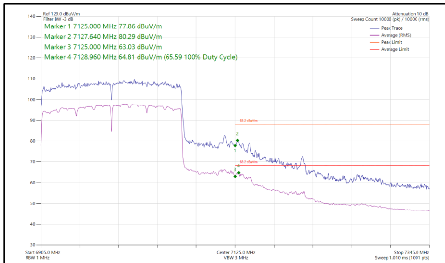
Figure 252 - 802.11ax HE160, SU, SISO, Core 1 - 6985 MHz Band Edge Frequency 7125 MHz
