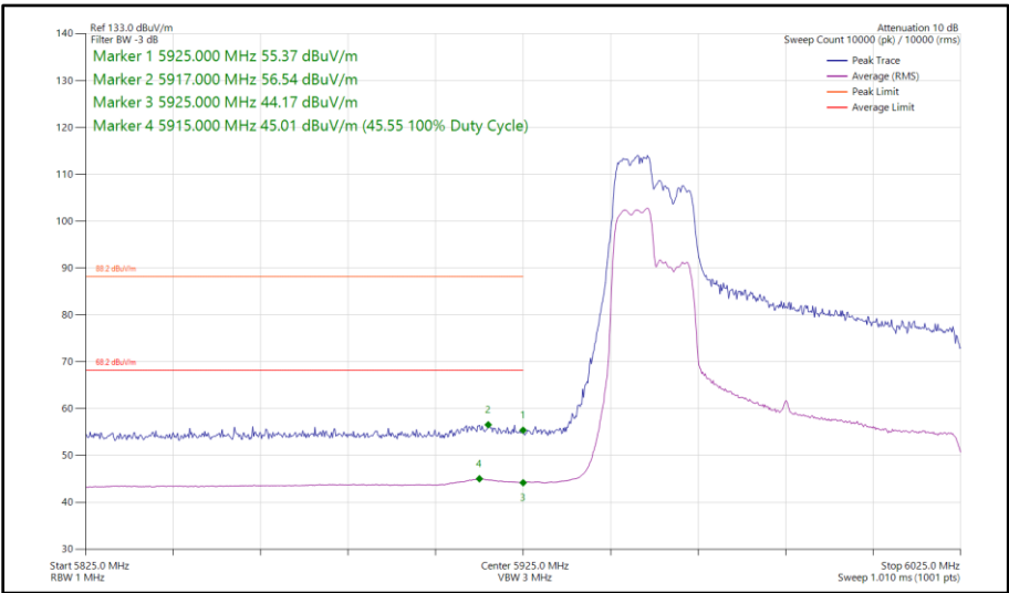
Figure 235 - 802.11ax HE80, RU 106-53, CDD, Core 0 - Core 1 - 5985 MHz Band Edge Frequency 5925 MHz
