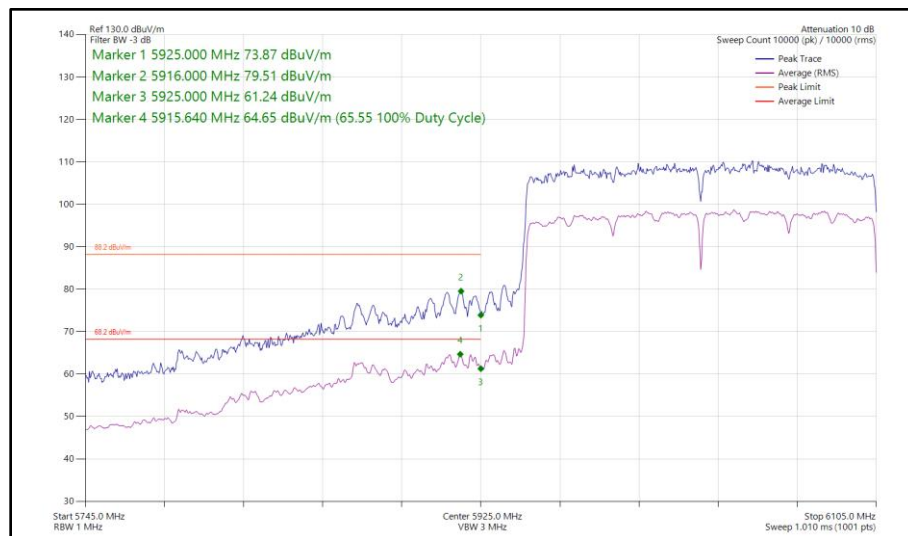
Figure 258 - 802.11ax HE160, SU, SDM, Core 0 - Core 1 - 6025 MHz Band Edge Frequency 5925 MHz
