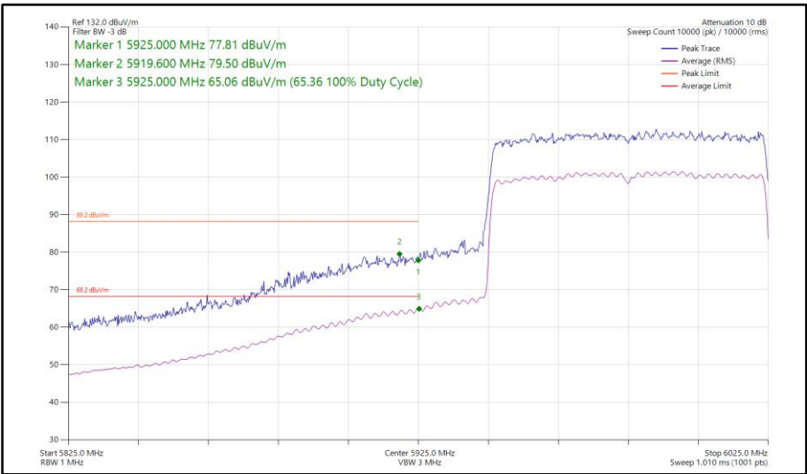
Figure 234 - 802.11ax HE80, SU, CDD, Core 0 - Core 1 - 5985 MHz Band Edge Frequency 5925 MHz
