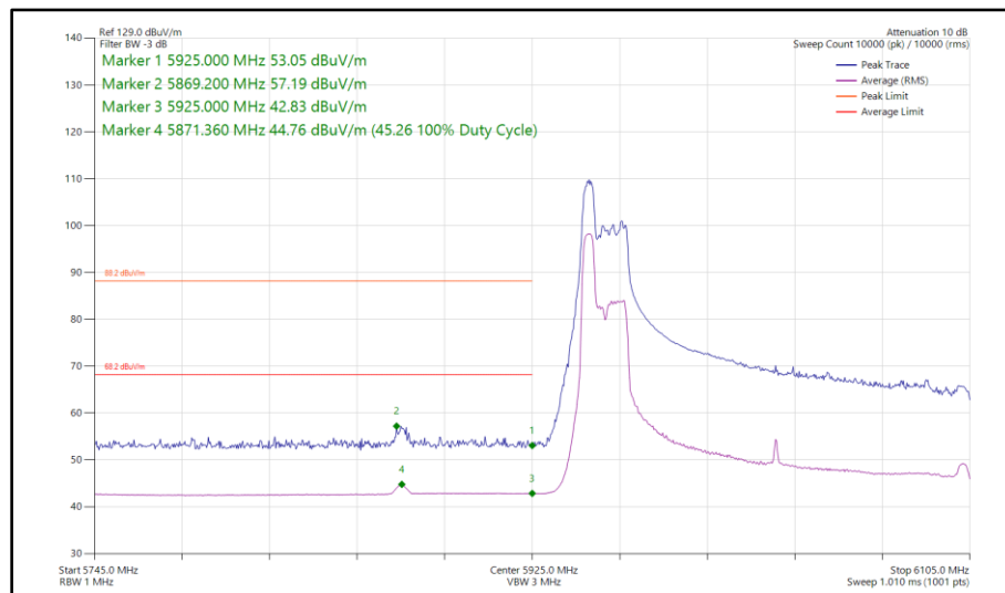
Figure 251 - 802.11ax HE160, RU 52-37P, SISO, Core 1 - 6025 MHz Band Edge Frequency 5925 MHz
