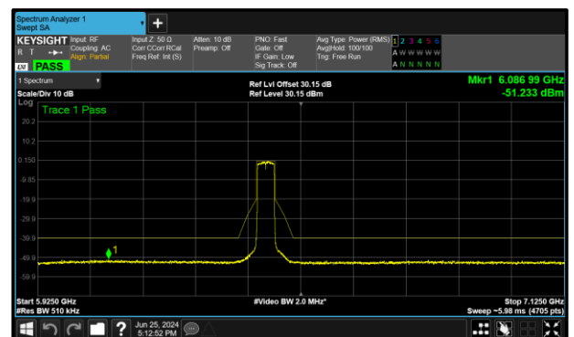
Figure 332 - B (Core 1) 6445 MHz (CH99)
