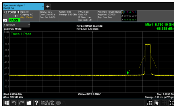
Figure 279 - A (Core 0) 6925 MHz (CH195)
