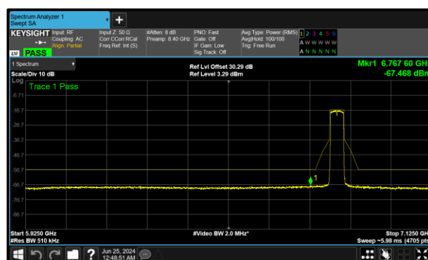
Figure 276 - B (Core 1) 6845 MHz (CH179)
