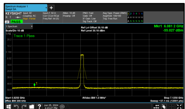
Figure 312 - B (Core 1) 6415 MHz (CH93)
