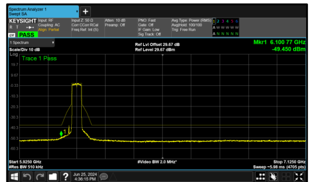
Figure 328 - B (Core 1) 6165 MHz (CH43)
