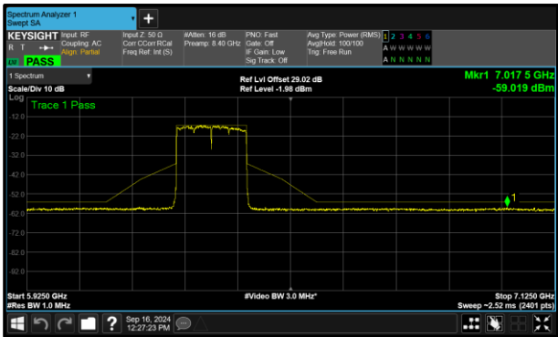
Figure 264 - B (Core 1) 802.11ax HE160 SU VLP 6345 MHz (CH79)
