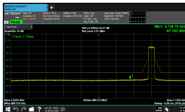
Figure 278 - B (Core 1) 6885 MHz (CH187)
