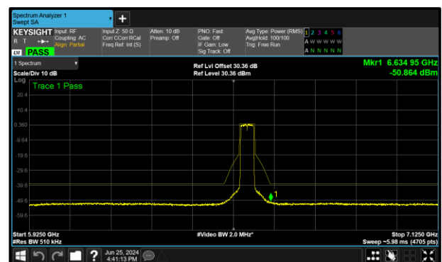
Figure 338 - B (Core 1) 6565 MHz (CH123)
