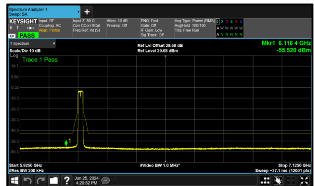
Figure 310 - B (Core 1) 6175 MHz (CH45)
