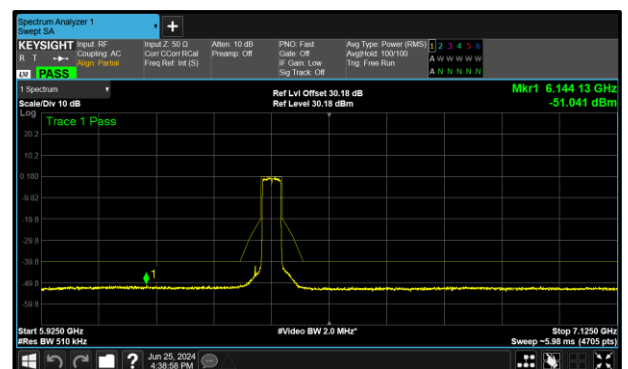
Figure 330 - B (Core 1) 6405 MHz (CH91)
