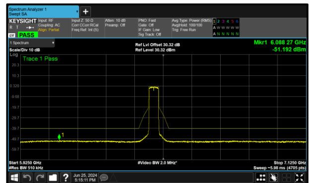
Figure 334 - B (Core 1) 6485 MHz (CH107)
