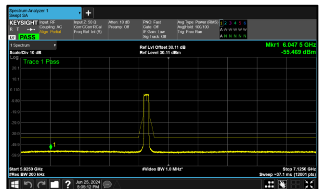
Figure 314 - B (Core 1) 6435 MHz (CH97)
