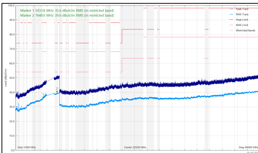
Figure 284 - U-NII-7 - 6695 MHz (CH149), HE20, SU, CDD, Core 0 + Core 1, 1 GHz to 40 GHz, Vertical
