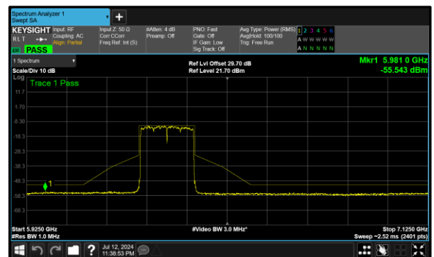
Figure 336 - B (Core 1) 802.11ax HE160 SU LPI 6345 MHz (CH79)
