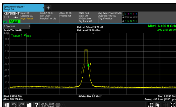
Figure 303 - B (Core 1) 802.11a SP 6475 MHz (CH105)
