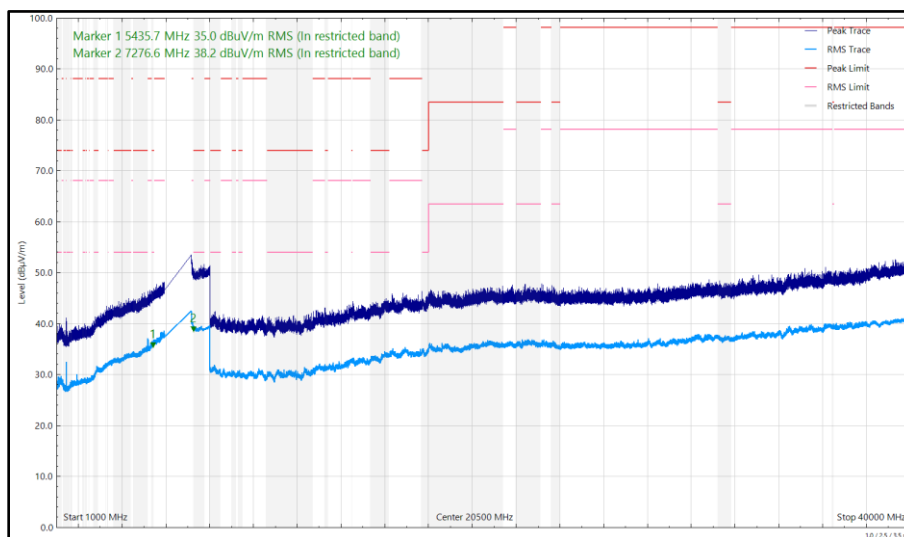
Figure 288 - U-NII-8 - 6895 MHz (CH189), HE20, SU, CDD, Core 0 + Core 1, 1 GHz to 40 GHz, Vertical
