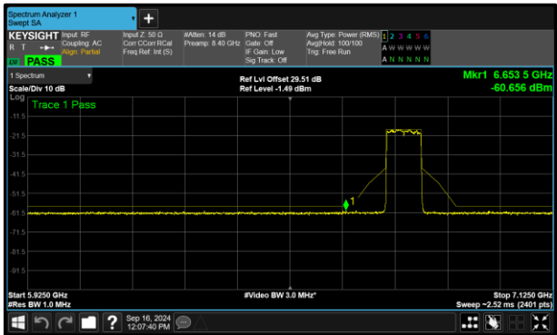
Figure 331 - A (Core 0) 802.11ax HE80 SU VLP 6785 MHz (CH167)
