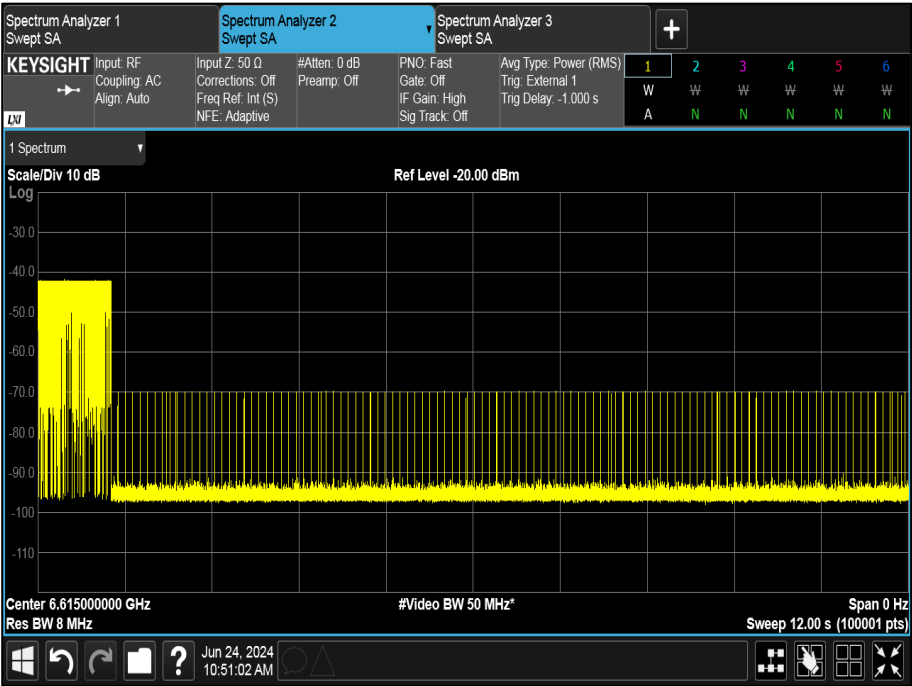
Figure 456 - U-NII-7, Minimum Bandwidth (AWGN Low)
